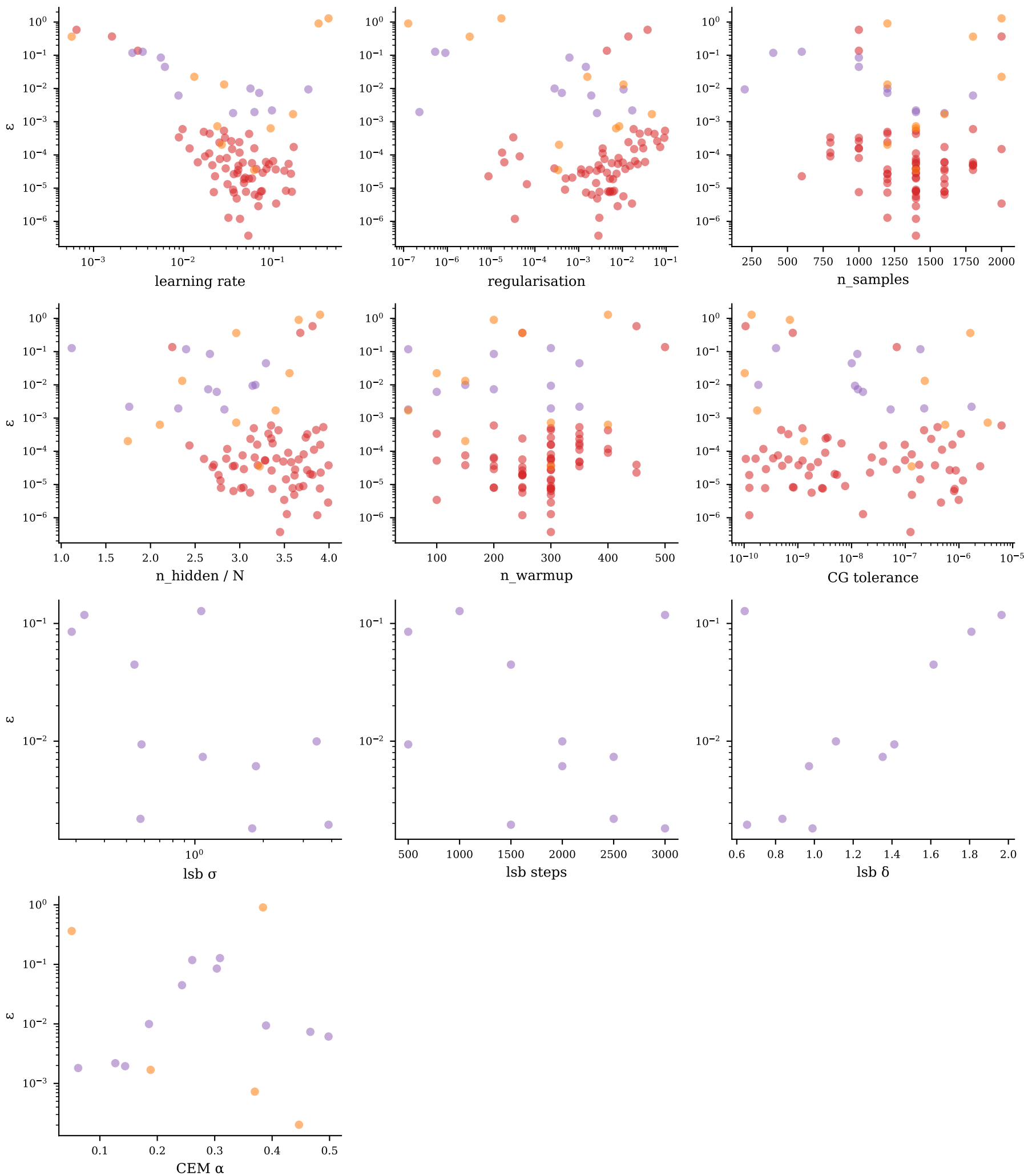
Hyperparameter sensitivity — j1j2_1d/j1j2_1d_20260527_170753/N8_J20.25
