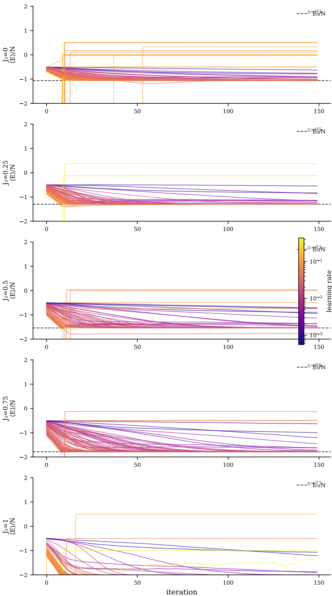
Convergence per J_2 - j1j2\_1d/j1j2\_1d\_20260527\_170753/N8 Each line = one trial · colour = learning rate
