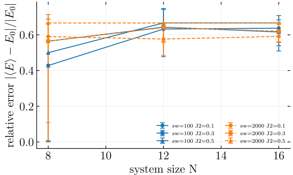
Heisenberg J1J2 1D — FPGA SA (median \pm IQR, 20 seeds)
