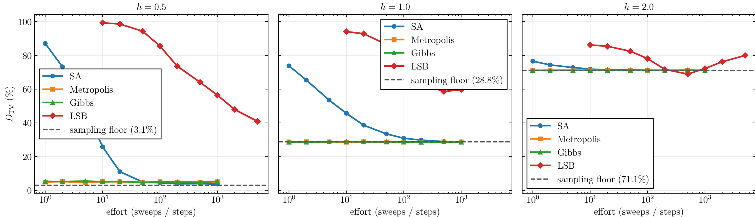
Sampling quality: SA / MH / Gibbs / LSB | TFIM 1D N = 16 n_{\text{samples}} = 10000
