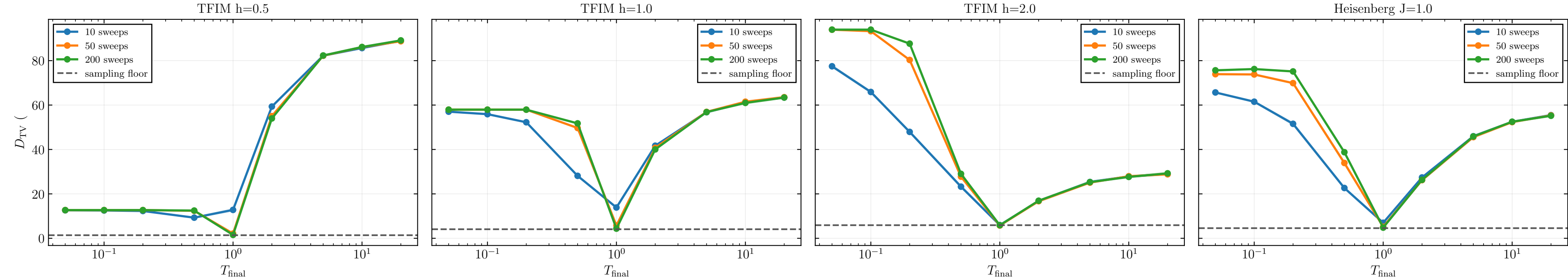
D_{\text{TV}} vs SA final temperature | N=8 n_{\text{samples}} = 10000 T_{\text{initial}} = 5
