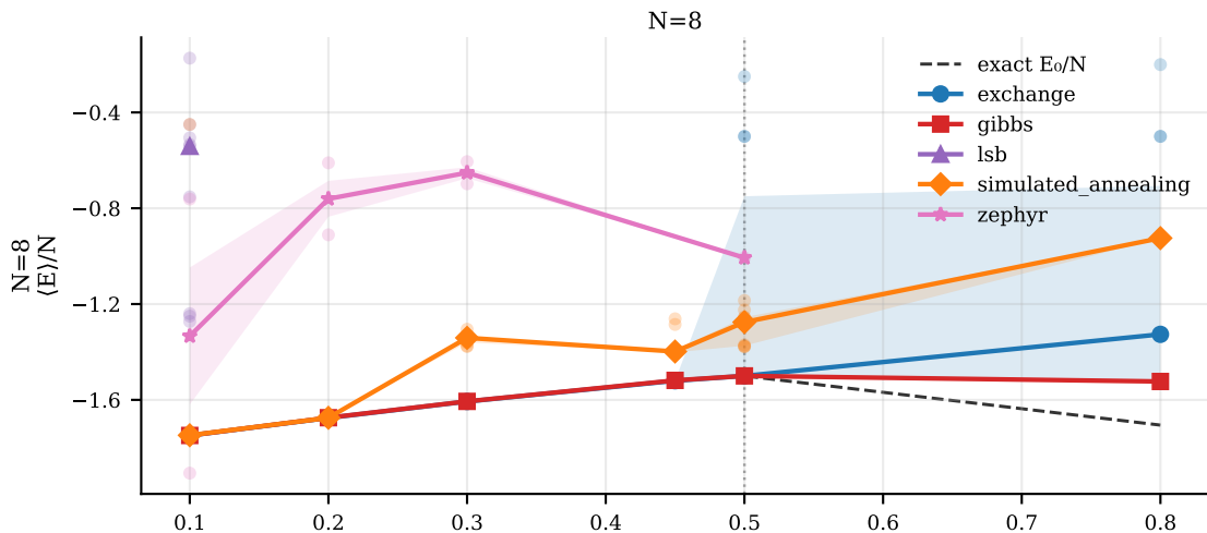
Converged \langle E \rangle / N per spin vs J_2 (heisenberg_j1j2_1d (isotropic Heisenberg)) Median \pm IQR over seeds
