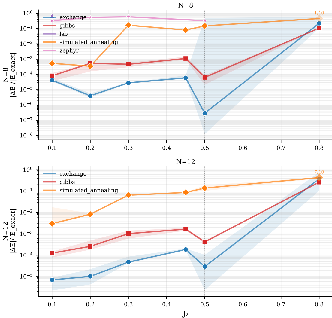
Relative energy error vs J_2 — heisenberg_j1j2_1d (isotropic Heisenberg)
