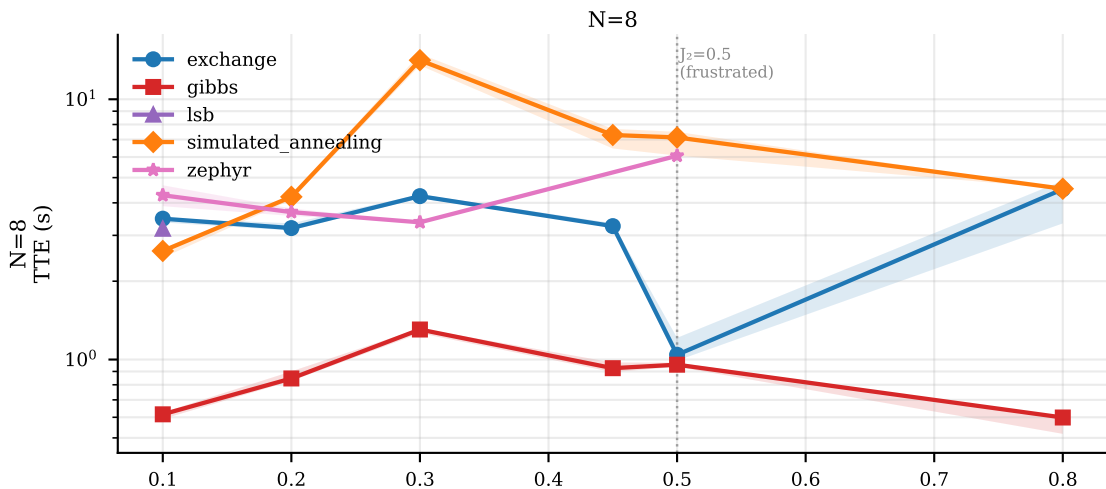
Time-to-Convergence vs J_2 (heisenberg_j1j2_1d (isotropic Heisenberg)) rolling std < 1.0%·|E_exact|, window=20
