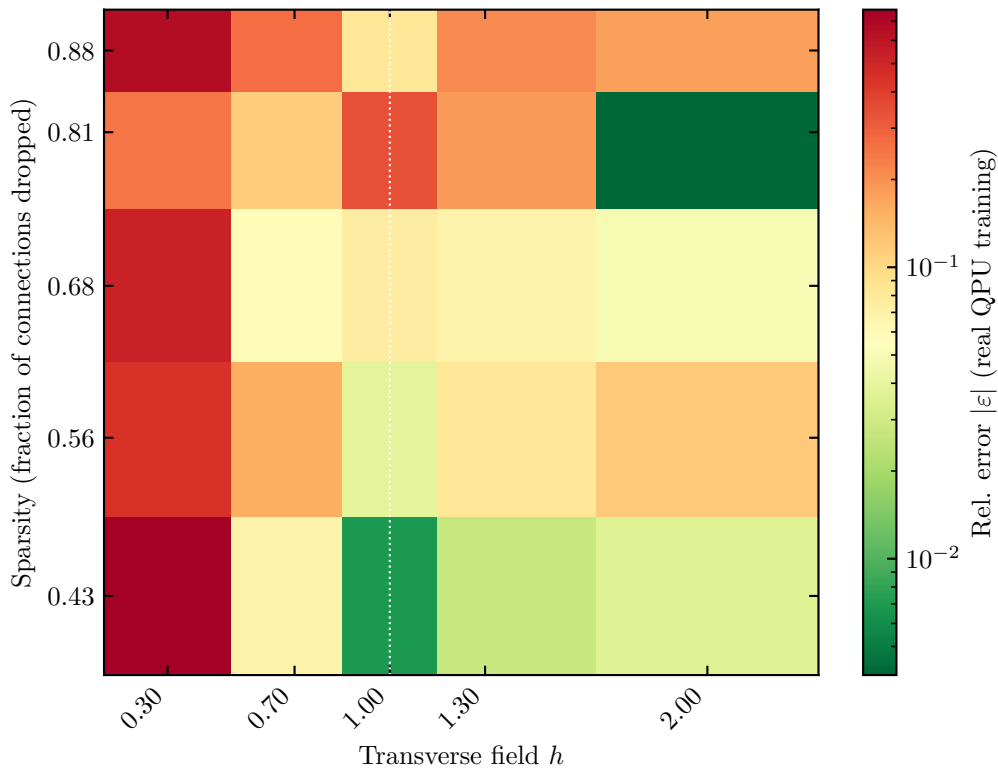
Zephyr, N = 16 — REAL QPU-trained accuracy
