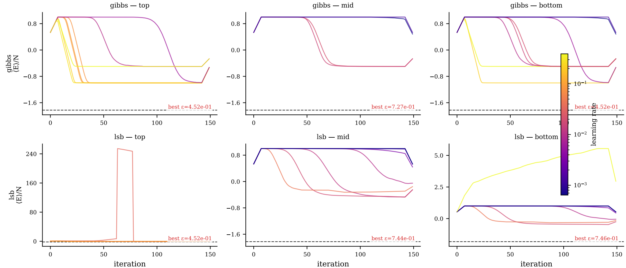
Convergence: top / mid / bottom 8 trials — heisenberg_xxz_1d/heisenberg_xxz_1d_20260527_150056/N8_delta1.0 Colour = learning rate
