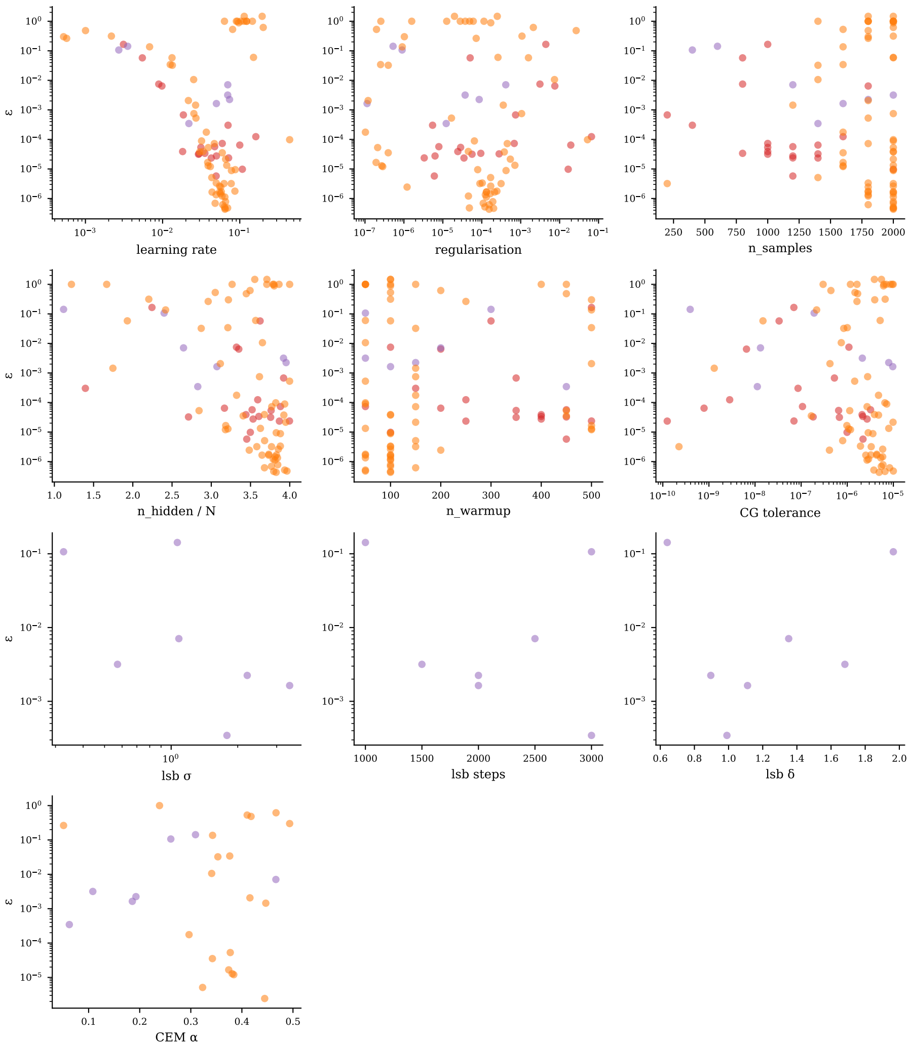
Hyperparameter sensitivity — j1j2_1d/j1j2_1d_20260527_152843/N8_J20.0
