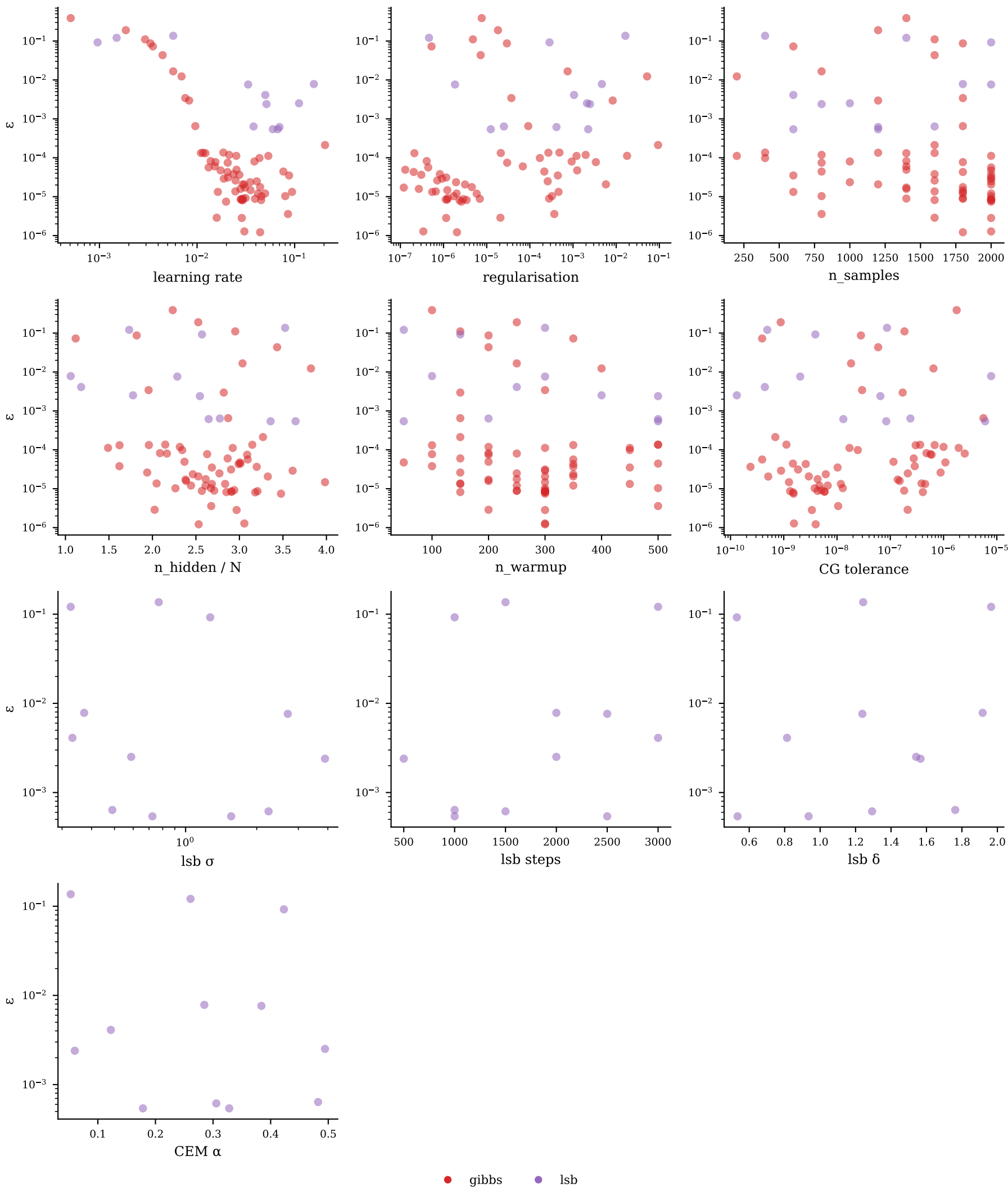
Hyperparameter sensitivity — j1j2_1d/j1j2_gibbs_lsb_v1/N8_J20.0
