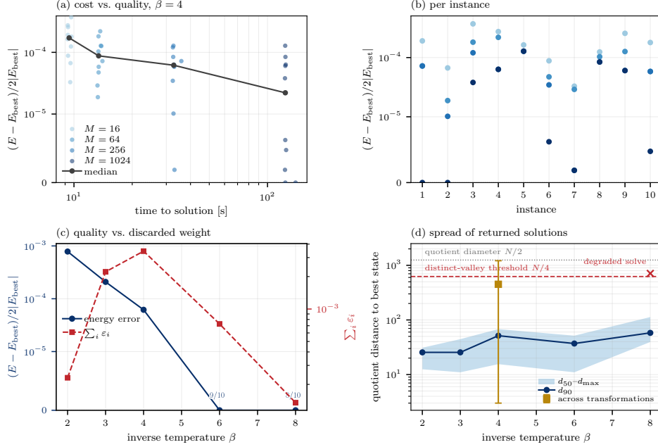
Figure 1: Ten 2500-spin ( 50 \times 50 ) square-lattice instances at bond dimension 8, on CPU. (a) Time to solution against relative energy error as the search breadth M = \text{max.states} varies over 16–1024; points are individual instances, the line their median. (b) The same runs resolved per instance. (c) Median energy error and median discarded weight \sum_i \varepsilon_i against \beta ; annotations count instances reaching the best energy found. E_{\text{best}} is the lowest energy over all settings here, not a certified optimum, so a zero error means “best found”, not “optimal”. The two curves in (c) diverge: quality improves monotonically with \beta while discarded weight peaks at \beta = 4 and then falls. (d) How far apart the returned solutions actually are, at M = 1024 . These instances carry no local fields, so E(\sigma) = E(-\sigma) exactly and every state has a degenerate mirror at Hamming distance N ; distances are therefore quotient distances \min(d, N - d) , on a space of diameter N/2 . Band and line are medians over the ten instances of the 50th, 90th and 100th percentile of the distance from each returned state to the best one. The whole returned set is a single tight cluster, one to two orders of magnitude below the N/4 threshold a diversity count would apply. The one point clearing it ( \beta = 8 , instance 1) is a degraded contraction — its energy is 8 above that instance’s best and it fails to return even the exact mirror — not a second optimum. The square marker asks the same question across contraction orders instead: one state from each of the eight lattice transformations, \beta = 4 , median over five instances of the pairwise minimum, median and maximum. Eight states from eight orders span the configuration space; 1024 states from one order do not.
