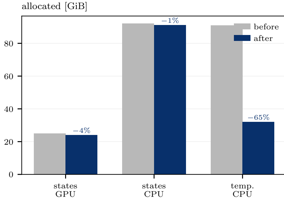
Figure 3: Allocated memory before and after the two allocation changes, on a 2048-spin bond-32 solve; percentages are the reduction. “states” is the matrix-backed branched configuration set, “temp.” the off-heap contraction temporaries. The temporaries change removes about two-thirds of the CPU heap; the states change is small in bytes because its benefit is a reduced live-object count rather than volume. Allocated bytes are hardware-independent — the H100 run reproduces the post-change figures (32.3 GiB CPU, 24.1 GiB GPU).
