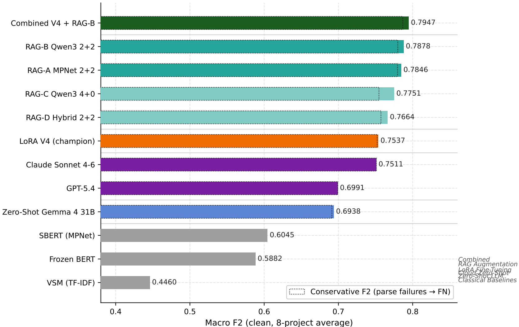
Fig 1 — Overall Performance Comparison: All Methods
