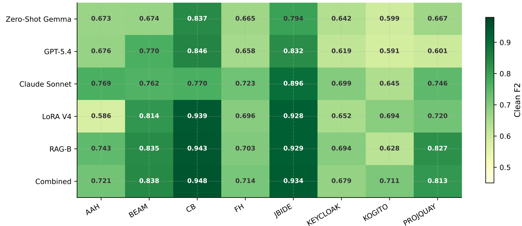
Fig 2 — Per-Project F2 Heatmap (Key Methods)
