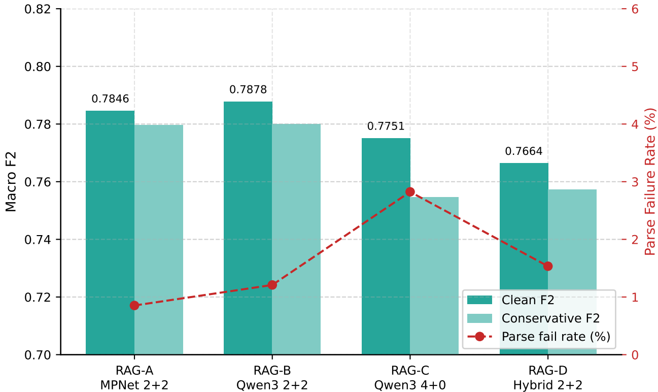
Fig 3 — RAG Ablation Study (A-D)
