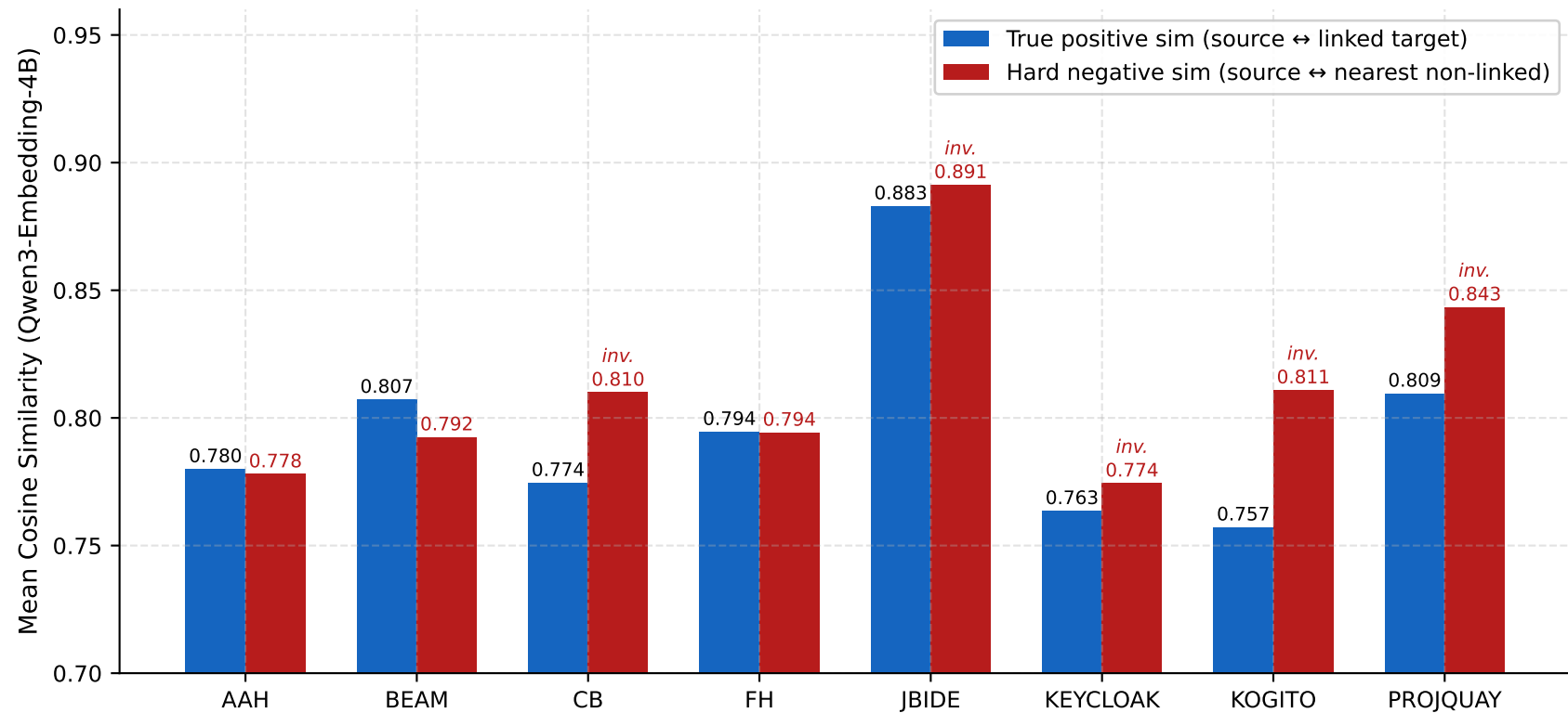
Fig 7 — Similarity Inversion: Hard Negatives vs True Positives (Test Split)
