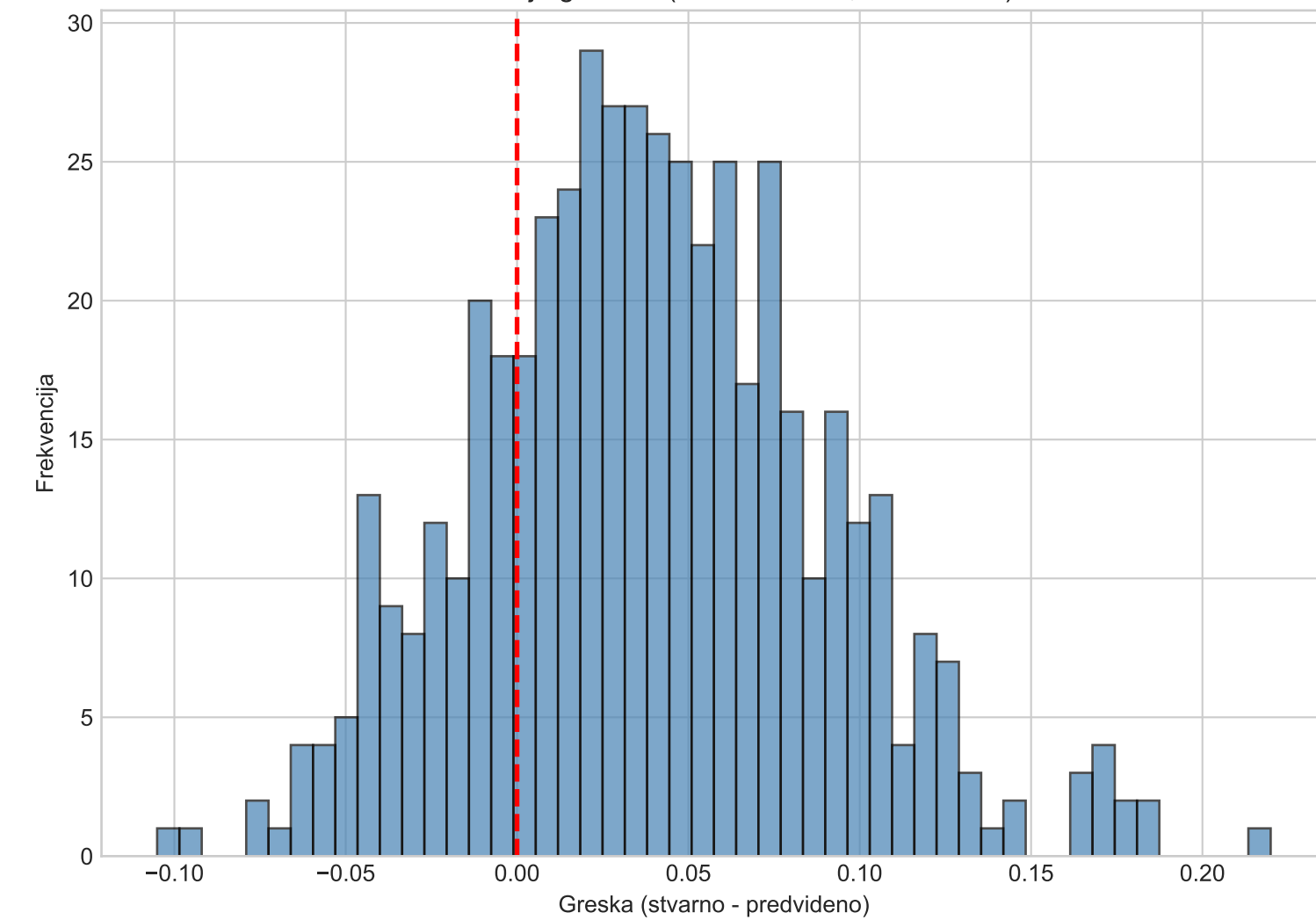
Distribucija gresaka (mean=0.0386, std=0.0505)
