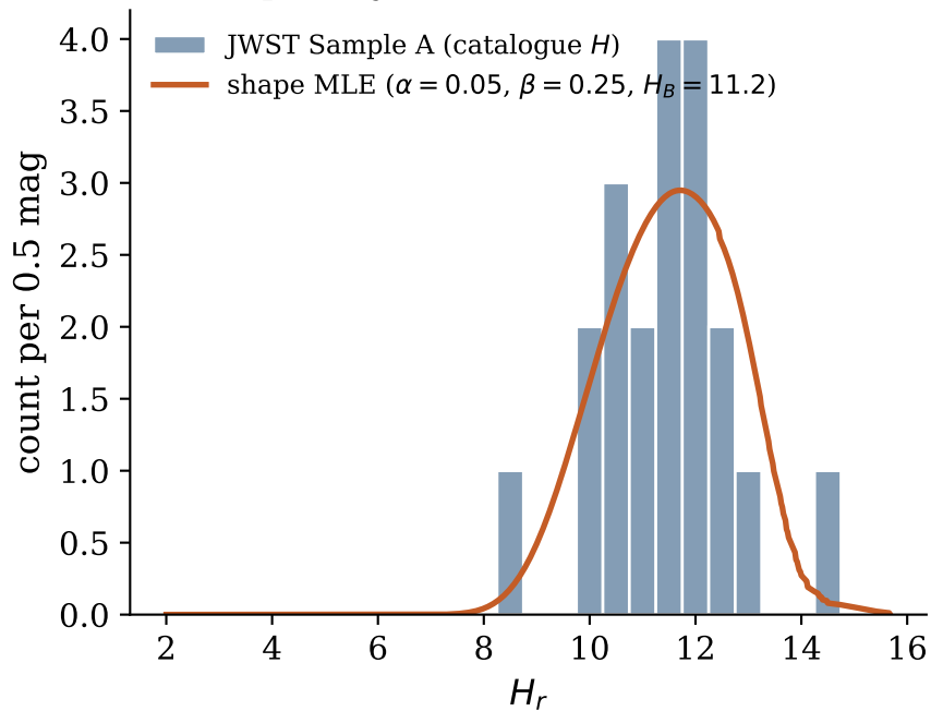
Shape-only fit, no measurement error
