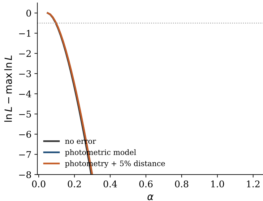
Likelihood slice in \alpha (Sample A, n = 20 )
