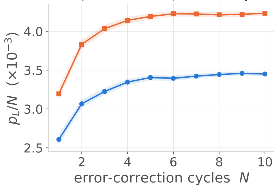
(c) cycle scan at p = 10^{-3} , |0\rangle_L
