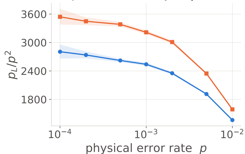
(a) p scan, memory in |0\rangle_L
