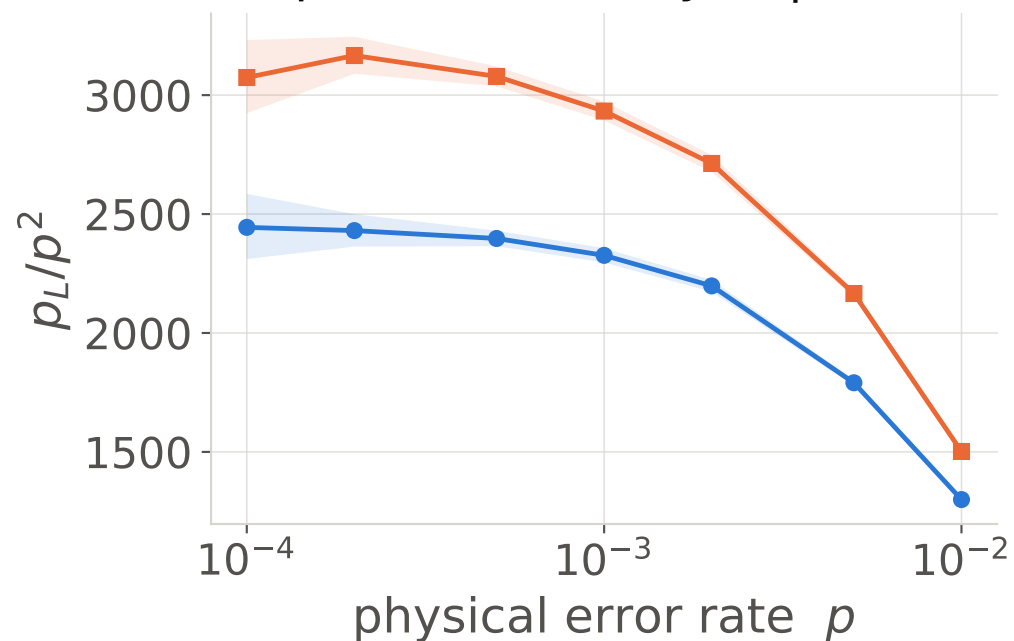
(b) p scan, memory in |+\rangle_L
