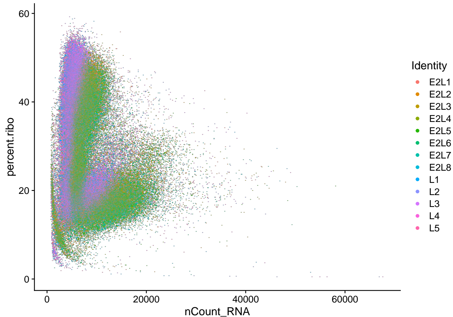
pre_QC: nCount_RNA vs percent.ribo
