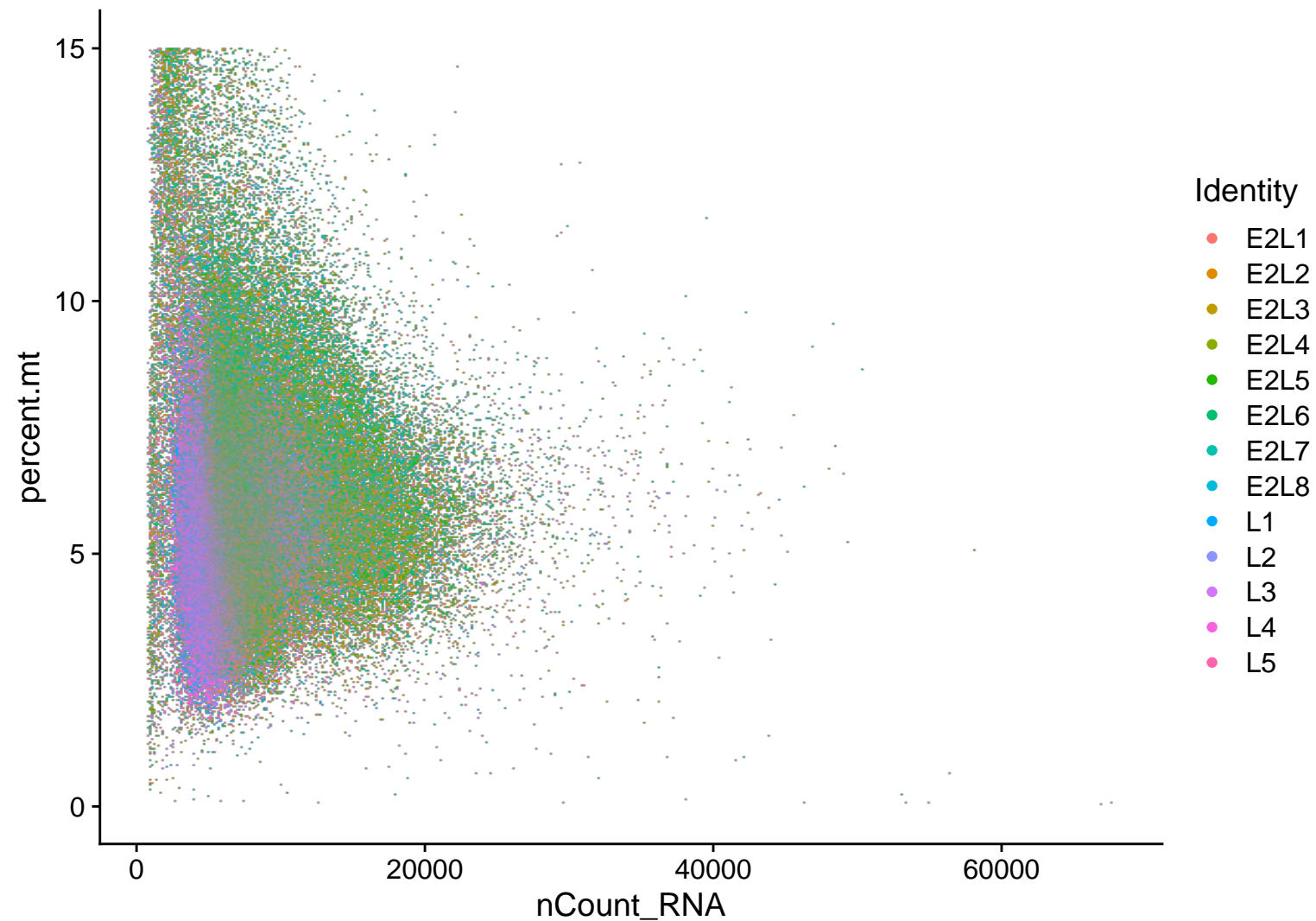
pre_QC: nCount_RNA vs percent.mt
