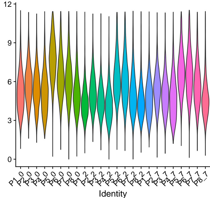
Post-QC: nCount_RNA & percent_final.mt per sa
