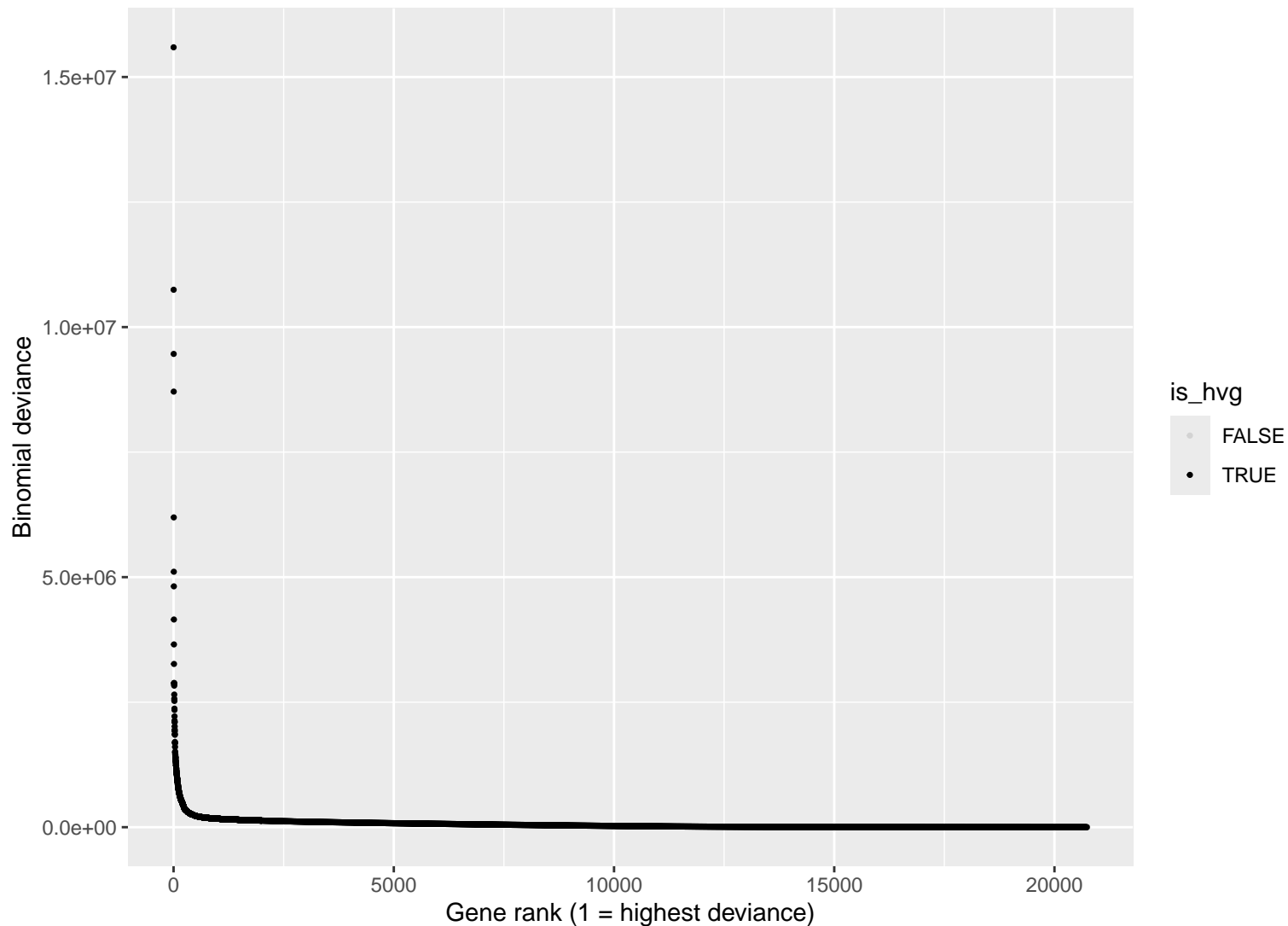
Deviance feature selection: rank vs deviance
