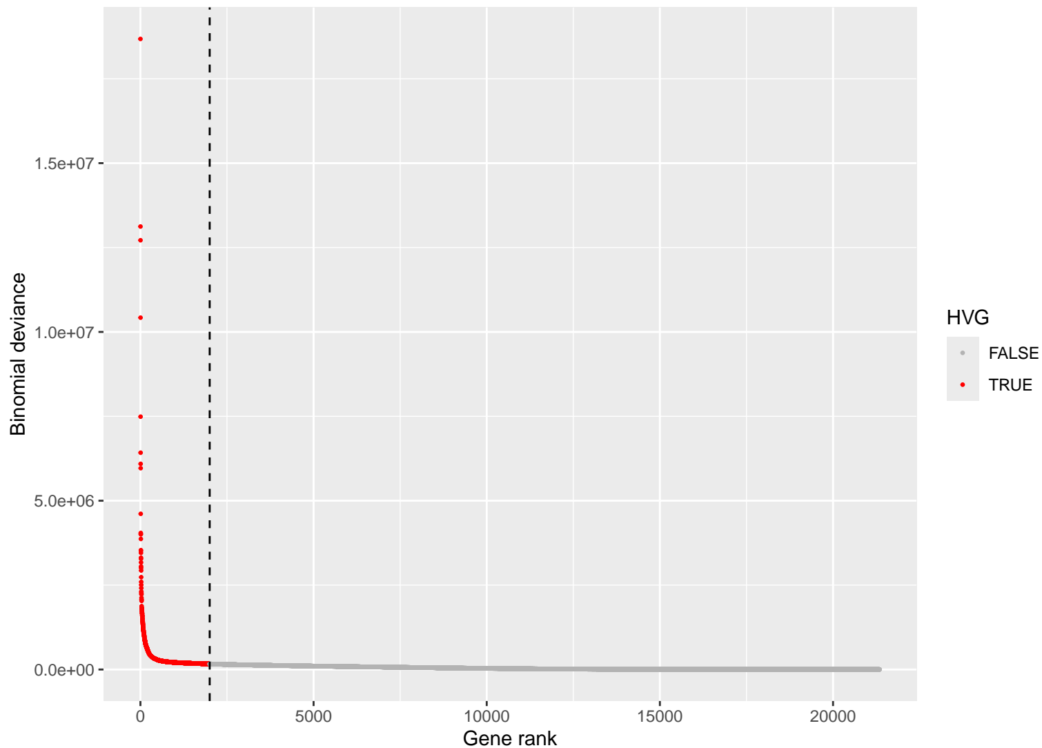
HVG selection by deviance (top 2000 highlighted)
