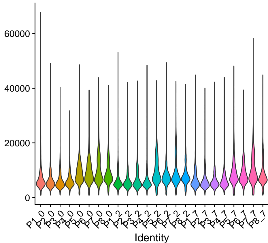
nCount_RNA
