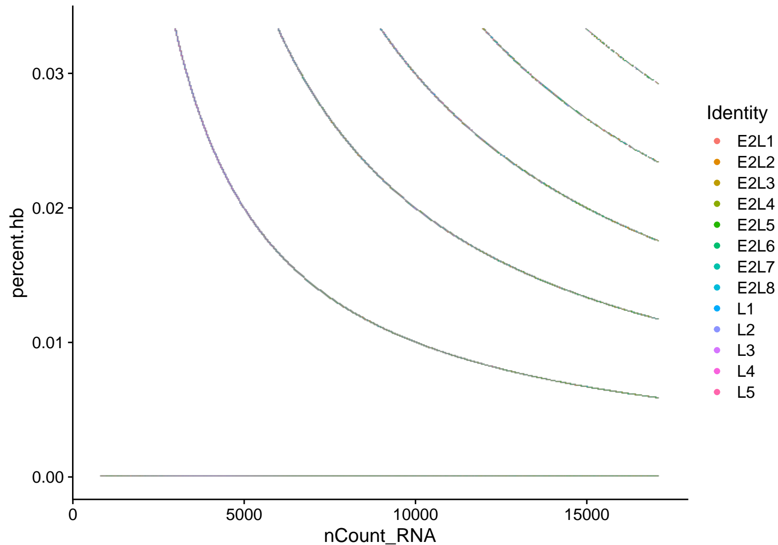
post_QC: nCount_RNA vs percent.hb
