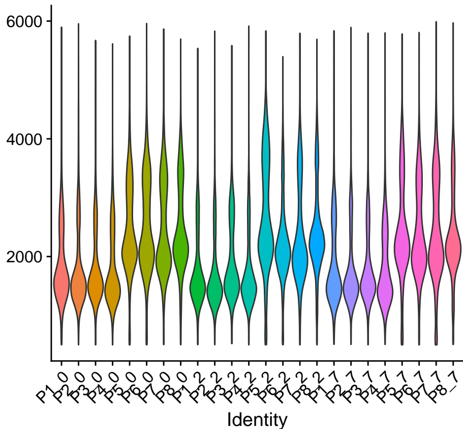
nFeature_RNA
