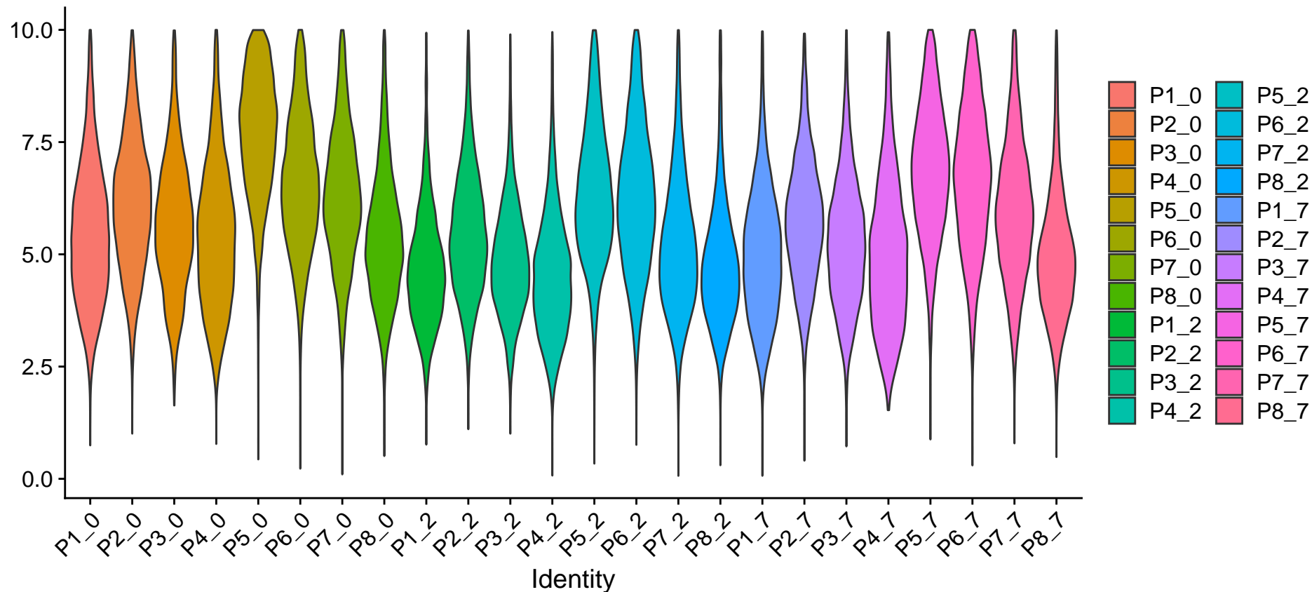
Pre-QC: percent_final.mt per sample
