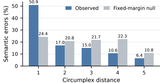
(c) Error locality versus the null
