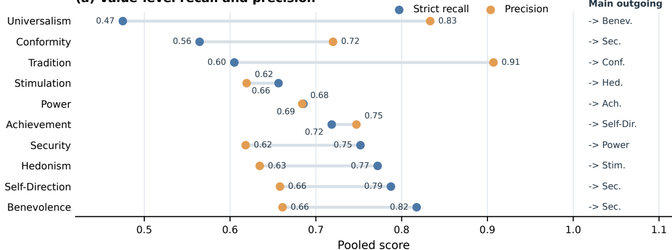
(a) Value-level recall and precision
