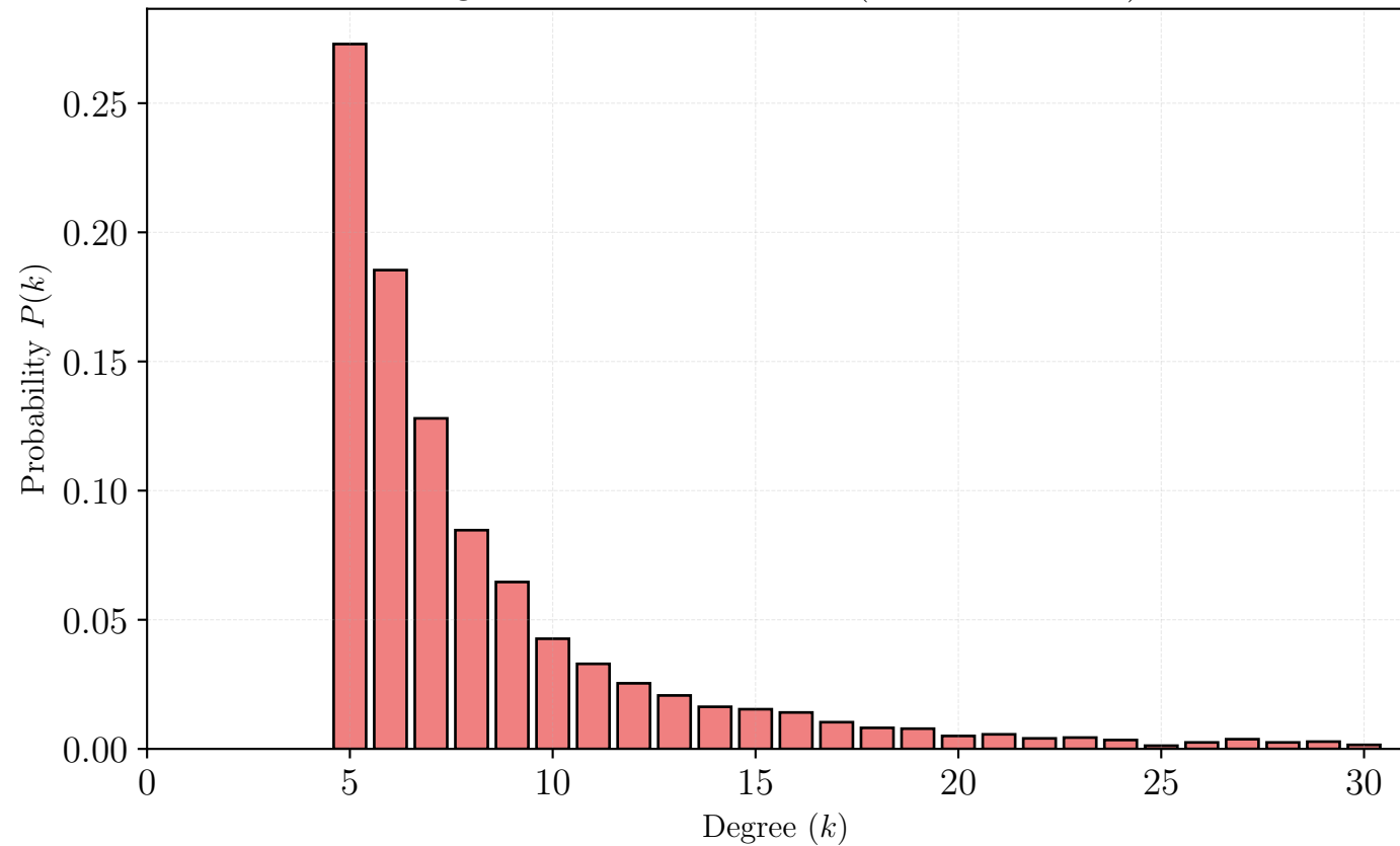
Degree Distribution - PDF (Barabási-Albert)
