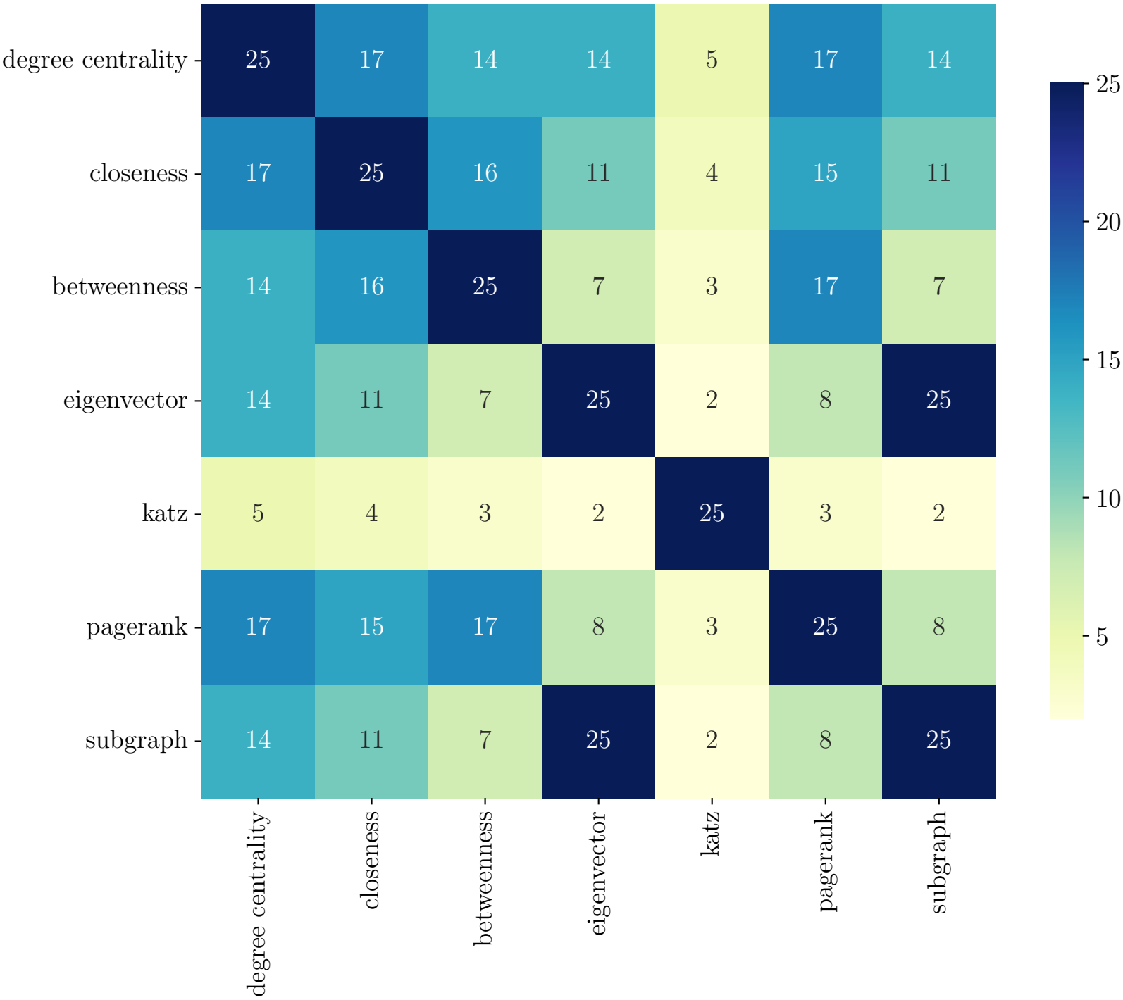
Overlap Matrix of Top 25 Nodes in Centrality Measures
