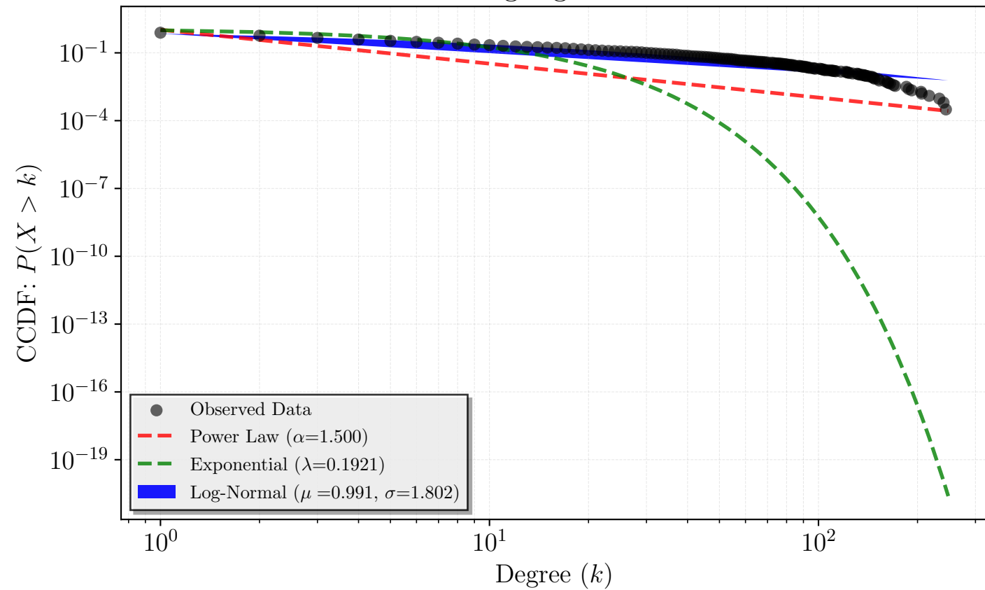
CCDF in log-log scale with fits
