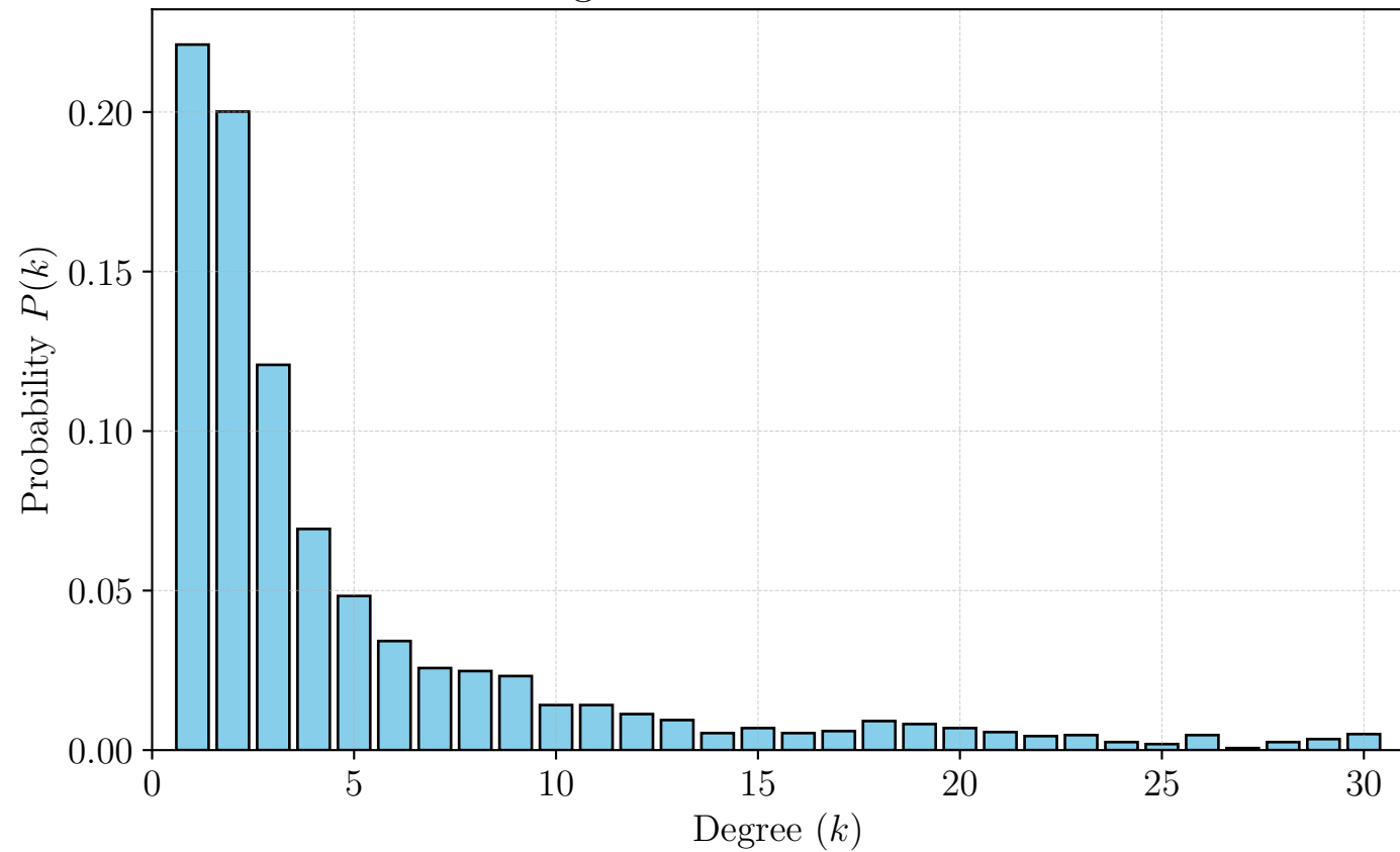
Degree Distribution - PDF
