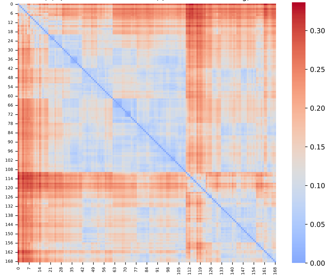
(b) Quantum Distance Matrix (Quantum HRP Ordering)
