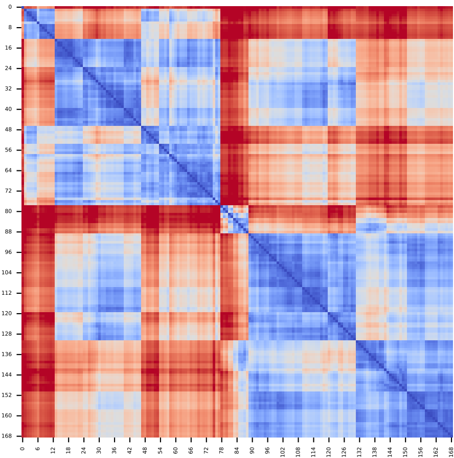
Perm 3
