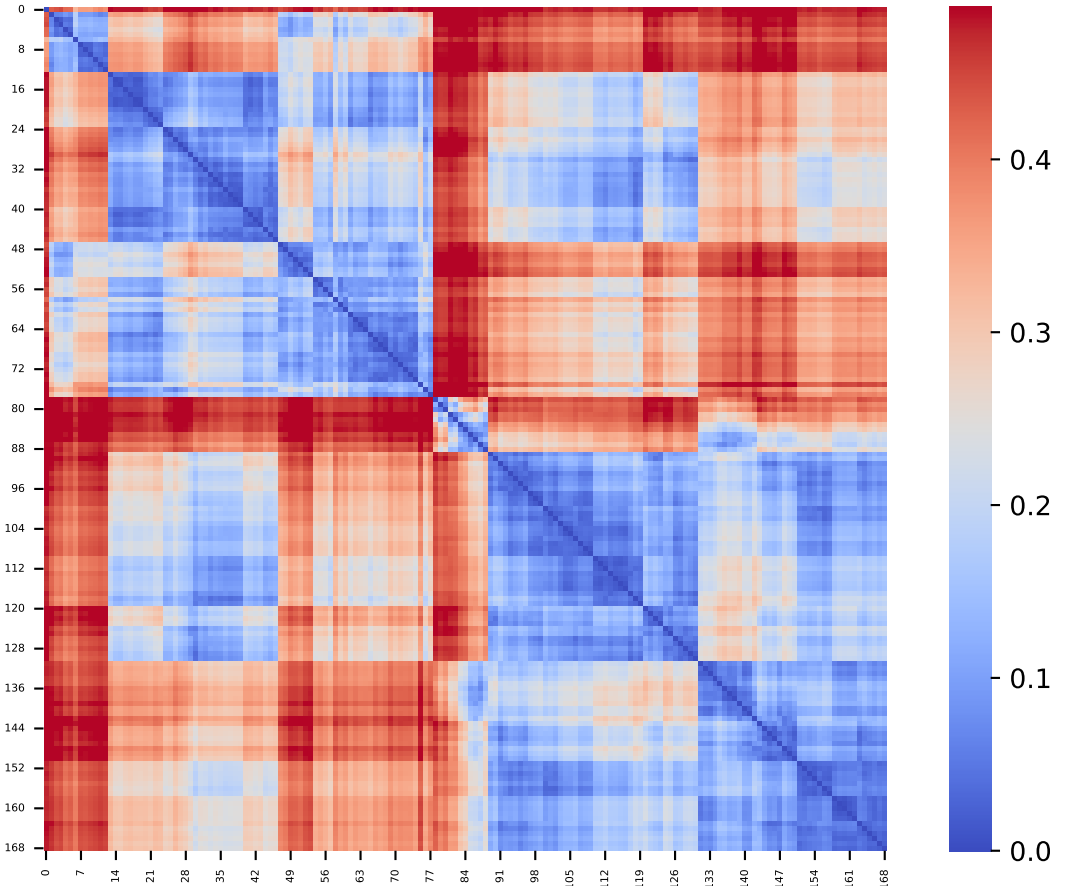
Perm 2
