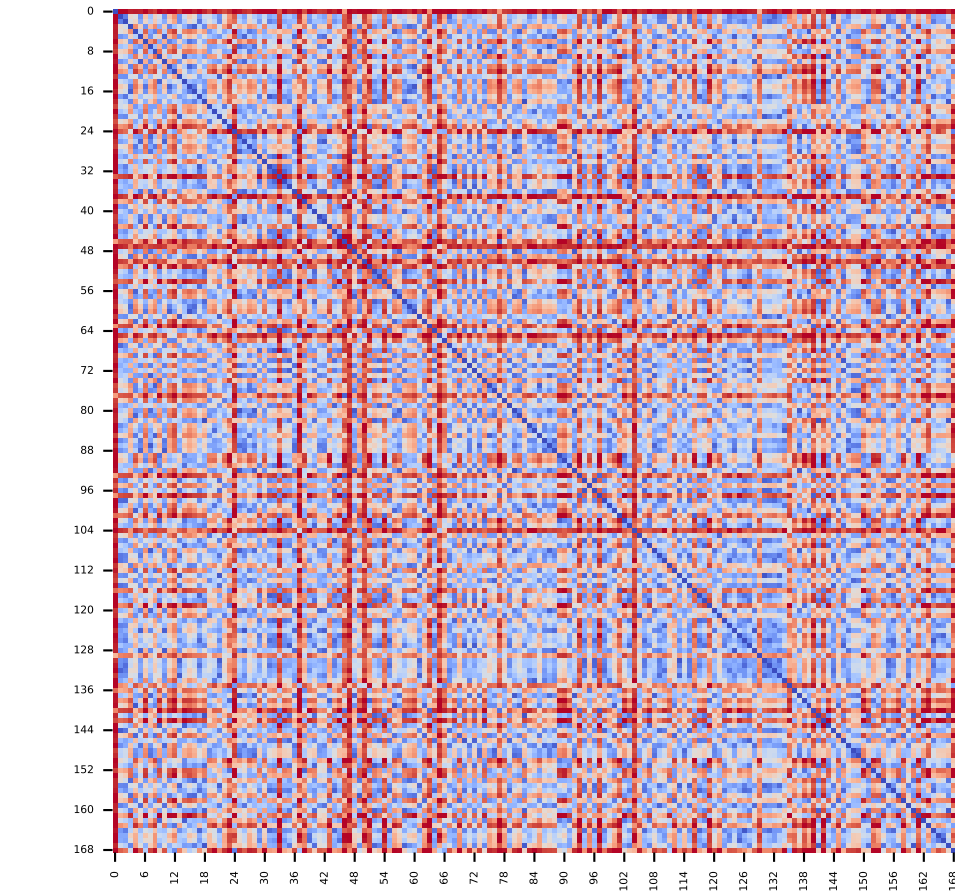
Perm 5 (seed=55)
