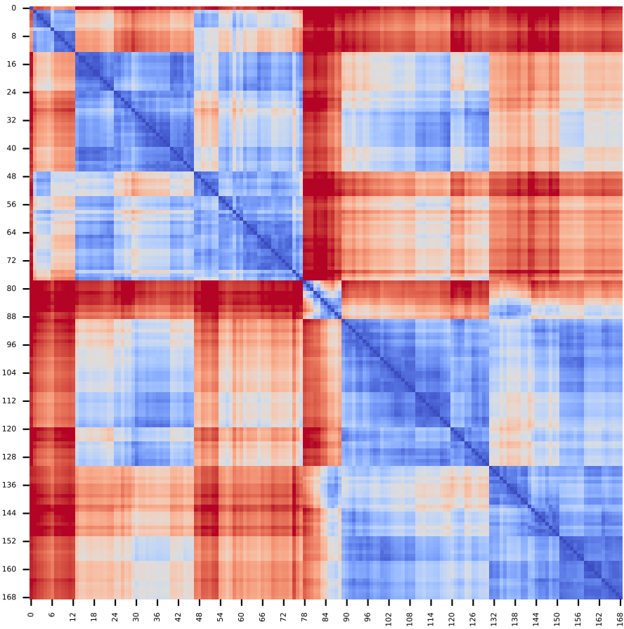
Perm 5
