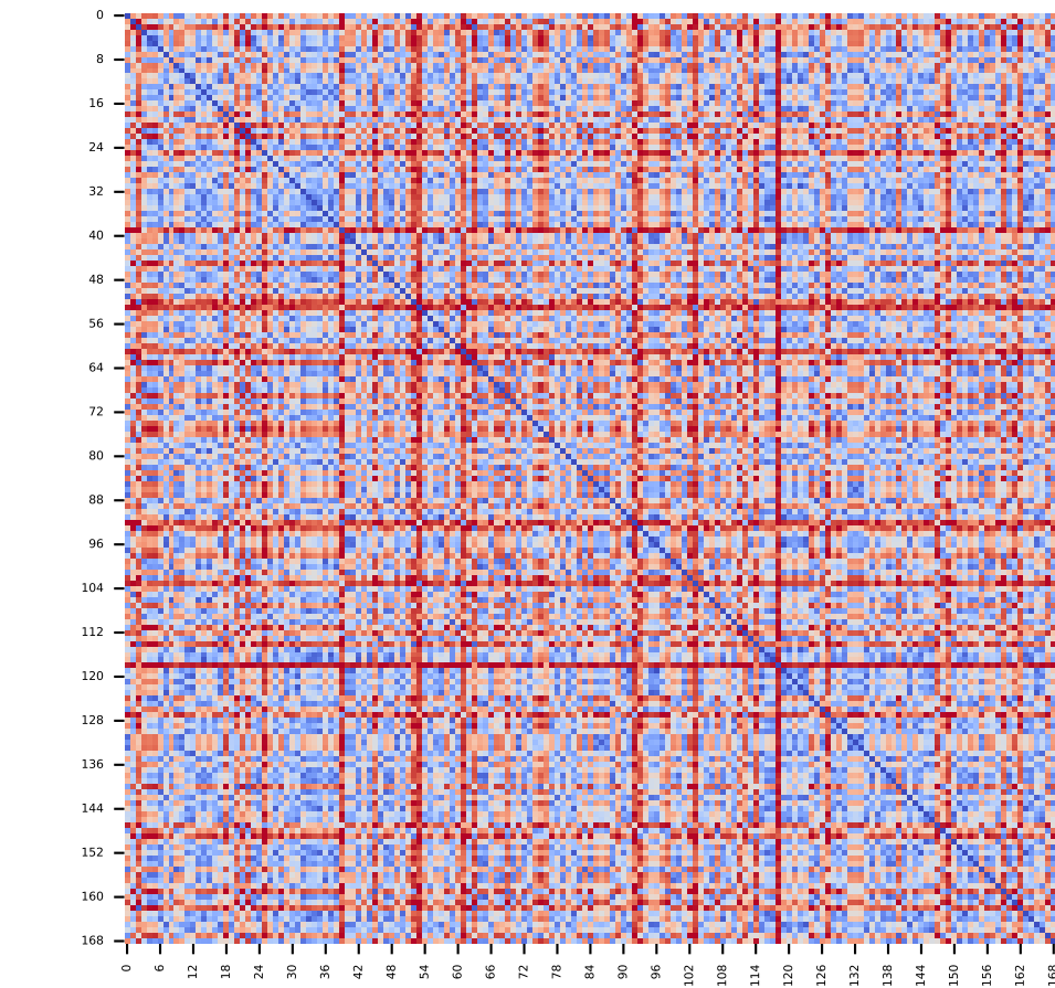
Perm 3 (seed=33)
