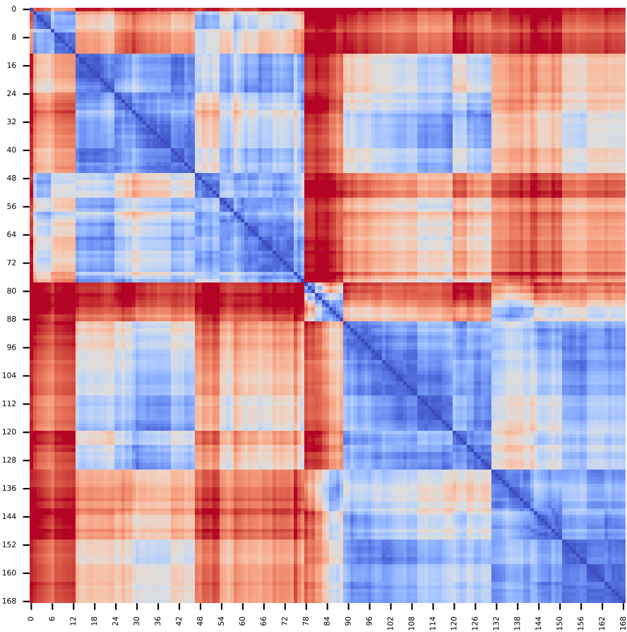
Perm 4
