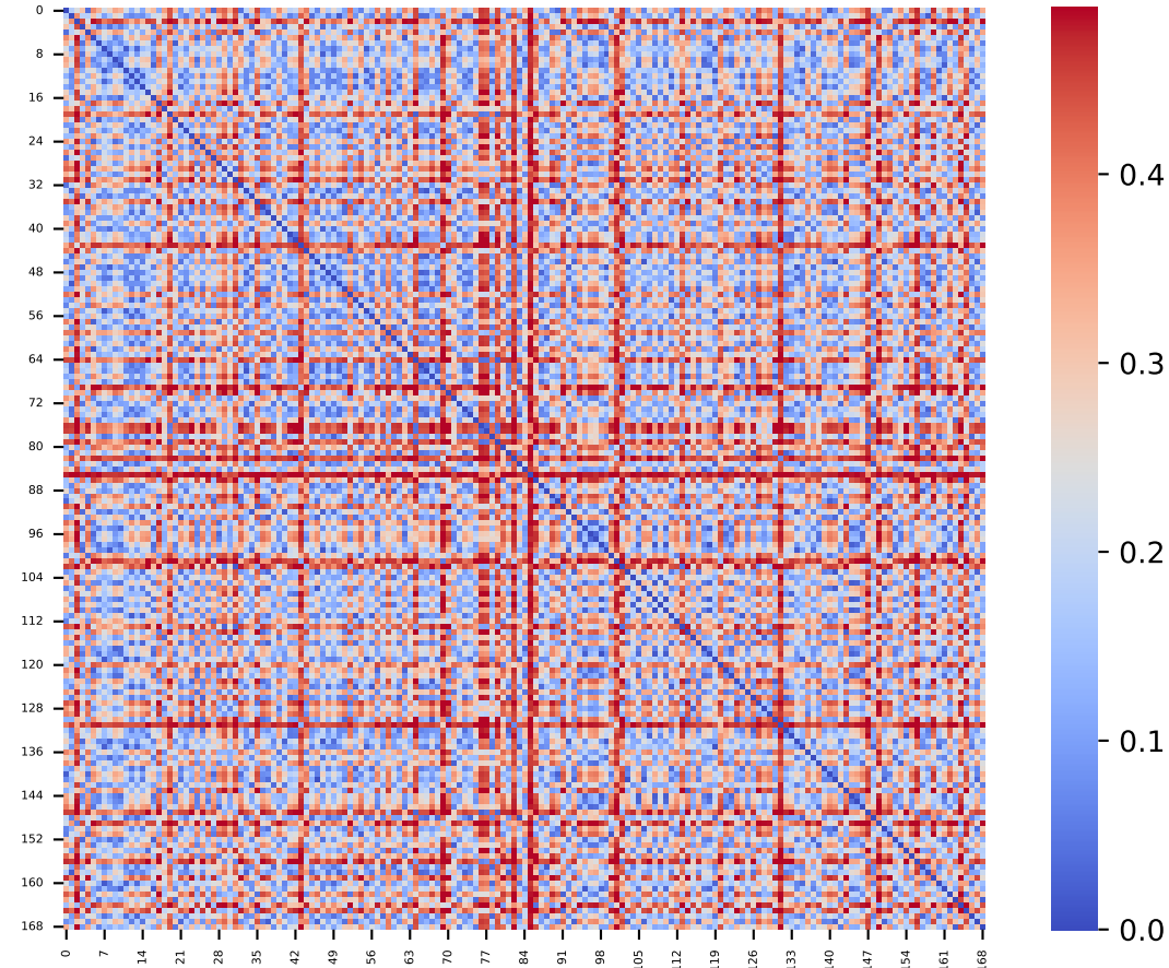
Perm 2 (seed=22)
