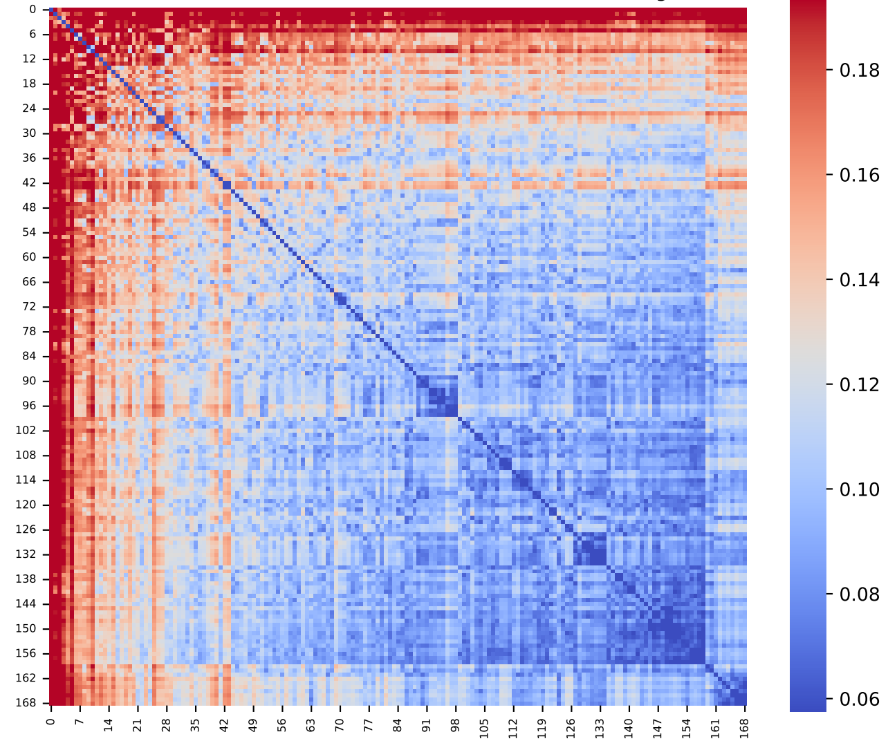
(b) Quantum Distance Matrix (Quantum HRP Ordering)
