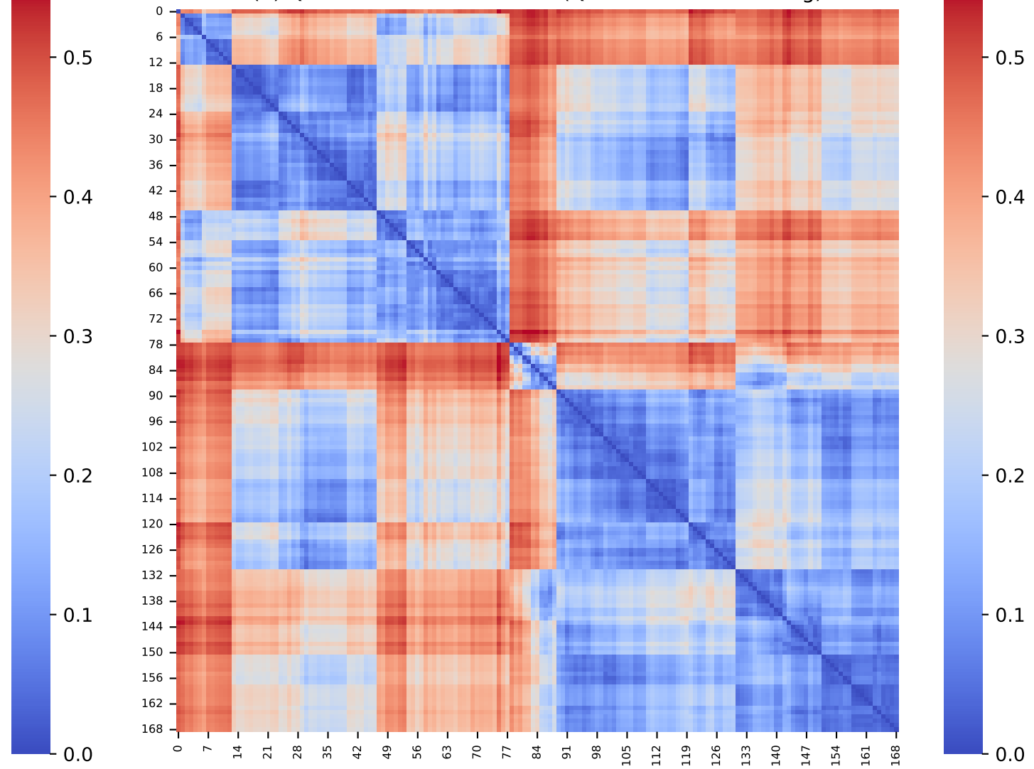
(b) Quantum Distance Matrix (Quantum HRP Ordering)
