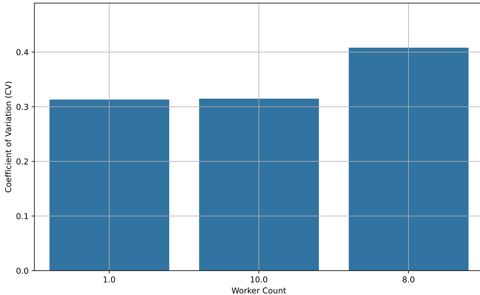
Bandwidth Consistency (Coefficient of Variation) Node: 222.214.219.199:7777
