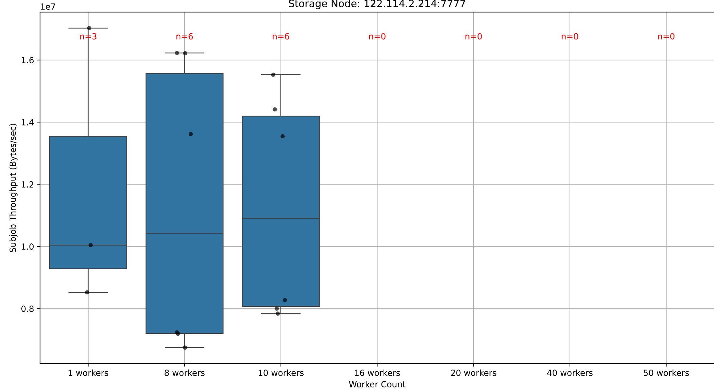
Bandwidth Distribution by Worker Count Storage Node: 122.114.2.214:7777
