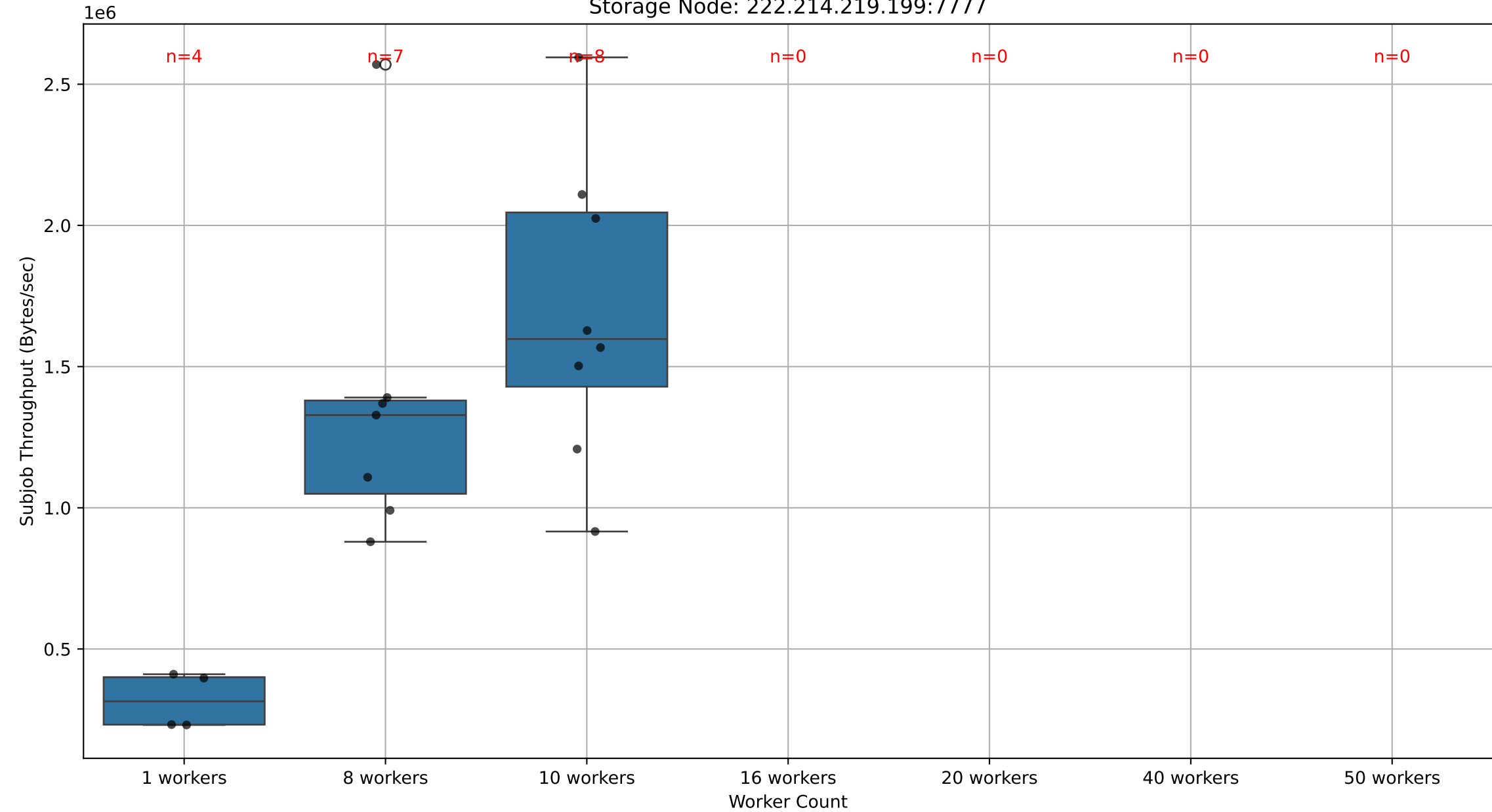
Bandwidth Distribution by Worker Count Storage Node: 222.214.219.199:7777
