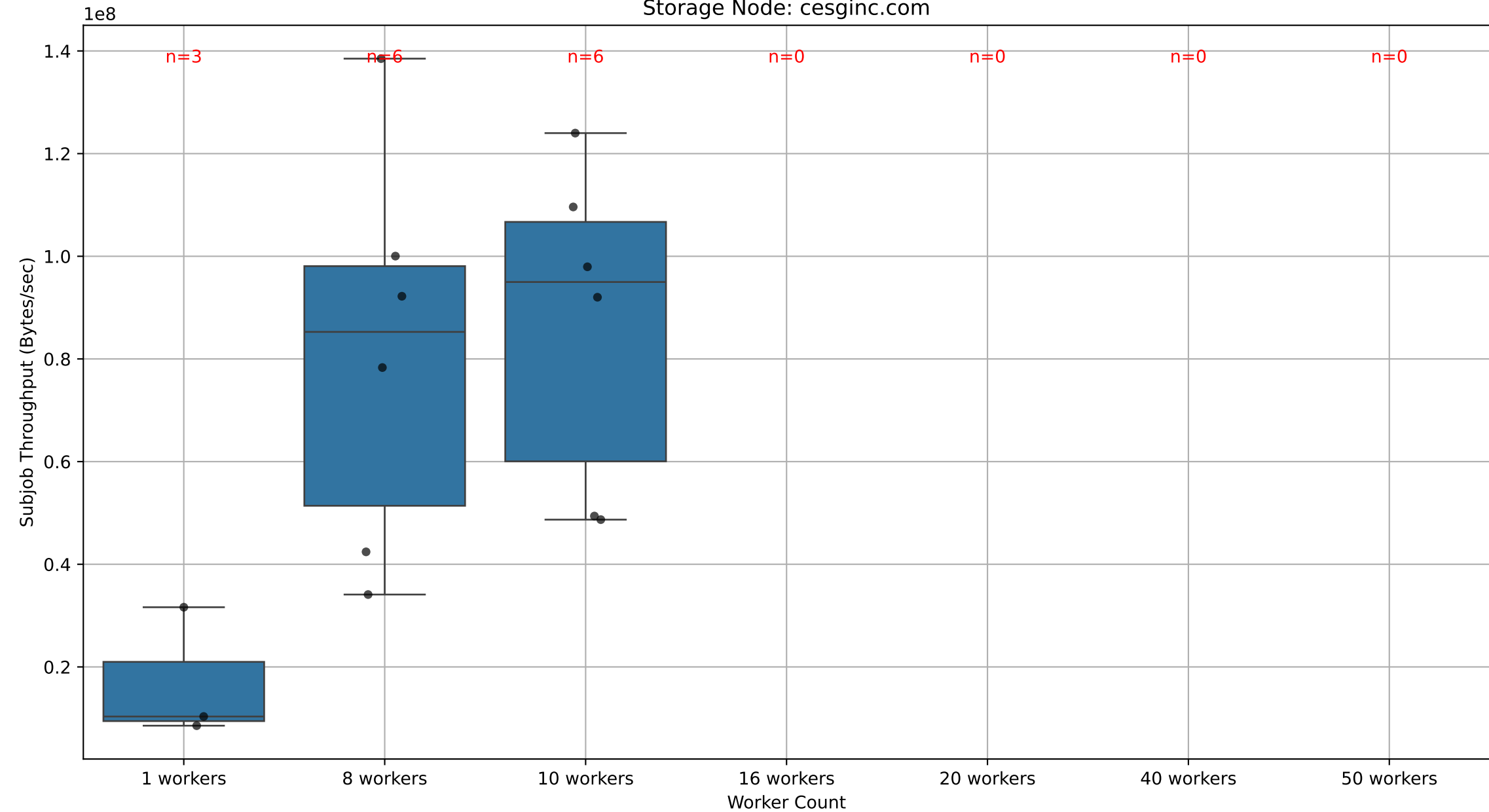
Bandwidth Distribution by Worker Count Storage Node: cesginc.com
