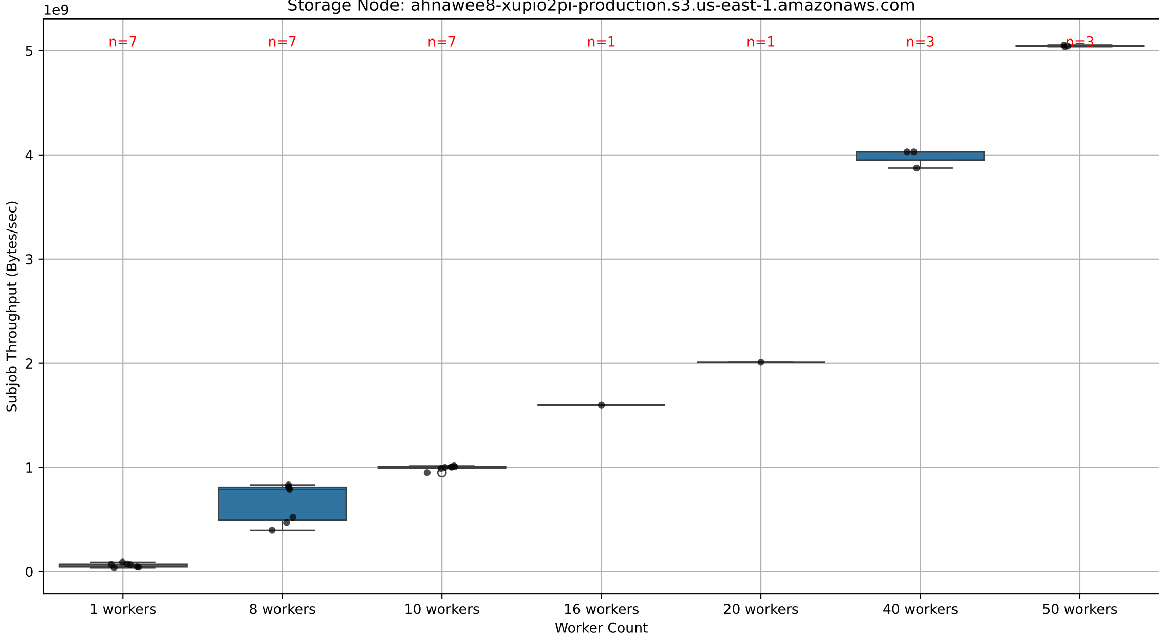
Bandwidth Distribution by Worker Count Storage Node: ahnawee8-xupio2pi-production.s3.us-east-1.amazonaws.com
