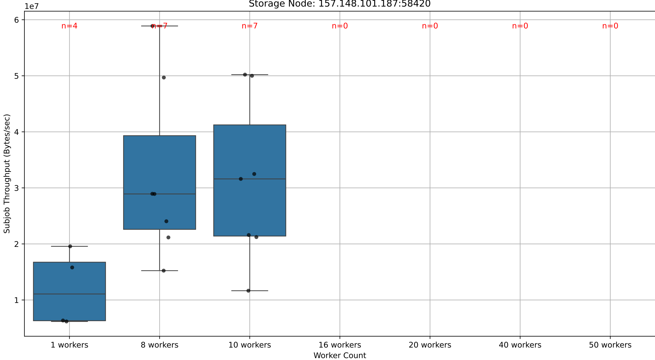
Bandwidth Distribution by Worker Count Storage Node: 157.148.101.187:58420
