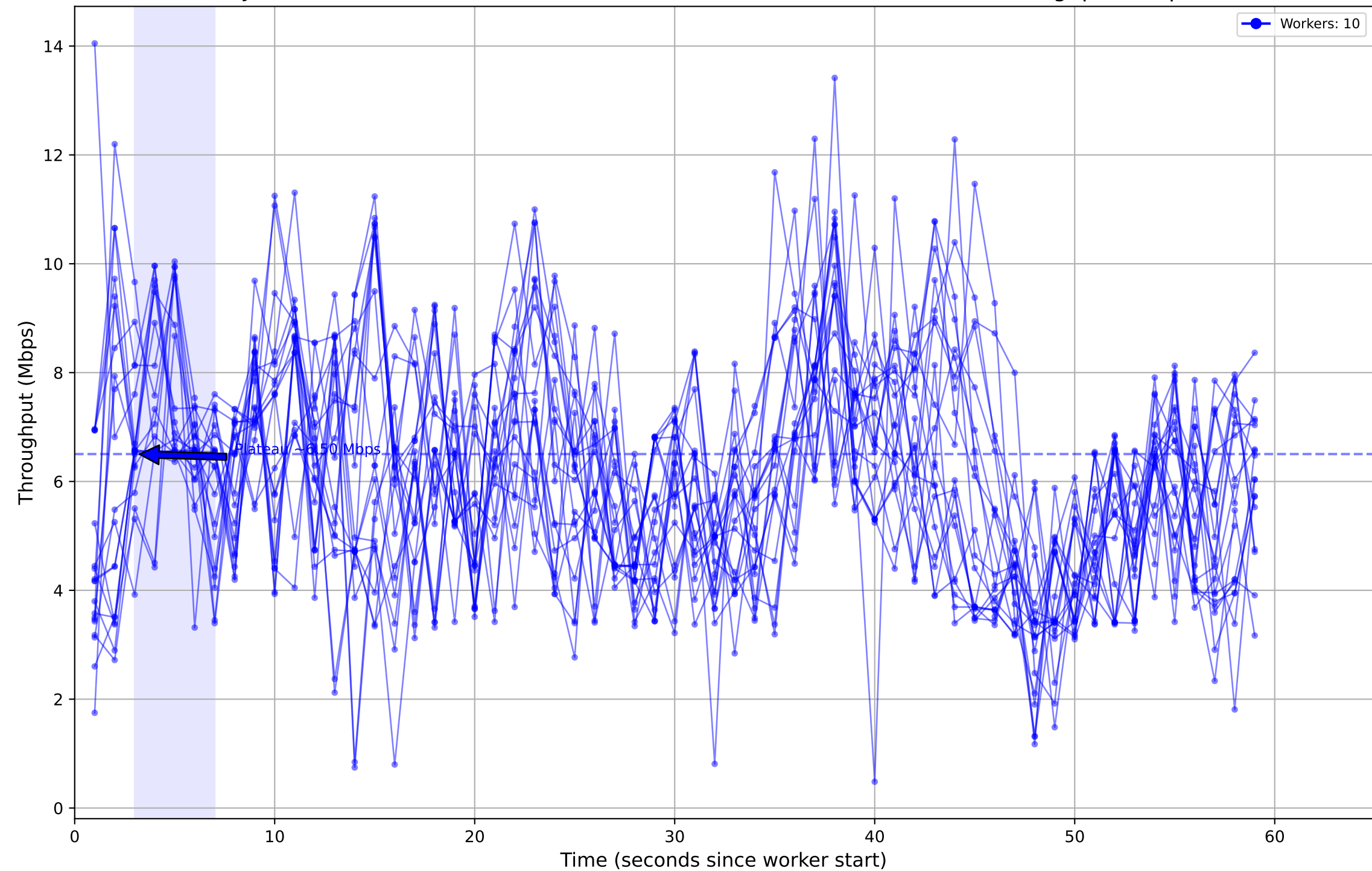
Job ID: c2ff83c6-263f-4bbf-a8f3-af5164ad62af - Individual Worker Throughput (Mbps)
