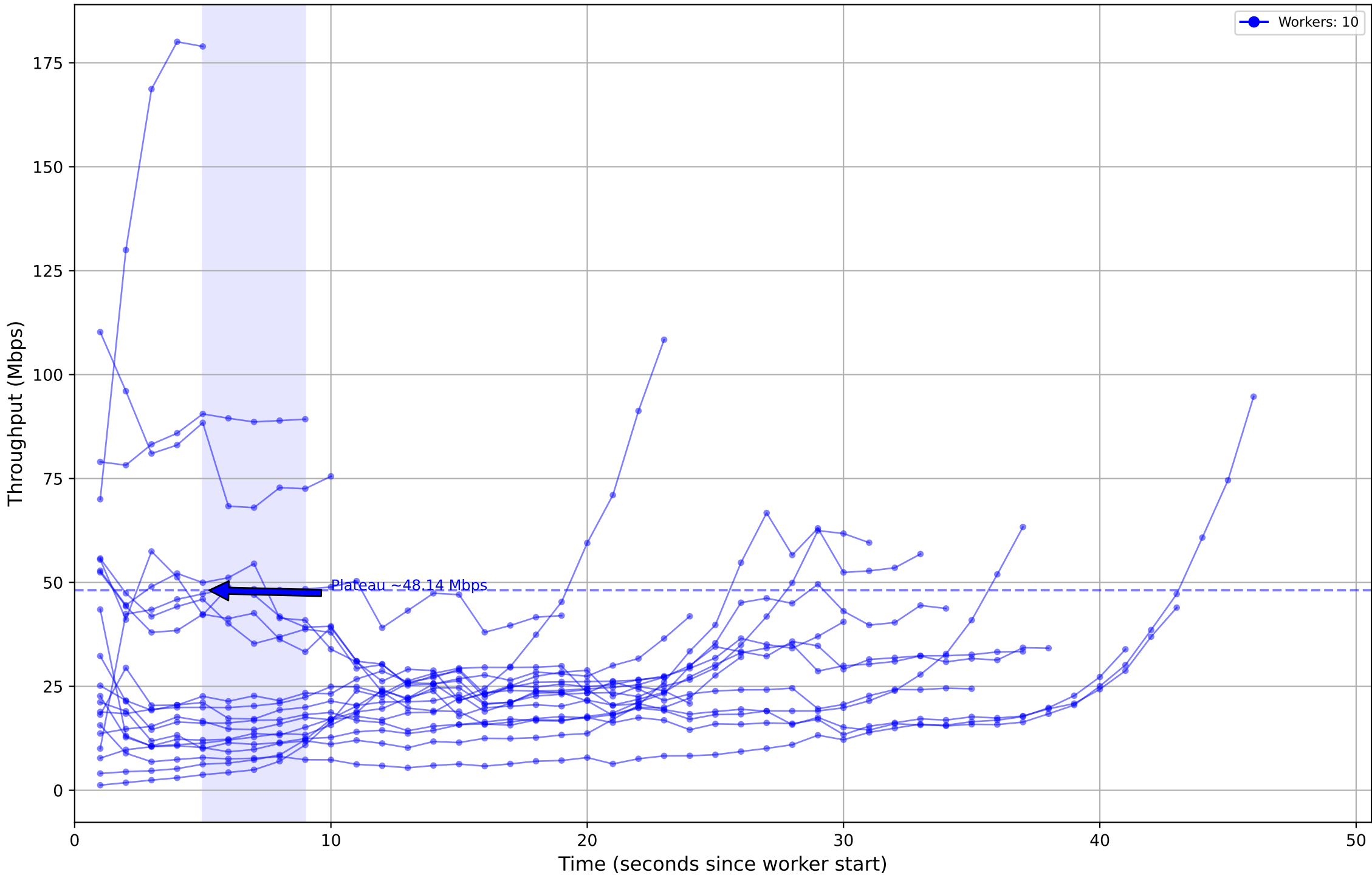
Job ID: 4c5bda2e-cf5b-4beb-8735-a712d13badaa - Individual Worker Throughput (Mbps)
