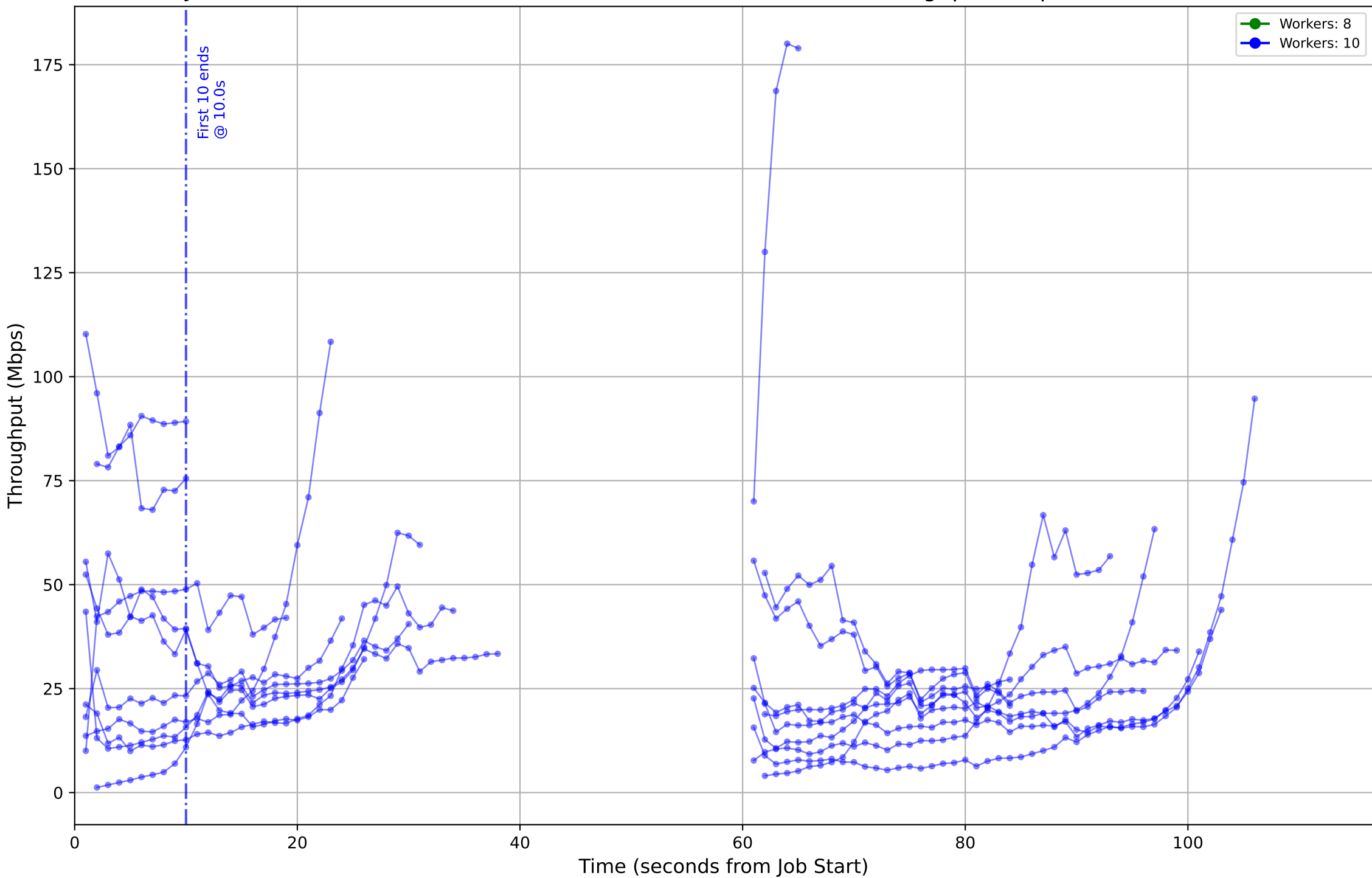
Job ID: 4c5bda2e-cf5b-4beb-8735-a712d13badaa - Worker Throughput (Mbps) (Absolute Time)
