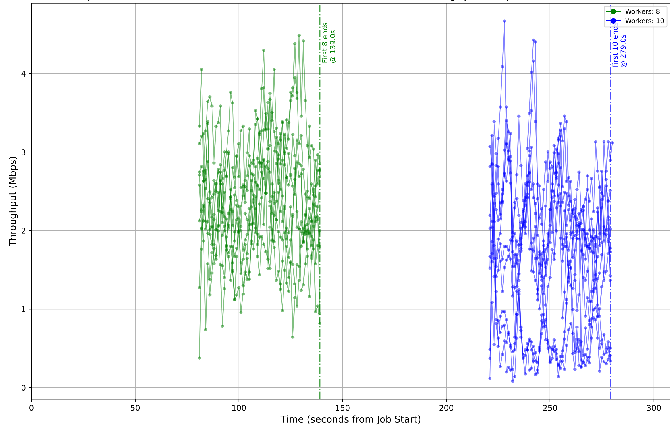
Job ID: 5ab38e34-c1a6-478e-ae9b-b502608205e5 - Worker Throughput (Mbps) (Absolute Time)
