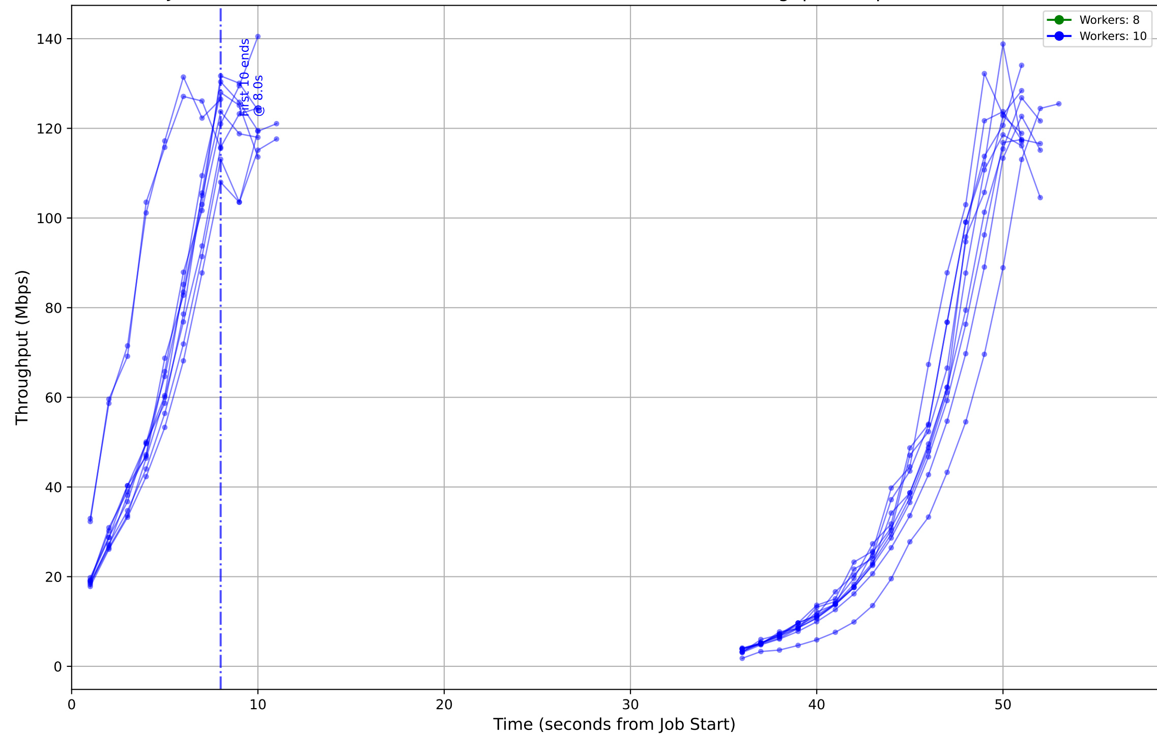
Job ID: 64ef3cc4-215c-43cb-b89a-b87dfd78a047 - Worker Throughput (Mbps) (Absolute Time)
