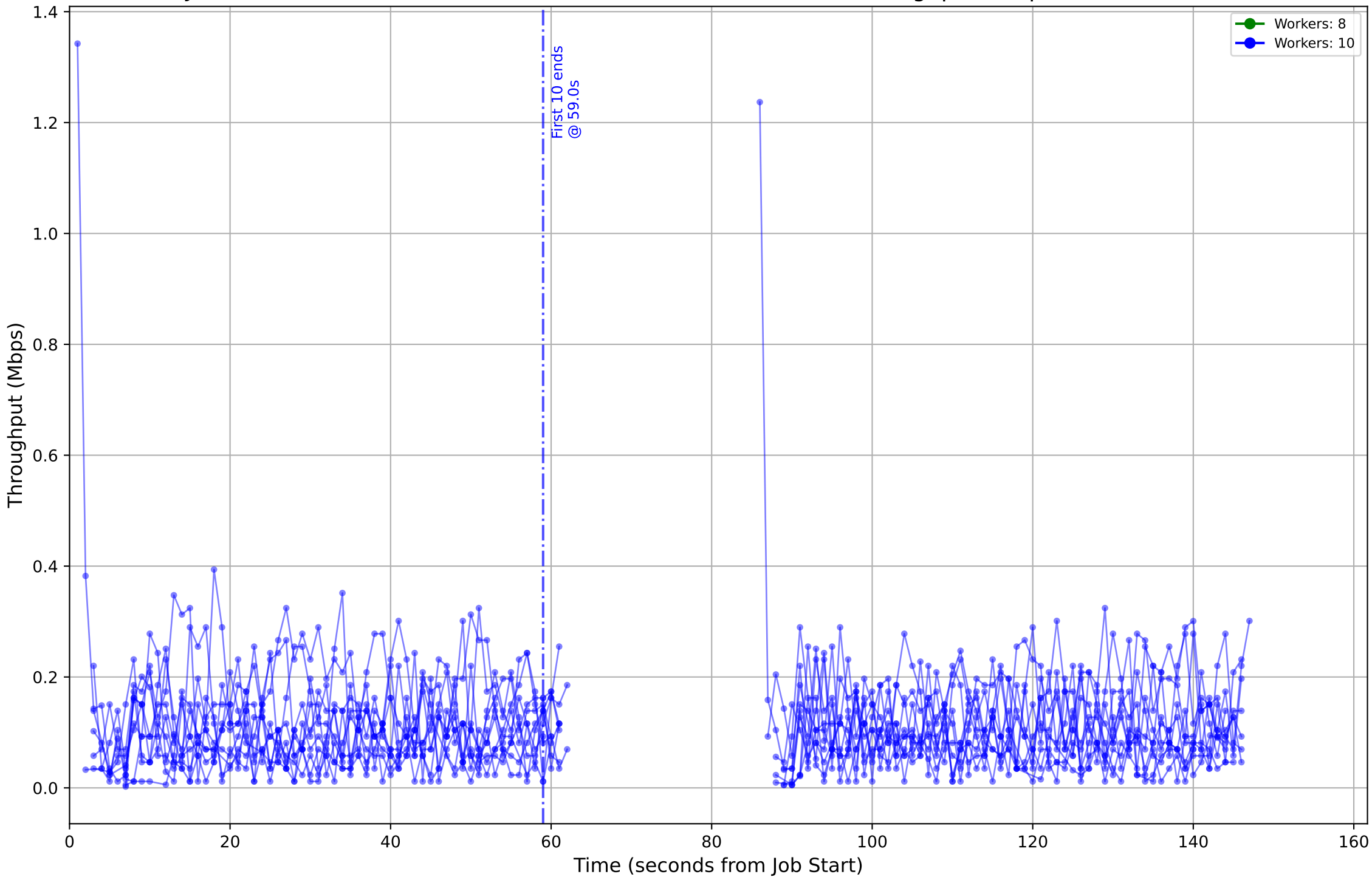
Job ID: 0995ff58-e2f1-4758-856a-199a1130cc48 - Worker Throughput (Mbps) (Absolute Time)
