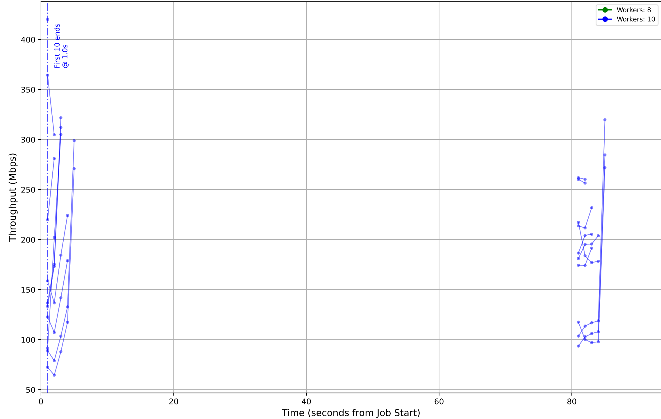
Job ID: 55b54989-740c-47a9-b33d-19afda9f8753 - Worker Throughput (Mbps) (Absolute Time)
