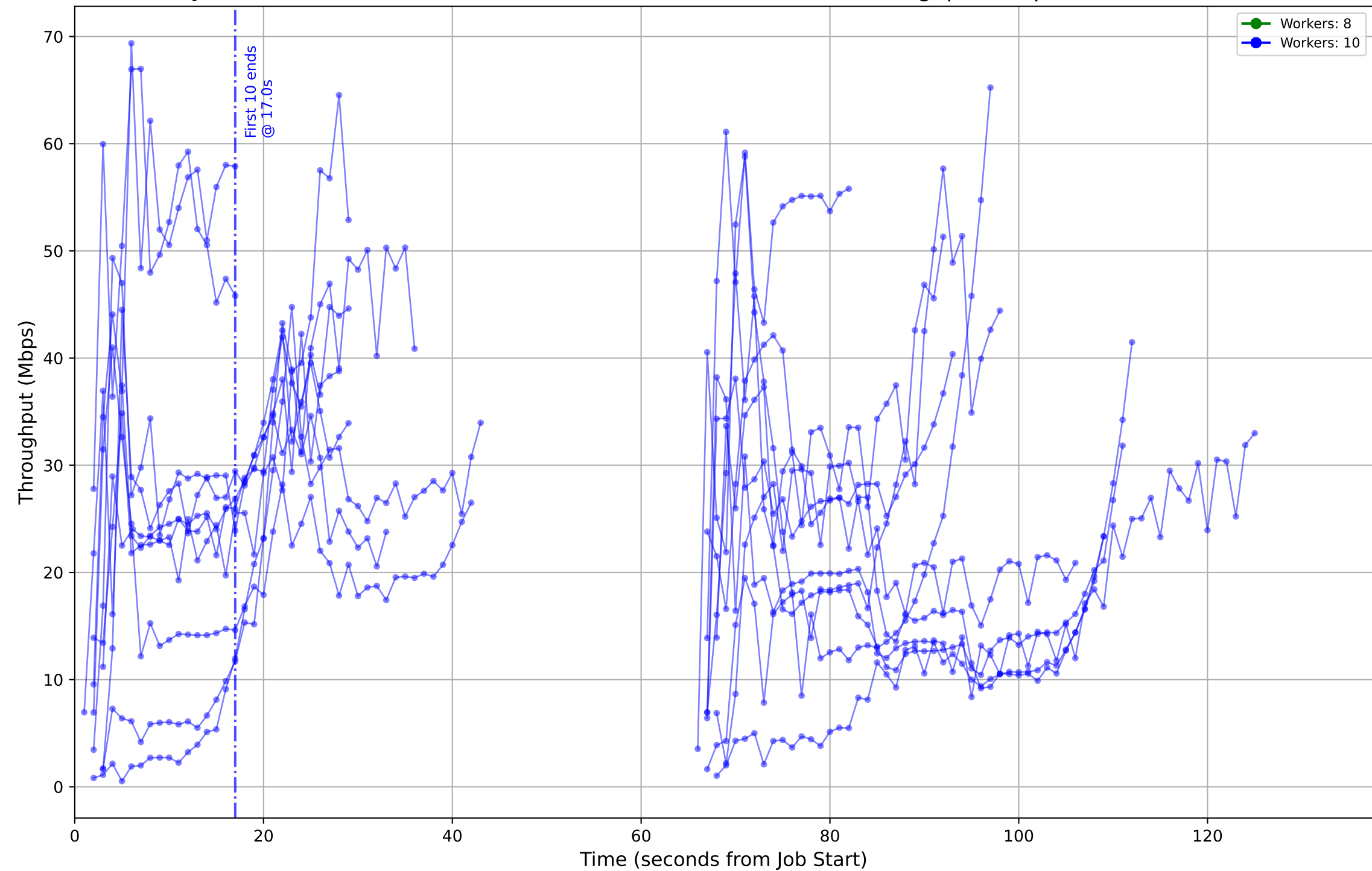
Job ID: 1f74596c-ef4b-4469-b225-391947f17174 - Worker Throughput (Mbps) (Absolute Time)
