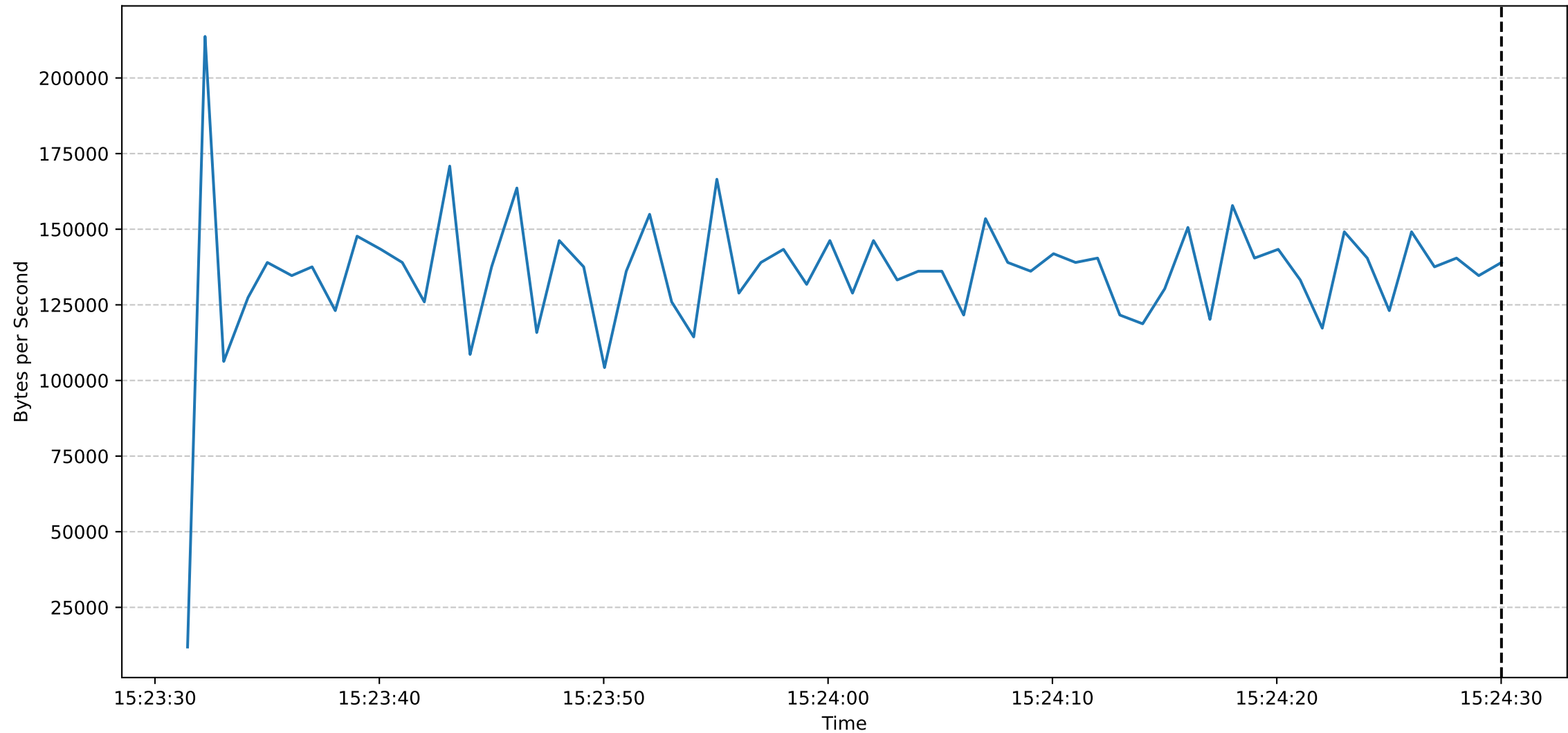
Sub Job ID: 4a80aa64-dde0-4323-b9e8-7222328b2cbf - Worker Download Speeds
