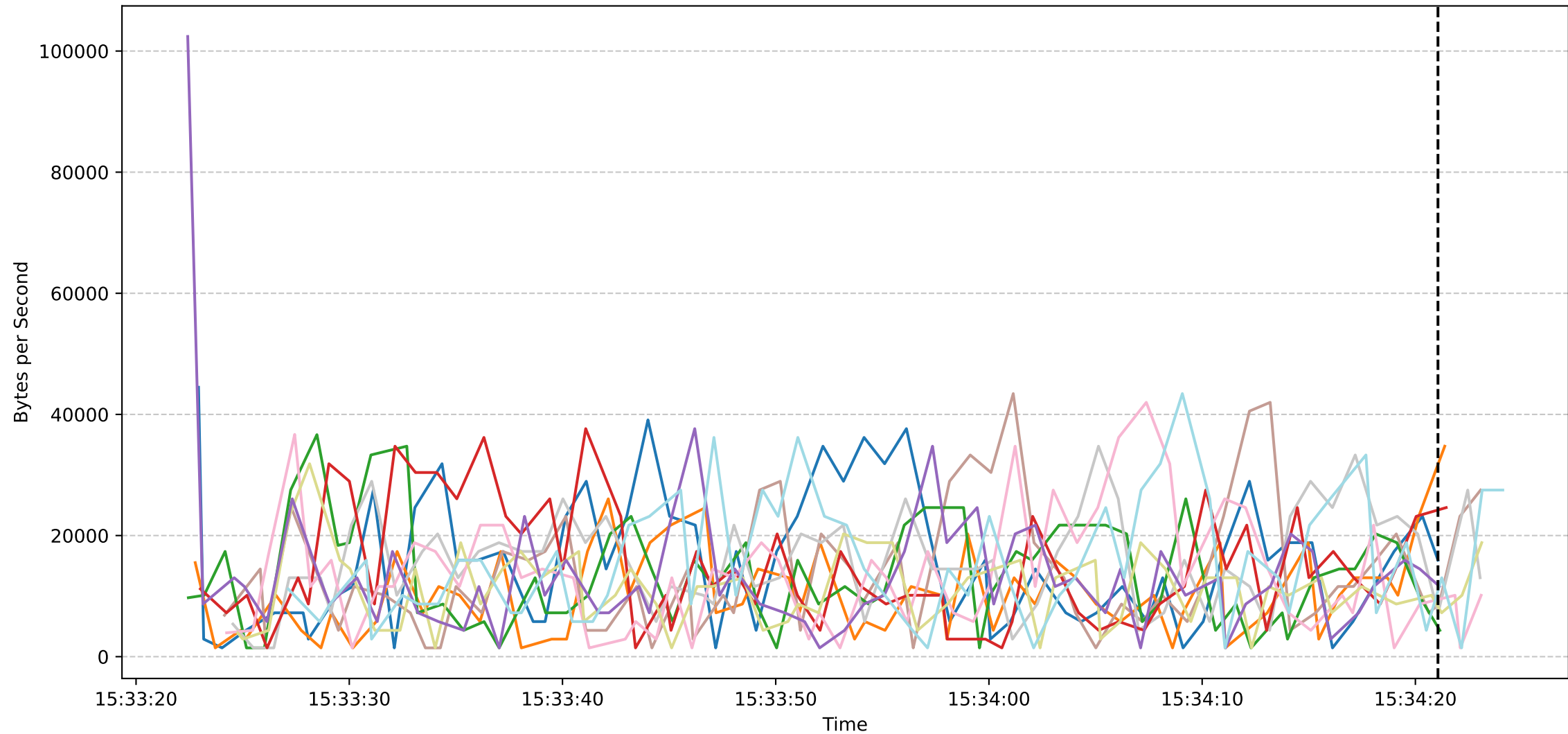
Sub Job ID: 0ef08a46-d69c-4963-8617-fa7f0a8d4b2a - Worker Download Speeds
