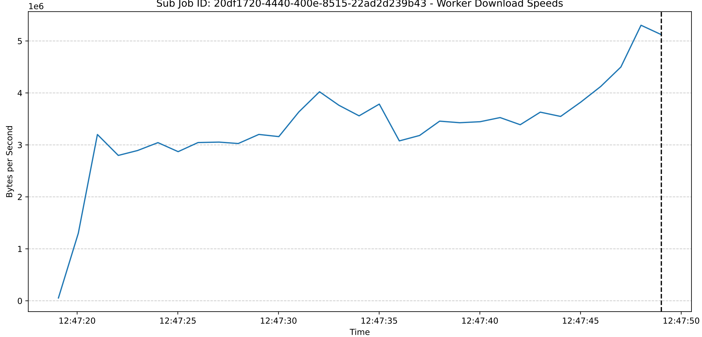
Sub Job ID: 20df1720-4440-400e-8515-22ad2d239b43 - Worker Download Speeds
