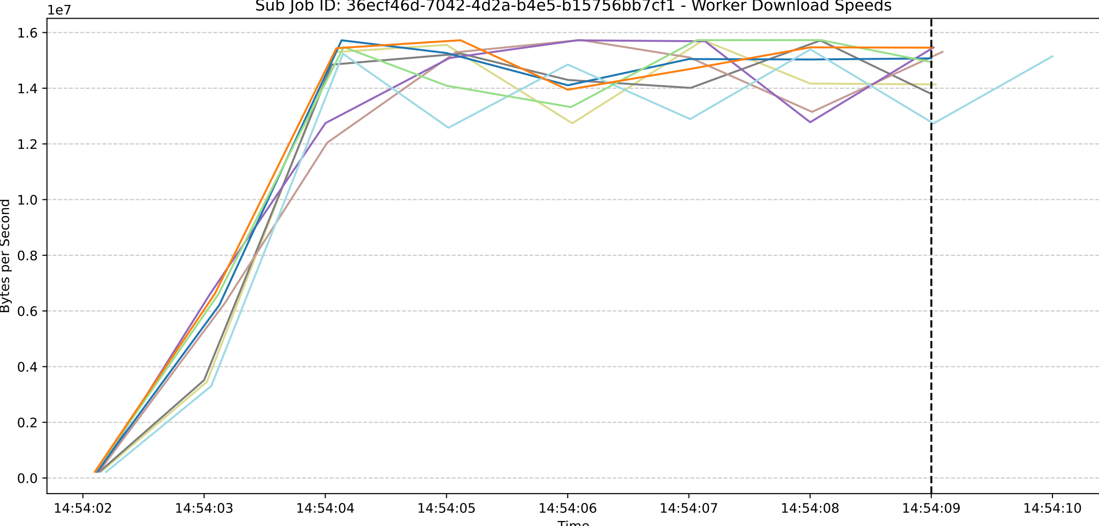
Sub Job ID: 36ecf46d-7042-4d2a-b4e5-b15756bb7cf1 - Worker Download Speeds
