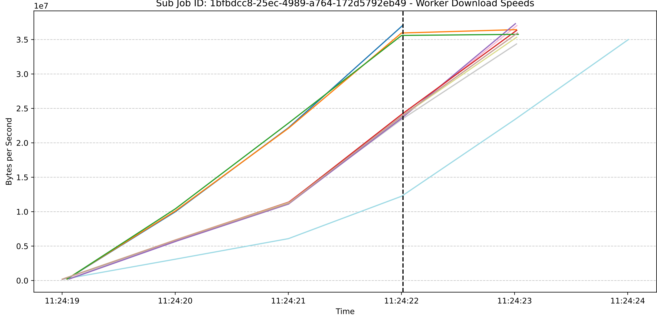
Sub Job ID: 1bfbdcc8-25ec-4989-a764-172d5792eb49 - Worker Download Speeds
