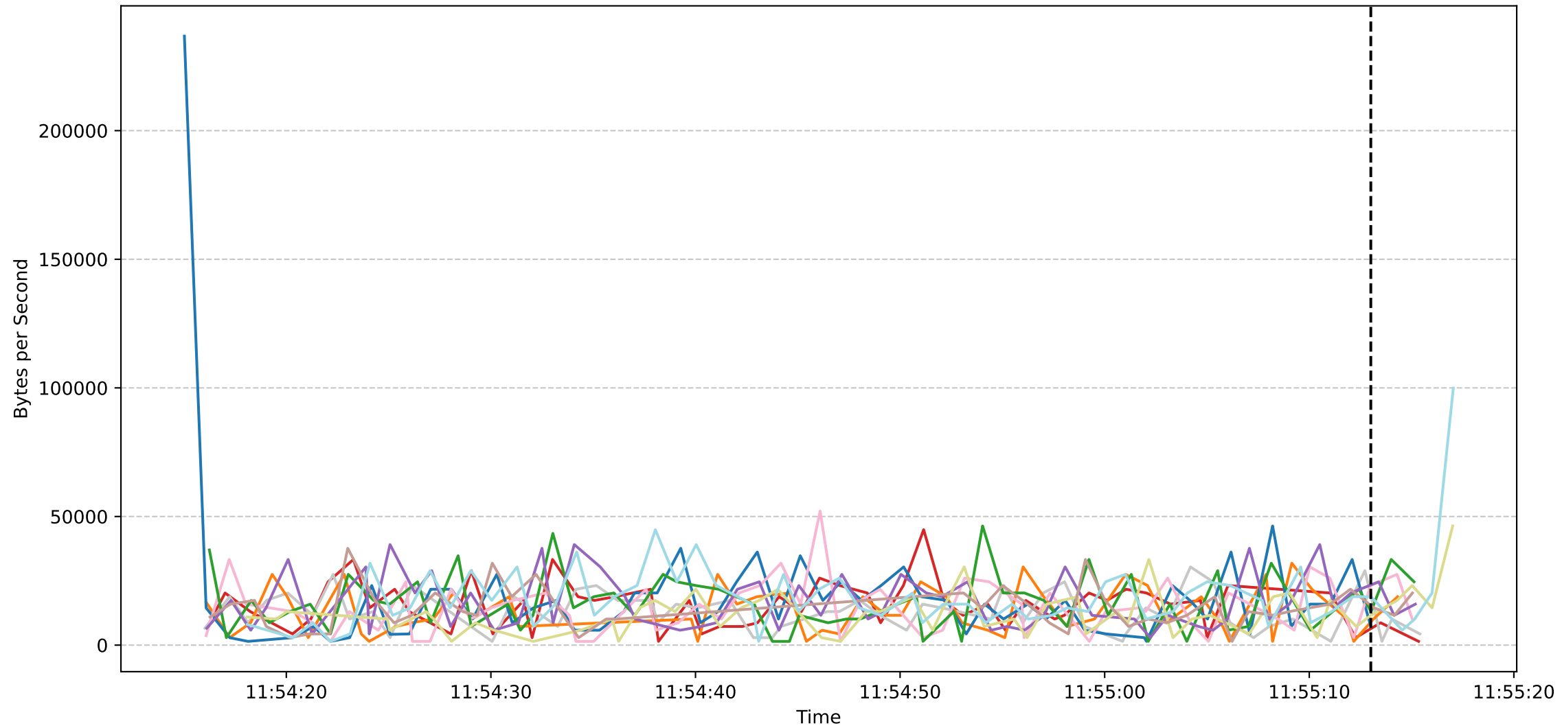
Sub Job ID: e8fe9bdf-6c63-4e7c-afa2-d69cd043ba7e - Worker Download Speeds
