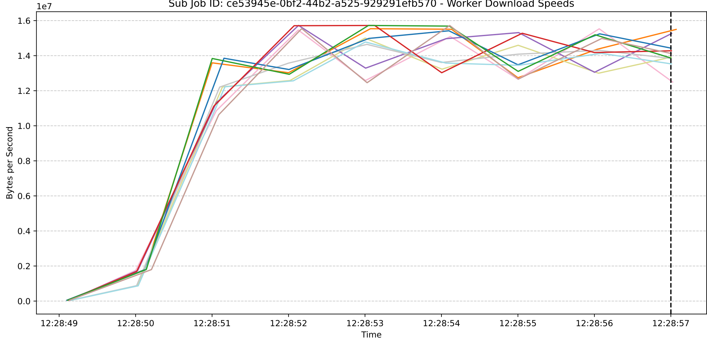
Sub Job ID: ce53945e-0bf2-44b2-a525-929291efb570 - Worker Download Speeds
