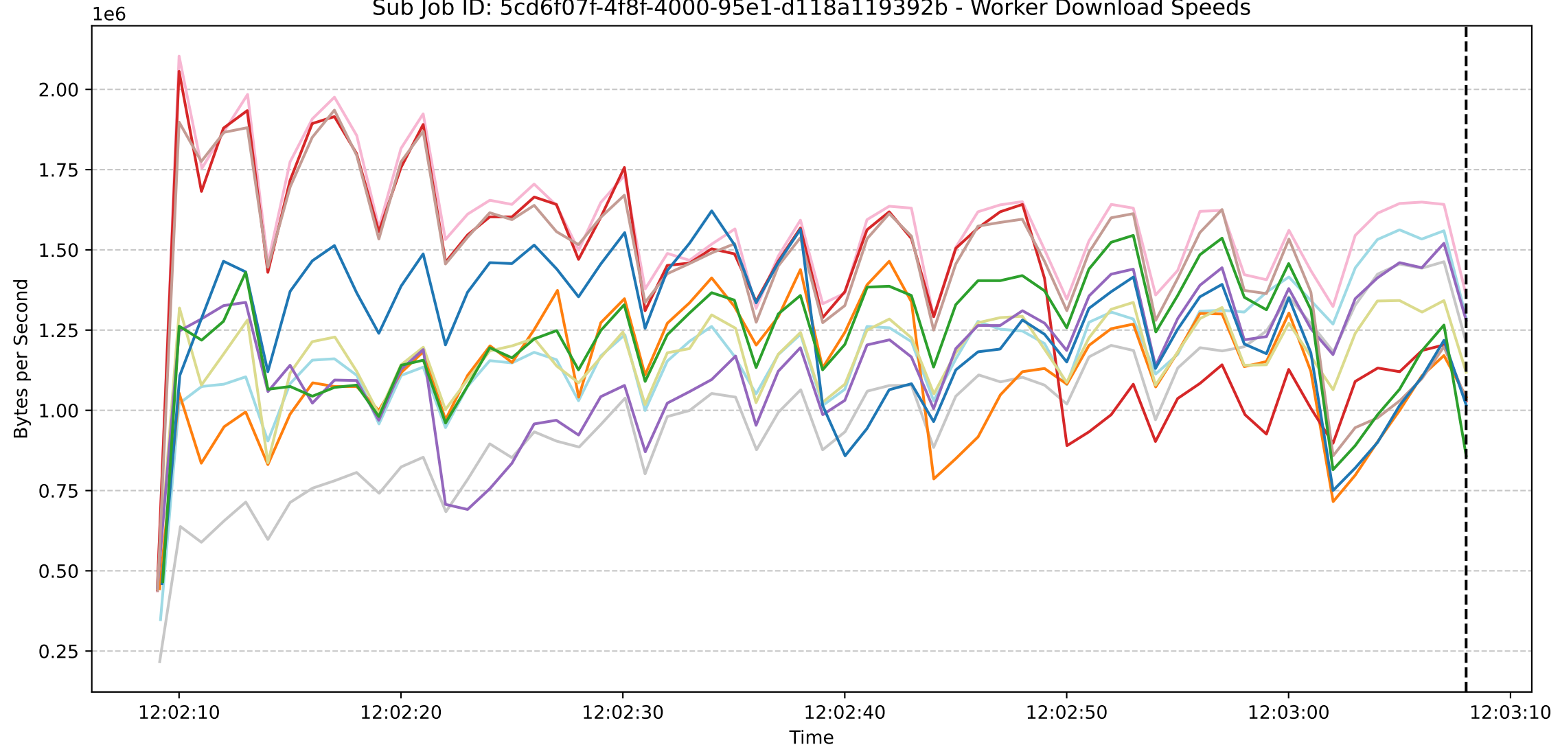
Sub Job ID: 5cd6f07f-4f8f-4000-95e1-d118a119392b - Worker Download Speeds
