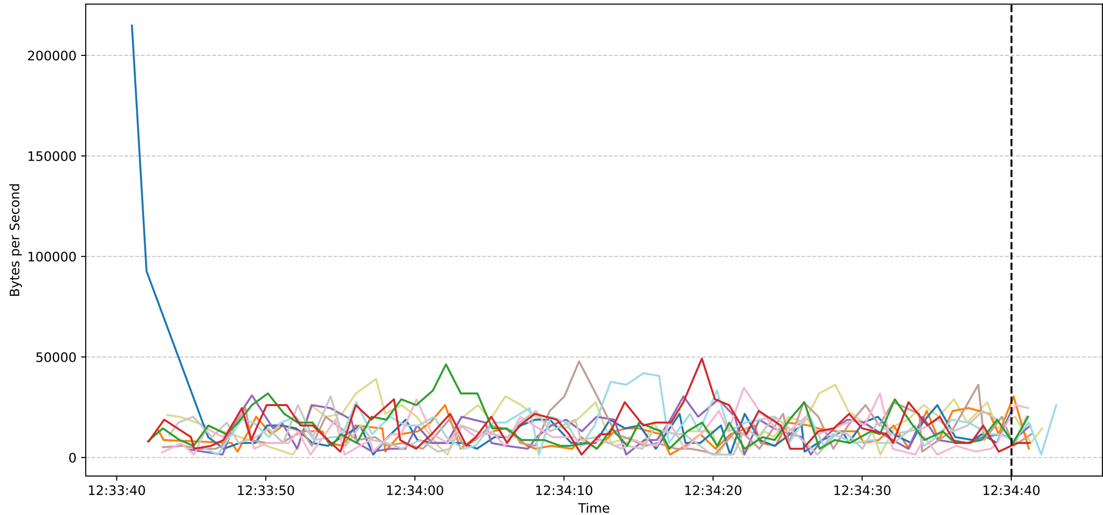
Sub Job ID: a14f7205-7557-412a-bdee-93ddf94c114d - Worker Download Speeds
