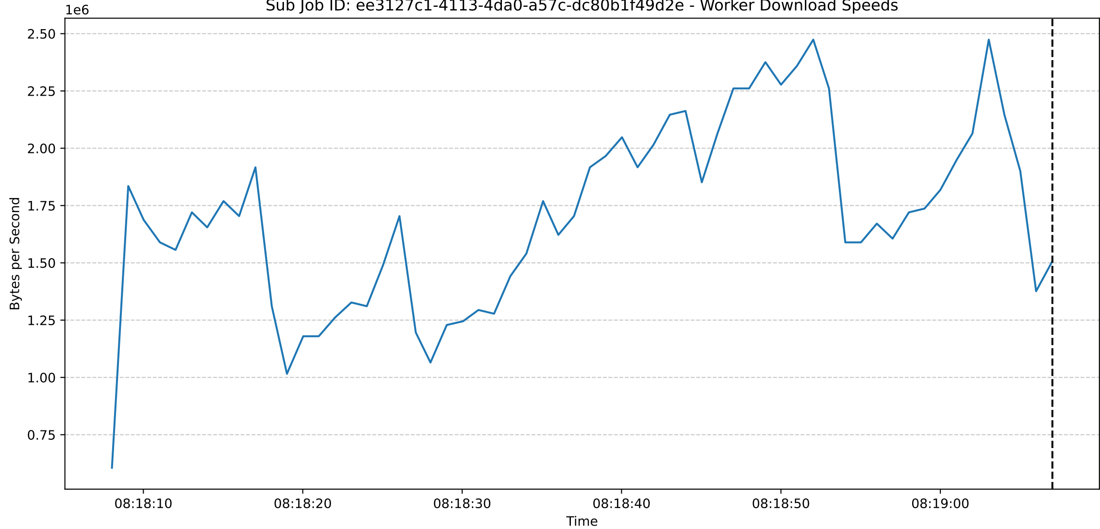
Sub Job ID: ee3127c1-4113-4da0-a57c-dc80b1f49d2e - Worker Download Speeds
