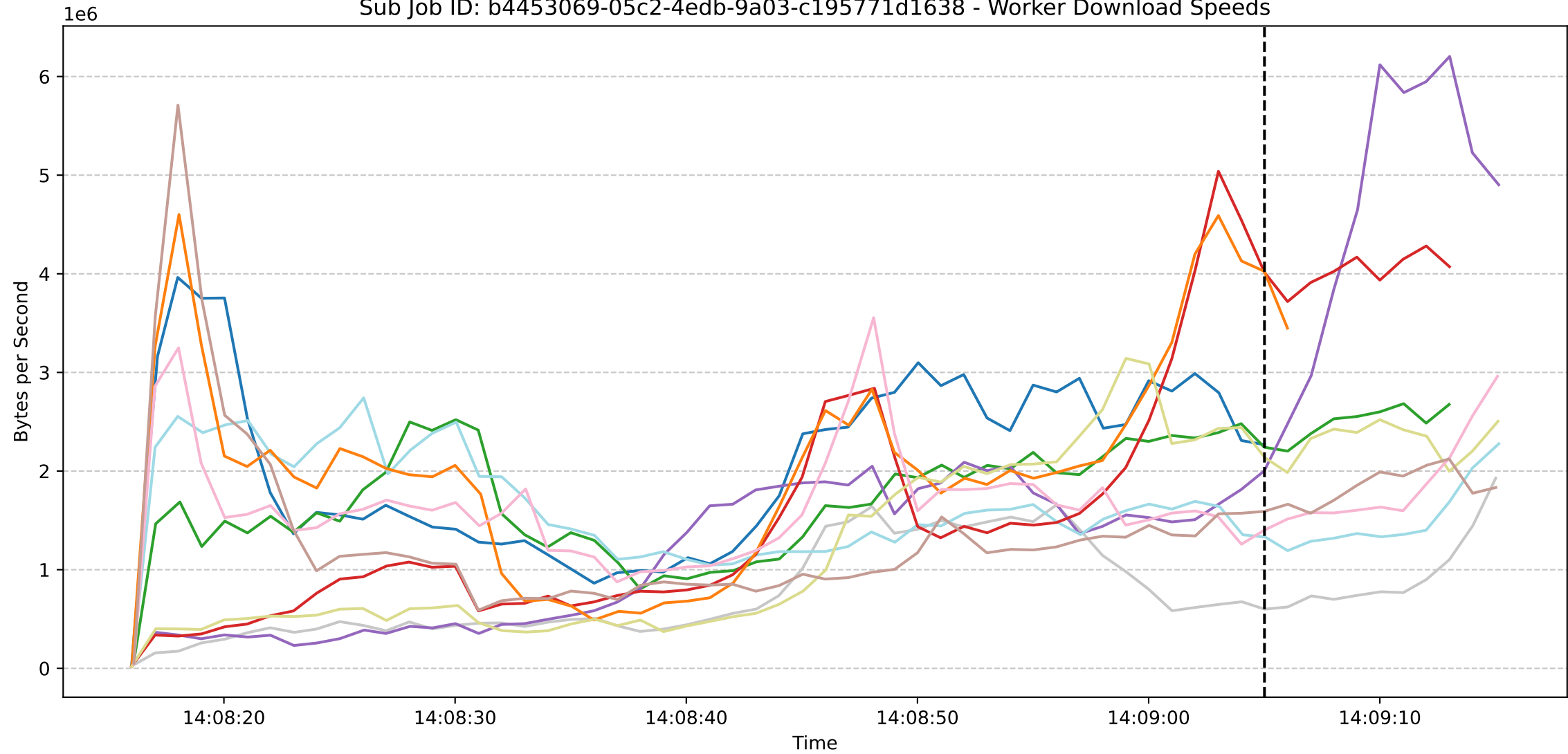
Sub Job ID: b4453069-05c2-4edb-9a03-c195771d1638 - Worker Download Speeds
