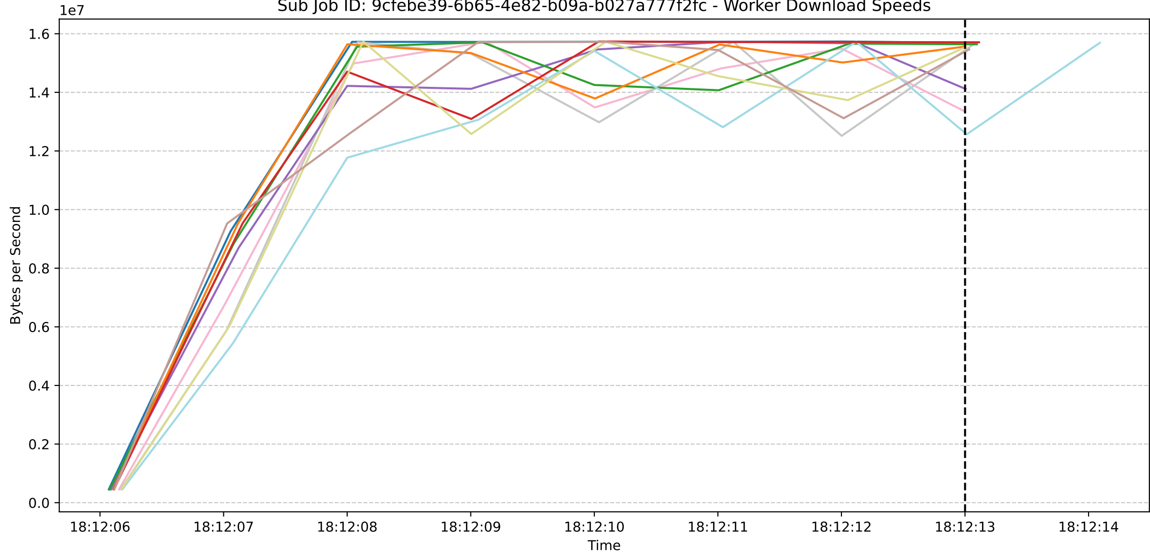
Sub Job ID: 9cfebe39-6b65-4e82-b09a-b027a777f2fc - Worker Download Speeds
