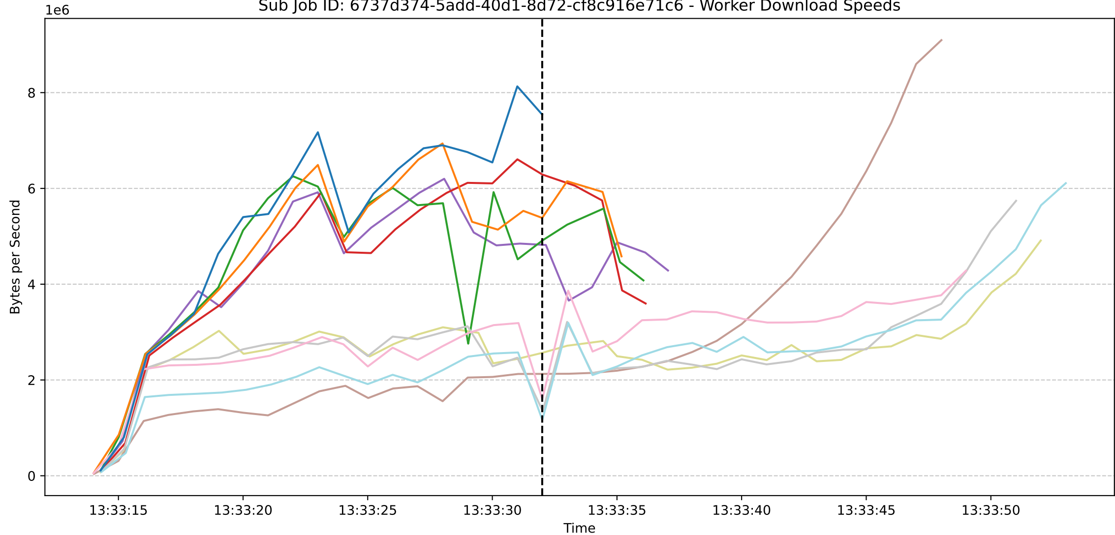
Sub Job ID: 6737d374-5add-40d1-8d72-cf8c916e71c6 - Worker Download Speeds
