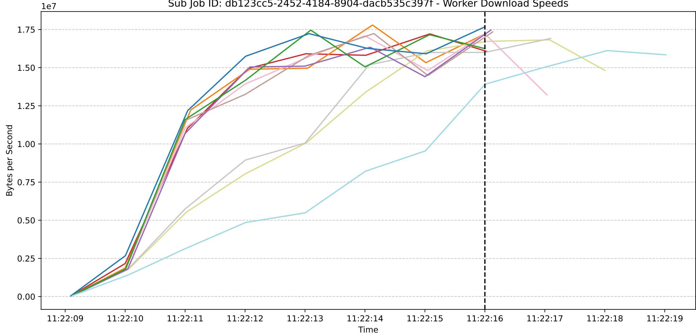
Sub Job ID: db123cc5-2452-4184-8904-dacb535c397f - Worker Download Speeds
