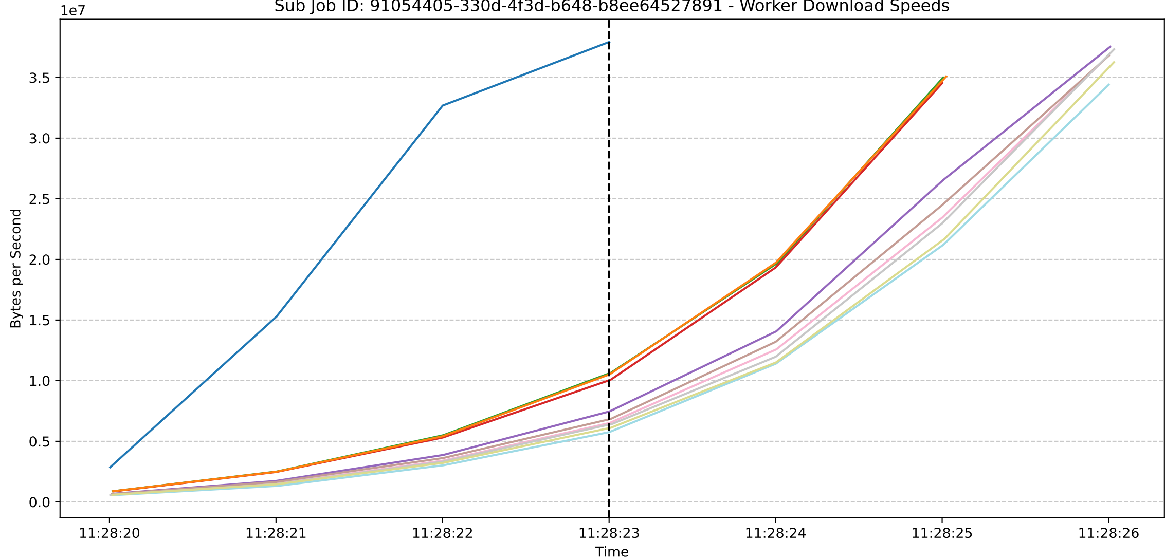
Sub Job ID: 91054405-330d-4f3d-b648-b8ee64527891 - Worker Download Speeds
