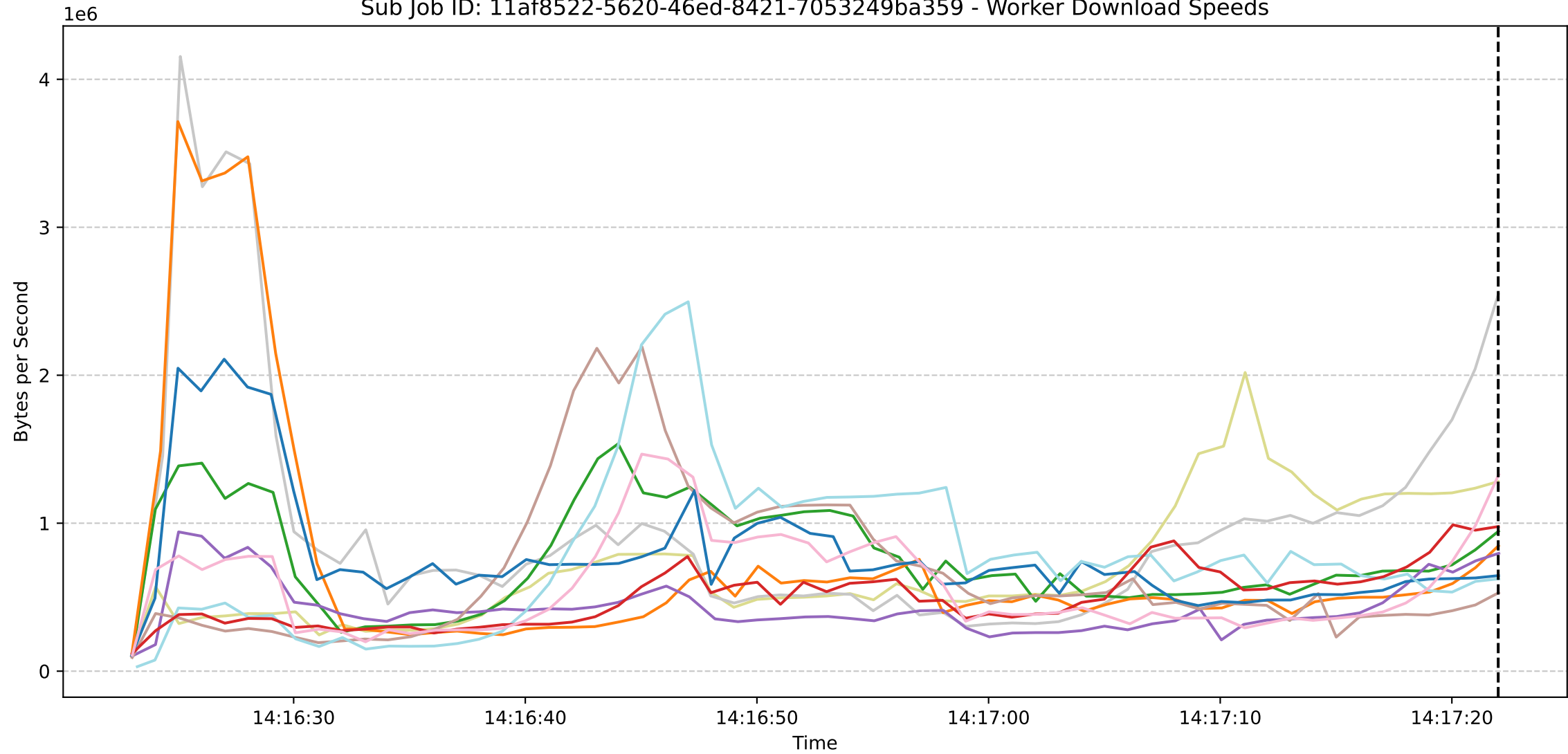
Sub Job ID: 11af8522-5620-46ed-8421-7053249ba359 - Worker Download Speeds
