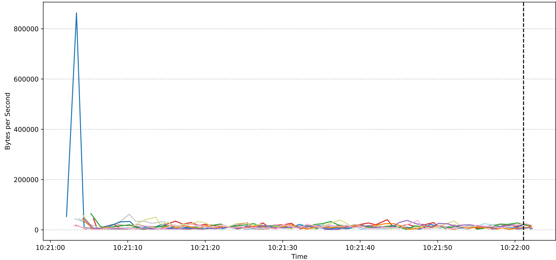
Sub Job ID: 227632d6-329d-4776-a810-a1d83d25f8df - Worker Download Speeds
