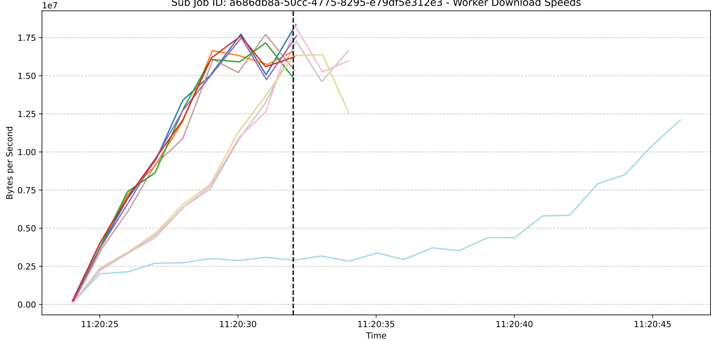
Sub Job ID: a686db8a-50cc-4775-8295-e79df5e312e3 - Worker Download Speeds
