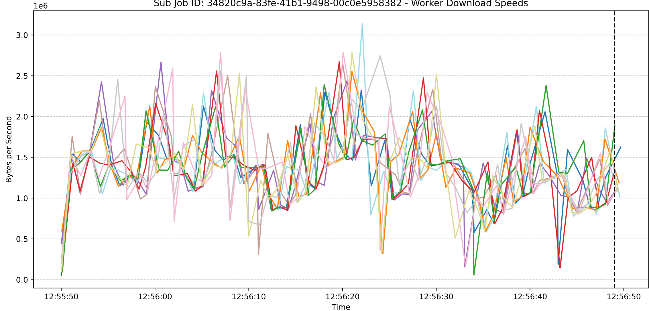
Sub Job ID: 34820c9a-83fe-41b1-9498-00c0e5958382 - Worker Download Speeds
