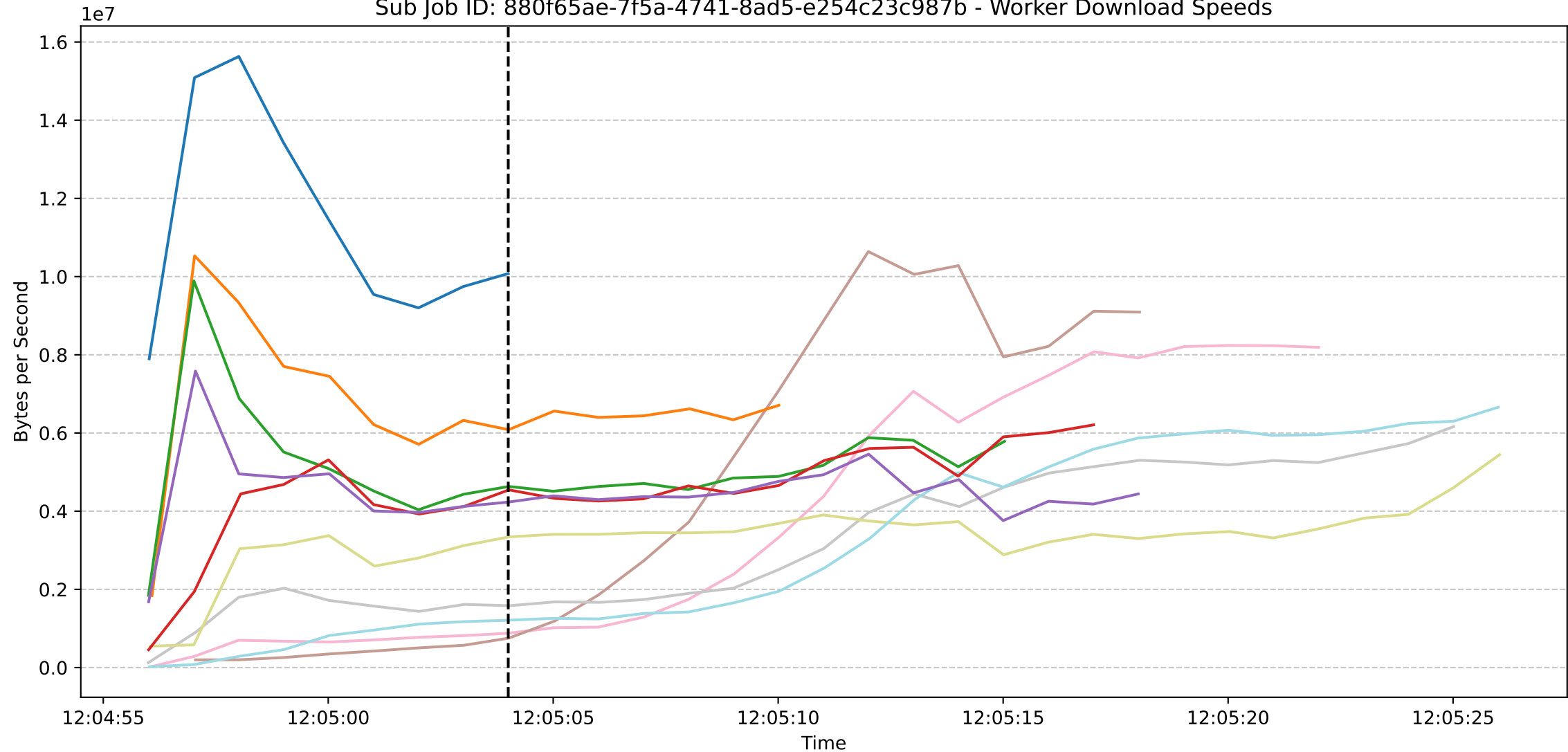
Sub Job ID: 880f65ae-7f5a-4741-8ad5-e254c23c987b - Worker Download Speeds
