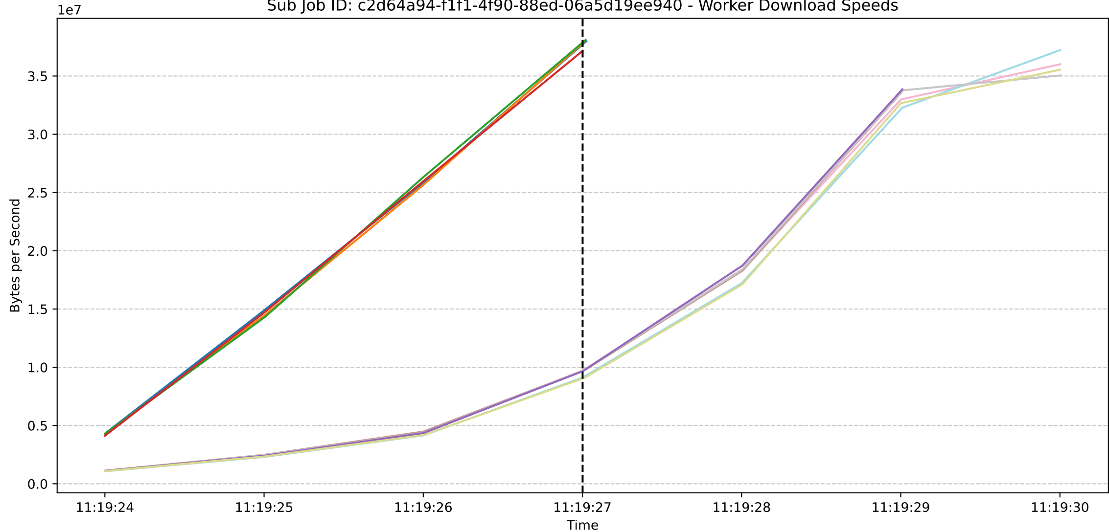
Sub Job ID: c2d64a94-f1f1-4f90-88ed-06a5d19ee940 - Worker Download Speeds
