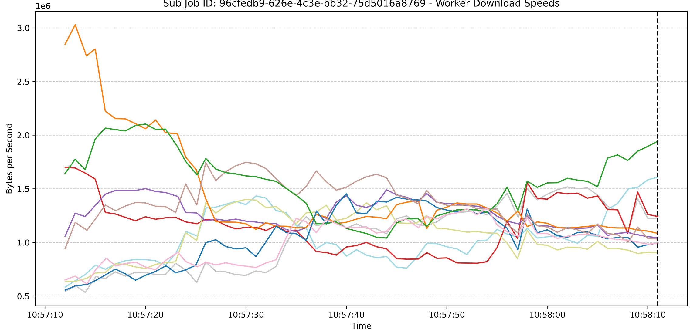
Sub Job ID: 96cfedb9-626e-4c3e-bb32-75d5016a8769 - Worker Download Speeds
