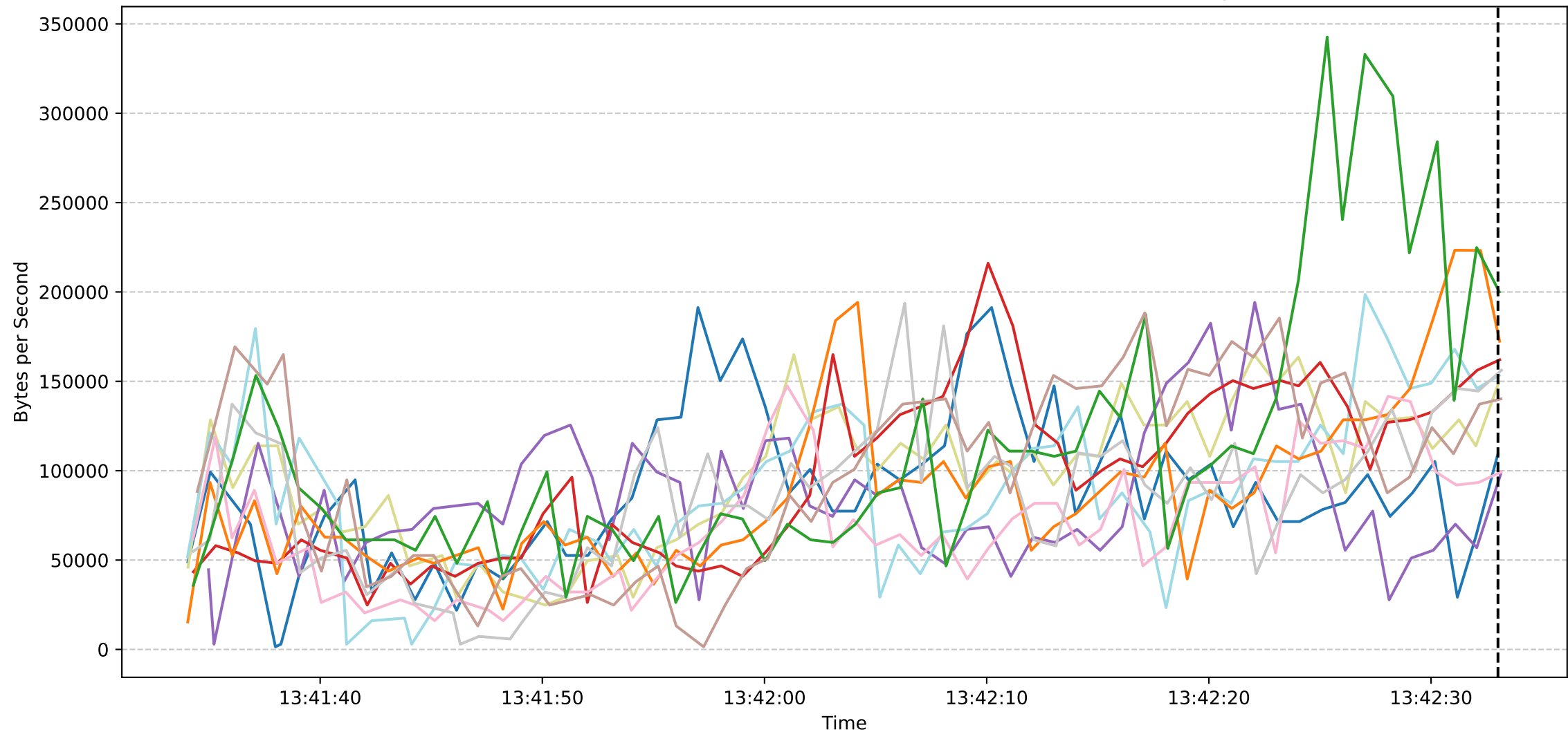
Sub Job ID: c594674c-4fc8-47f0-aa9d-ded657afc987 - Worker Download Speeds
