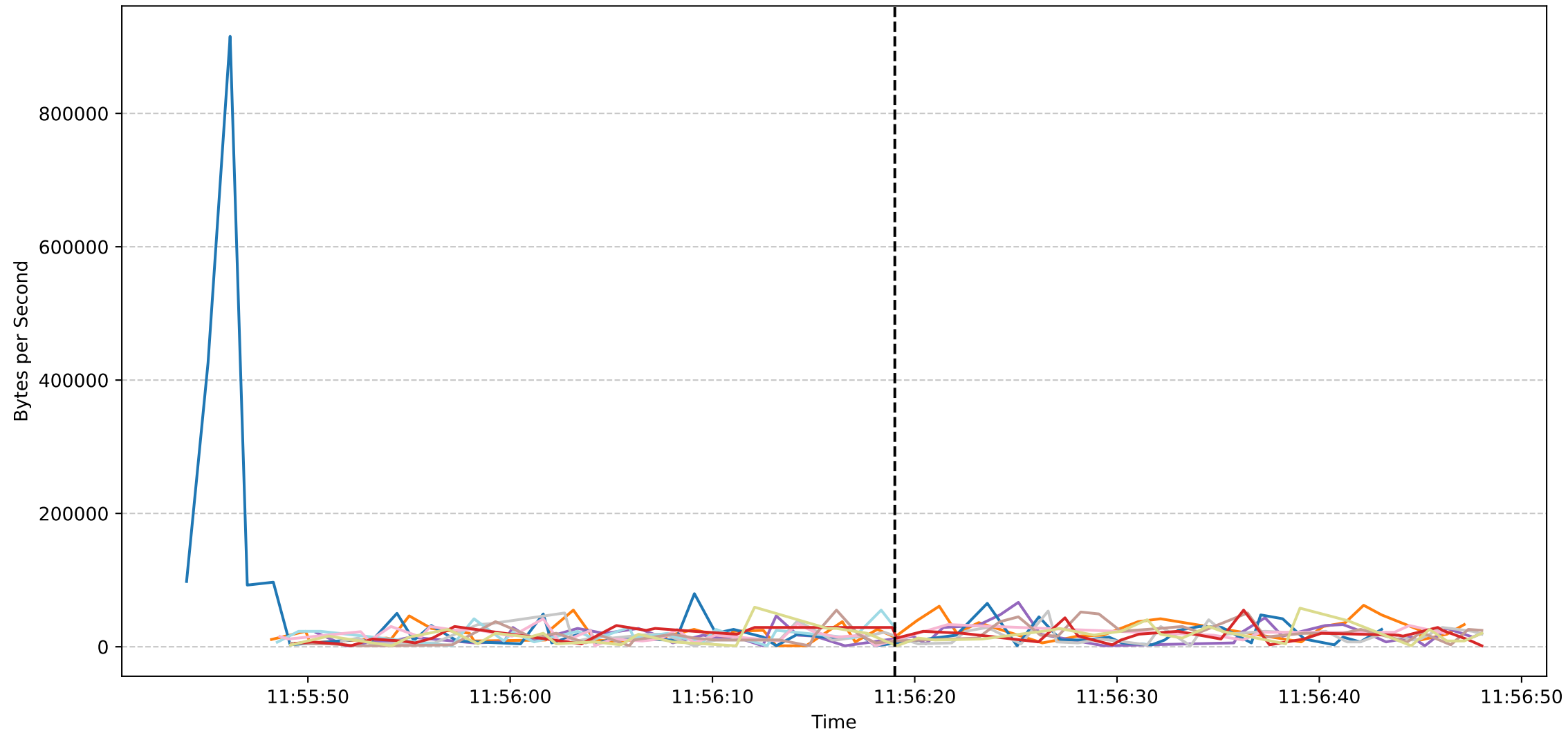
Sub Job ID: c6c6149a-decf-41f2-a962-2027d9f62b02 - Worker Download Speeds
