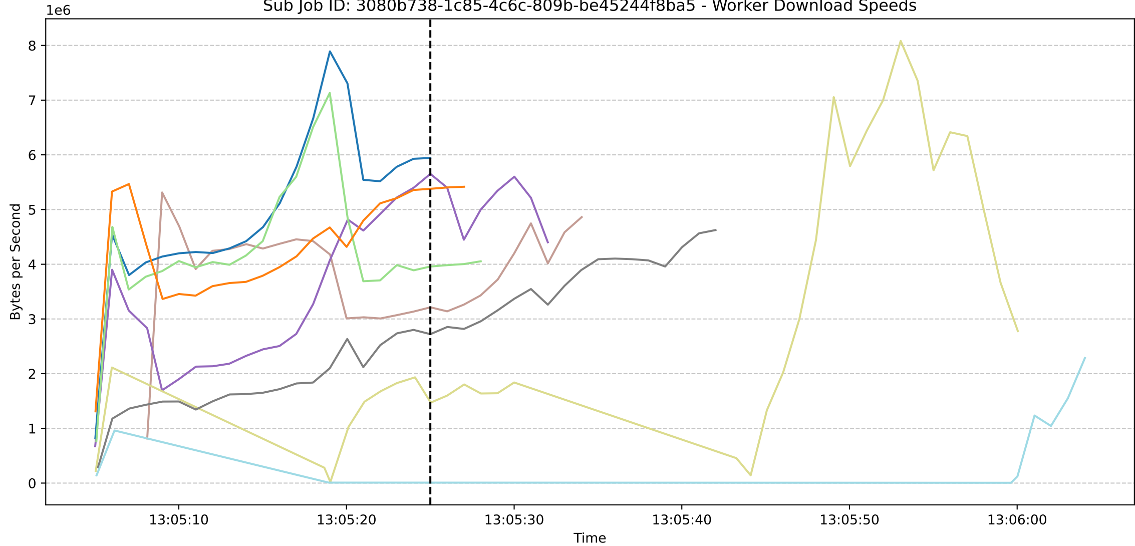
Sub Job ID: 3080b738-1c85-4c6c-809b-be45244f8ba5 - Worker Download Speeds
