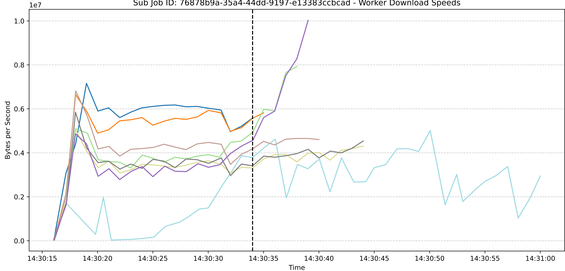
Sub Job ID: 76878b9a-35a4-44dd-9197-e13383ccbcad - Worker Download Speeds
