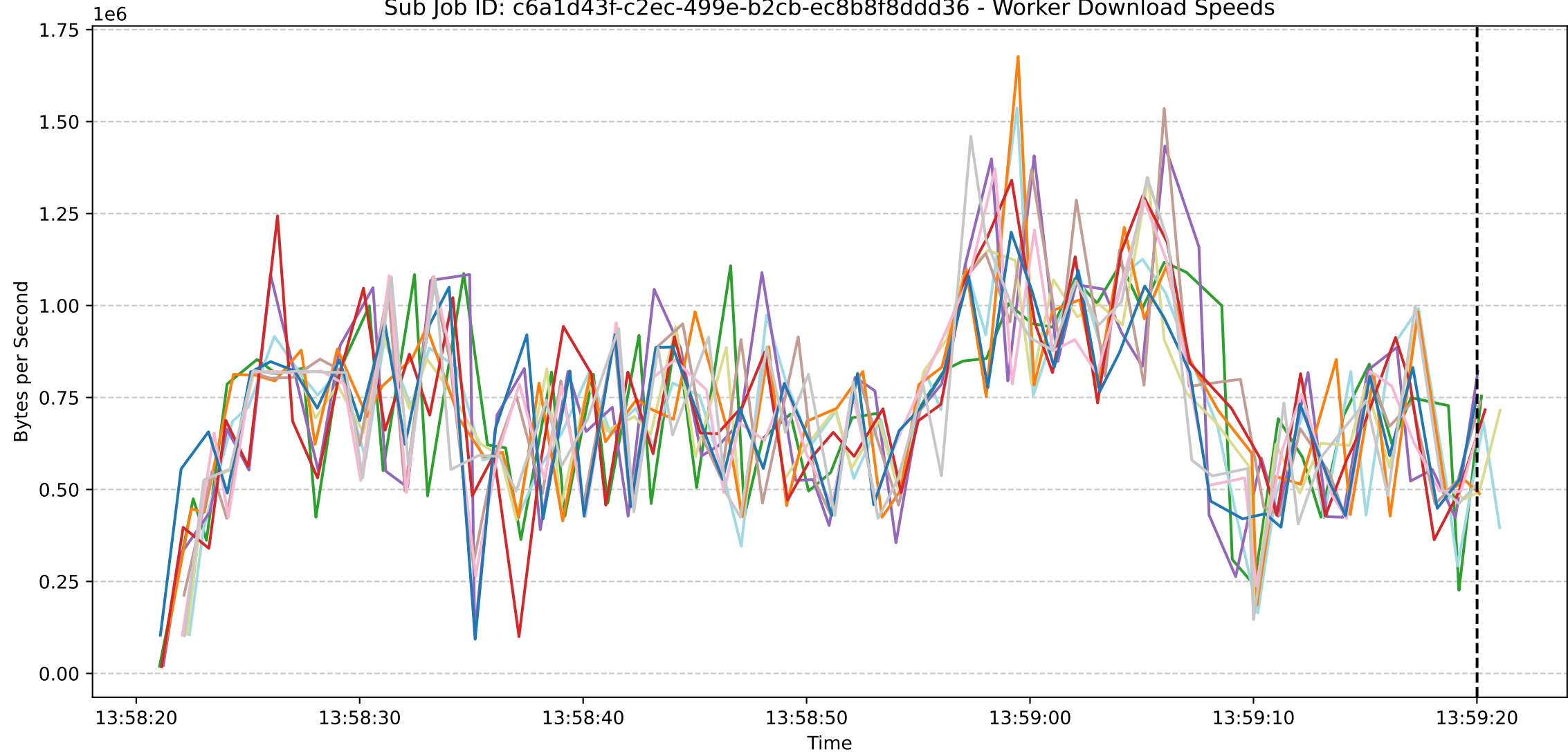
Sub Job ID: c6a1d43f-c2ec-499e-b2cb-ec8b8f8ddd36 - Worker Download Speeds
