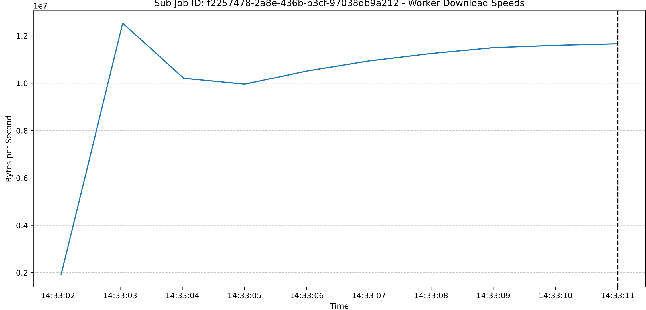
Sub Job ID: f2257478-2a8e-436b-b3cf-97038db9a212 - Worker Download Speeds
