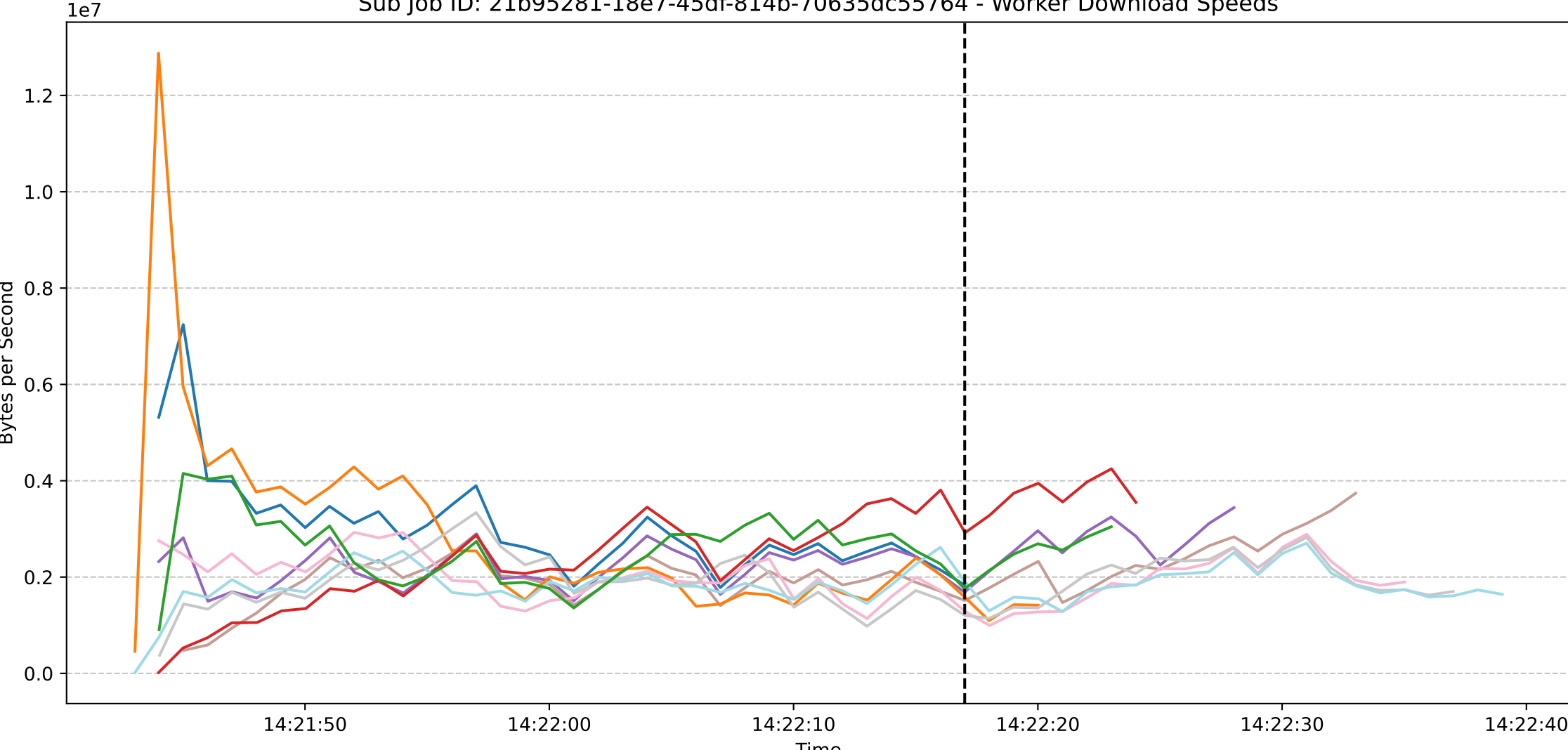
Sub Job ID: 21b95281-18e7-45df-814b-70635dc55764 - Worker Download Speeds
