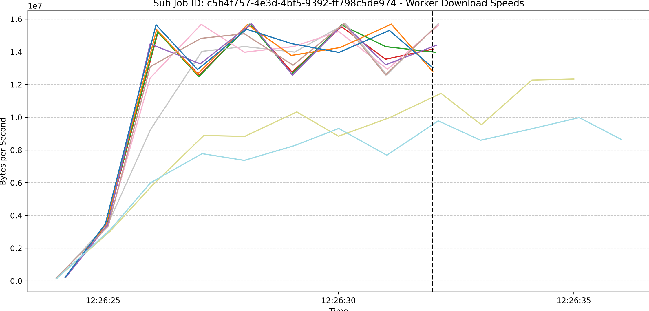
Sub Job ID: c5b4f757-4e3d-4bf5-9392-ff798c5de974 - Worker Download Speeds
