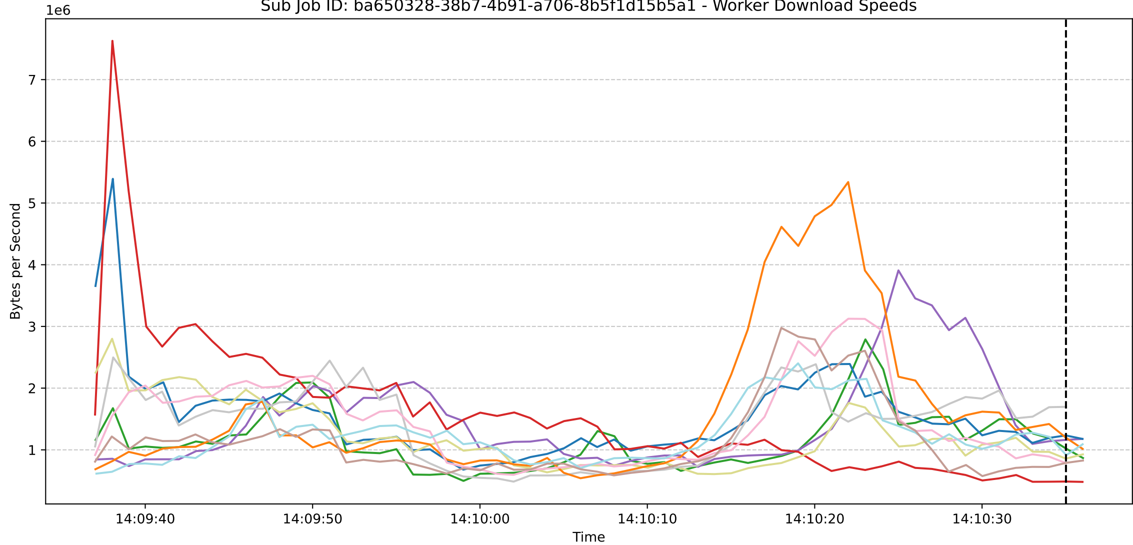
Sub Job ID: ba650328-38b7-4b91-a706-8b5f1d15b5a1 - Worker Download Speeds
