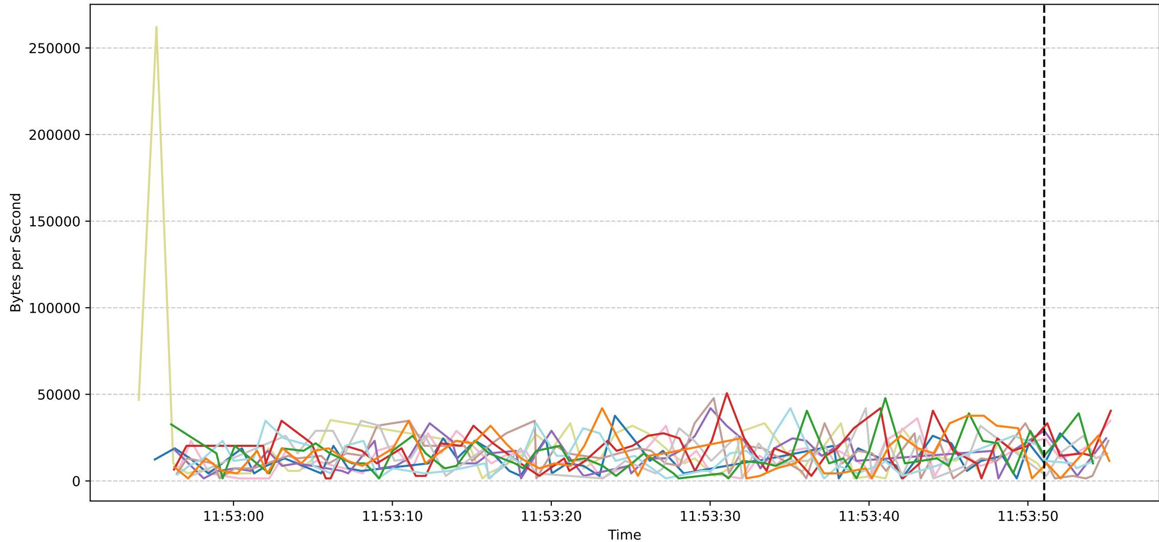
Sub Job ID: 651ad2dd-5862-4bc5-bf0b-8d9aebcb570e - Worker Download Speeds
