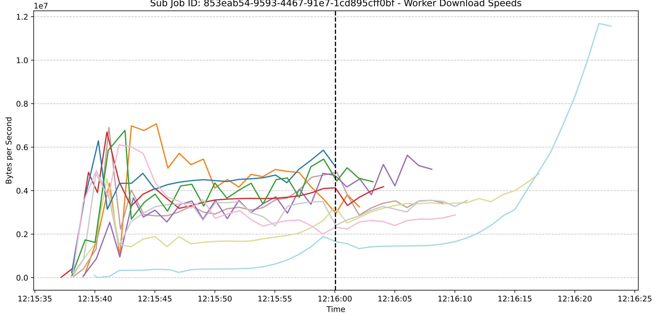
Sub Job ID: 853eab54-9593-4467-91e7-1cd895cff0bf - Worker Download Speeds
