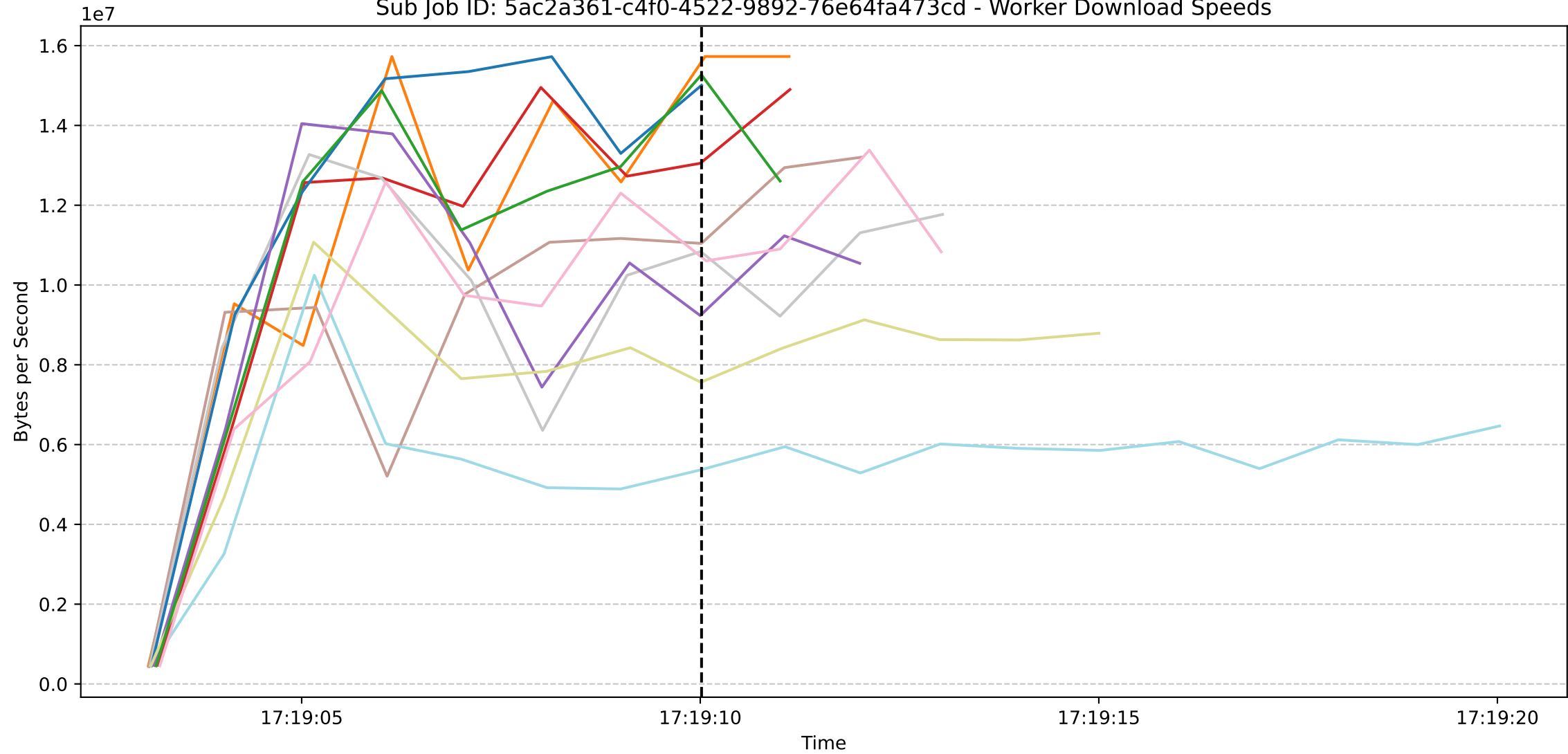
Sub Job ID: 5ac2a361-c4f0-4522-9892-76e64fa473cd - Worker Download Speeds
