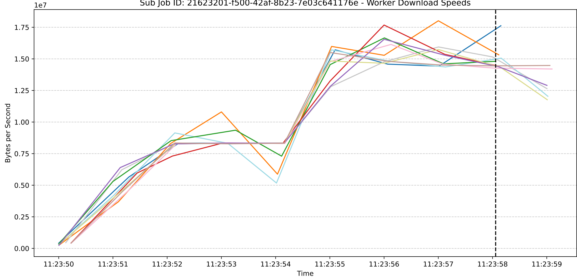
Sub Job ID: 21623201-f500-42af-8b23-7e03c641176e - Worker Download Speeds
