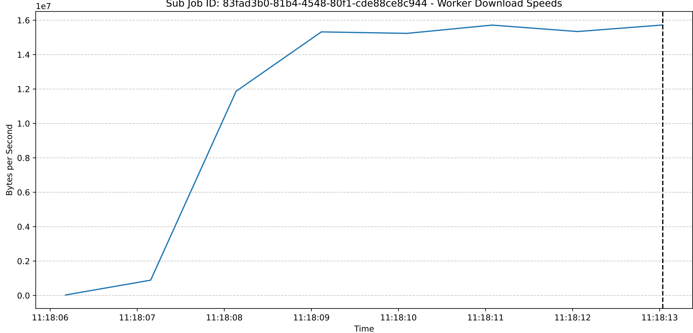
Sub Job ID: 83fad3b0-81b4-4548-80f1-cde88ce8c944 - Worker Download Speeds
