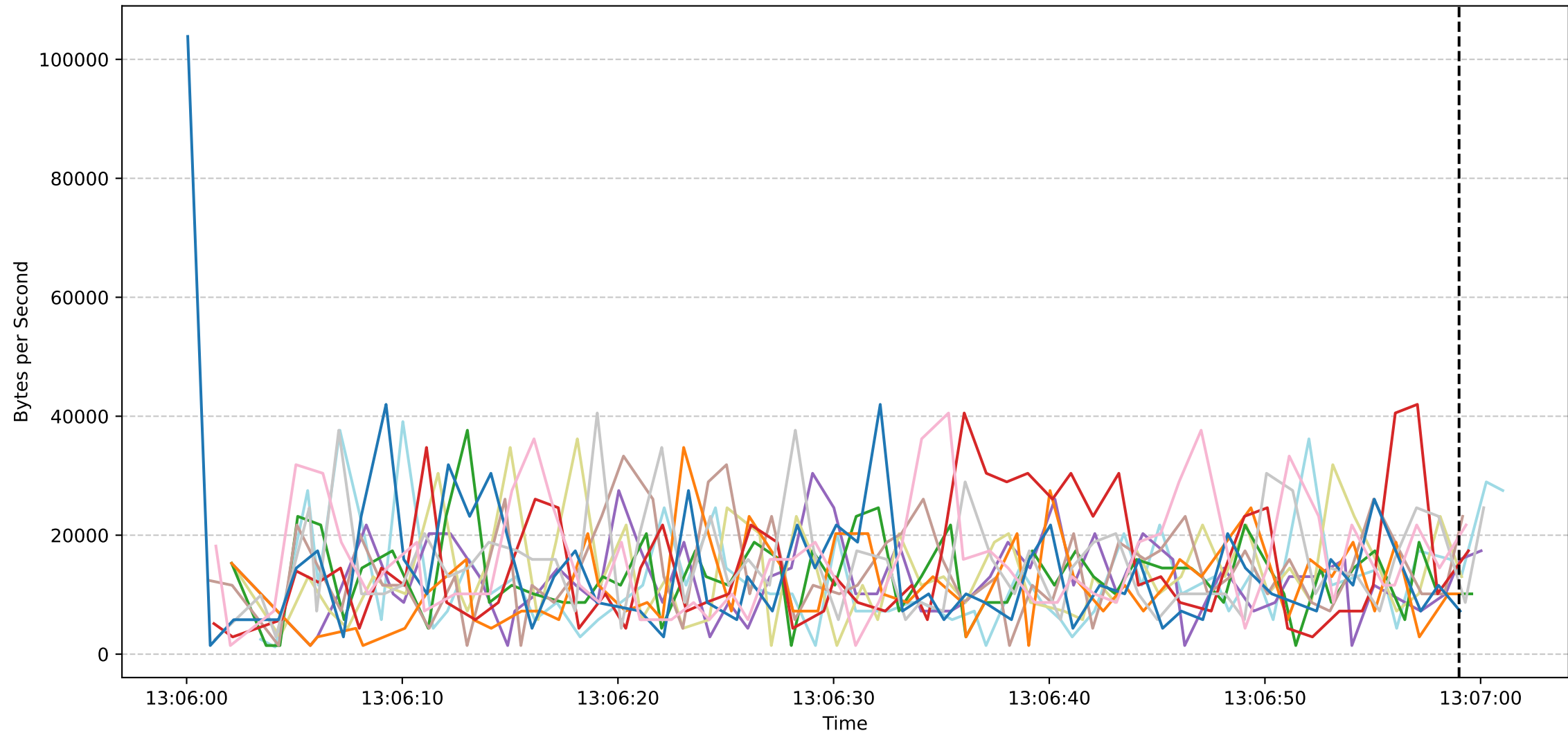
Sub Job ID: e416f307-c56a-4b24-917b-71c342a68f6b - Worker Download Speeds
