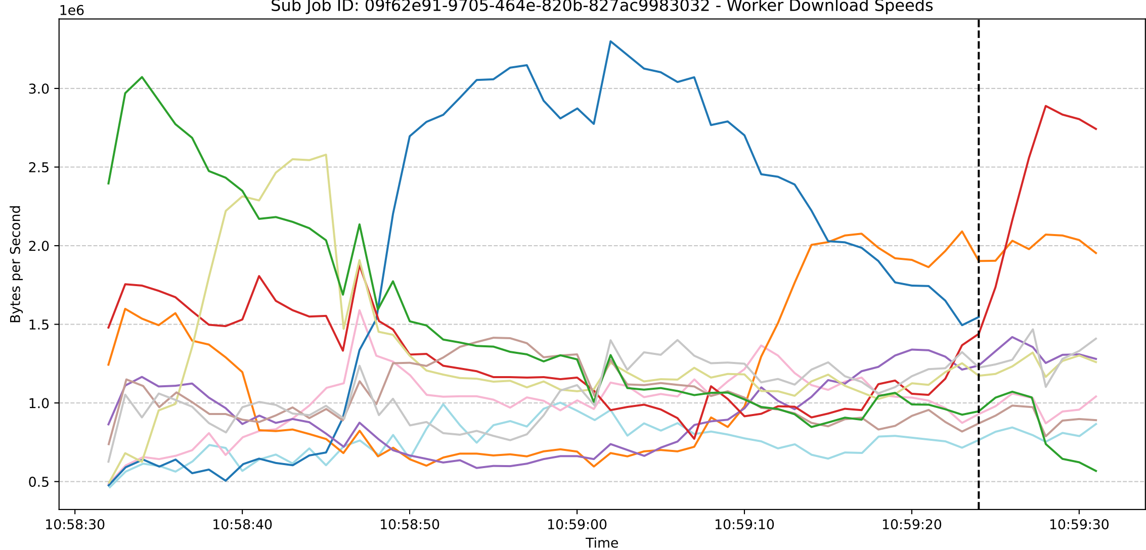
Sub Job ID: 09f62e91-9705-464e-820b-827ac9983032 - Worker Download Speeds
