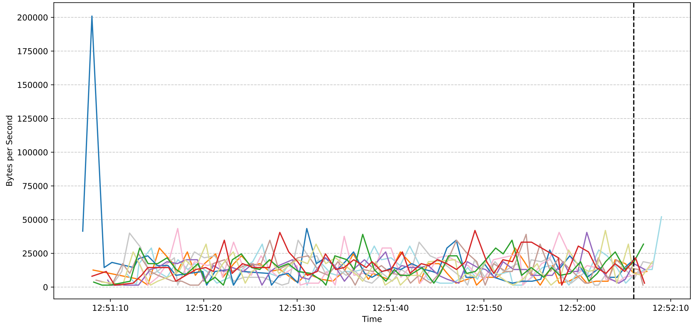
Sub Job ID: 1a3761e3-991c-41ae-8d59-7e06104019b4 - Worker Download Speeds
