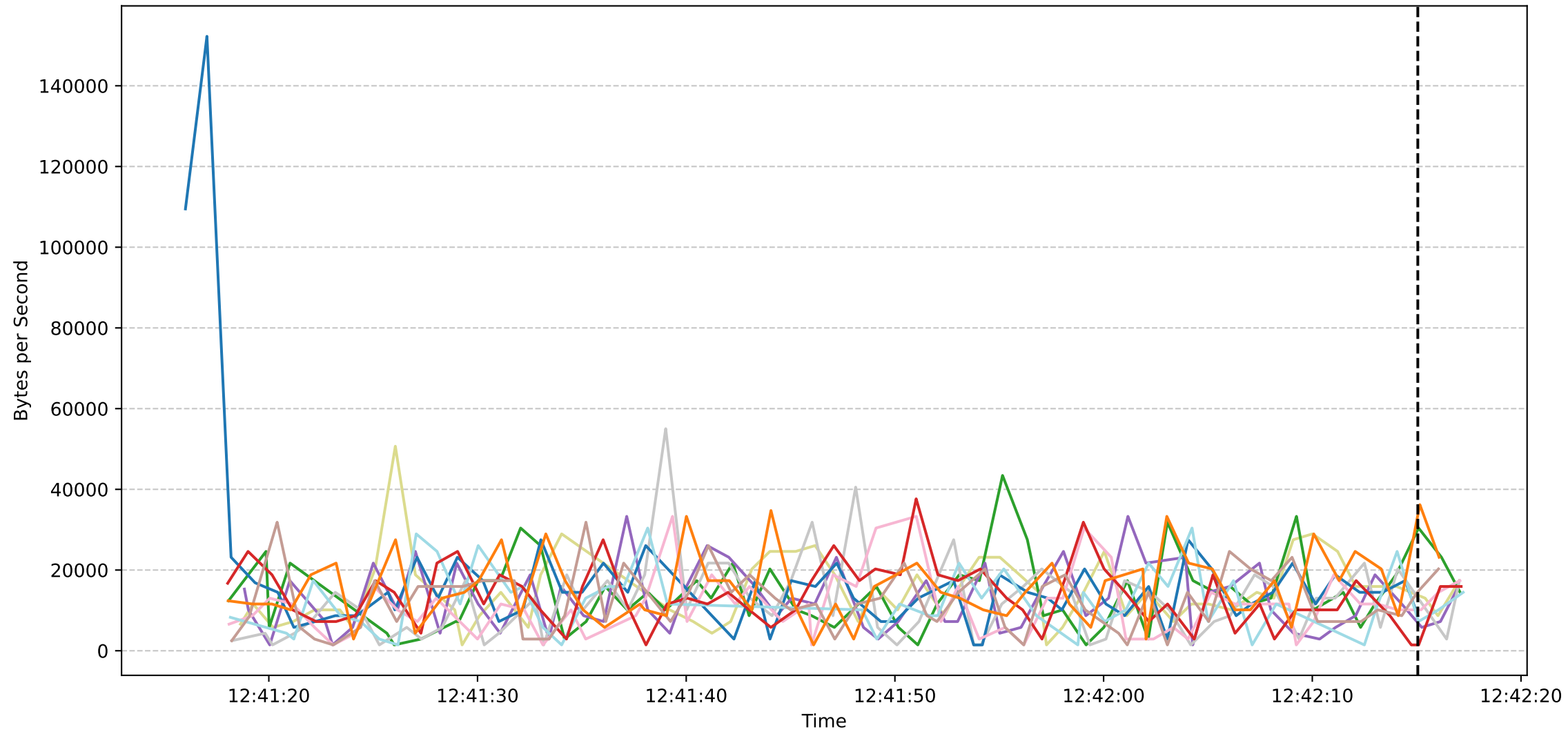
Sub Job ID: b88d8755-2b06-4a79-a4f3-1d772164f374 - Worker Download Speeds
