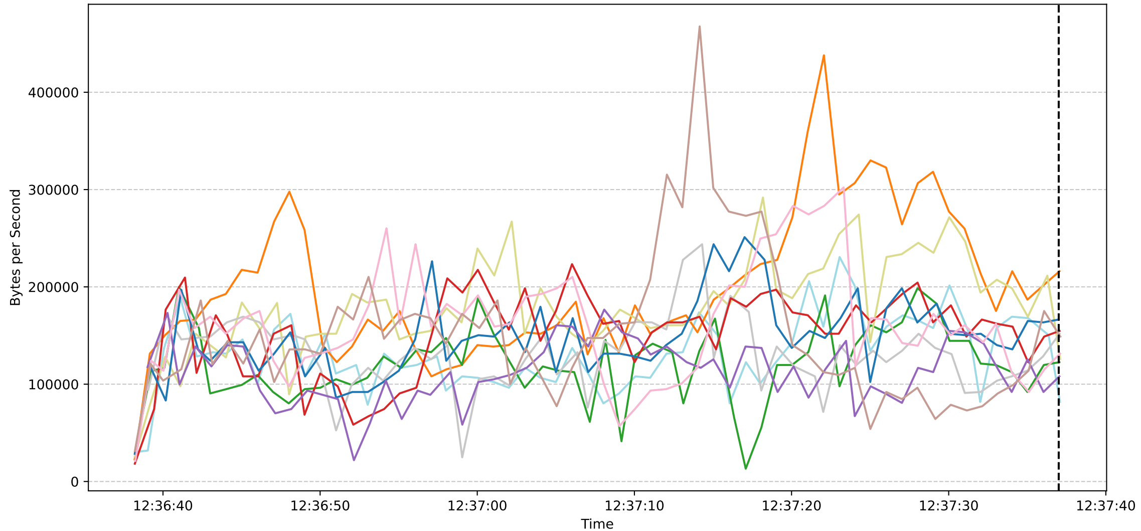
Sub Job ID: 86f7ed84-9097-437c-90a8-2095ca85cb26 - Worker Download Speeds
