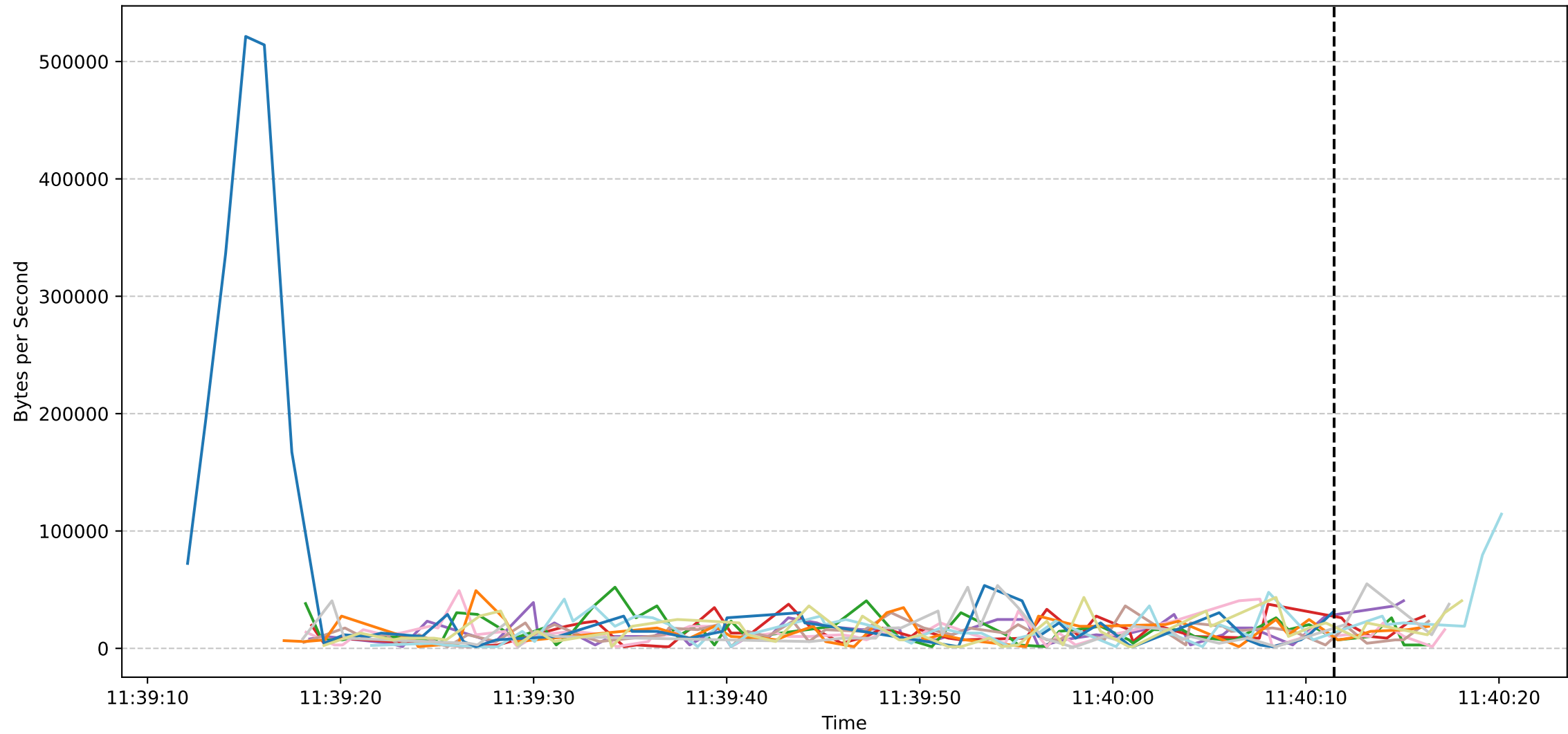
Sub Job ID: 4dc5f42f-8962-4831-a828-b021123d7b02 - Worker Download Speeds
