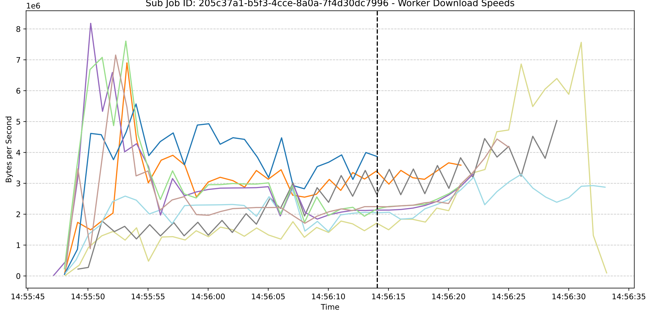
Sub Job ID: 205c37a1-b5f3-4cce-8a0a-7f4d30dc7996 - Worker Download Speeds
