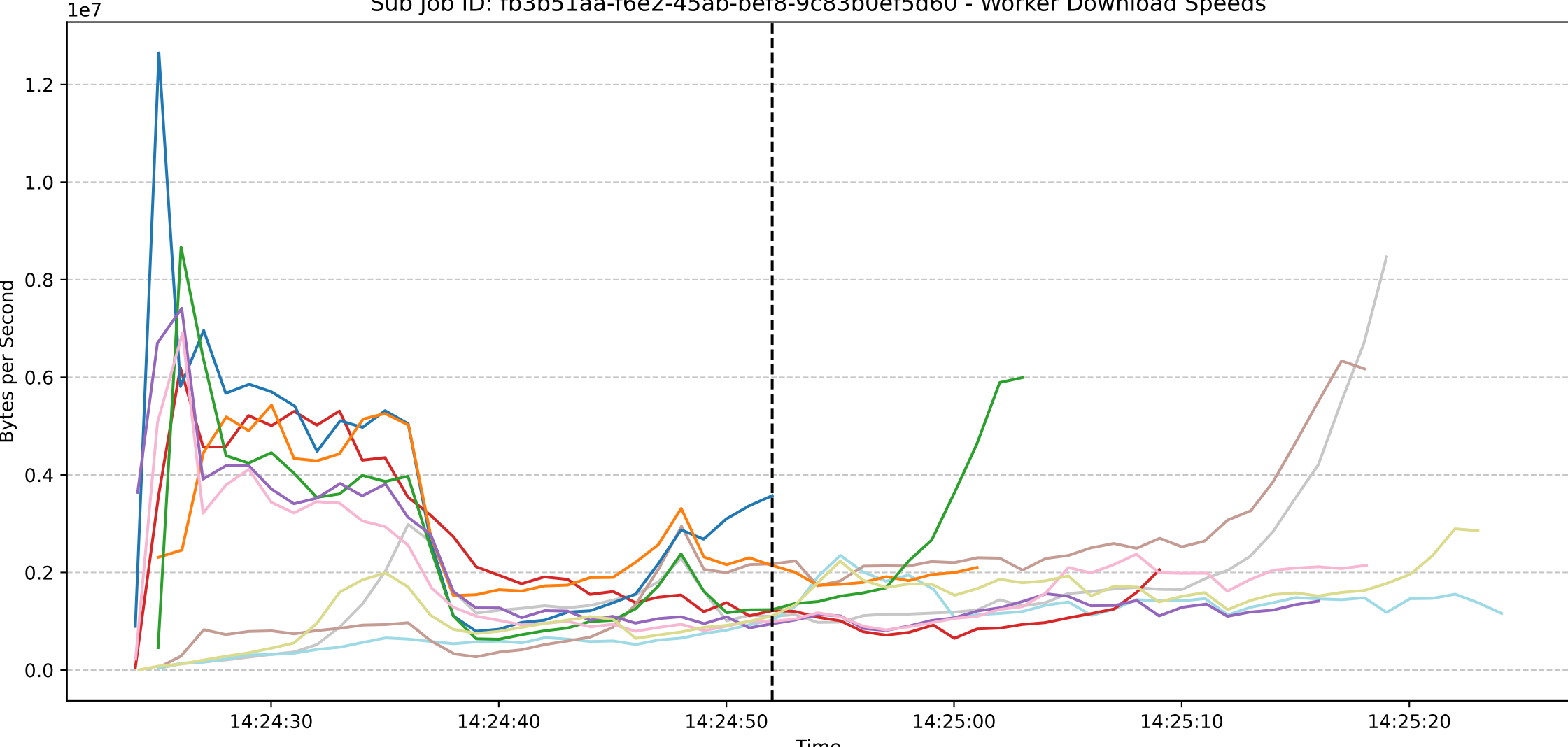
Sub Job ID: fb3b51aa-f6e2-45ab-bef8-9c83b0ef5d60 - Worker Download Speeds
