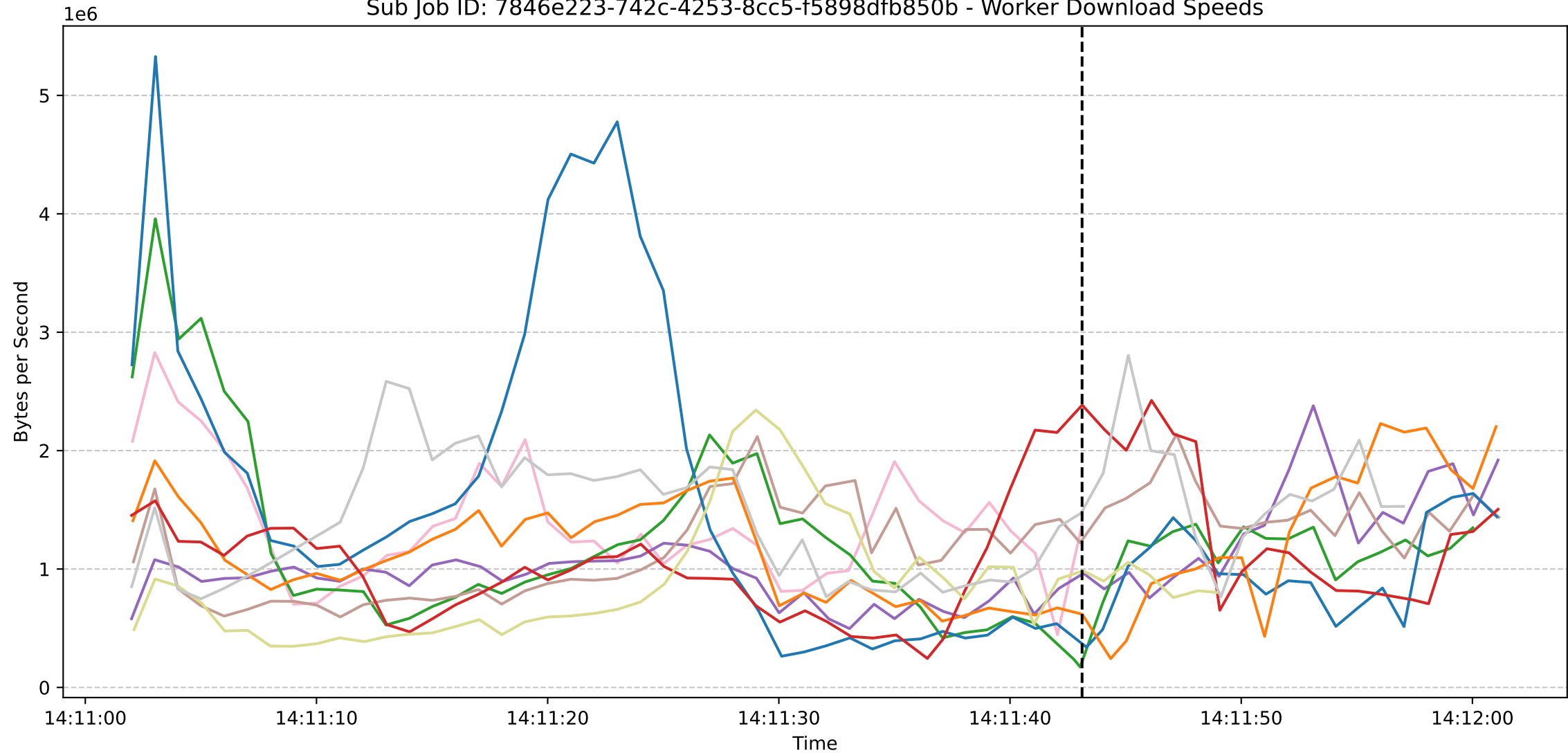
Sub Job ID: 7846e223-742c-4253-8cc5-f5898dfb850b - Worker Download Speeds
