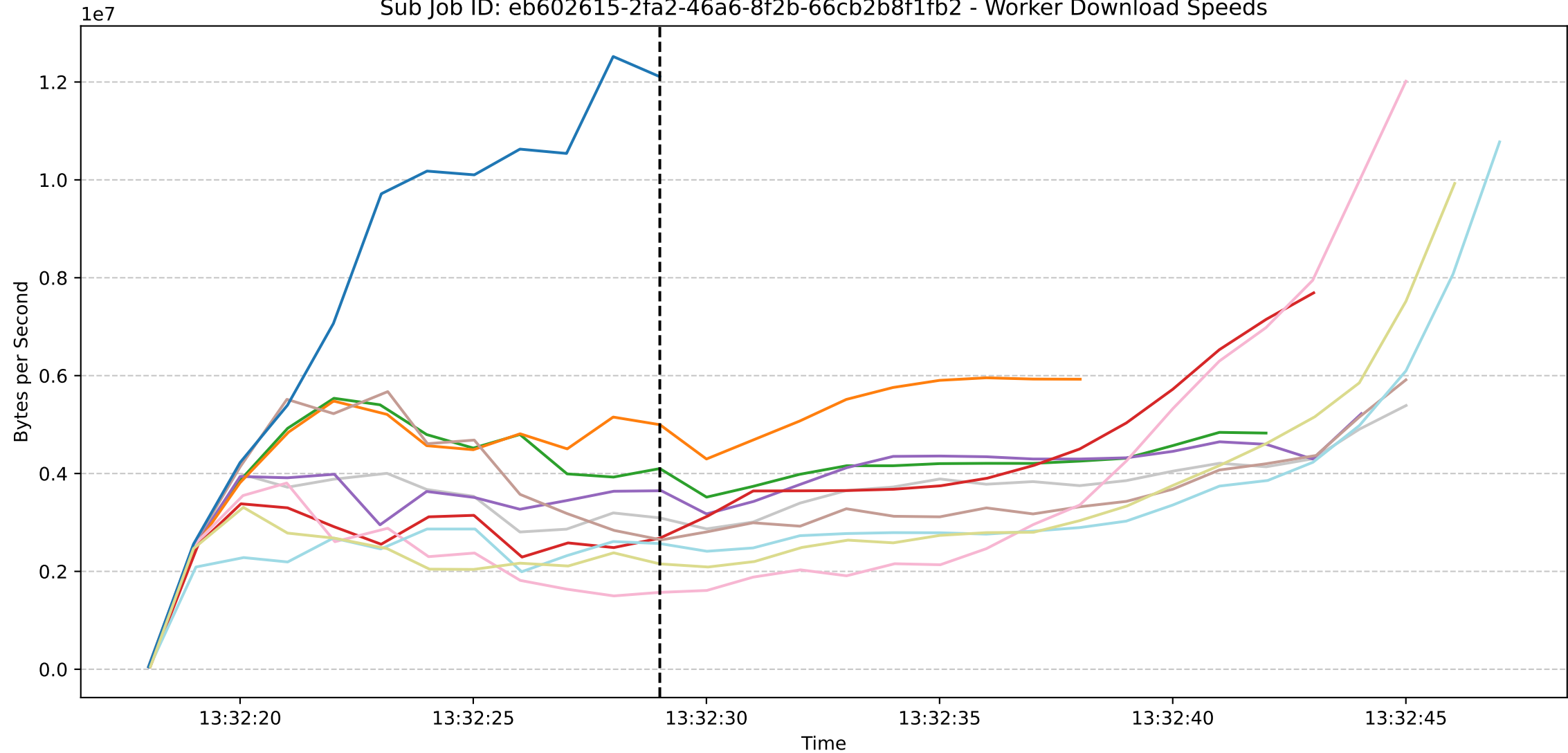
Sub Job ID: eb602615-2fa2-46a6-8f2b-66cb2b8f1fb2 - Worker Download Speeds
