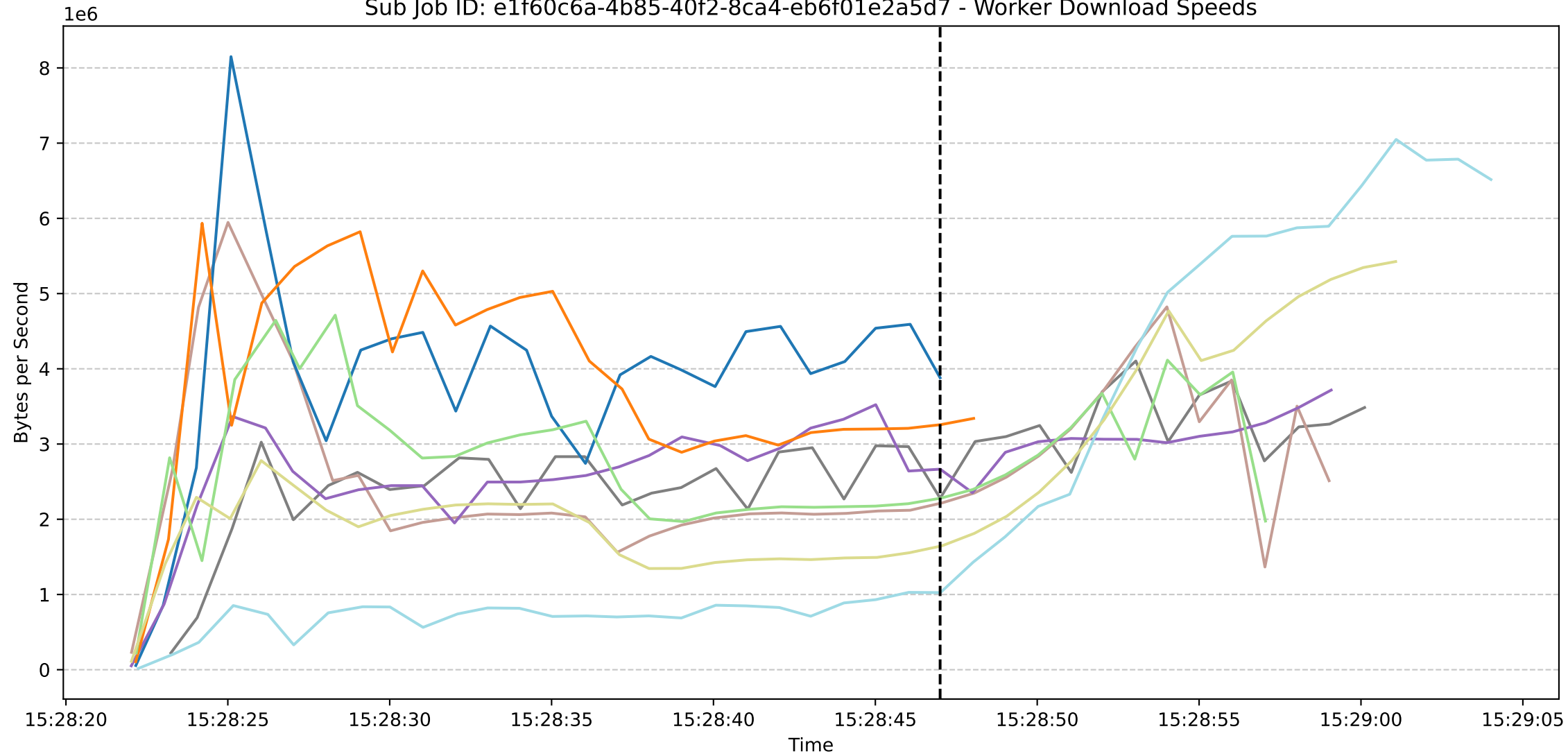
Sub Job ID: e1f60c6a-4b85-40f2-8ca4-eb6f01e2a5d7 - Worker Download Speeds
