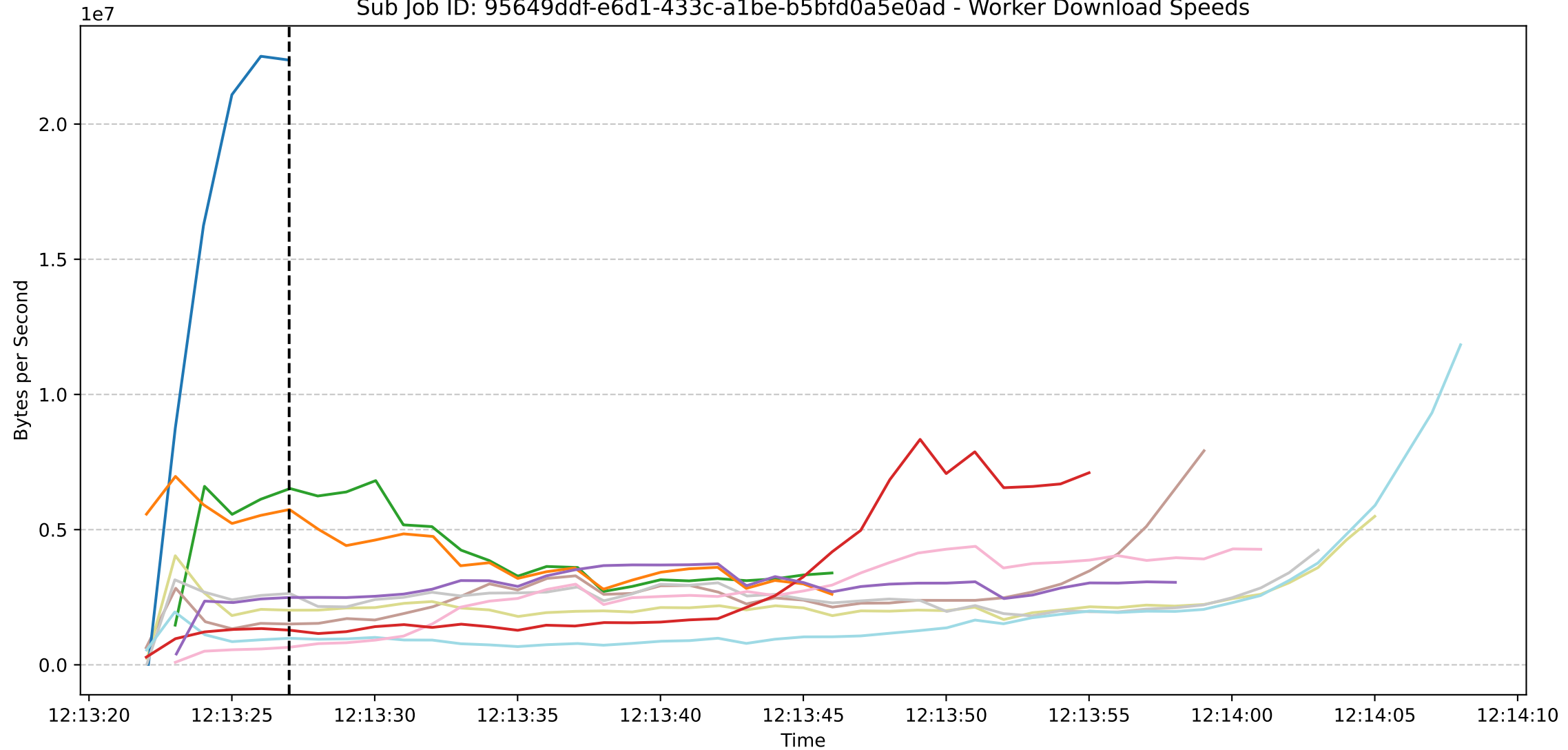
Sub Job ID: 95649ddf-e6d1-433c-a1be-b5bfd0a5e0ad - Worker Download Speeds
