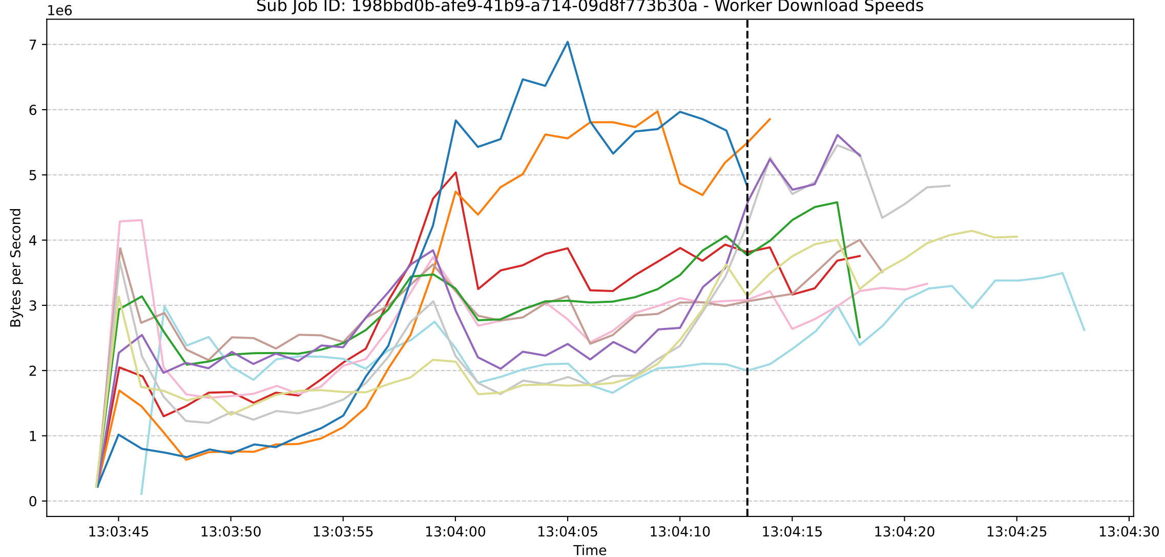
Sub Job ID: 198bbd0b-afe9-41b9-a714-09d8f773b30a - Worker Download Speeds
