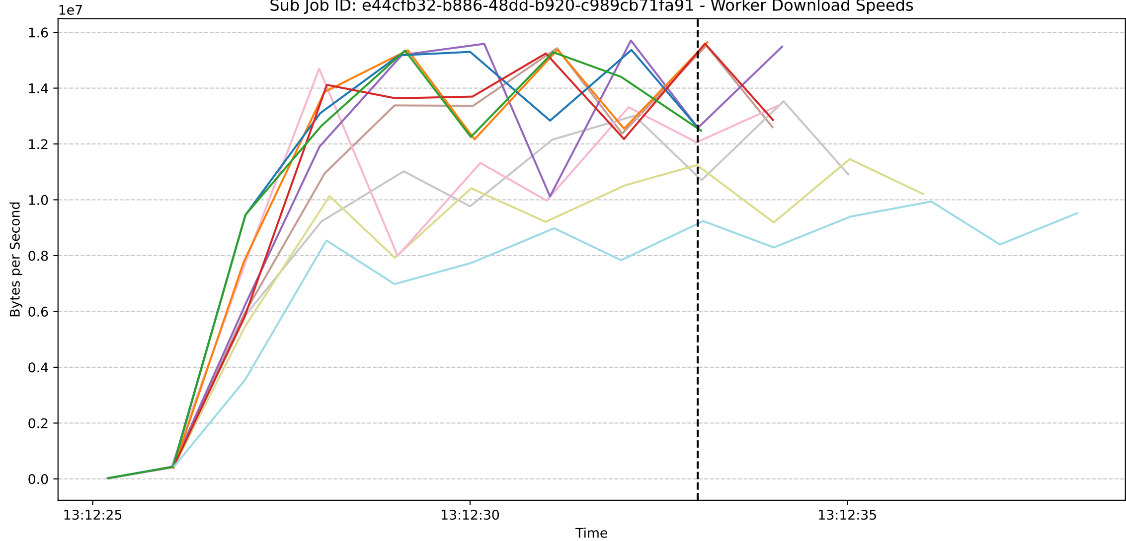
Sub Job ID: e44cfb32-b886-48dd-b920-c989cb71fa91 - Worker Download Speeds
