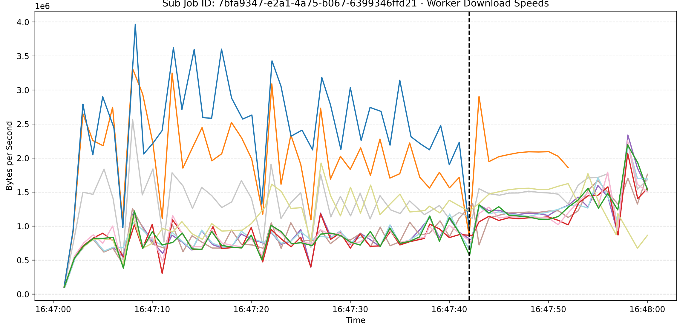
Sub Job ID: 7bfa9347-e2a1-4a75-b067-6399346ffd21 - Worker Download Speeds
