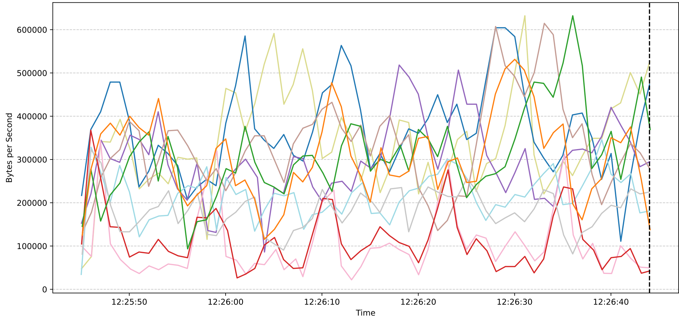
Sub Job ID: af07d920-533f-4b8f-bc72-bde5e1d6c61b - Worker Download Speeds
