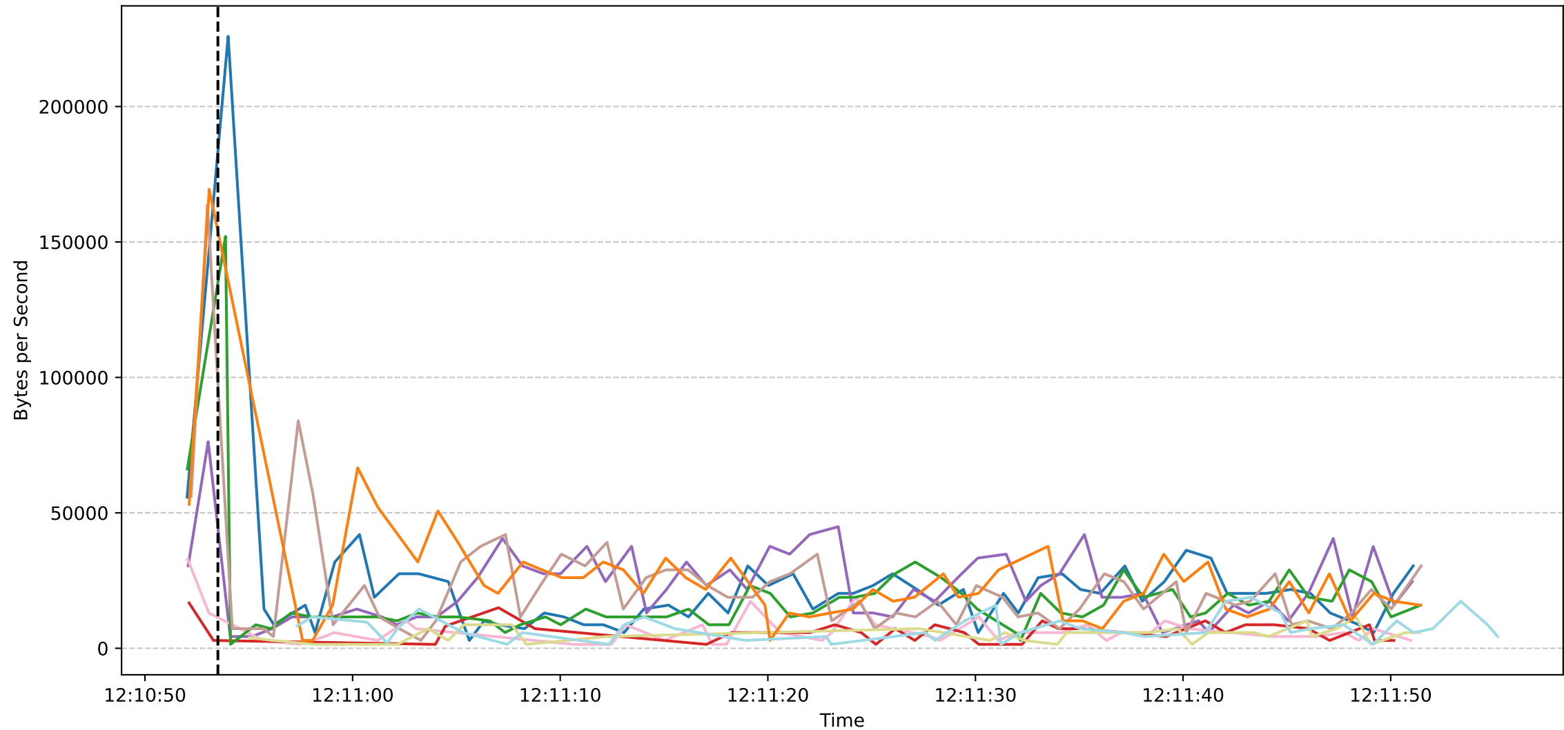
Sub Job ID: 38f82f7a-4230-47b8-a84e-266bb4c09998 - Worker Download Speeds
