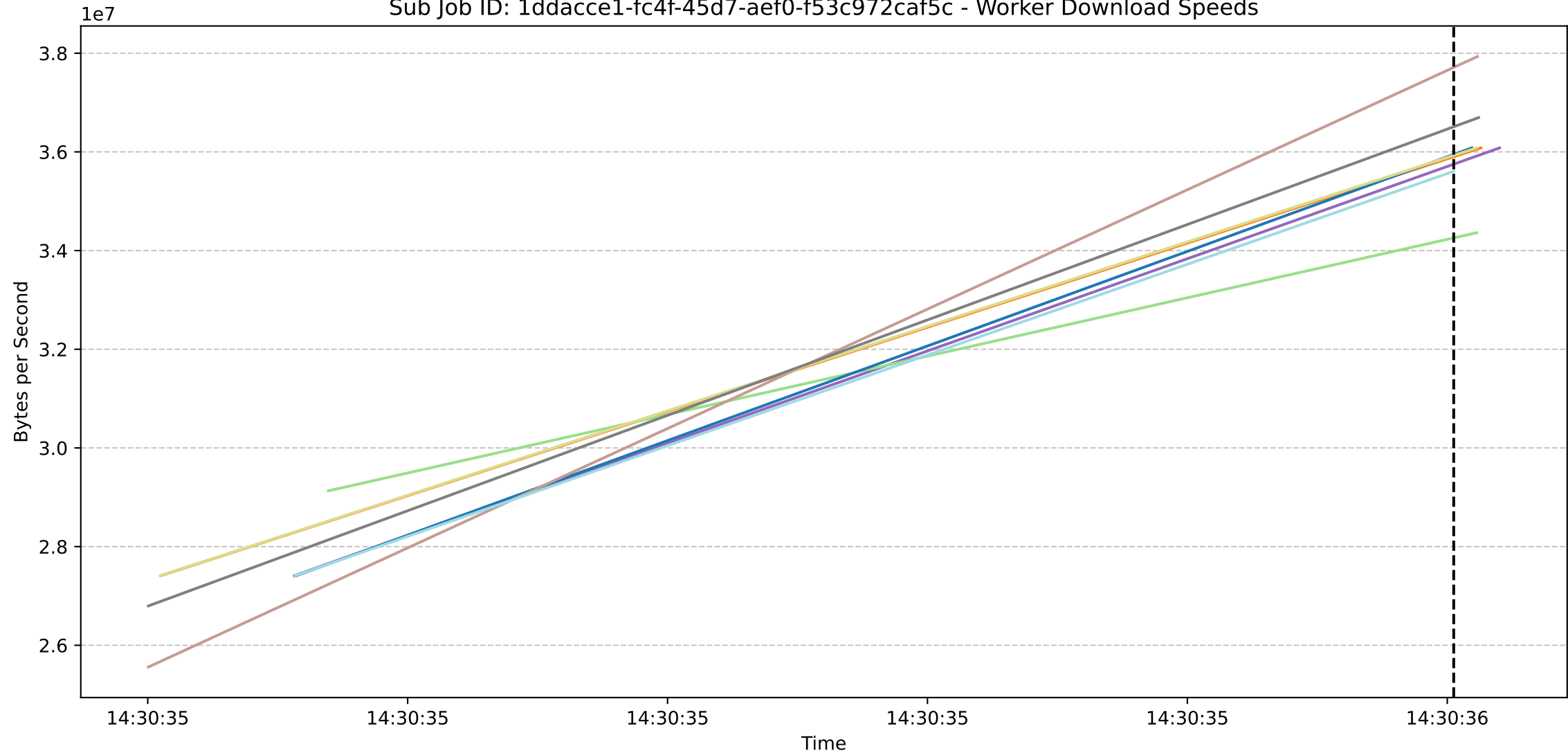
Sub Job ID: 1ddacce1-fc4f-45d7-aef0-f53c972caf5c - Worker Download Speeds
