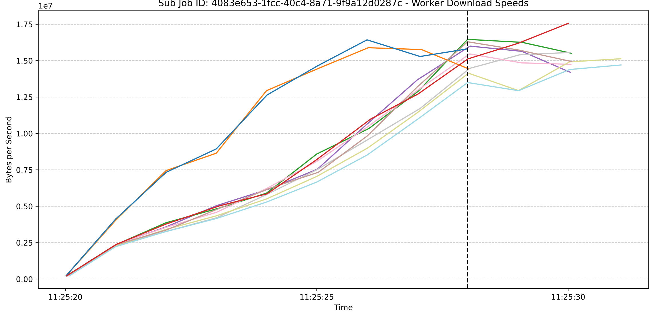
Sub Job ID: 4083e653-1fcc-40c4-8a71-9f9a12d0287c - Worker Download Speeds
