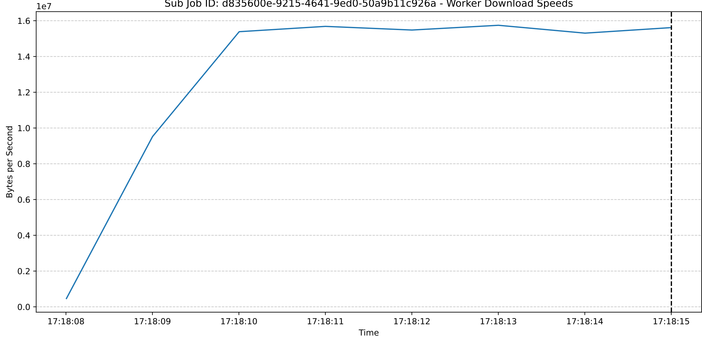
Sub Job ID: d835600e-9215-4641-9ed0-50a9b11c926a - Worker Download Speeds
