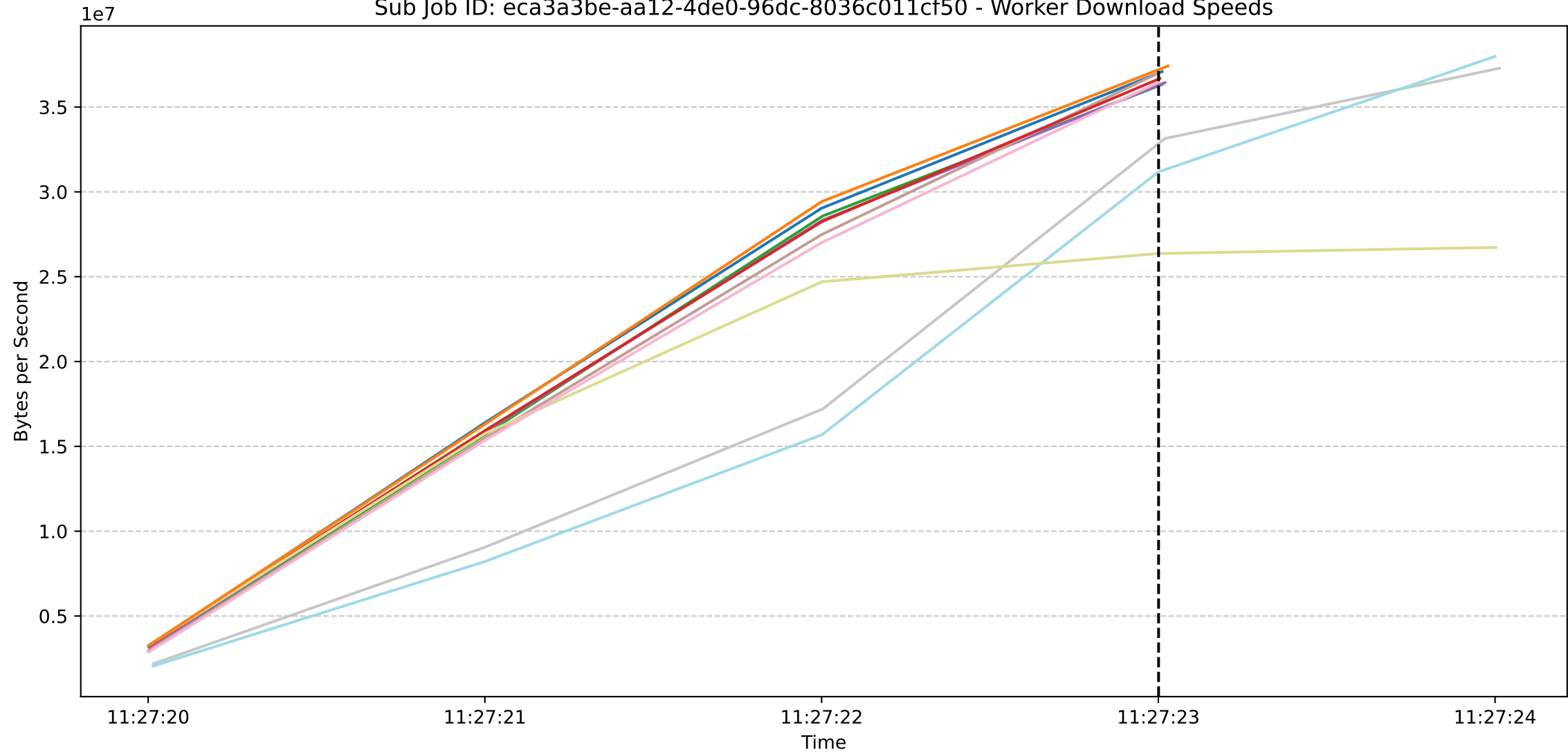
Sub Job ID: eca3a3be-aa12-4de0-96dc-8036c011cf50 - Worker Download Speeds
