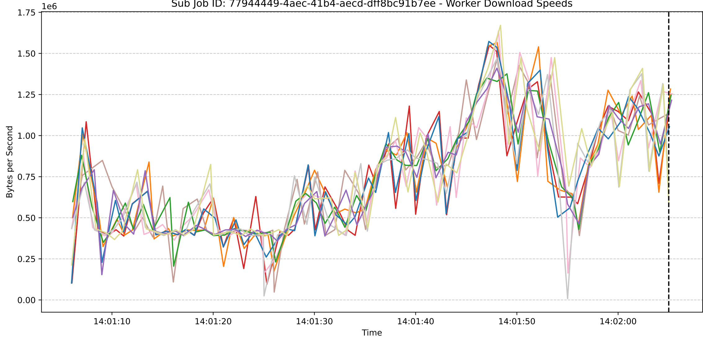
Sub Job ID: 77944449-4aec-41b4-aecd-dff8bc91b7ee - Worker Download Speeds
