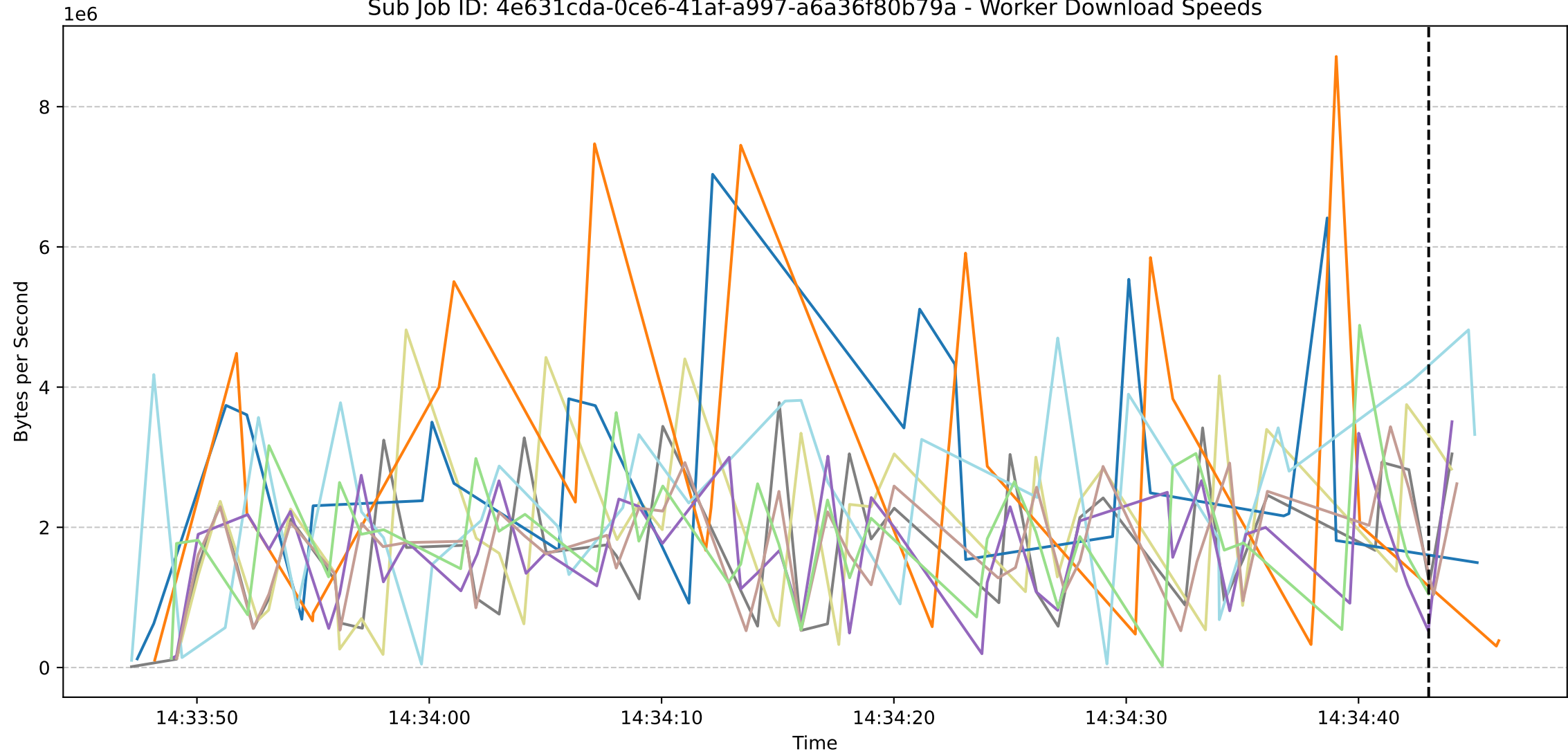
Sub Job ID: 4e631cda-0ce6-41af-a997-a6a36f80b79a - Worker Download Speeds
