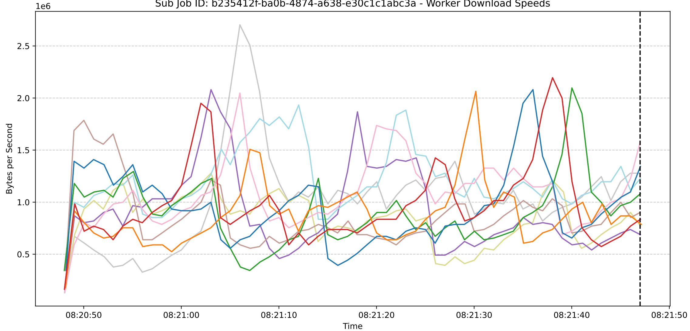
Sub Job ID: b235412f-ba0b-4874-a638-e30c1c1abc3a - Worker Download Speeds
