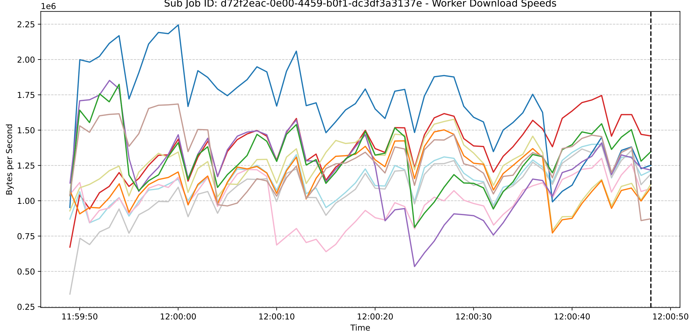
Sub Job ID: d72f2eac-0e00-4459-b0f1-dc3df3a3137e - Worker Download Speeds
