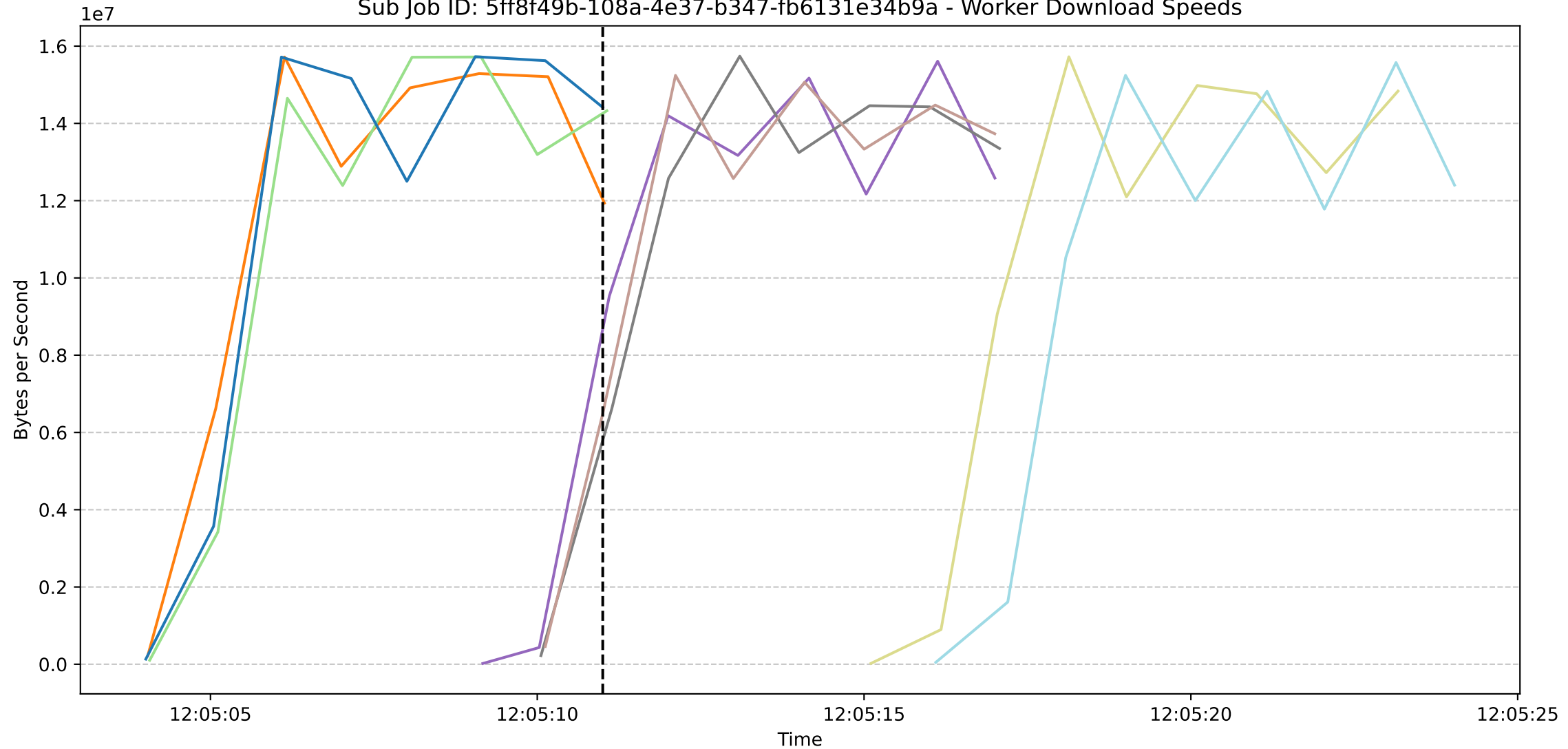
Sub Job ID: 5ff8f49b-108a-4e37-b347-fb6131e34b9a - Worker Download Speeds
