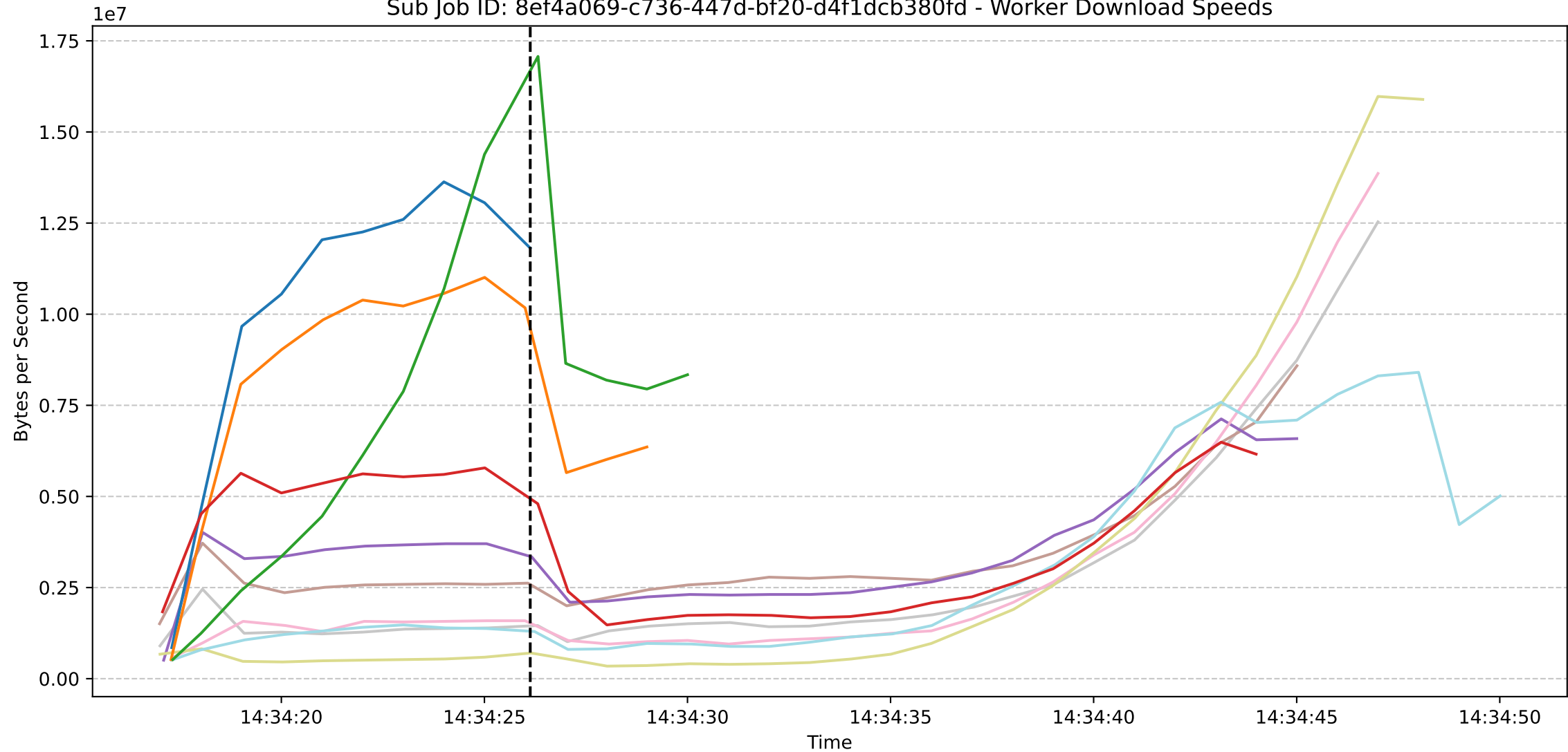
Sub Job ID: 8ef4a069-c736-447d-bf20-d4f1dcb380fd - Worker Download Speeds
