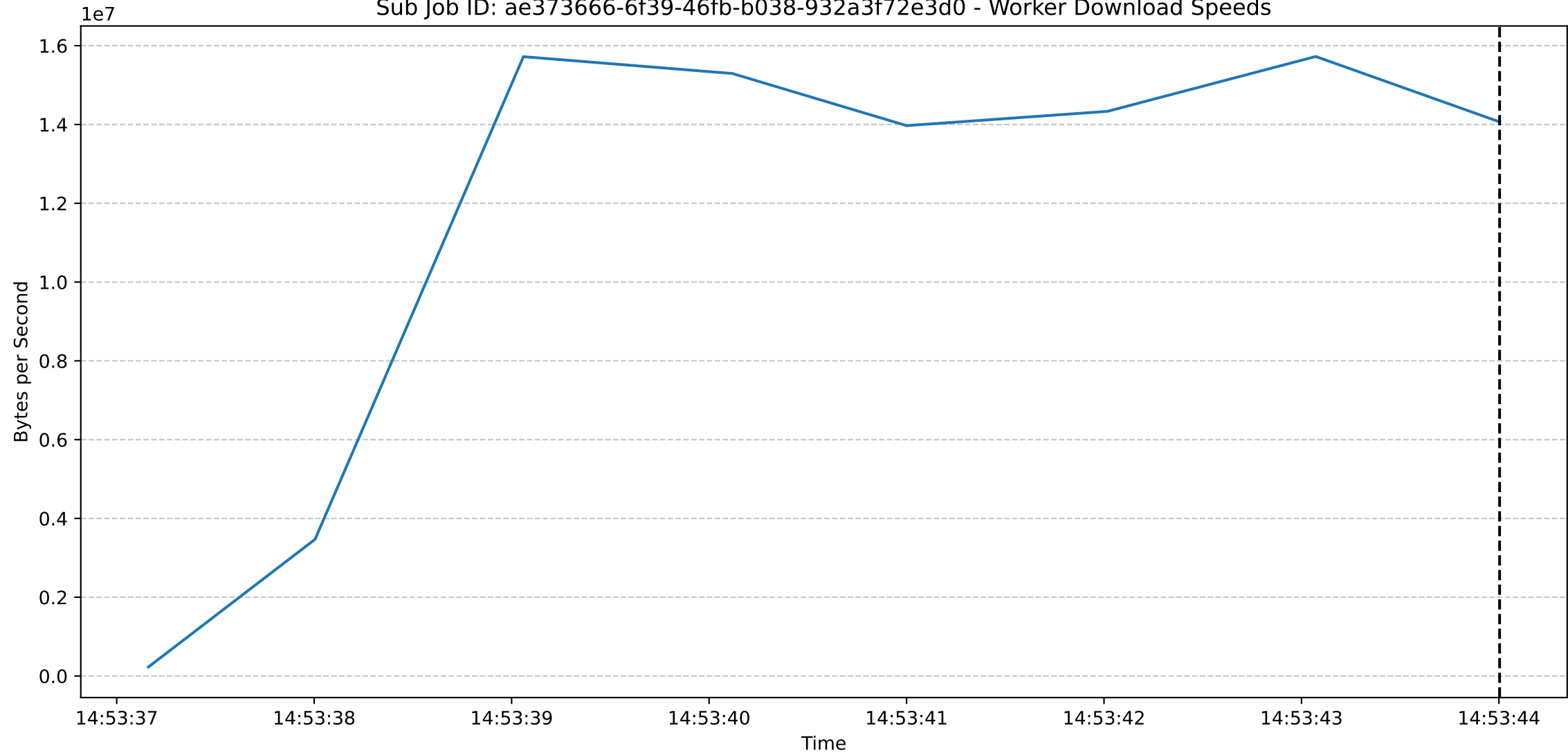
Sub Job ID: ae373666-6f39-46fb-b038-932a3f72e3d0 - Worker Download Speeds
