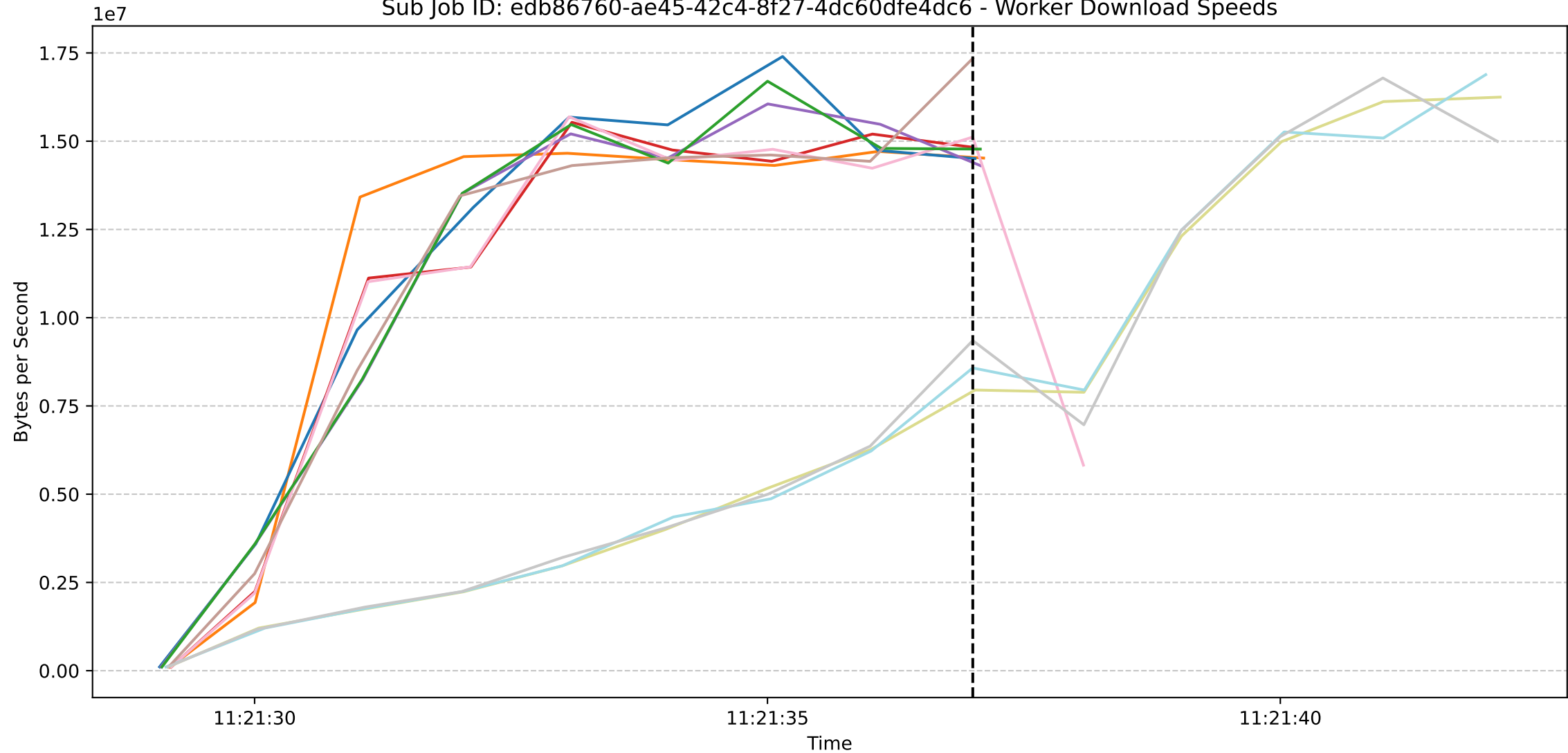
Sub Job ID: edb86760-ae45-42c4-8f27-4dc60dfe4dc6 - Worker Download Speeds
