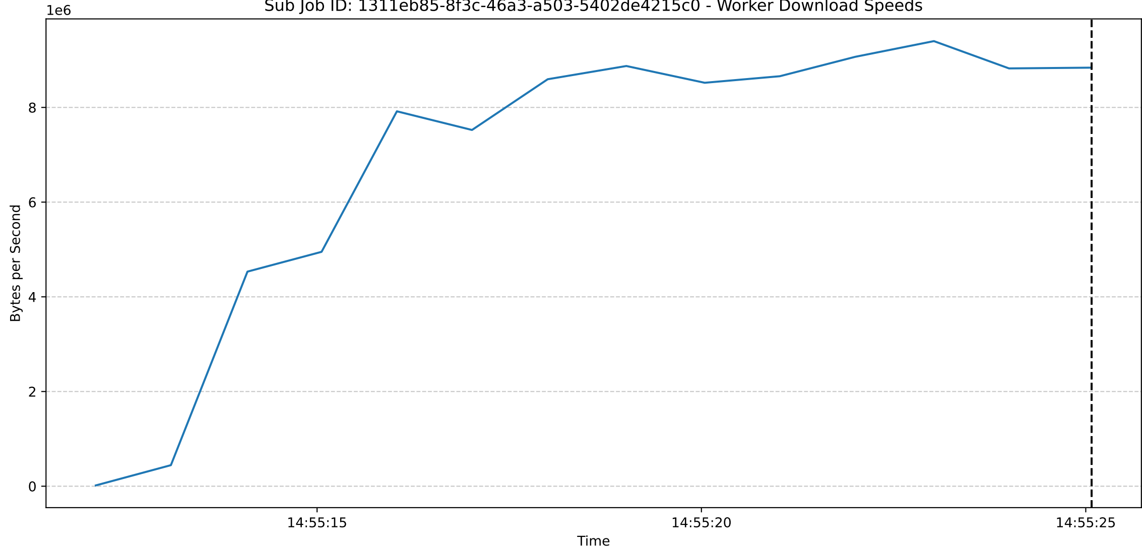
Sub Job ID: 1311eb85-8f3c-46a3-a503-5402de4215c0 - Worker Download Speeds
