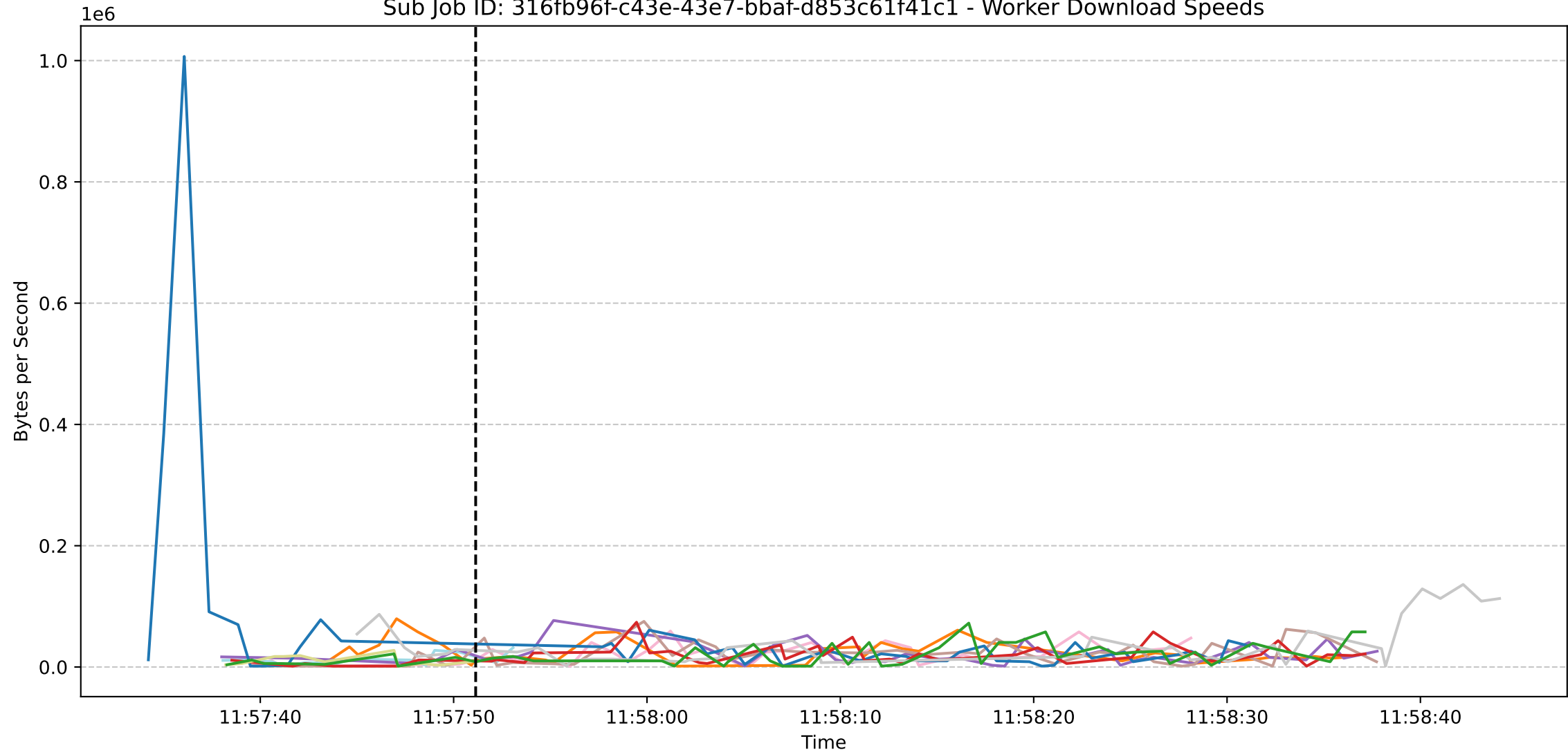
Sub Job ID: 316fb96f-c43e-43e7-bbaf-d853c61f41c1 - Worker Download Speeds
