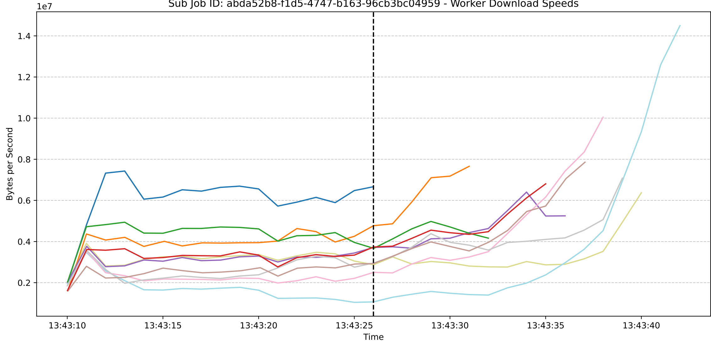
Sub Job ID: abda52b8-f1d5-4747-b163-96cb3bc04959 - Worker Download Speeds
