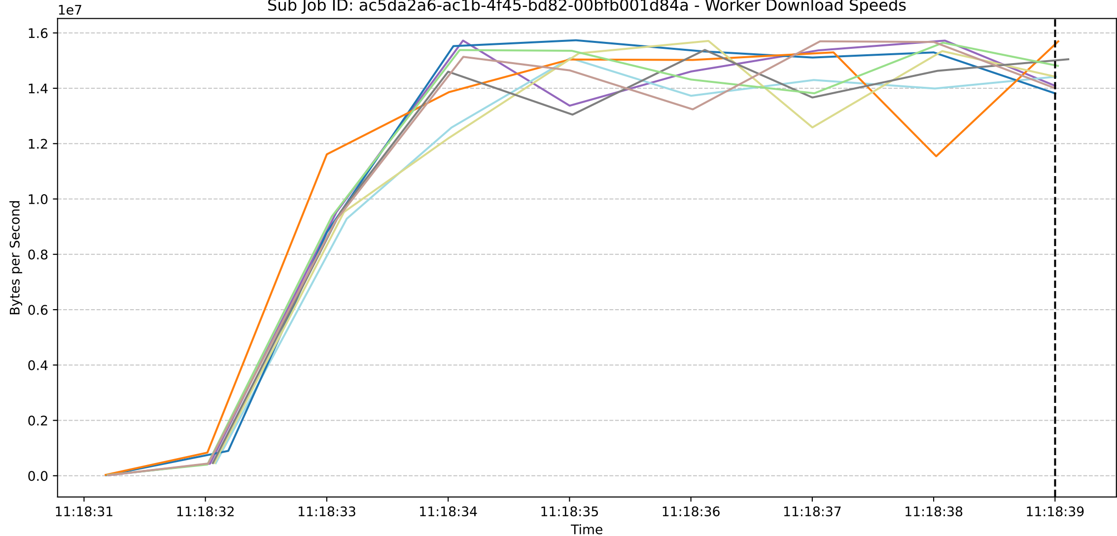
Sub Job ID: ac5da2a6-ac1b-4f45-bd82-00bfb001d84a - Worker Download Speeds
