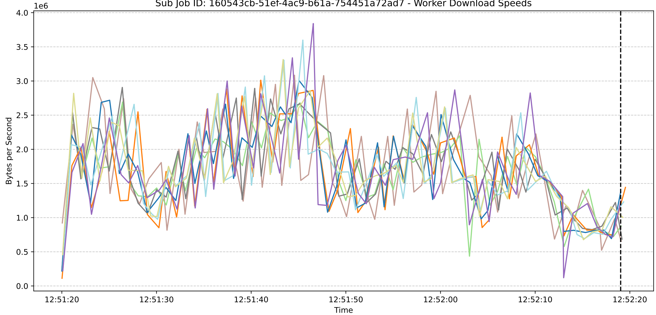
Sub Job ID: 160543cb-51ef-4ac9-b61a-754451a72ad7 - Worker Download Speeds
