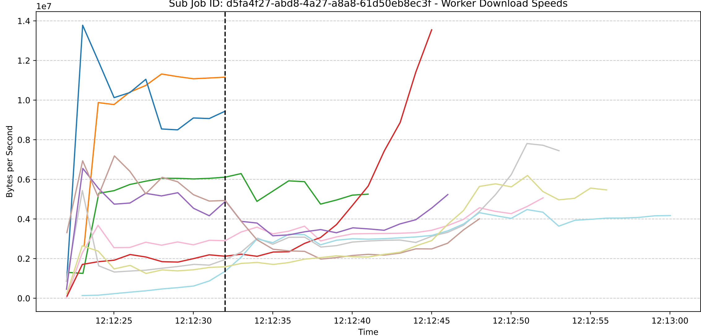
Sub Job ID: d5fa4f27-abd8-4a27-a8a8-61d50eb8ec3f - Worker Download Speeds
