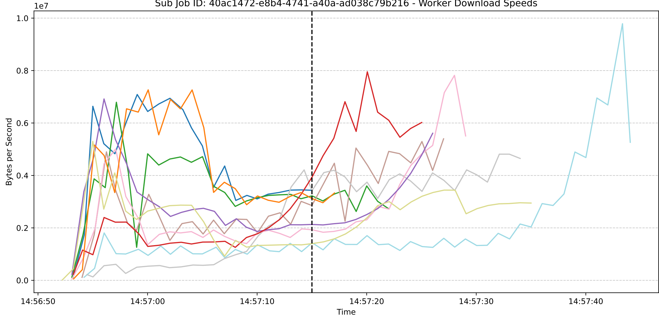
Sub Job ID: 40ac1472-e8b4-4741-a40a-ad038c79b216 - Worker Download Speeds
