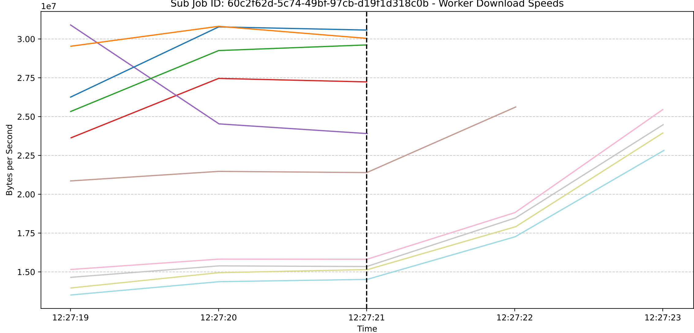
Sub Job ID: 60c2f62d-5c74-49bf-97cb-d19f1d318c0b - Worker Download Speeds
