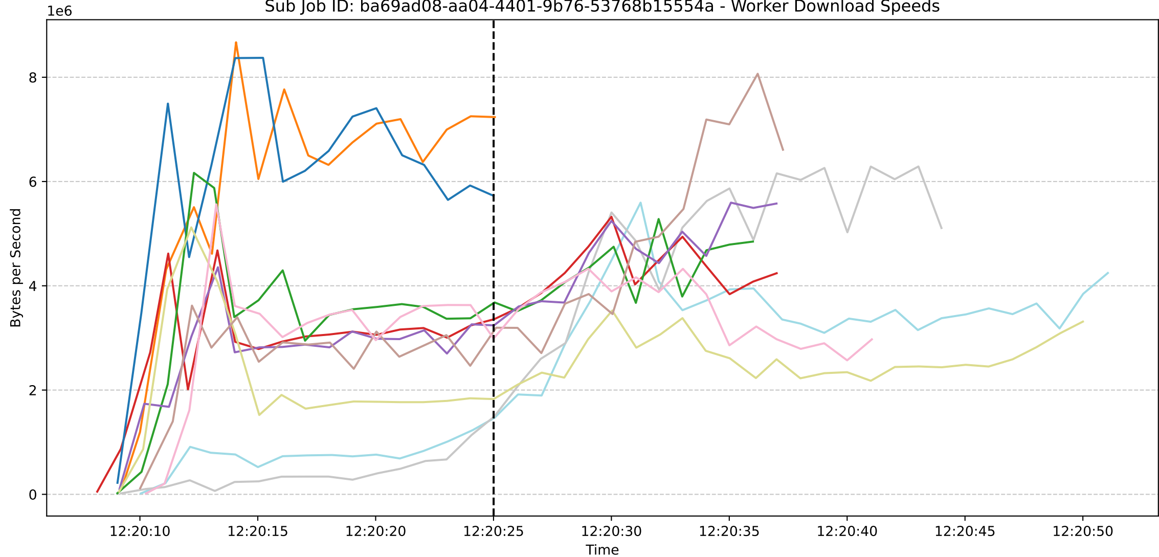
Sub Job ID: ba69ad08-aa04-4401-9b76-53768b15554a - Worker Download Speeds
