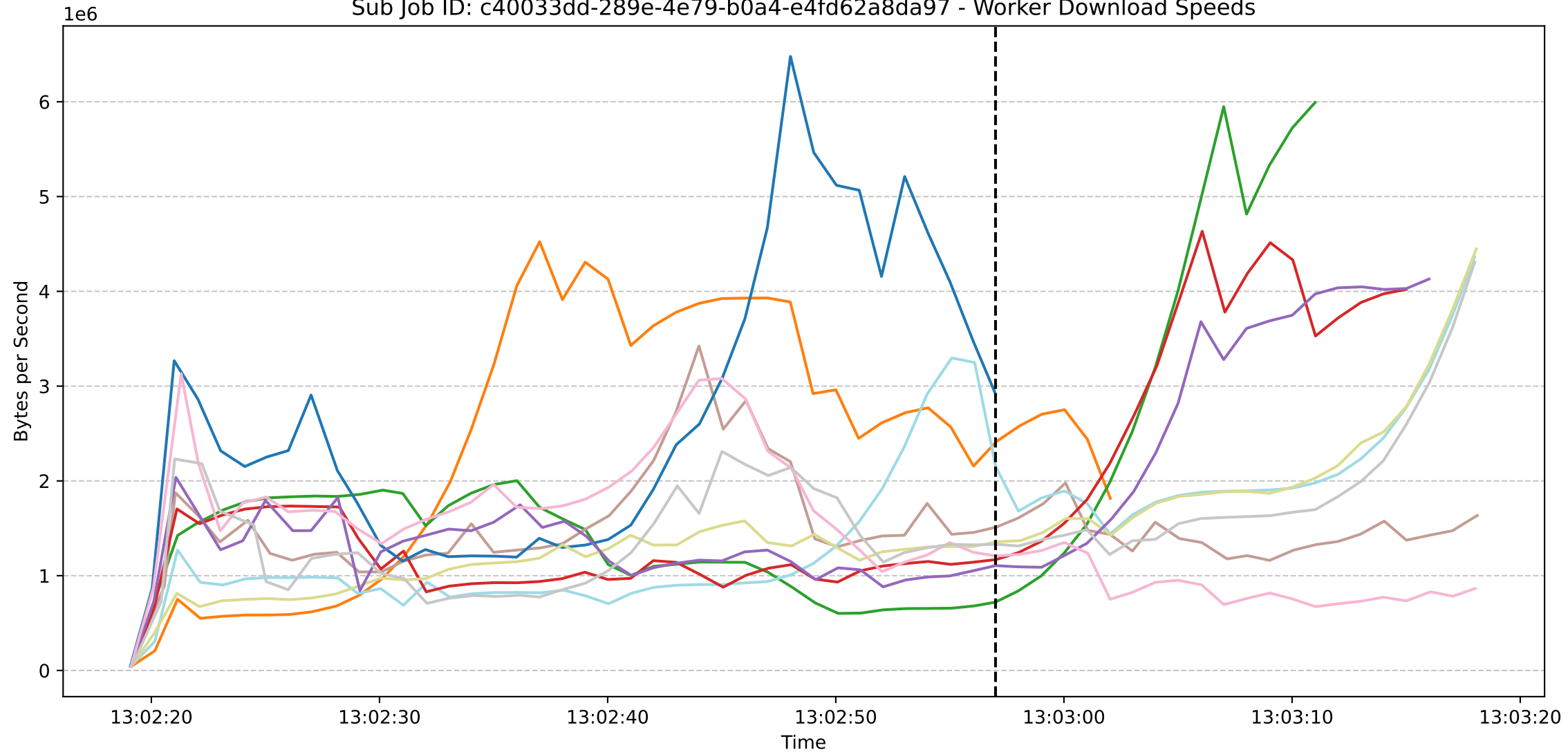
Sub Job ID: c40033dd-289e-4e79-b0a4-e4fd62a8da97 - Worker Download Speeds
