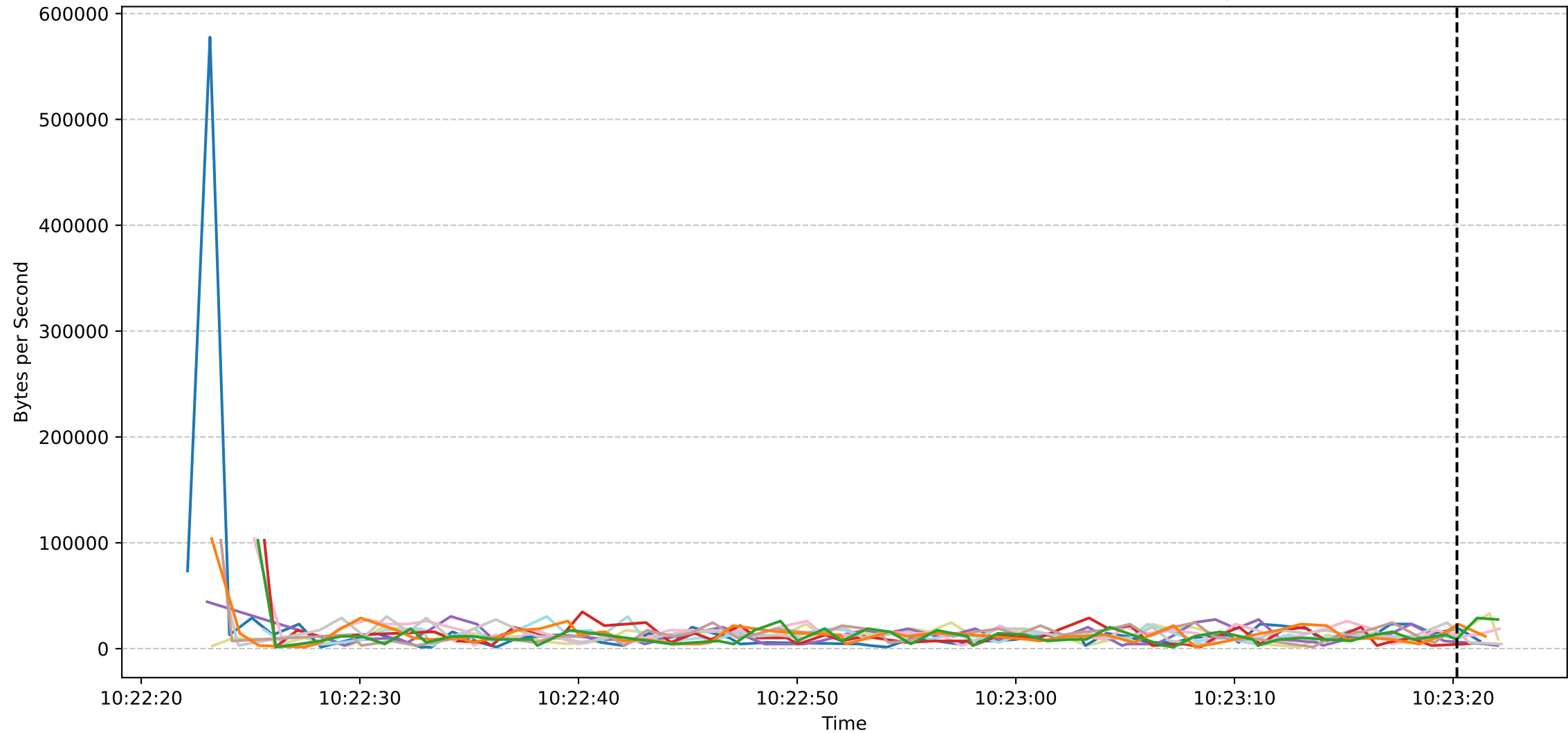
Sub Job ID: 05d0a4cf-b8f5-4a5d-8036-19f2630e47b0 - Worker Download Speeds
