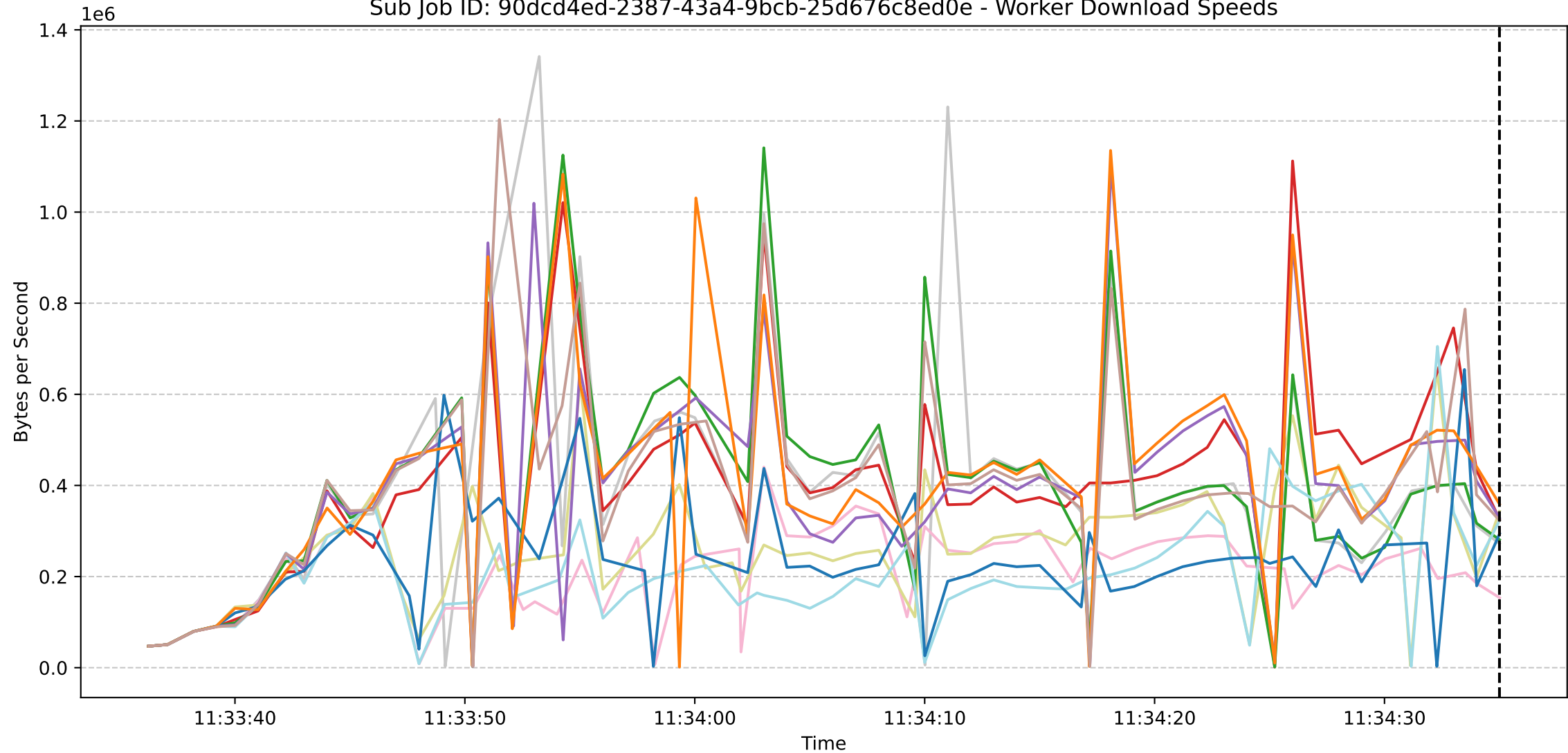
Sub Job ID: 90dcd4ed-2387-43a4-9bcb-25d676c8ed0e - Worker Download Speeds
