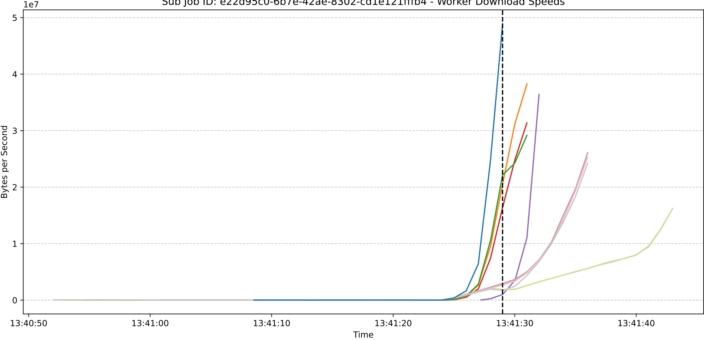
Sub Job ID: e22d95c0-6b7e-42ae-8302-cd1e121fffb4 - Worker Download Speeds
