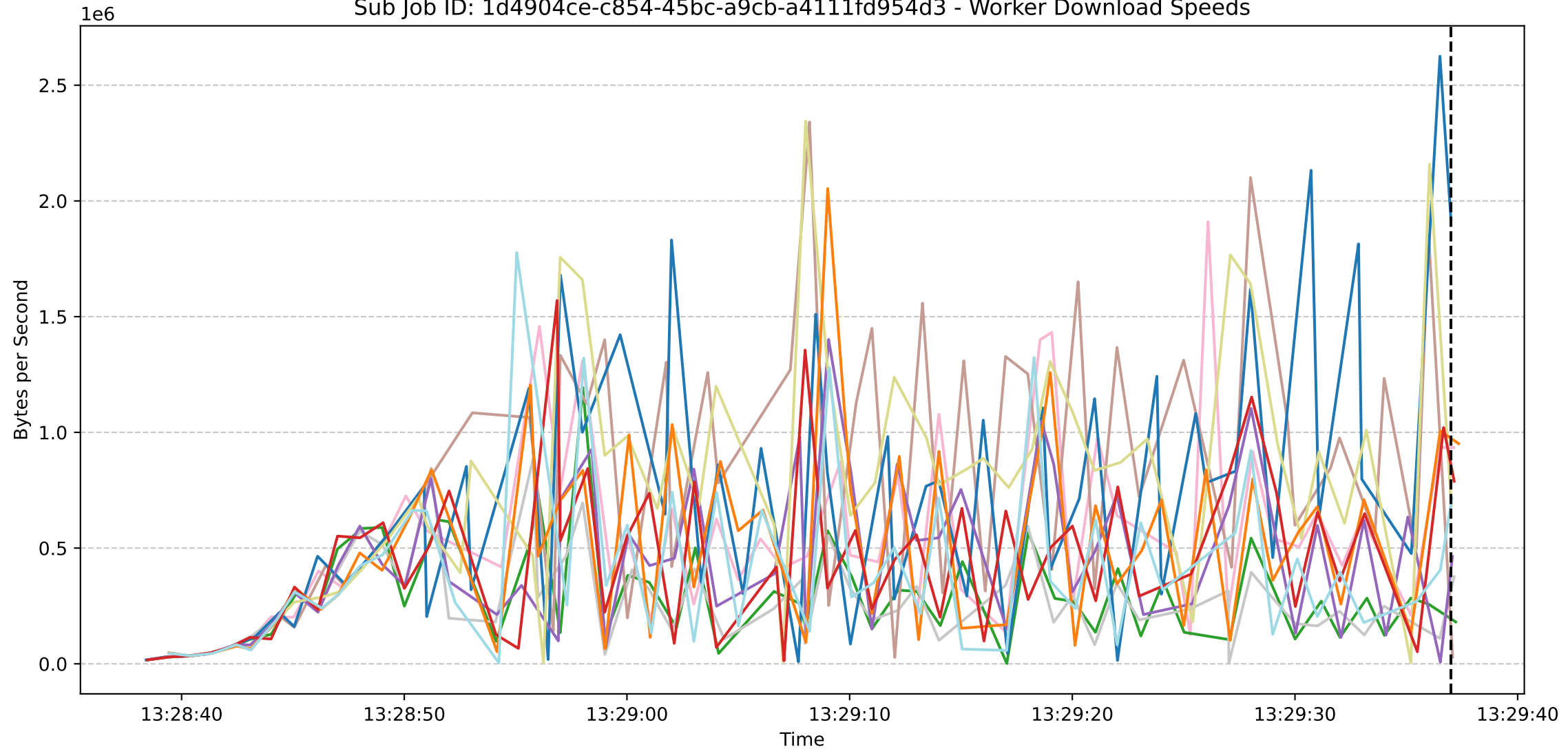
Sub Job ID: 1d4904ce-c854-45bc-a9cb-a4111fd954d3 - Worker Download Speeds
