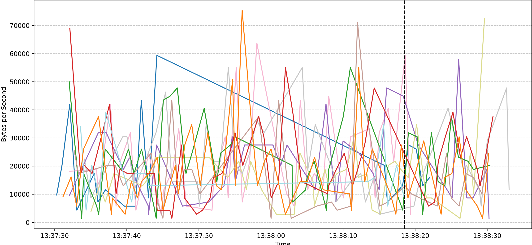
Sub Job ID: 9fc0bc38-154a-4387-b1e5-9f2143fa5815 - Worker Download Speeds
