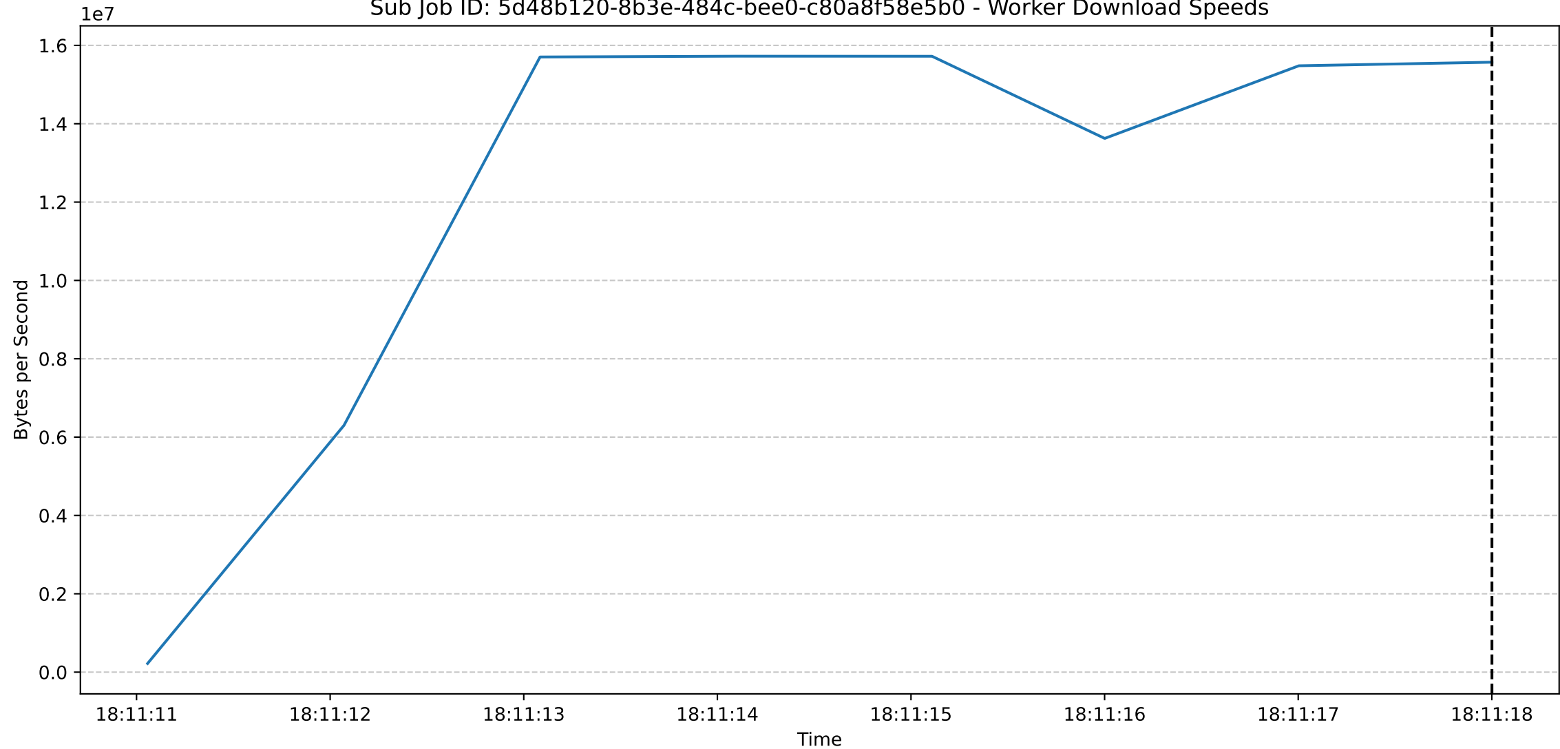
Sub Job ID: 5d48b120-8b3e-484c-bee0-c80a8f58e5b0 - Worker Download Speeds
