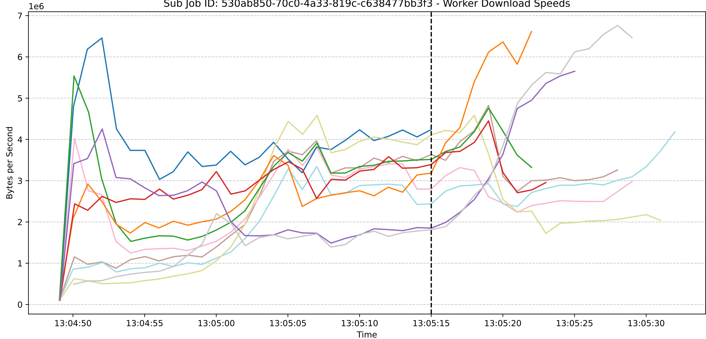
Sub Job ID: 530ab850-70c0-4a33-819c-c638477bb3f3 - Worker Download Speeds
