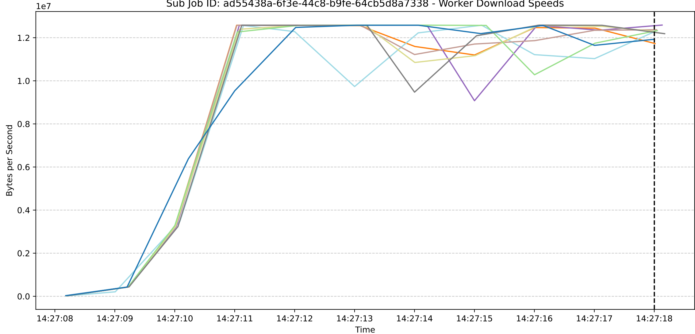
Sub Job ID: ad55438a-6f3e-44c8-b9fe-64cb5d8a7338 - Worker Download Speeds
