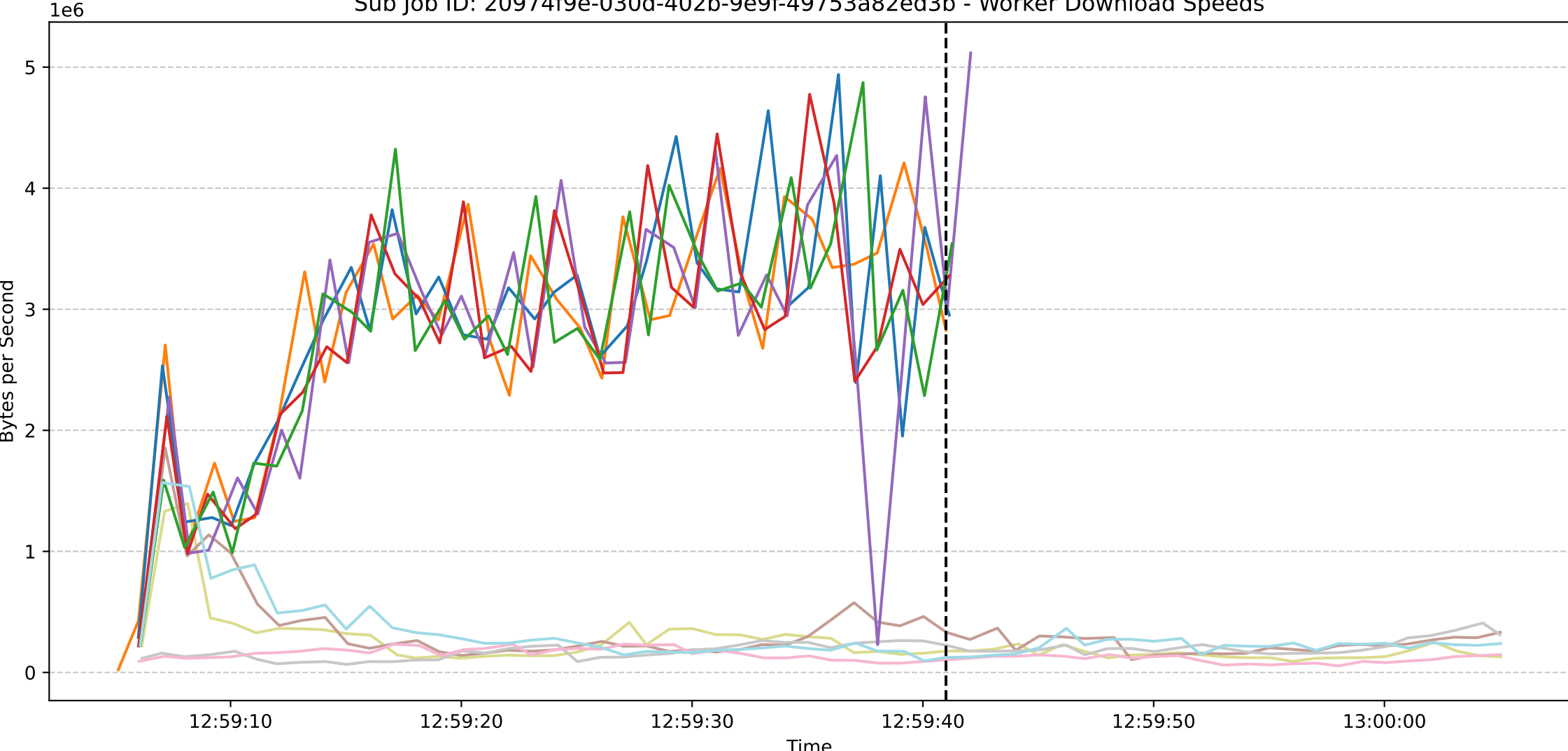
Sub Job ID: 20974f9e-030d-402b-9e9f-49753a82ed3b - Worker Download Speeds
