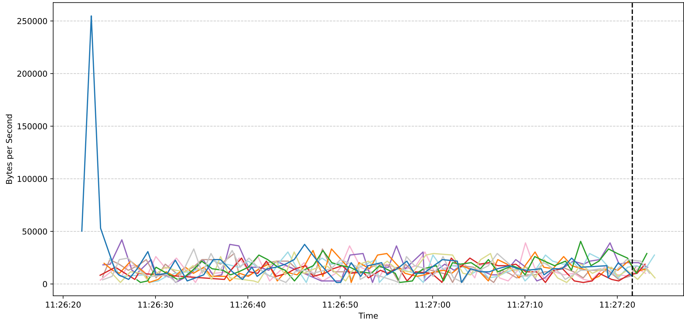
Sub Job ID: 38d29936-d9d1-4f8a-a321-87e6026797d9 - Worker Download Speeds
