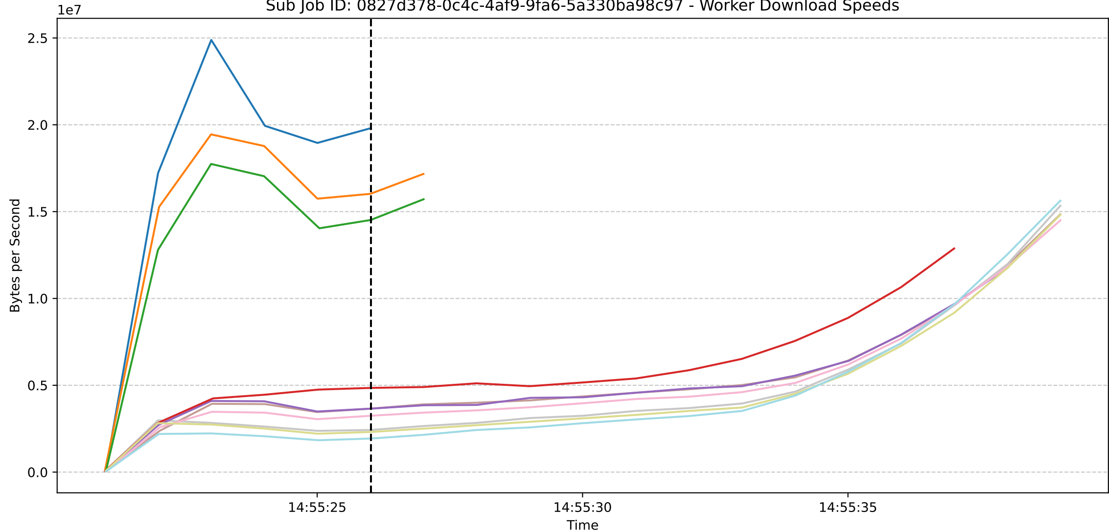
Sub Job ID: 0827d378-0c4c-4af9-9fa6-5a330ba98c97 - Worker Download Speeds
