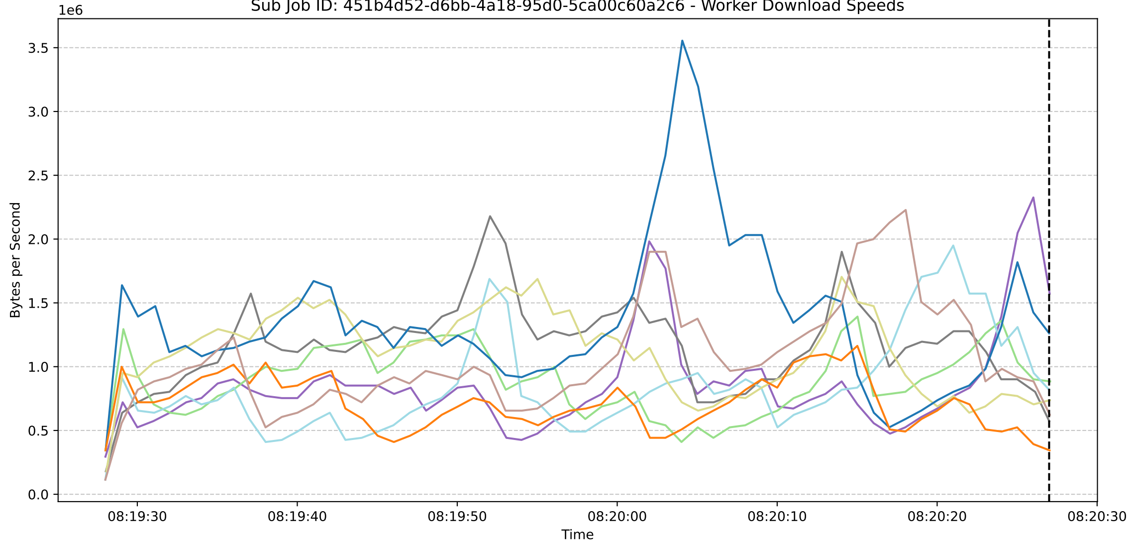
Sub Job ID: 451b4d52-d6bb-4a18-95d0-5ca00c60a2c6 - Worker Download Speeds
