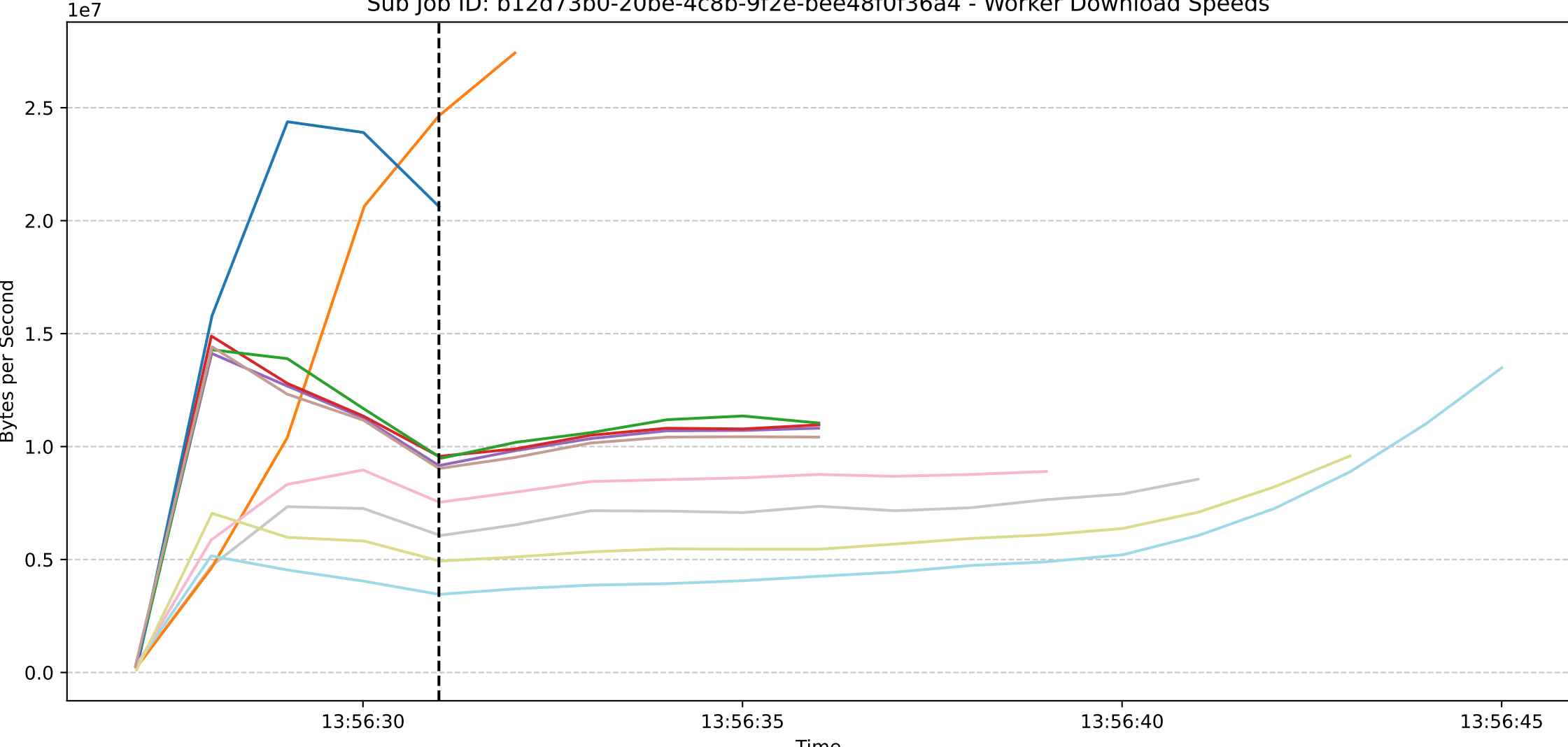
Sub Job ID: b12d73b0-20be-4c8b-9f2e-bee48f0f36a4 - Worker Download Speeds
