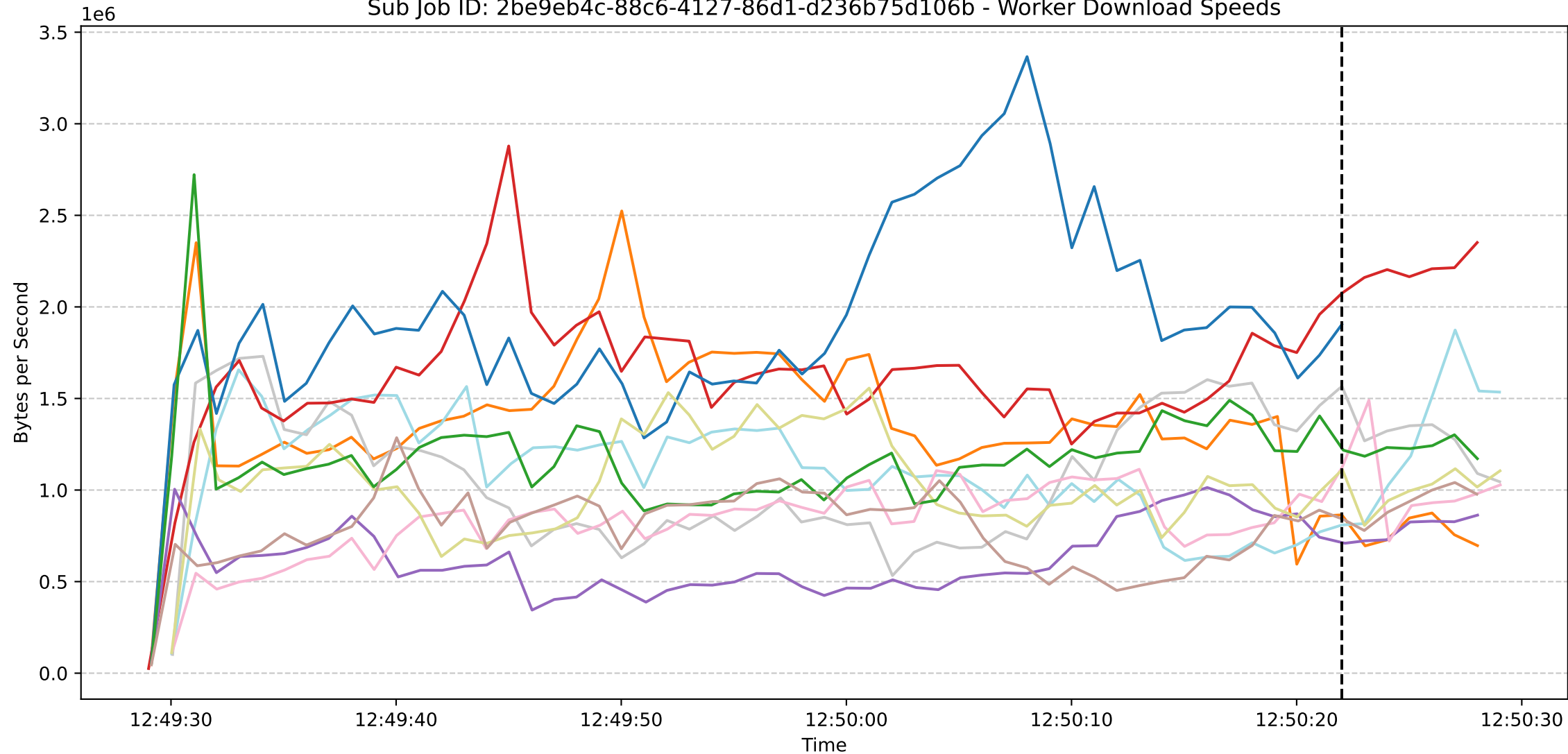
Sub Job ID: 2be9eb4c-88c6-4127-86d1-d236b75d106b - Worker Download Speeds
