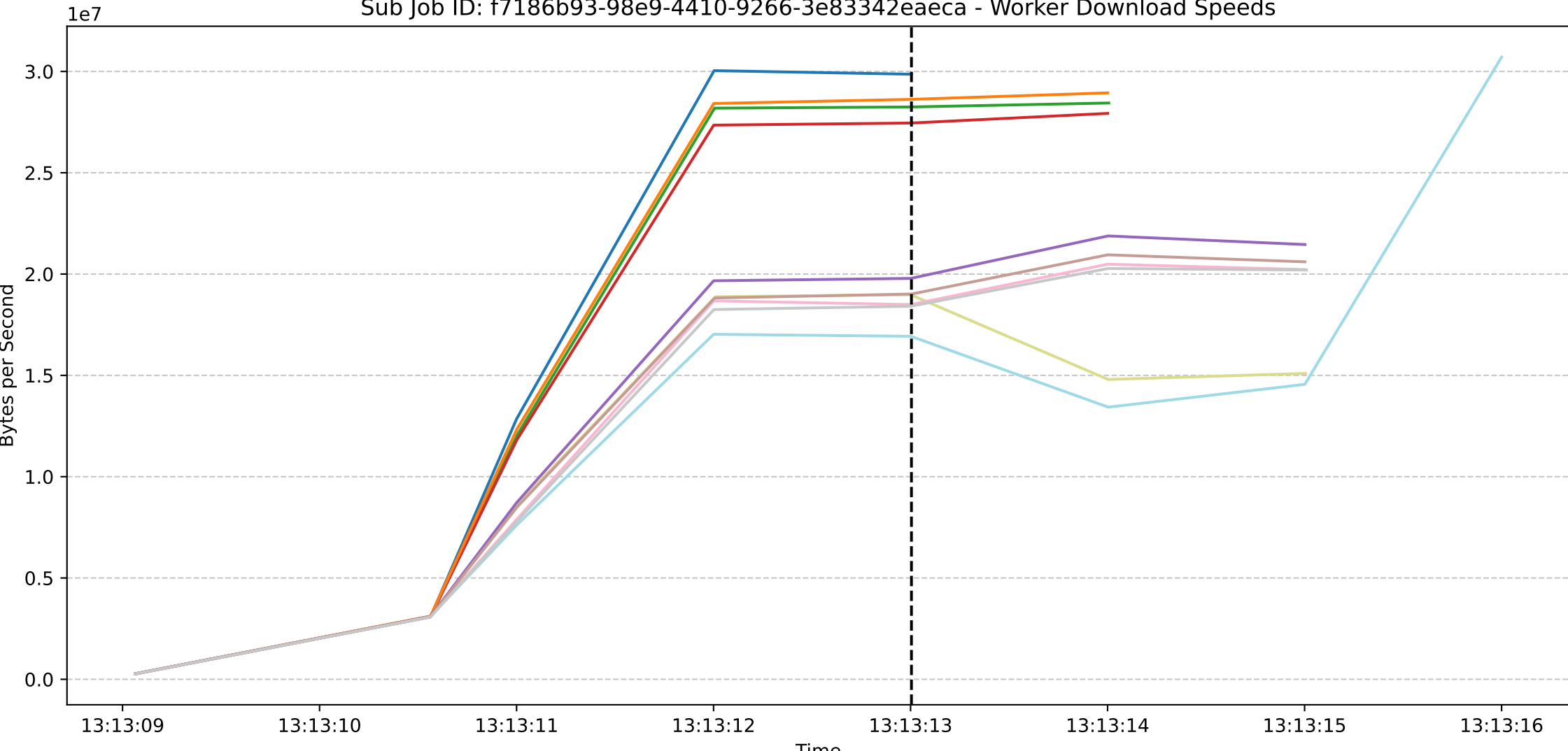
Sub Job ID: f7186b93-98e9-4410-9266-3e83342eaeca - Worker Download Speeds
