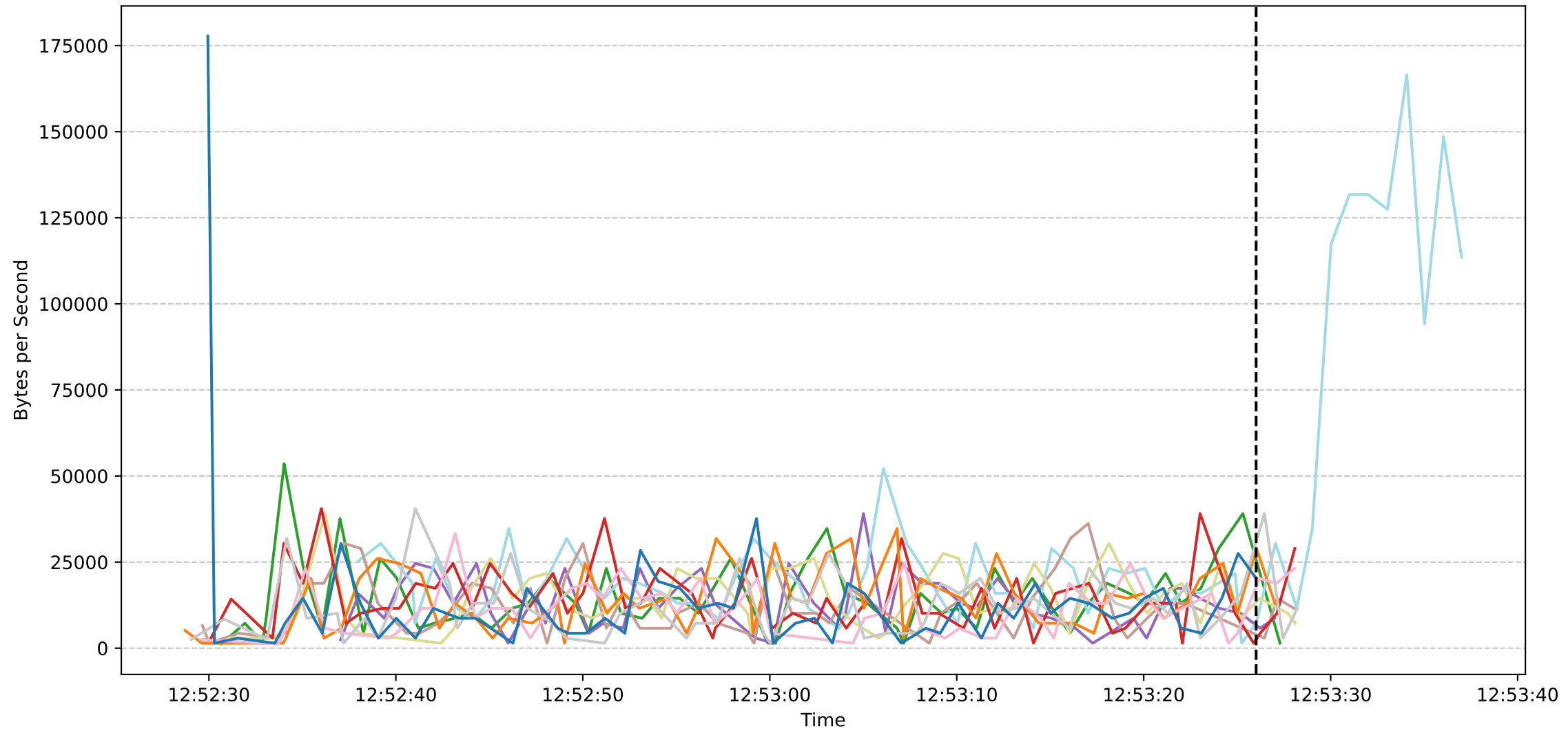
Sub Job ID: 300af3e0-149b-4b05-804c-141a221e22ad - Worker Download Speeds
