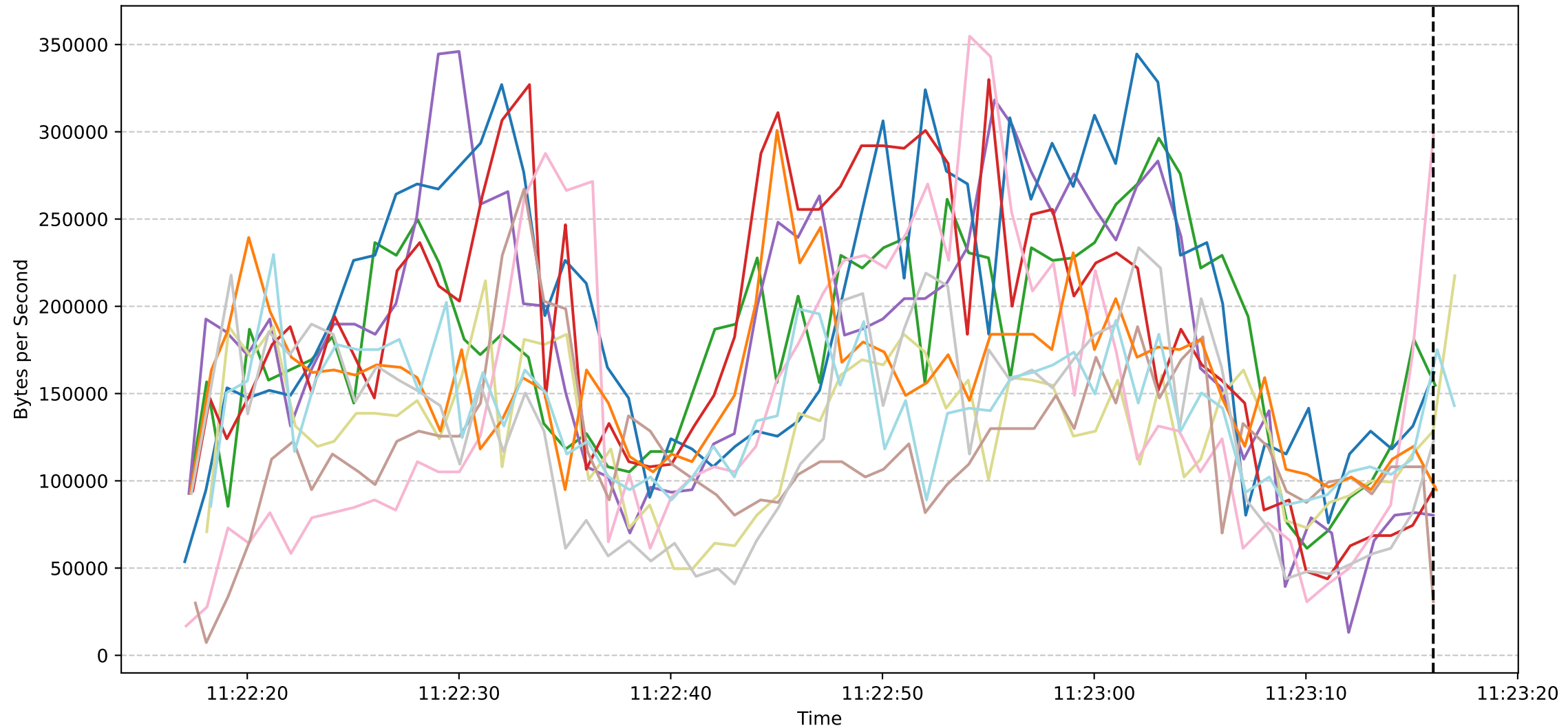
Sub Job ID: 1a50dc56-eb14-4af2-a734-92eacf473633 - Worker Download Speeds
