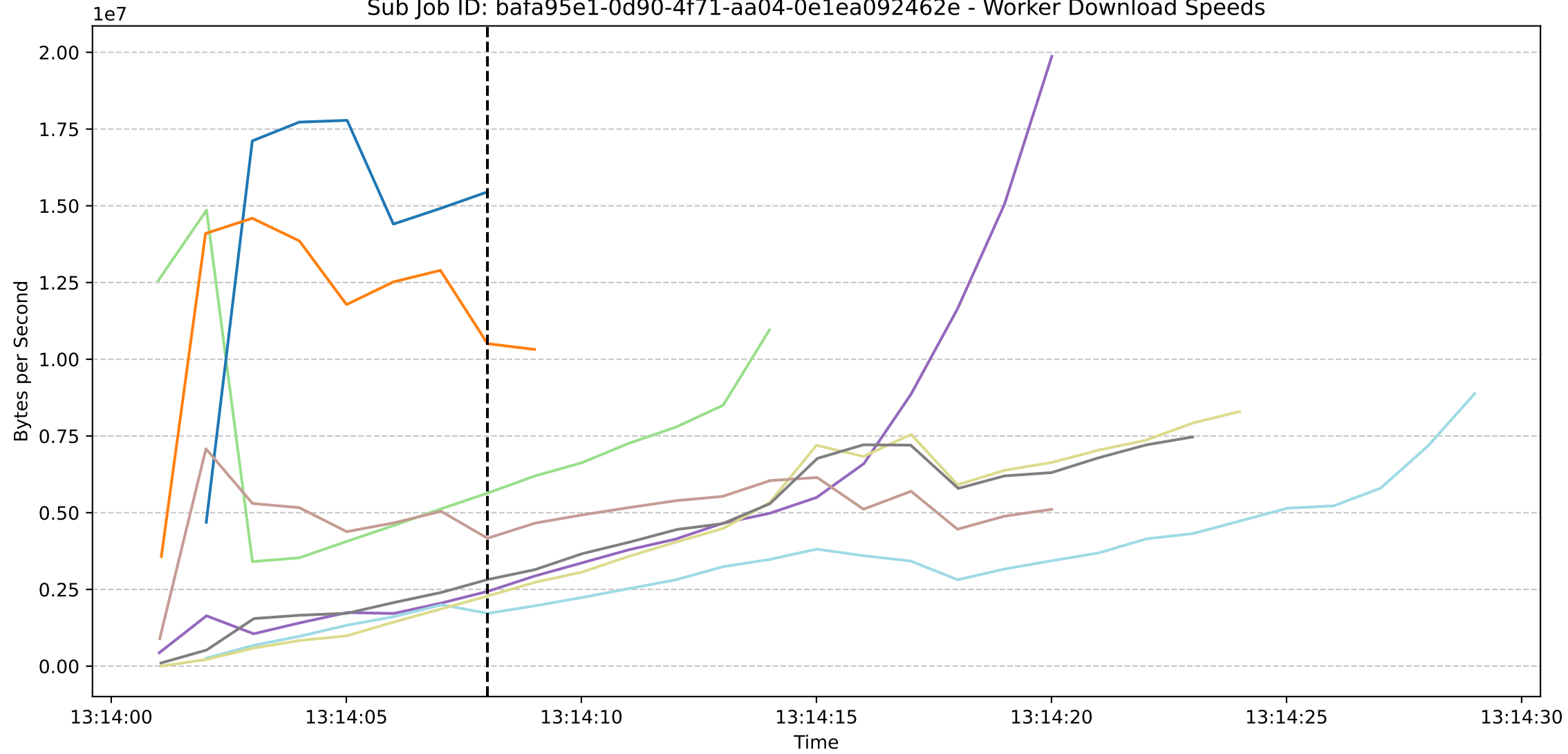
Sub Job ID: bafa95e1-0d90-4f71-aa04-0e1ea092462e - Worker Download Speeds
