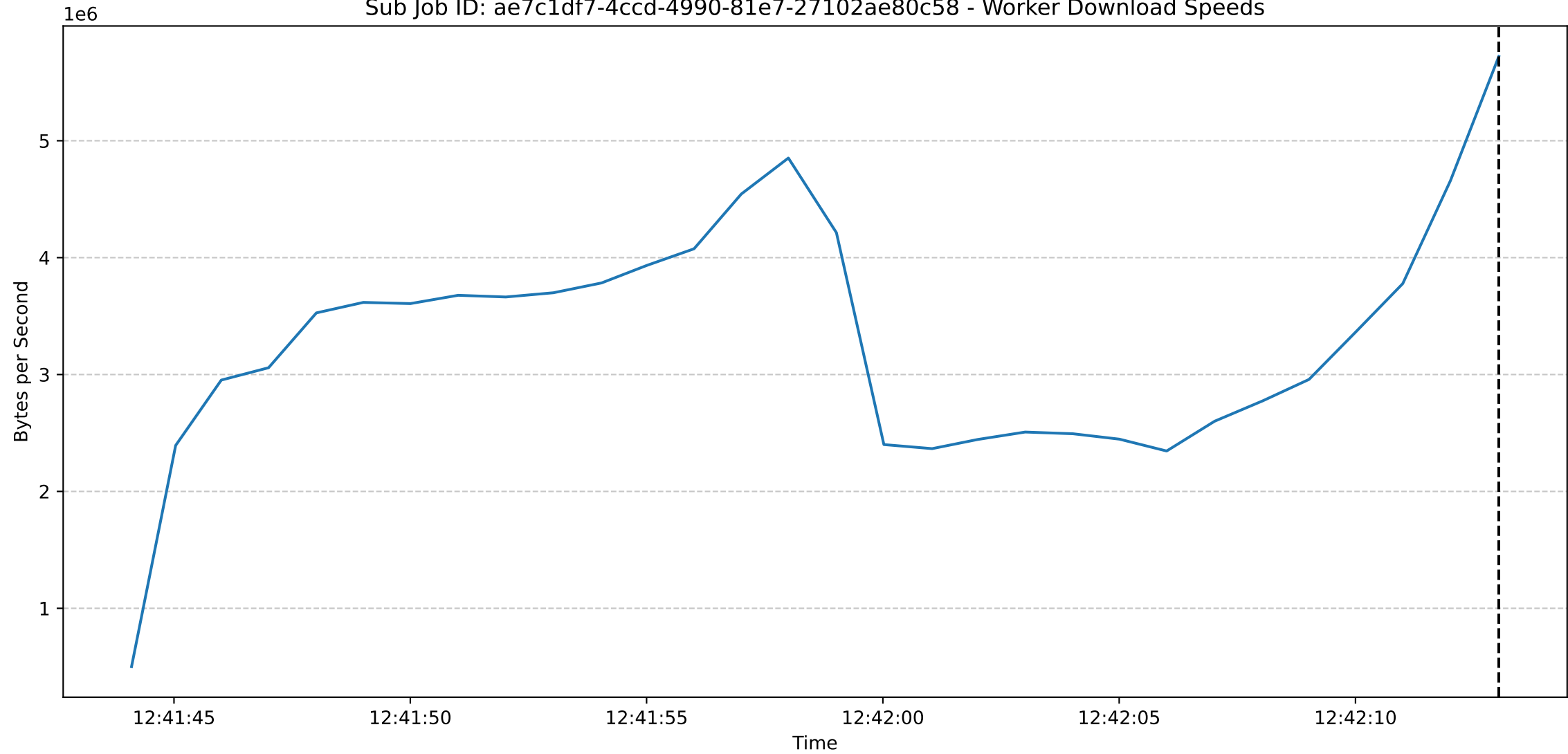
Sub Job ID: ae7c1df7-4ccd-4990-81e7-27102ae80c58 - Worker Download Speeds
