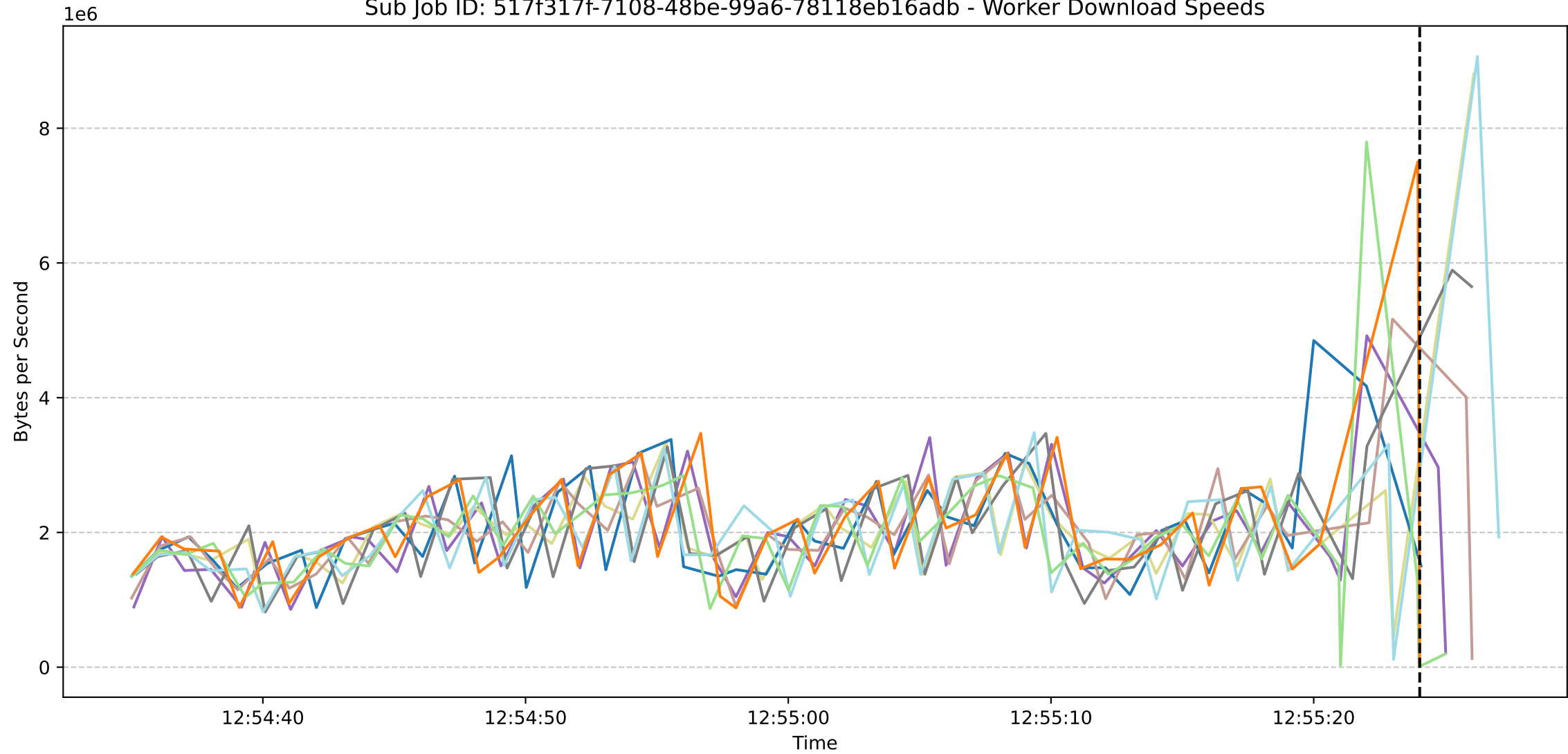
Sub Job ID: 517f317f-7108-48be-99a6-78118eb16adb - Worker Download Speeds
