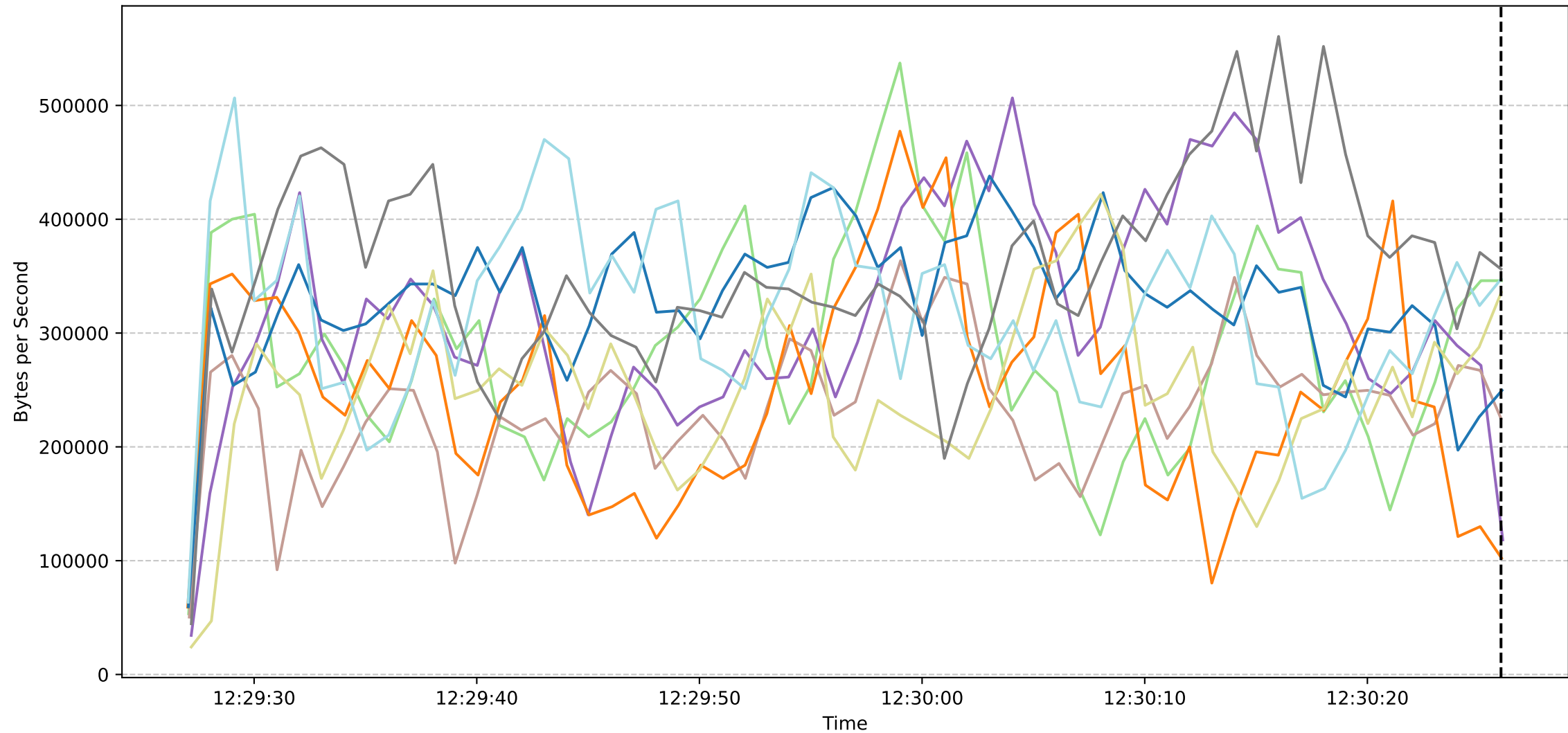
Sub Job ID: a057e966-83a9-47e6-bf0f-b84c65994c34 - Worker Download Speeds
