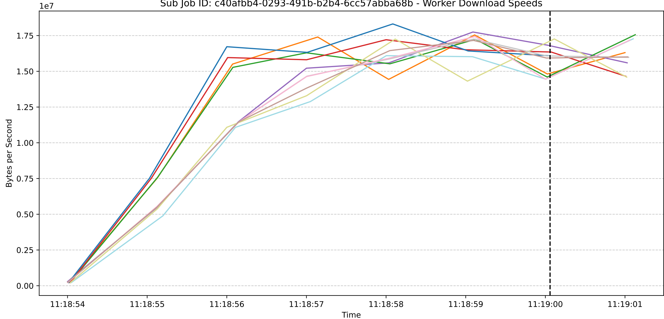
Sub Job ID: c40afbb4-0293-491b-b2b4-6cc57abba68b - Worker Download Speeds
