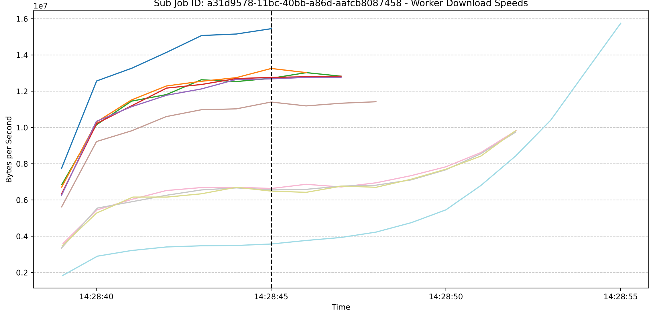
Sub Job ID: a31d9578-11bc-40bb-a86d-aafcb8087458 - Worker Download Speeds
