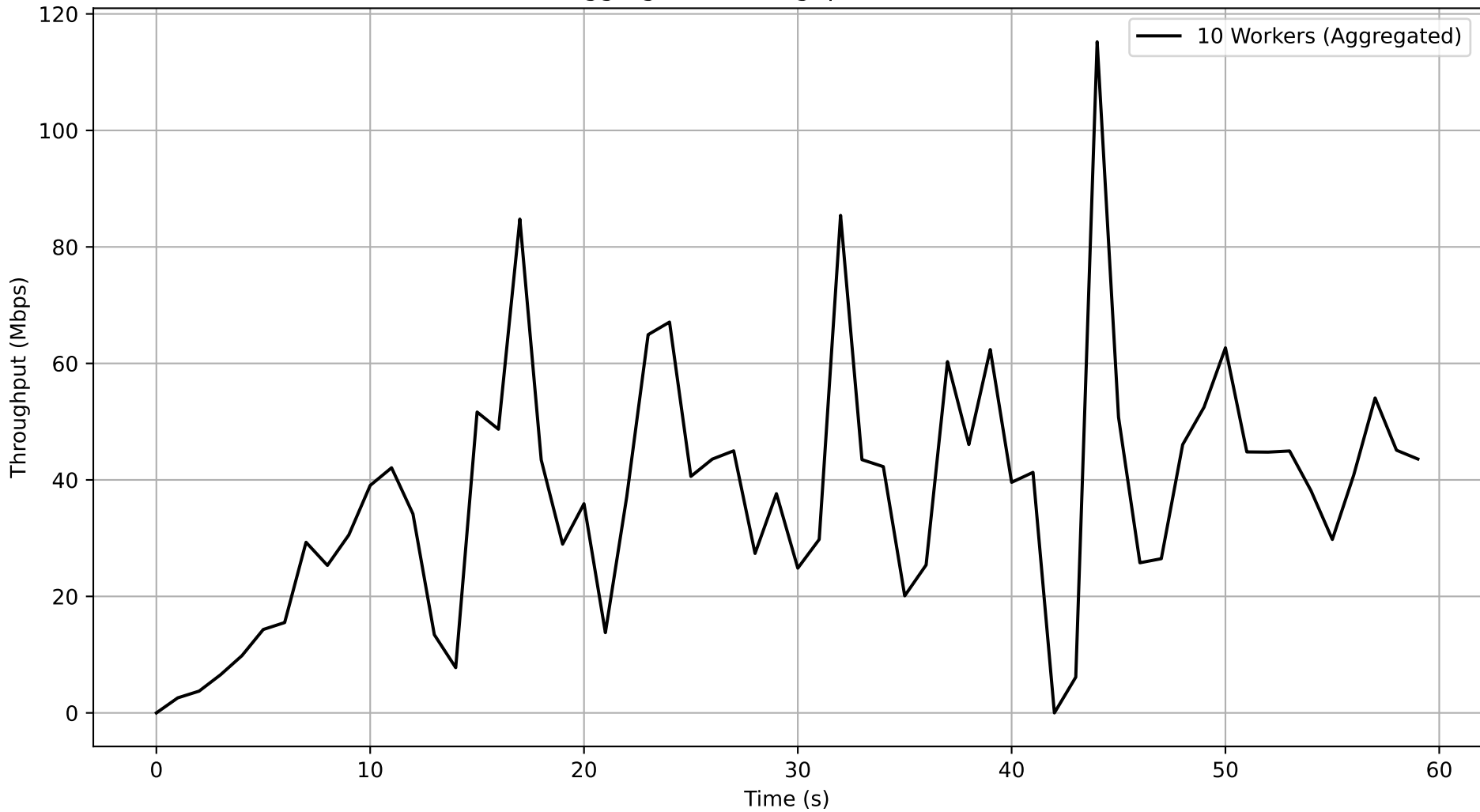
Job db252037-a59c-43f1-adb5-538f5e24fbfd - Subjob 59da326f-433b-4f68-943e-7e923a27af11 Aggregated Throughput Over Time
