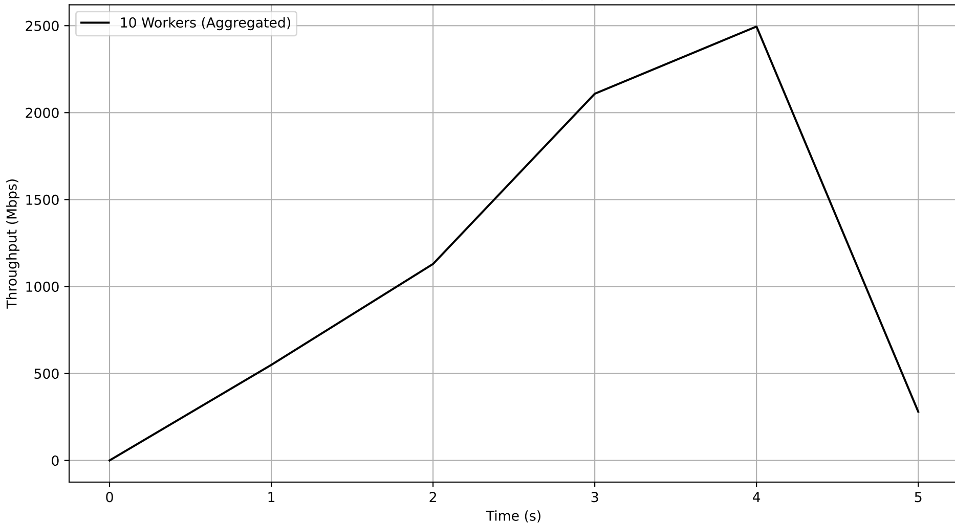
Job dc100bbf-b6bc-436d-90a4-8d0921e97afb - Subjob 1bfbdcc8-25ec-4989-a764-172d5792eb49 Aggregated Throughput Over Time
