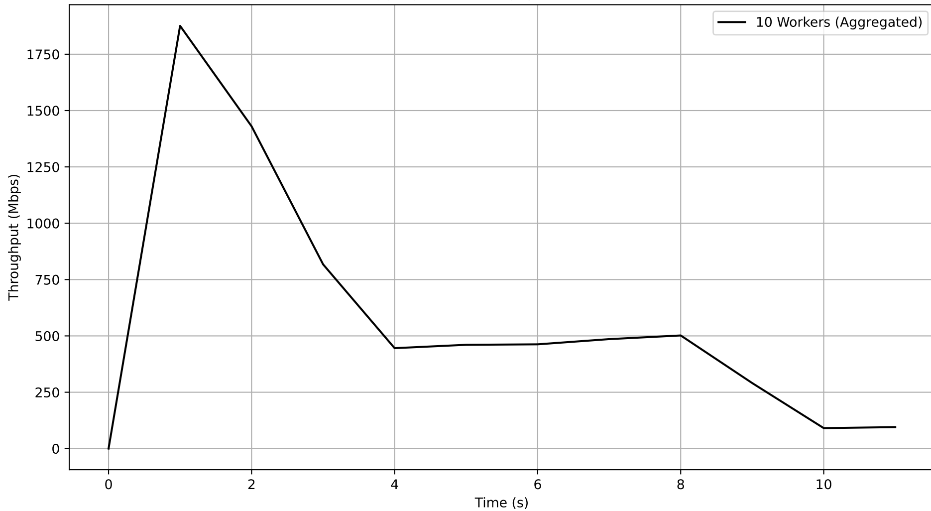
Job 50e3de30-efbe-4d79-8da6-13a09c1a83a7 - Subjob 57d0cb1e-cda7-4851-8a62-b7662ec2002e Aggregated Throughput Over Time
