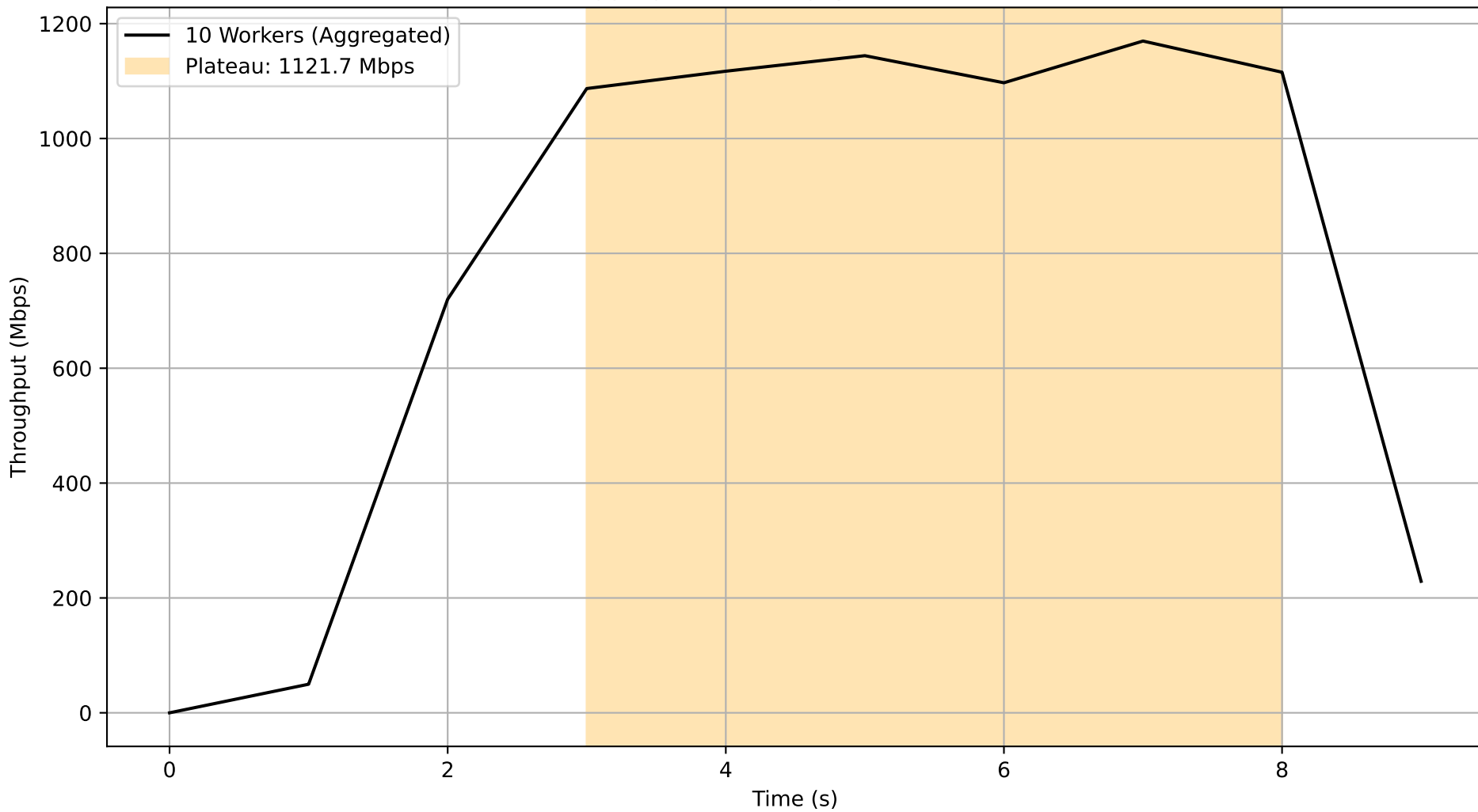
Job 7eb3d672-9c08-4a15-97ec-49b5dbfc2946 - Subjob 780b06a6-6c35-45c9-b42a-fdb449a029be Aggregated Throughput Over Time
