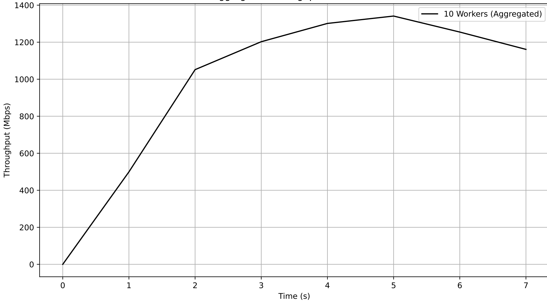
Job 0c66d895-471b-4059-a1ff-9a7926ed099e - Subjob c40afbb4-0293-491b-b2b4-6cc57abba68b Aggregated Throughput Over Time
