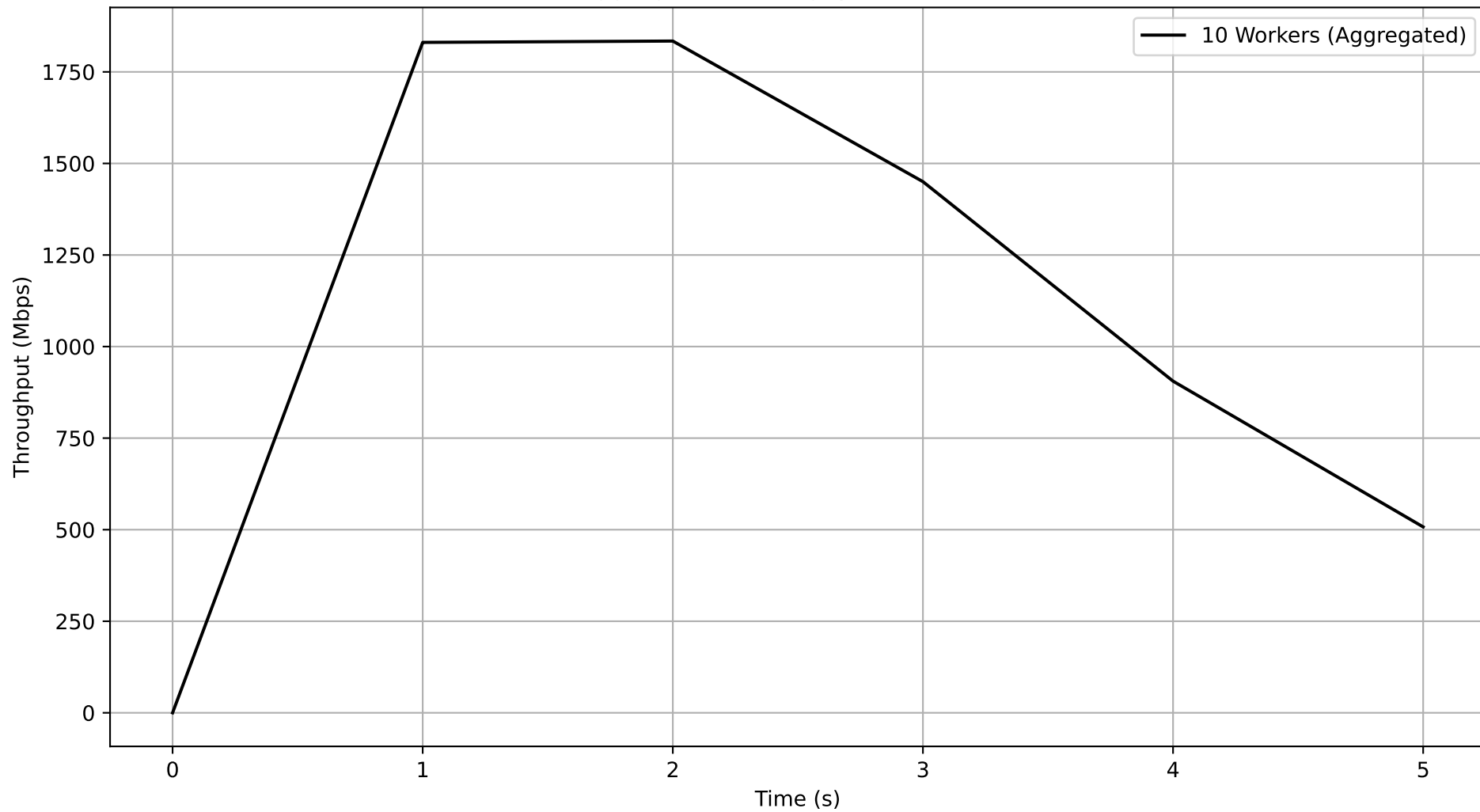
Job e25cad75-6db5-4d61-8217-293312c01378 - Subjob 9ed2a16d-c4d3-409c-b7b1-8679a5b01a3e Aggregated Throughput Over Time
