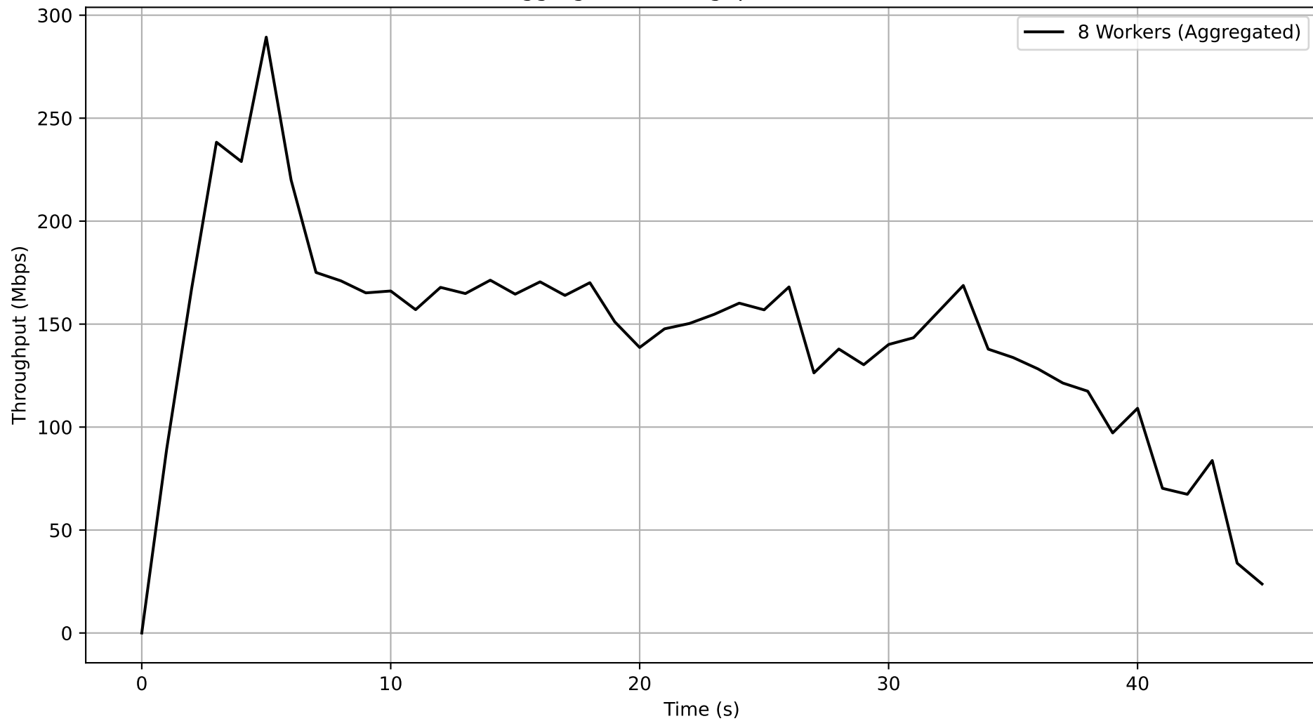
Job 86873df7-323e-40b9-a8b5-f13e825c4437 - Subjob 205c37a1-b5f3-4cce-8a0a-7f4d30dc7996 Aggregated Throughput Over Time
