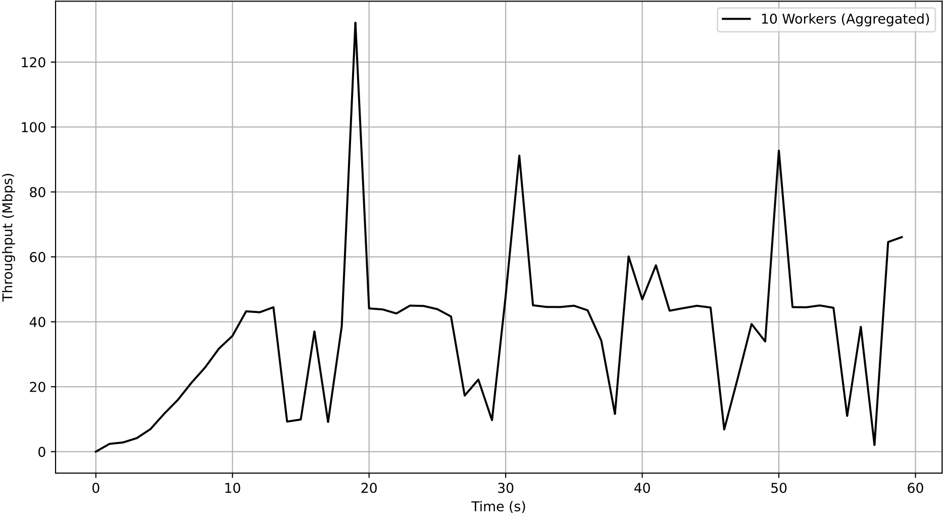
Job 94926e15-2b50-427a-b2ba-207b88bc8787 - Subjob 5557ac57-e218-4fe4-ab88-d2427a8c1e36 Aggregated Throughput Over Time
