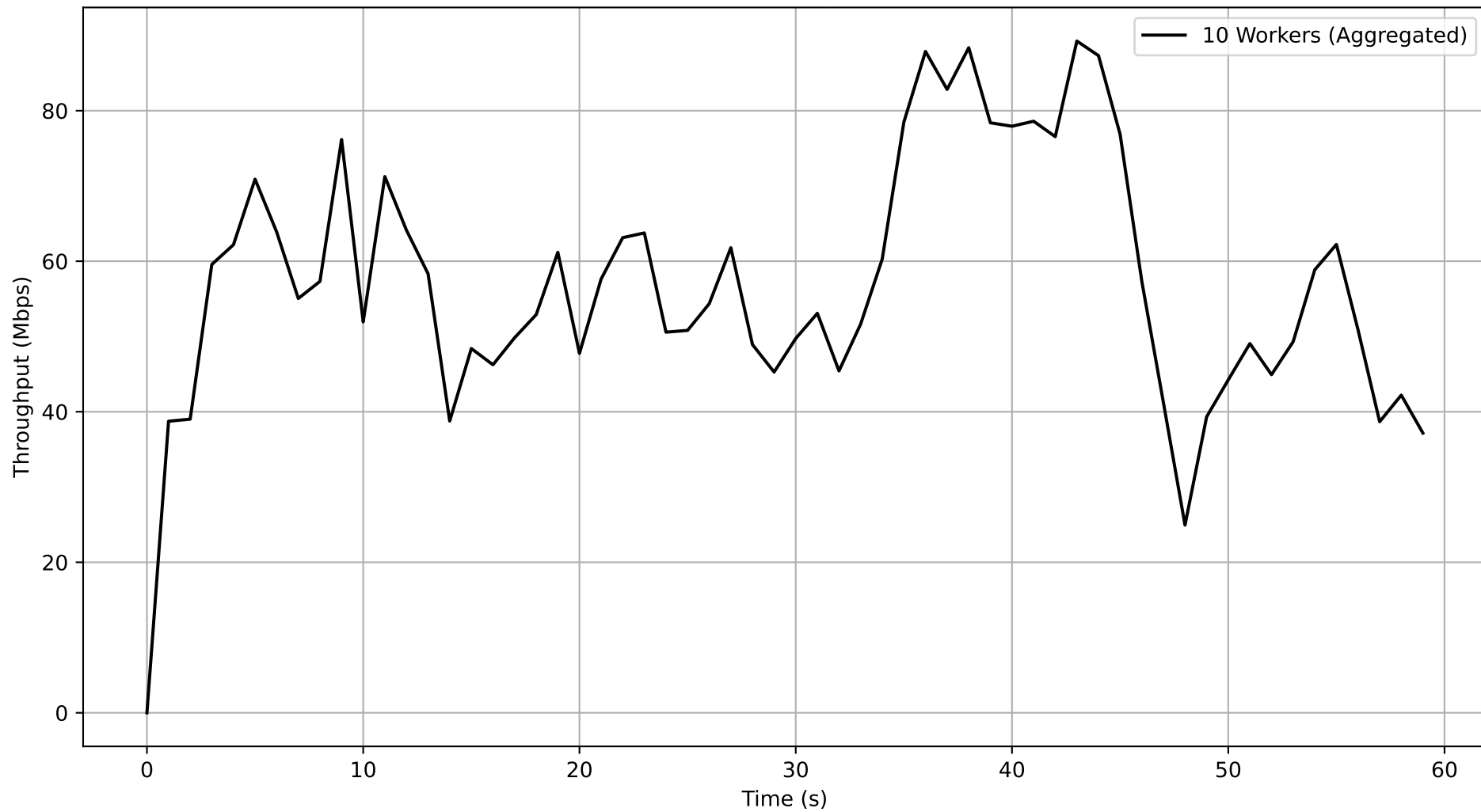
Job c2ff83c6-263f-4bbf-a8f3-af5164ad62af - Subjob c6a1d43f-c2ec-499e-b2cb-ec8b8f8ddd36 Aggregated Throughput Over Time
