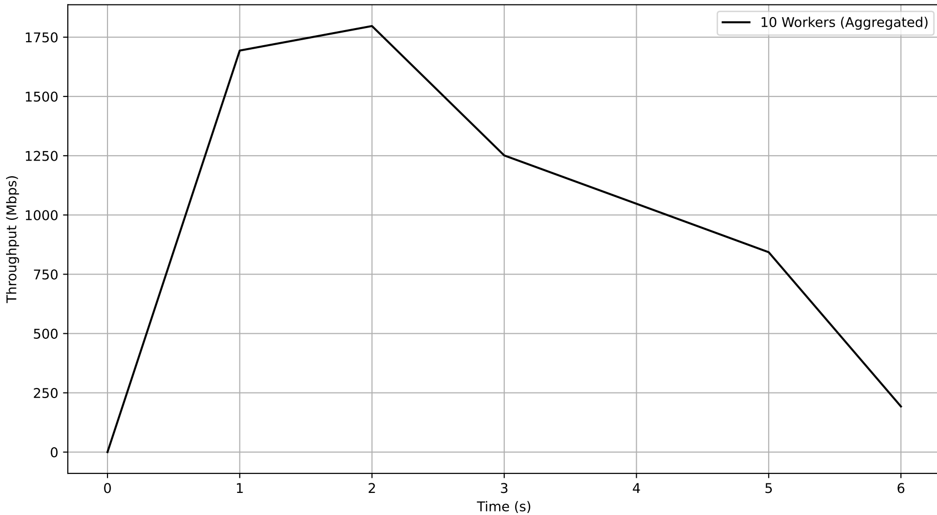
Job 764df5aa-ae55-46db-b185-6d43be3bd179 - Subjob f0dc35a3-4e0d-4b5f-91a9-46388d113690 Aggregated Throughput Over Time
