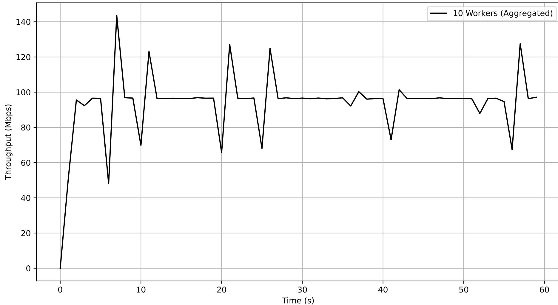
Job f84dd79d-0bfb-4c3b-9d43-a8a7dce26fa7 - Subjob 7bfa9347-e2a1-4a75-b067-6399346ffd21 Aggregated Throughput Over Time
