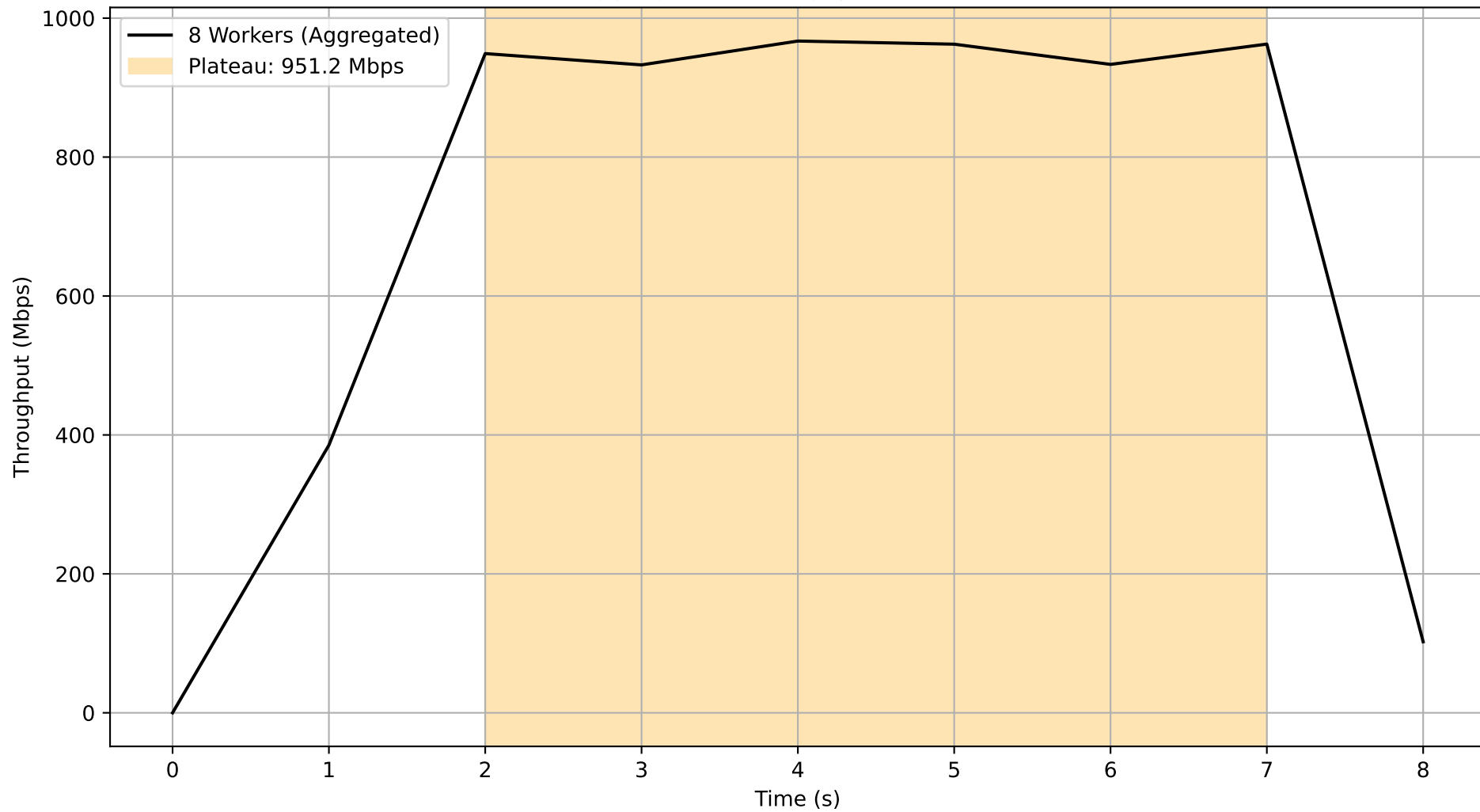
Job 61828f8a-b2fc-4800-b817-544c6b0e8d55 - Subjob b3df2c8e-7c7e-4920-ad02-fbc32d15a318 Aggregated Throughput Over Time
