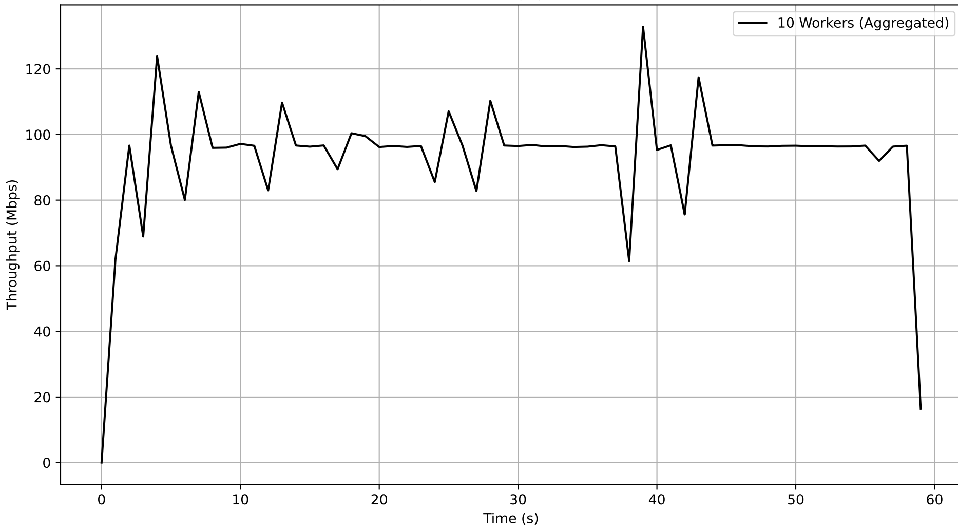
Job f84dd79d-0bfb-4c3b-9d43-a8a7dce26fa7 - Subjob a40ae954-9fb9-436c-974e-a370148900ff Aggregated Throughput Over Time
