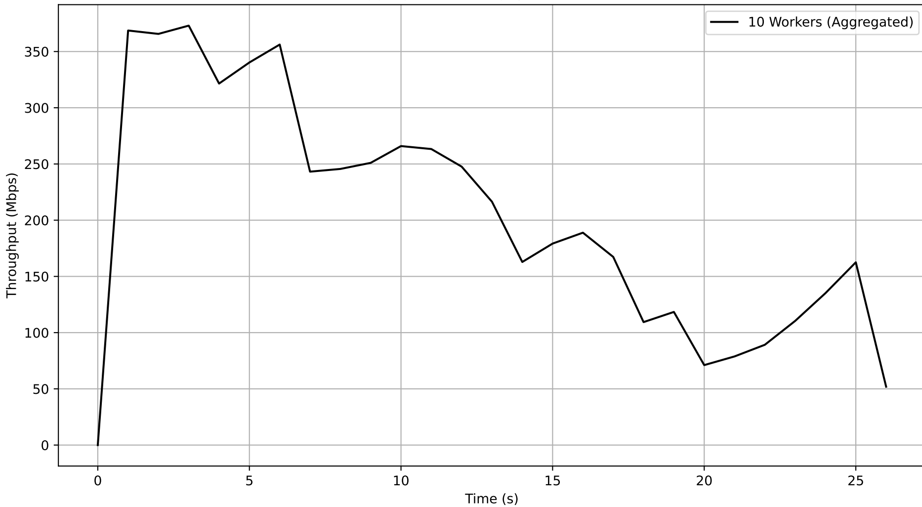
Job 408fc2c0-a8eb-4503-9ee5-ccefb6896cad - Subjob 90b9640b-e12c-41a1-978e-d2f488bf82a3 Aggregated Throughput Over Time
