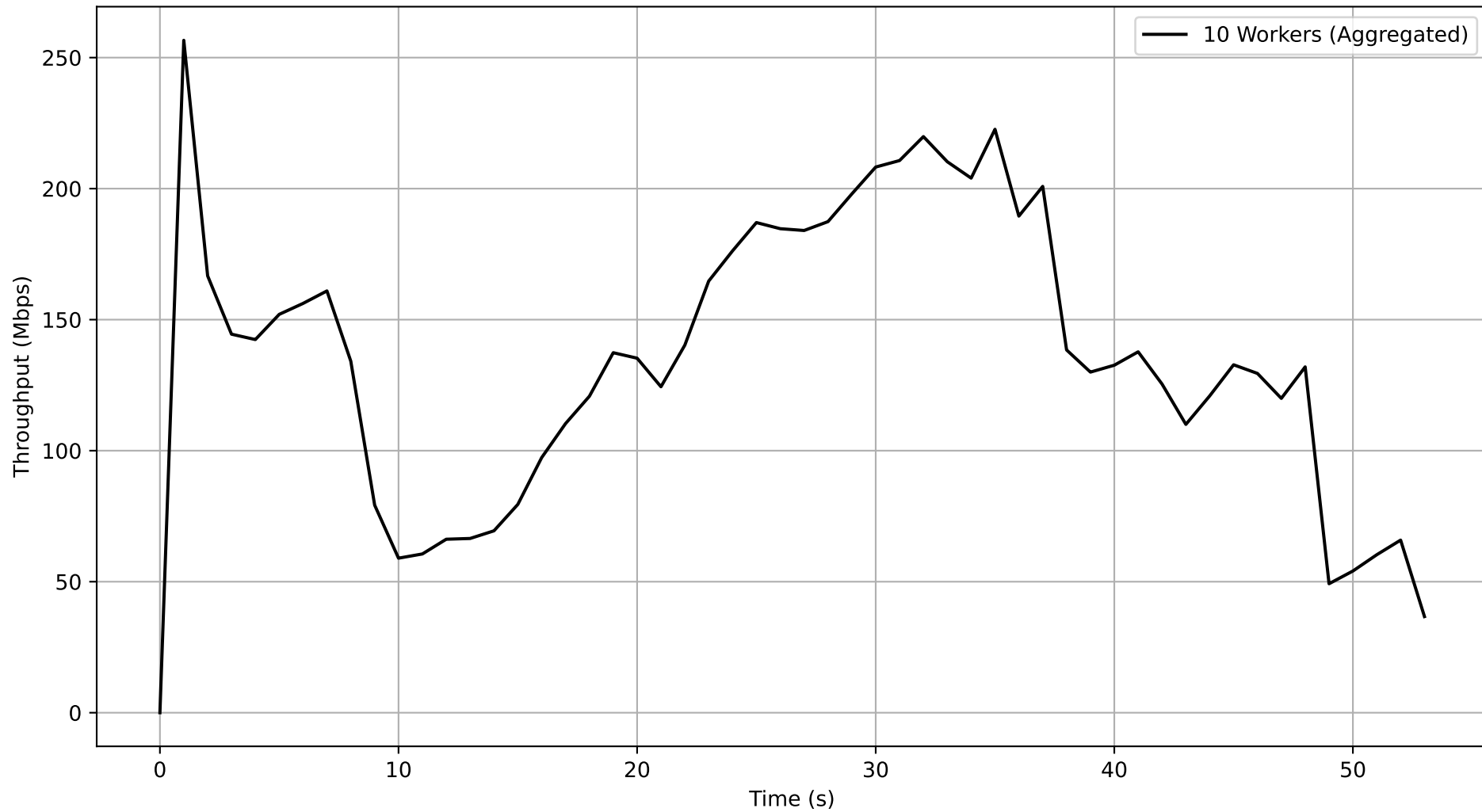
Job e9f94805-e0ba-430d-ab6d-eb022ce9e6d5 - Subjob 9b6b74aa-de3c-46ea-a42c-df737ab824ae Aggregated Throughput Over Time
