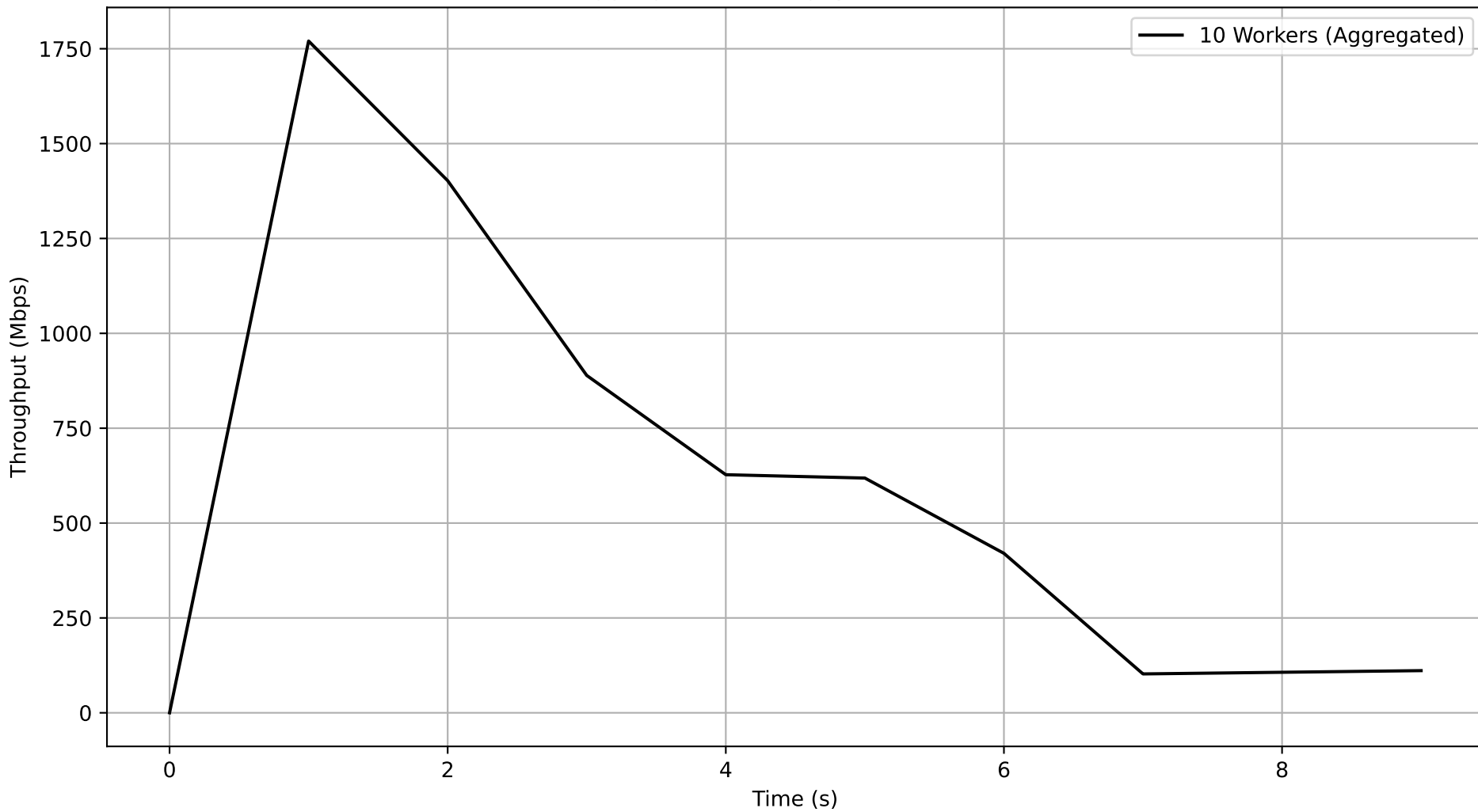
Job 56bba3ef-1420-4874-9f21-c624d27a7066 - Subjob d5fab82d-4423-45e6-bdba-aea92cbf7832 Aggregated Throughput Over Time
