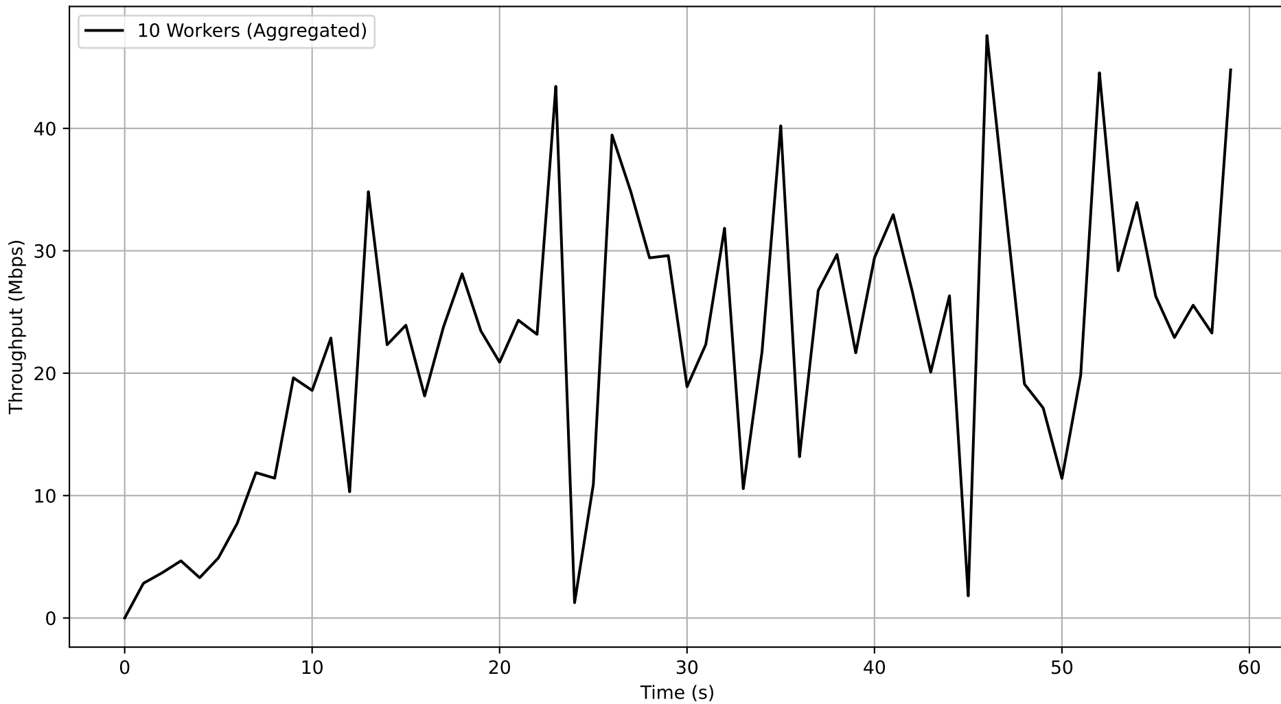
Job bd7c0ffe-0168-40d2-b8c2-fc5bb47063b6 - Subjob f956fe34-1c6d-49b8-add7-ad96dbbbc6704 Aggregated Throughput Over Time
