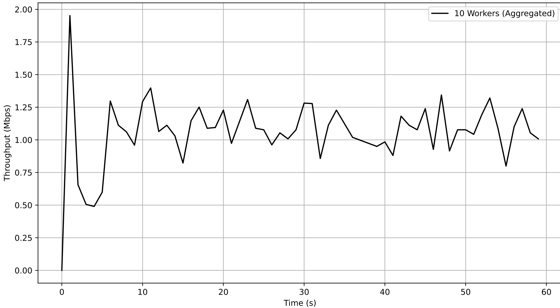
Job 0995ff58-e2f1-4758-856a-199a1130cc48 - Subjob 750378f3-3e06-485d-8a2c-8fe16a9f1f84 Aggregated Throughput Over Time
