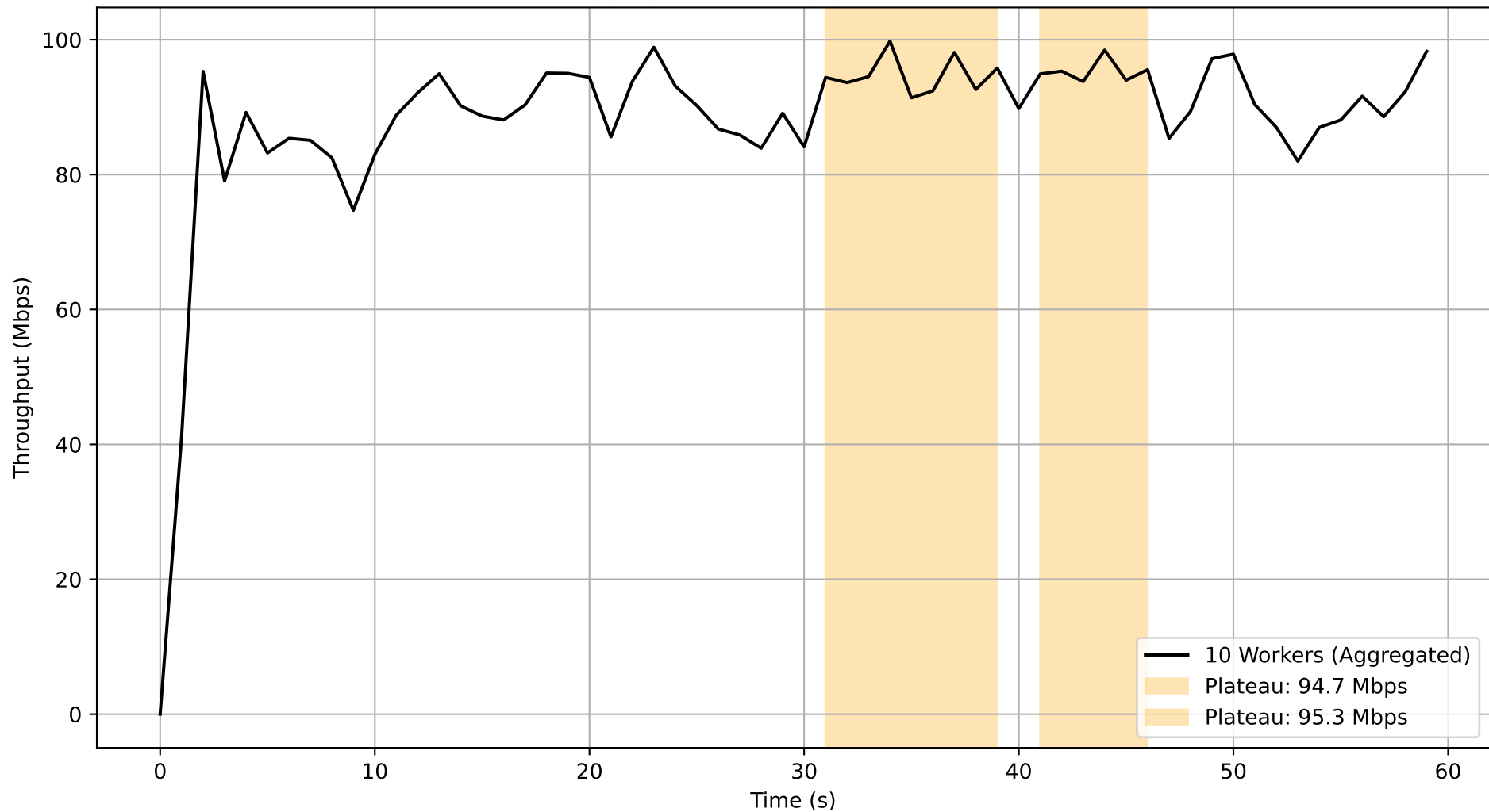
Job 11603013-d76a-4ee8-a557-3531e27b0df1 - Subjob 18ed96cd-946f-4f44-b0b1-161ca3398a12 Aggregated Throughput Over Time
