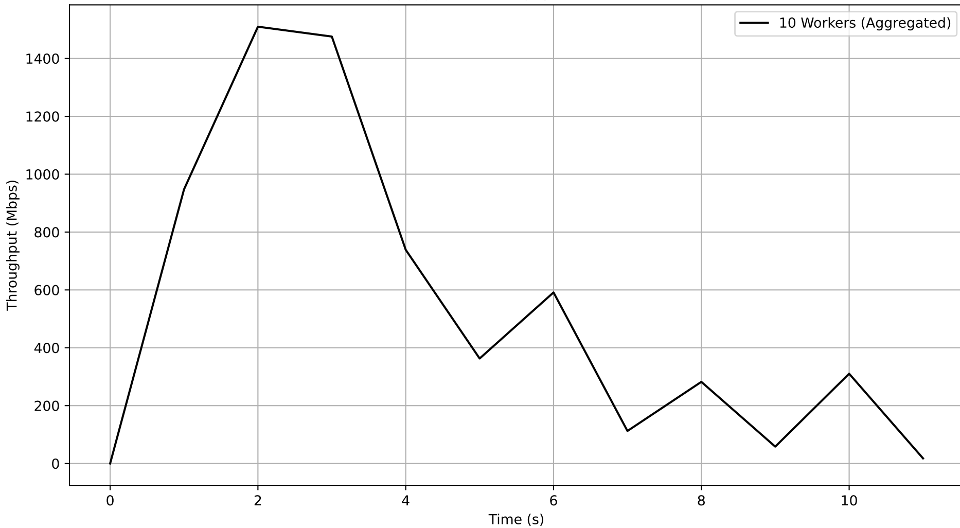
Job ee20e442-b38b-4ef6-8646-b2a40ab1ca16 - Subjob fe870dd3-4fa7-4553-8233-5055ddd2d242 Aggregated Throughput Over Time
