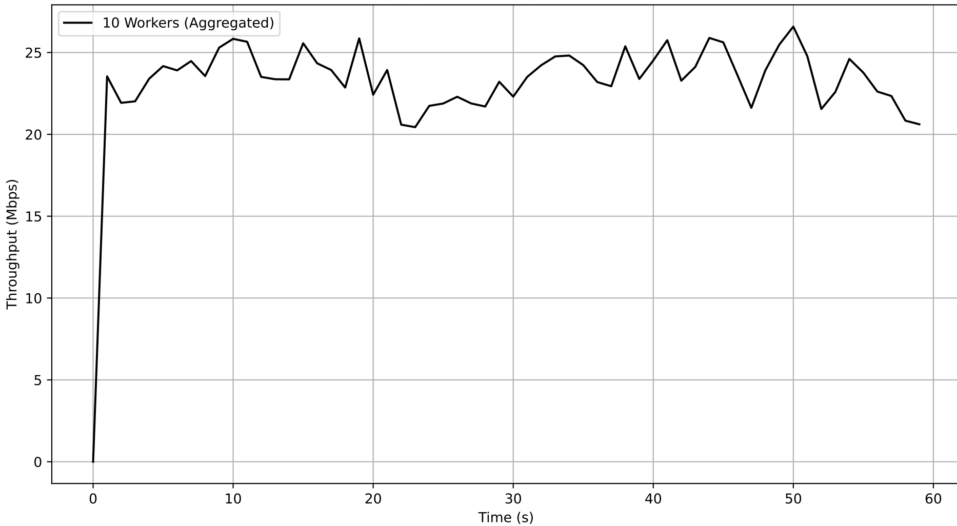
Job 69acafca-47c2-4e59-a191-d8528d4f1e2d - Subjob e547b5a3-63ef-4ae0-a2a0-939feed488be Aggregated Throughput Over Time
