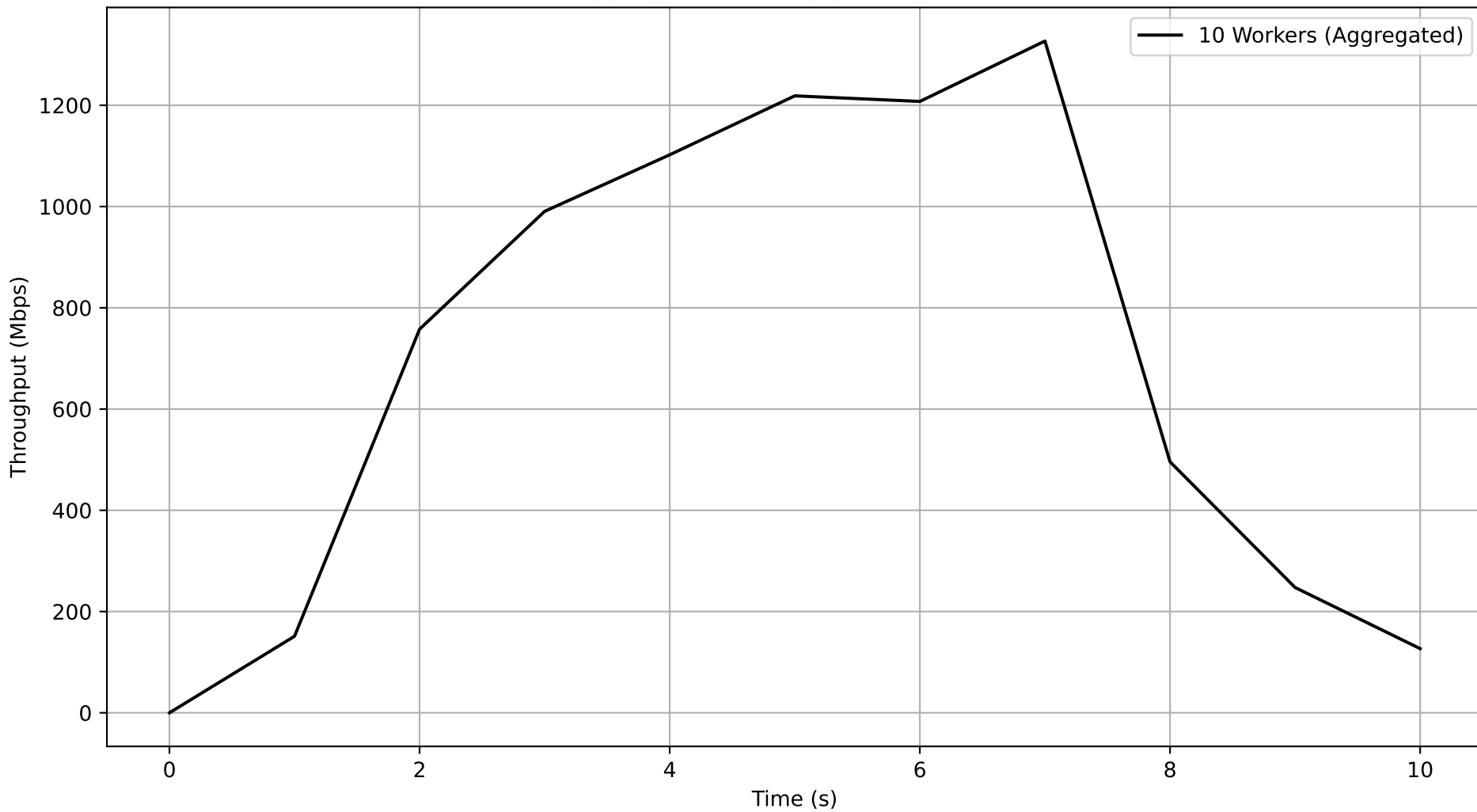
Job dc4872b5-7c9d-40f5-8511-b55c6f98475e - Subjob db123cc5-2452-4184-8904-dacb535c397f Aggregated Throughput Over Time
