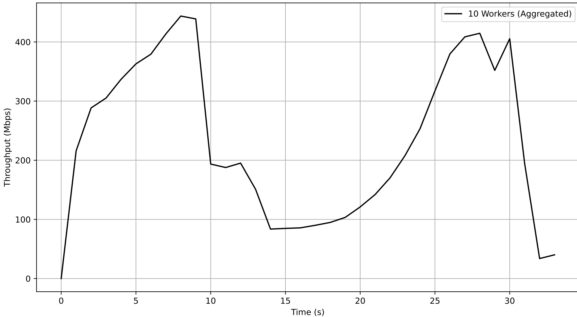
Job 02d466c5-ba4f-4bed-8651-7efbbbed94d54 - Subjob 8ef4a069-c736-447d-bf20-d4f1dcb380fd Aggregated Throughput Over Time
