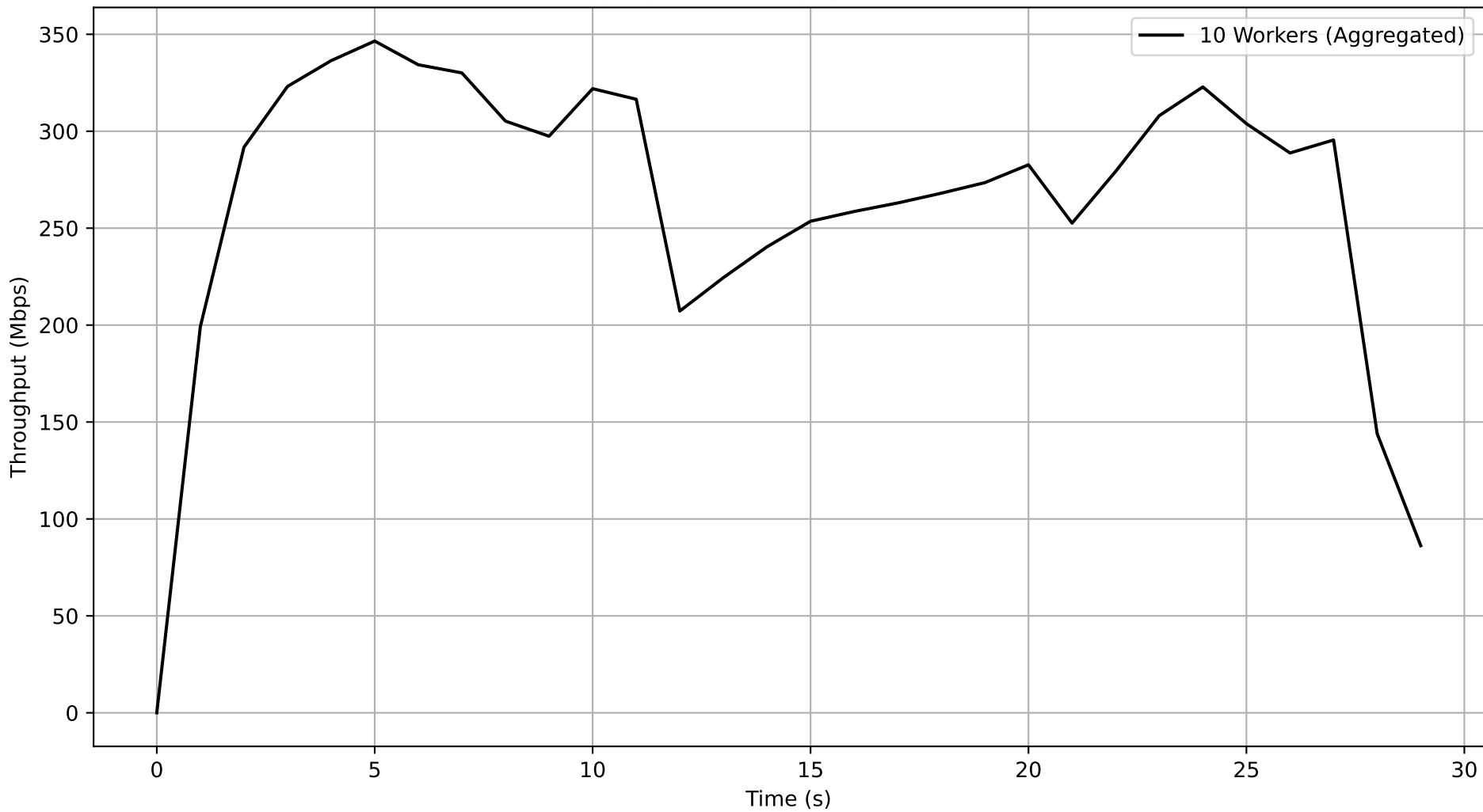
Job ad3b74ec-c767-4b8c-94d6-f07cf3742c43 - Subjob eb602615-2fa2-46a6-8f2b-66cb2b8f1fb2 Aggregated Throughput Over Time
