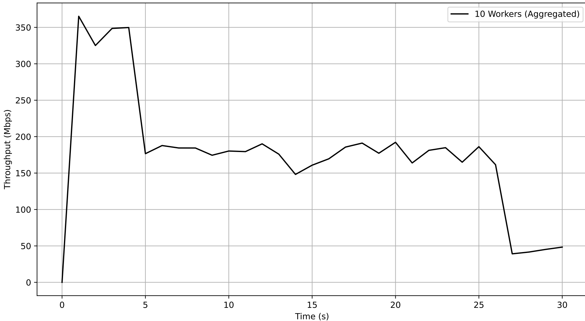
Job ae51b993-7de7-4333-8b0c-b304aa2e14eb - Subjob 84b03ce9-eb8e-4041-9e9e-d98b72757f20 Aggregated Throughput Over Time
