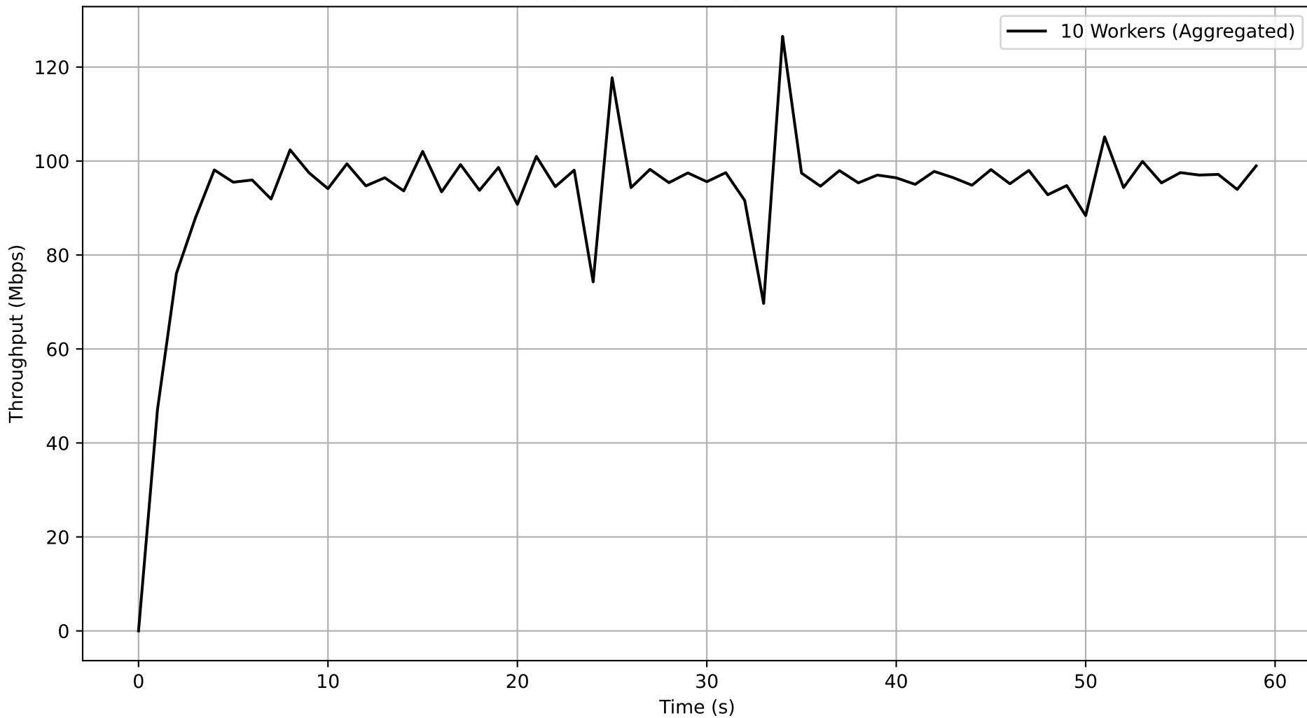
Job 6fdc8043-0101-450a-9733-5a5c54de69e0 - Subjob 3f294494-3fe7-47fd-8f2a-f15a536fc8da Aggregated Throughput Over Time
