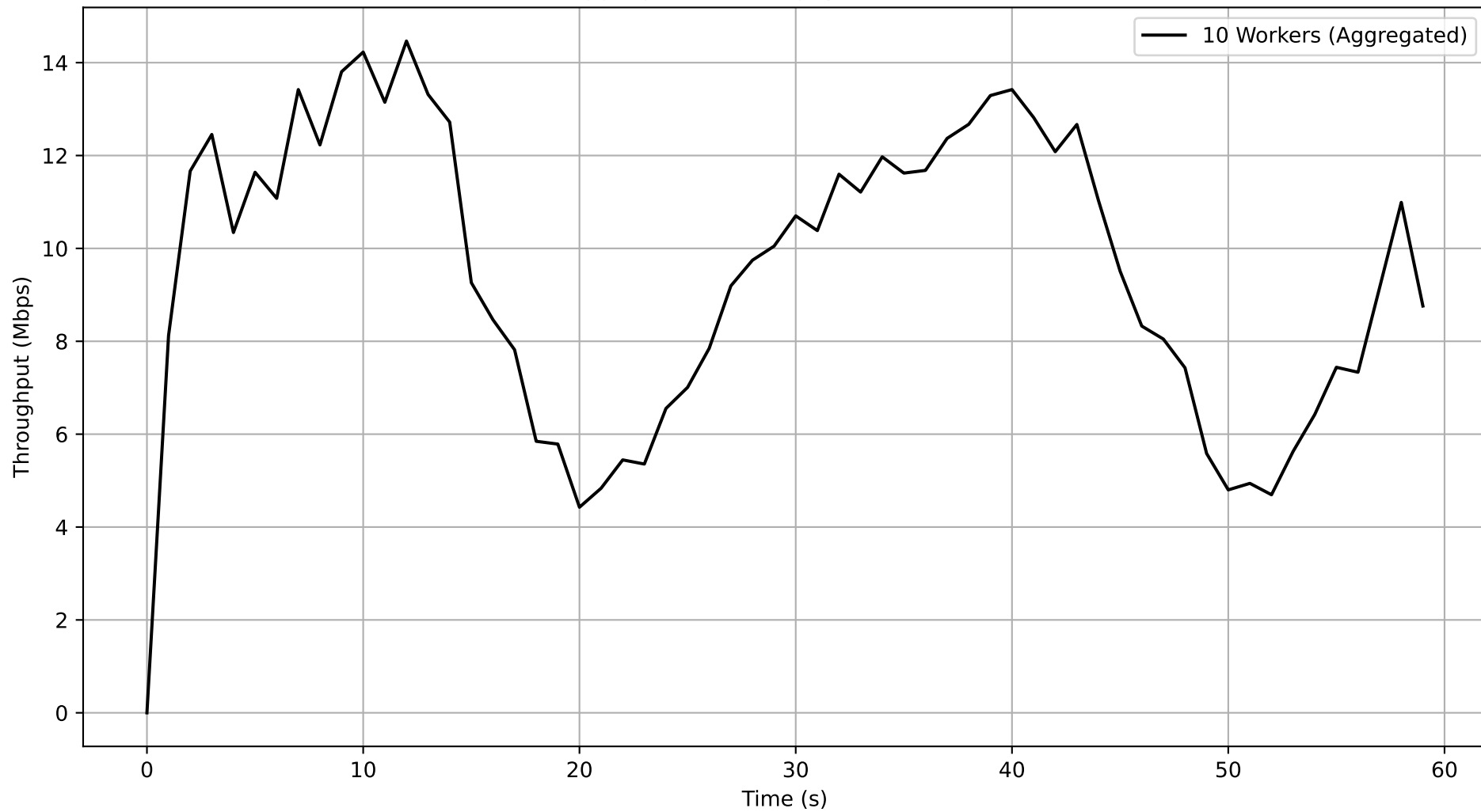
Job bd6c9540-117d-498c-8471-7e7e51979971 - Subjob f388d0bb-eb0e-4191-b23a-9dbfbd6b27b6 Aggregated Throughput Over Time
