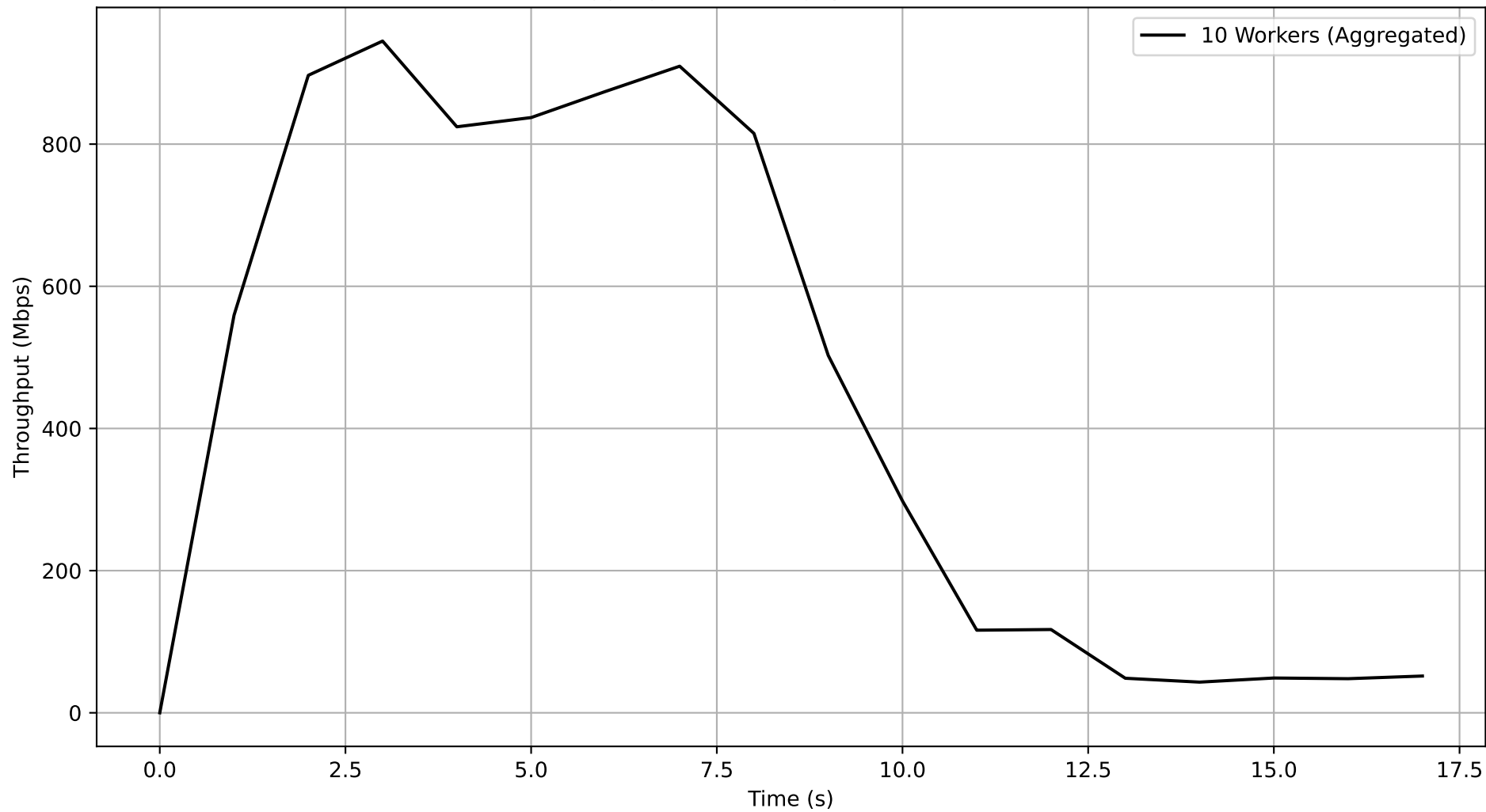
Job 37333d94-3012-4bcc-9bfd-4d15873af31b - Subjob 5ac2a361-c4f0-4522-9892-76e64fa473cd Aggregated Throughput Over Time
