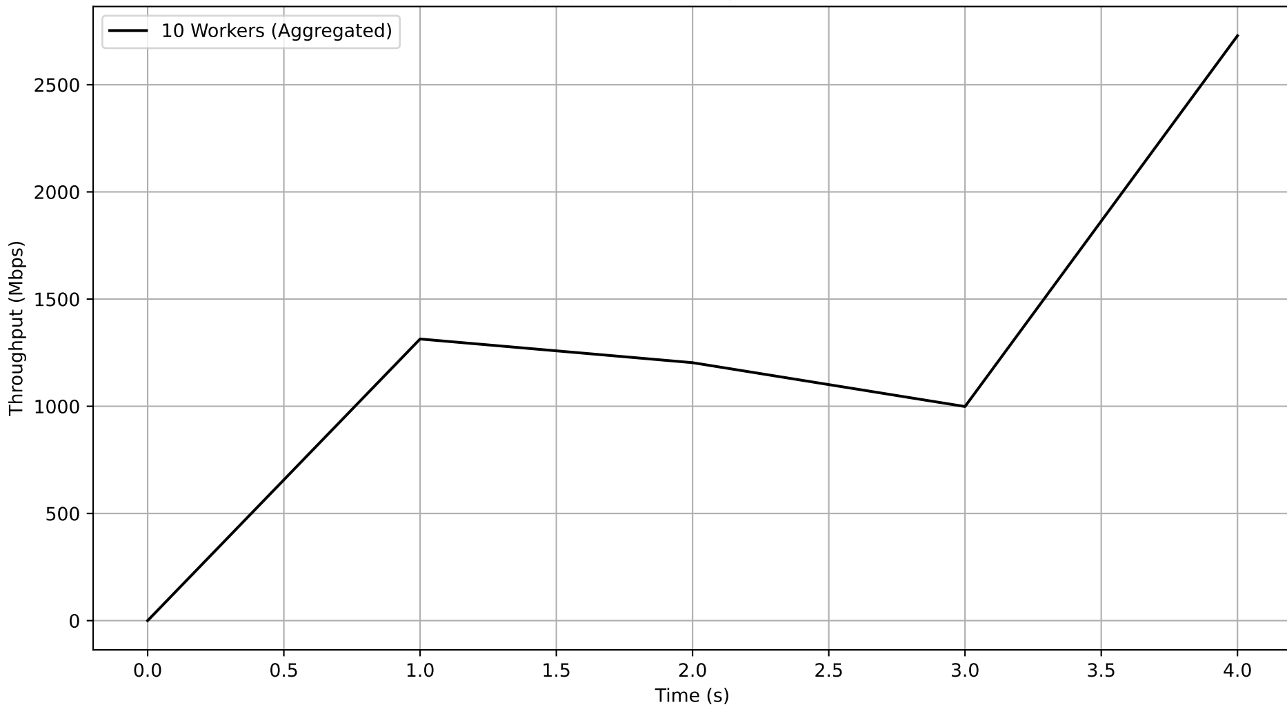
Job b32db341-8233-426e-a82a-eb5c6f358ebf - Subjob b003ece1-ff38-48f8-84f6-0cac153b5bcd Aggregated Throughput Over Time
