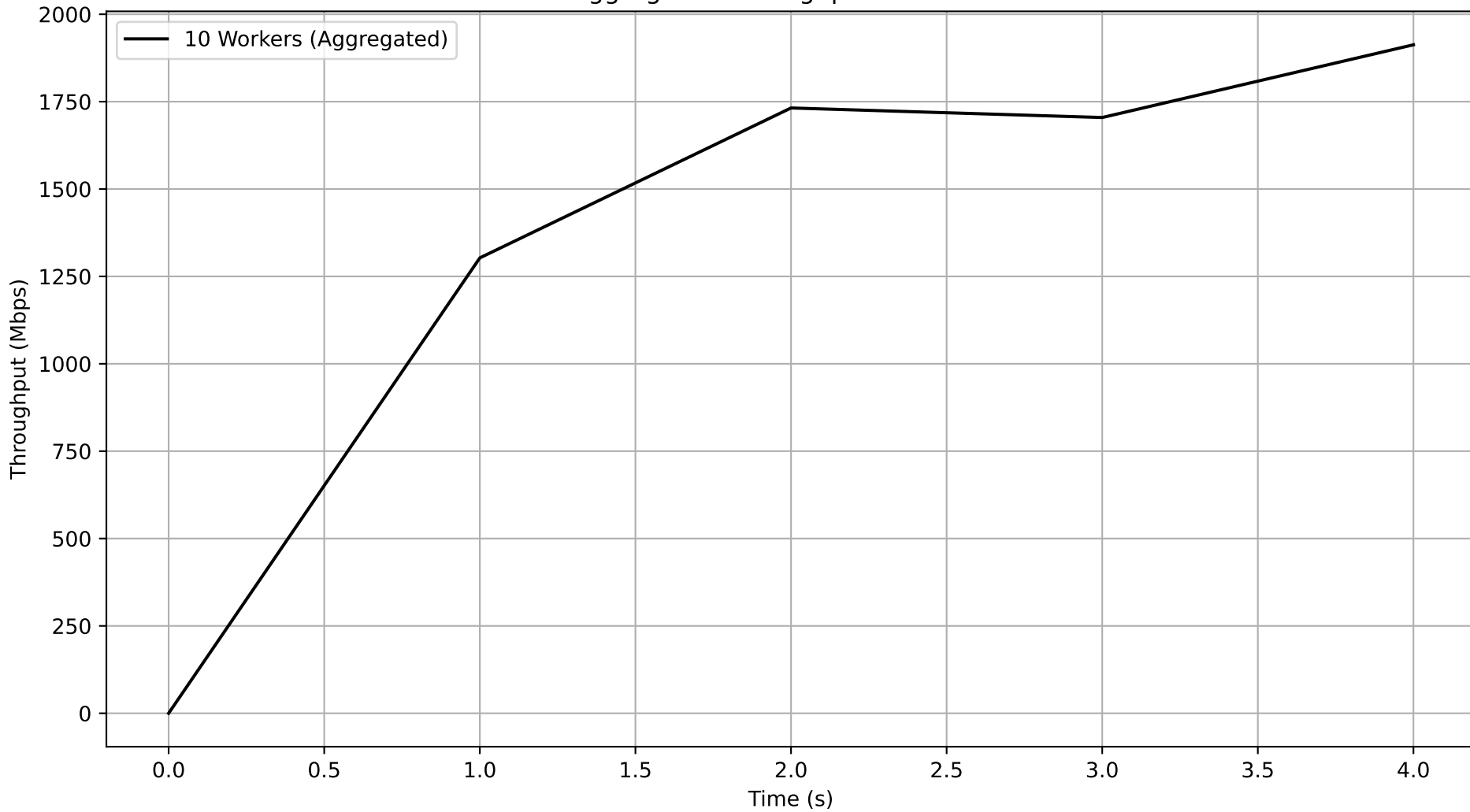
Job dc100bbf-b6bc-436d-90a4-8d0921e97afb - Subjob dc5d74a1-906f-42f1-a978-12830e9f215e Aggregated Throughput Over Time
