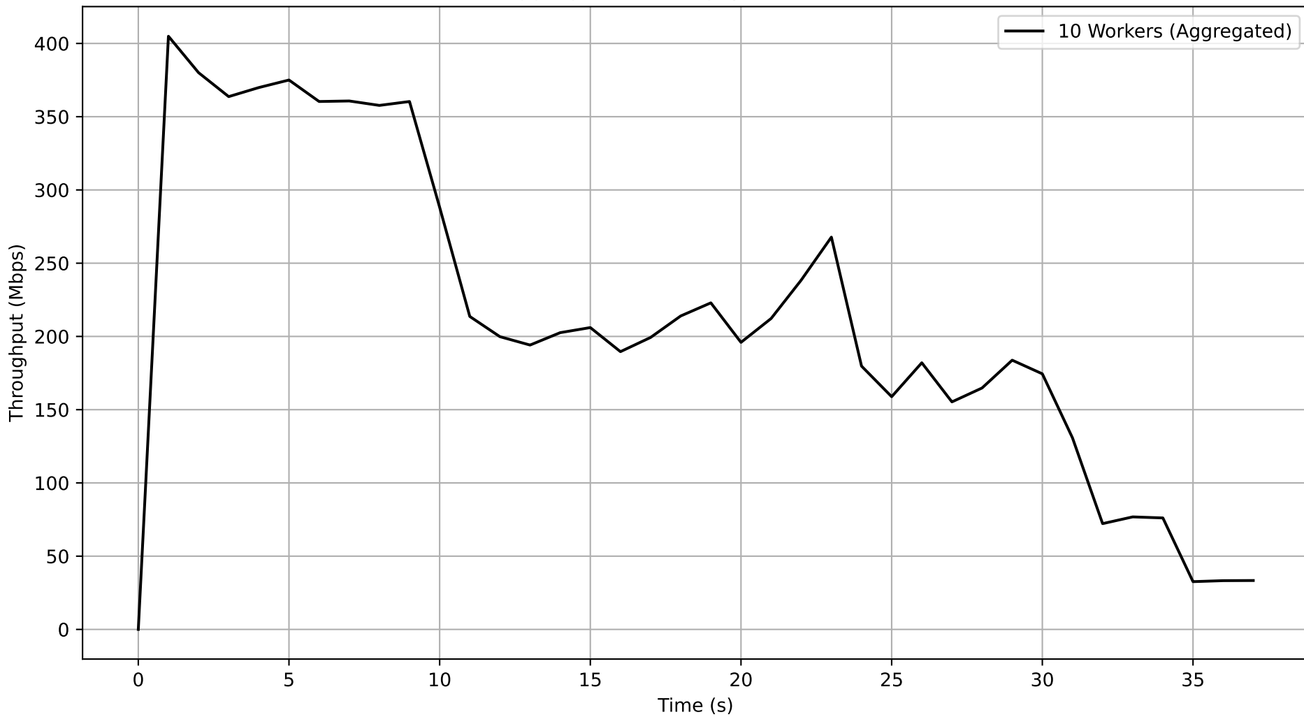
Job 4c5bda2e-cf5b-4beb-8735-a712d13badaa - Subjob d5fa4f27-abd8-4a27-a8a8-61d50eb8ec3f Aggregated Throughput Over Time
