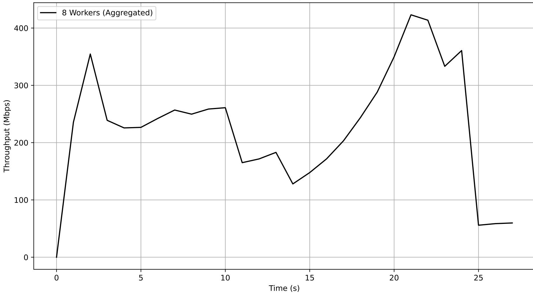
Job 02d466c5-ba4f-4bed-8651-7efbbbed94d54 - Subjob 98f952e1-5d2b-493c-88e7-4b555578b430 Aggregated Throughput Over Time
