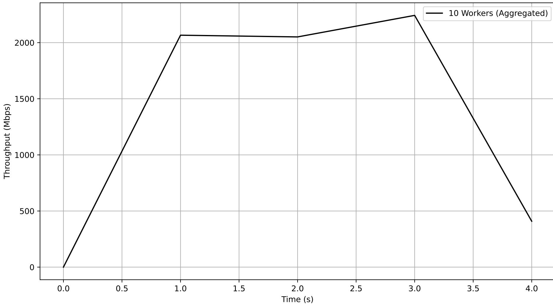
Job c854ca33-b6dd-4e56-bb20-385e8f712b25 - Subjob 16dcbb2a-03ef-4ae8-9195-8e2bf6299f8f Aggregated Throughput Over Time
