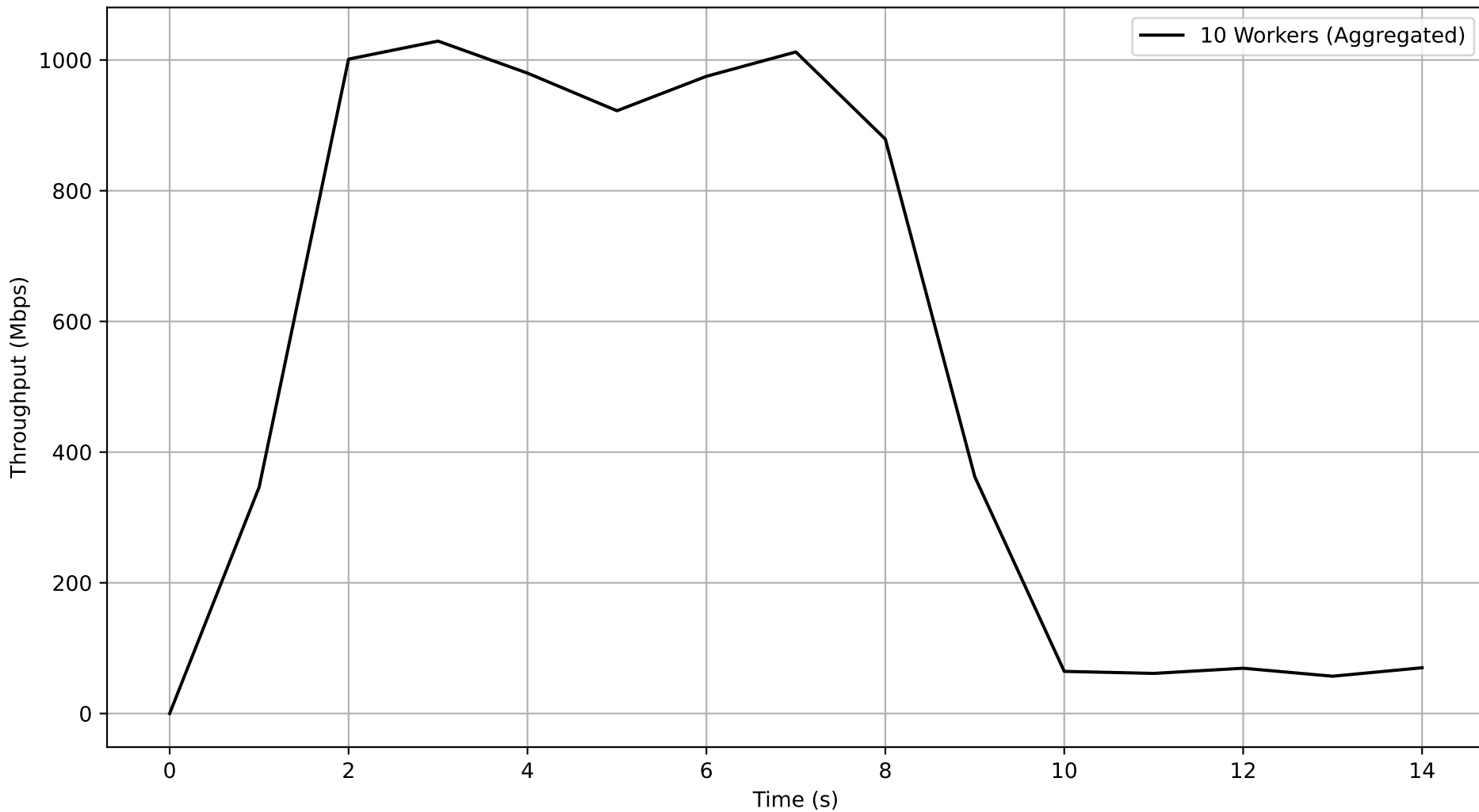
Job e6d3cdac-31bf-4908-a83d-9419882d3f98 - Subjob 9f554205-d98a-4ee2-9874-2991cd94d3be Aggregated Throughput Over Time
