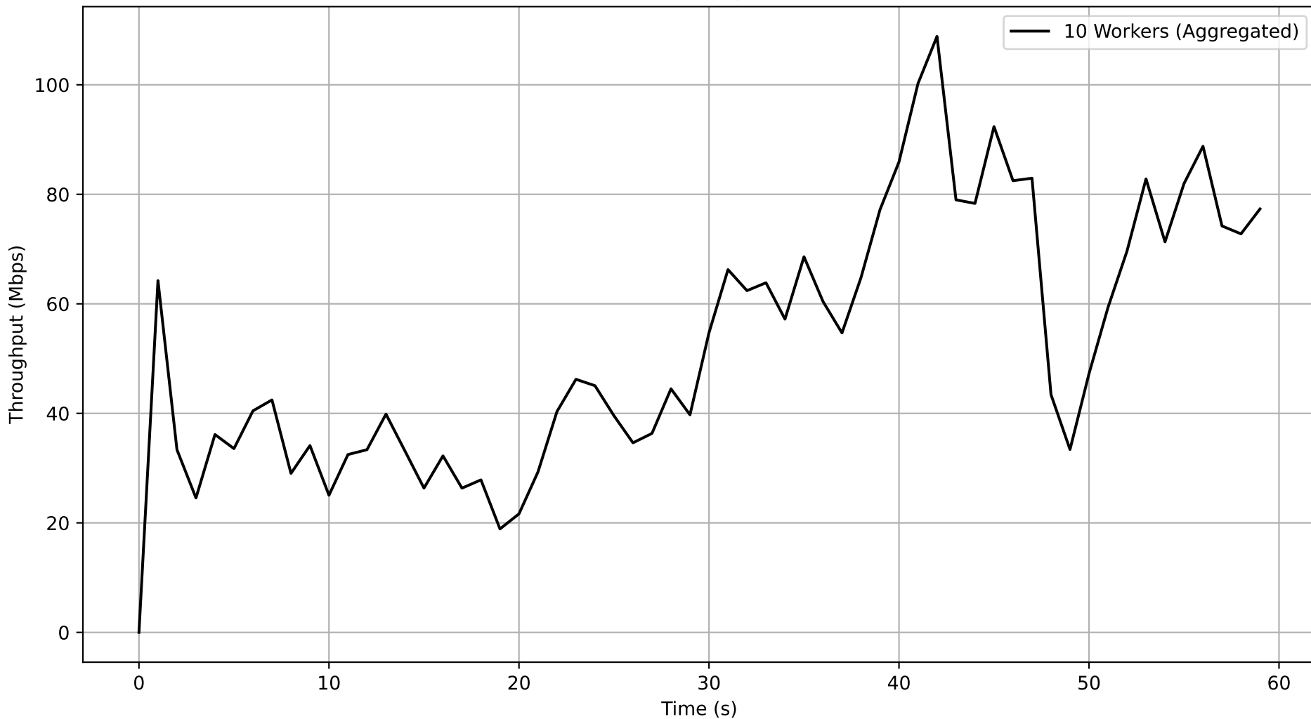
Job d91afa3b-be78-4f10-8de1-e385d0e28c21 - Subjob 77944449-4aec-41b4-aecd-dff8bc91b7ee Aggregated Throughput Over Time
