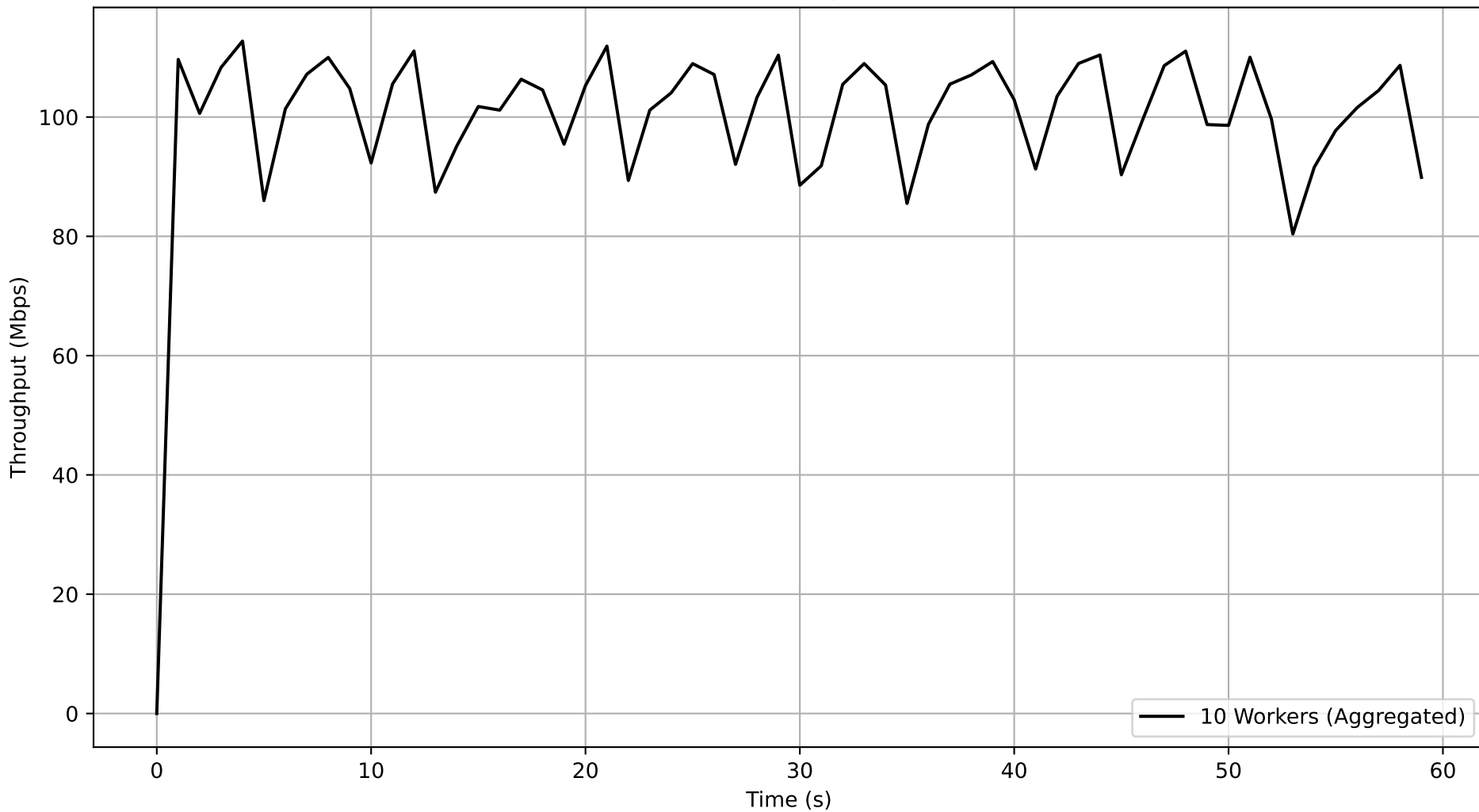
Job d0b3872b-b68c-417f-ac20-a9ec83b07a35 - Subjob 5cd6f07f-4f8f-4000-95e1-d118a119392b Aggregated Throughput Over Time
