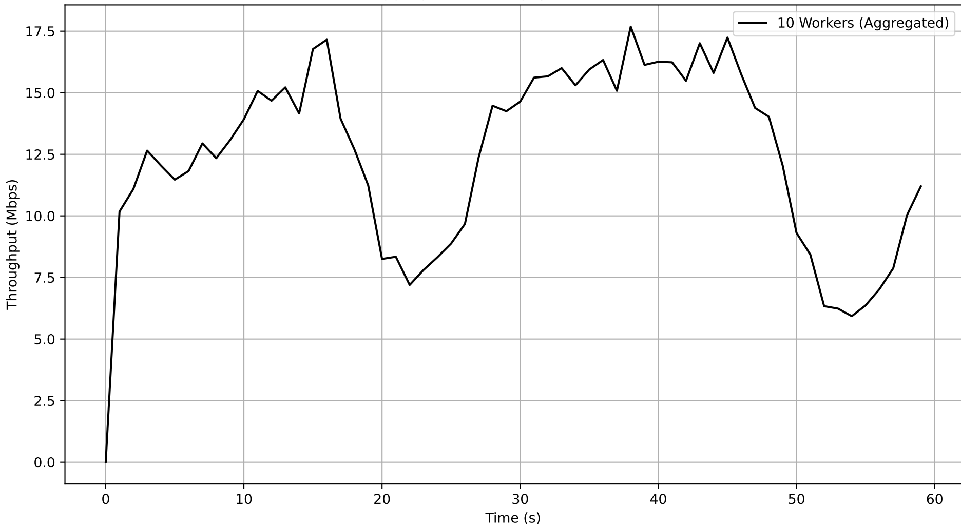
Job 041b3bbb-48e7-4ee1-8254-2218698ea01e - Subjob 1a50dc56-eb14-4af2-a734-92eacf473633 Aggregated Throughput Over Time
