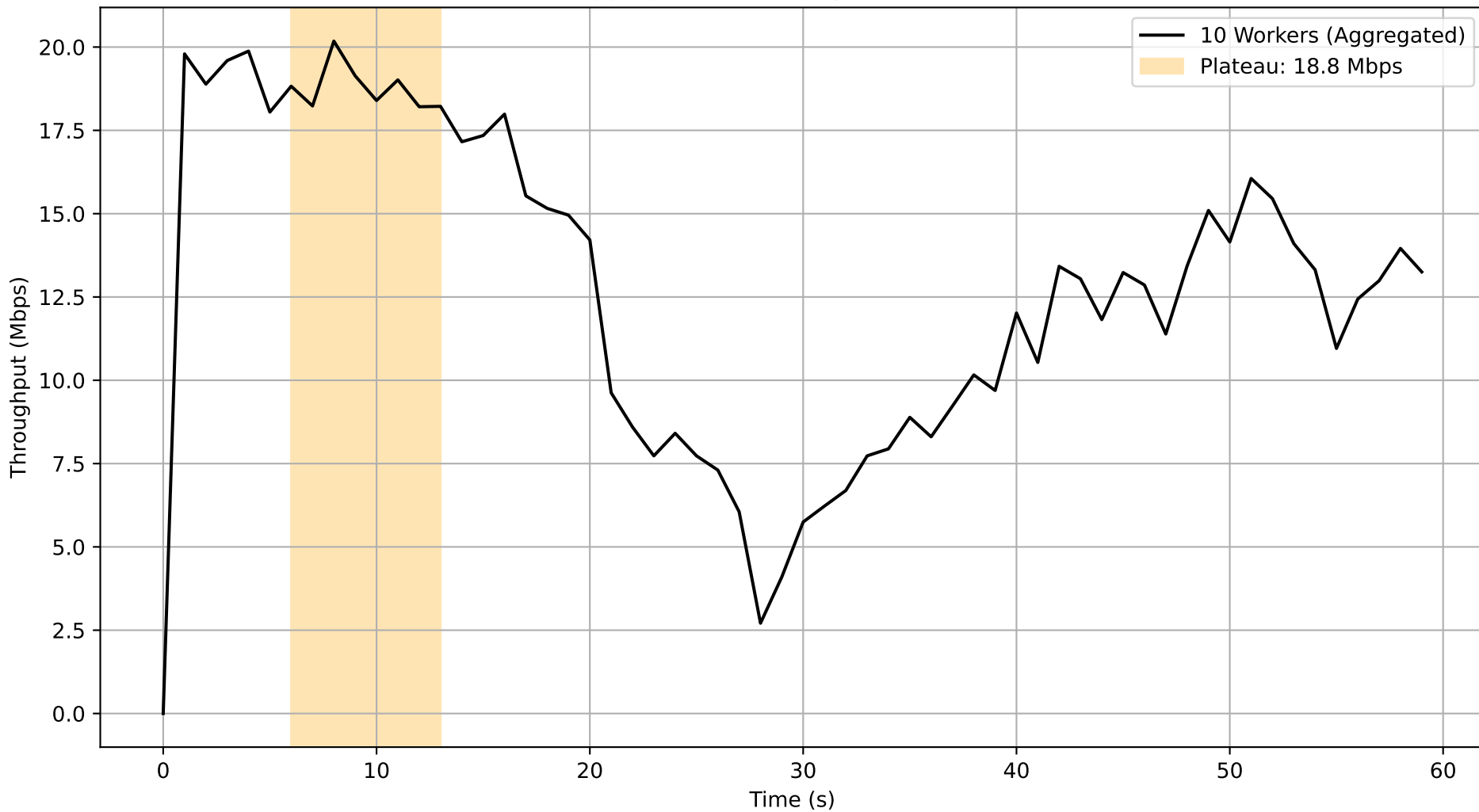
Job db415af2-770a-40ce-a7ad-b319626cd356 - Subjob f7212e3e-549e-4bc0-b780-84fb08ae0eab Aggregated Throughput Over Time
