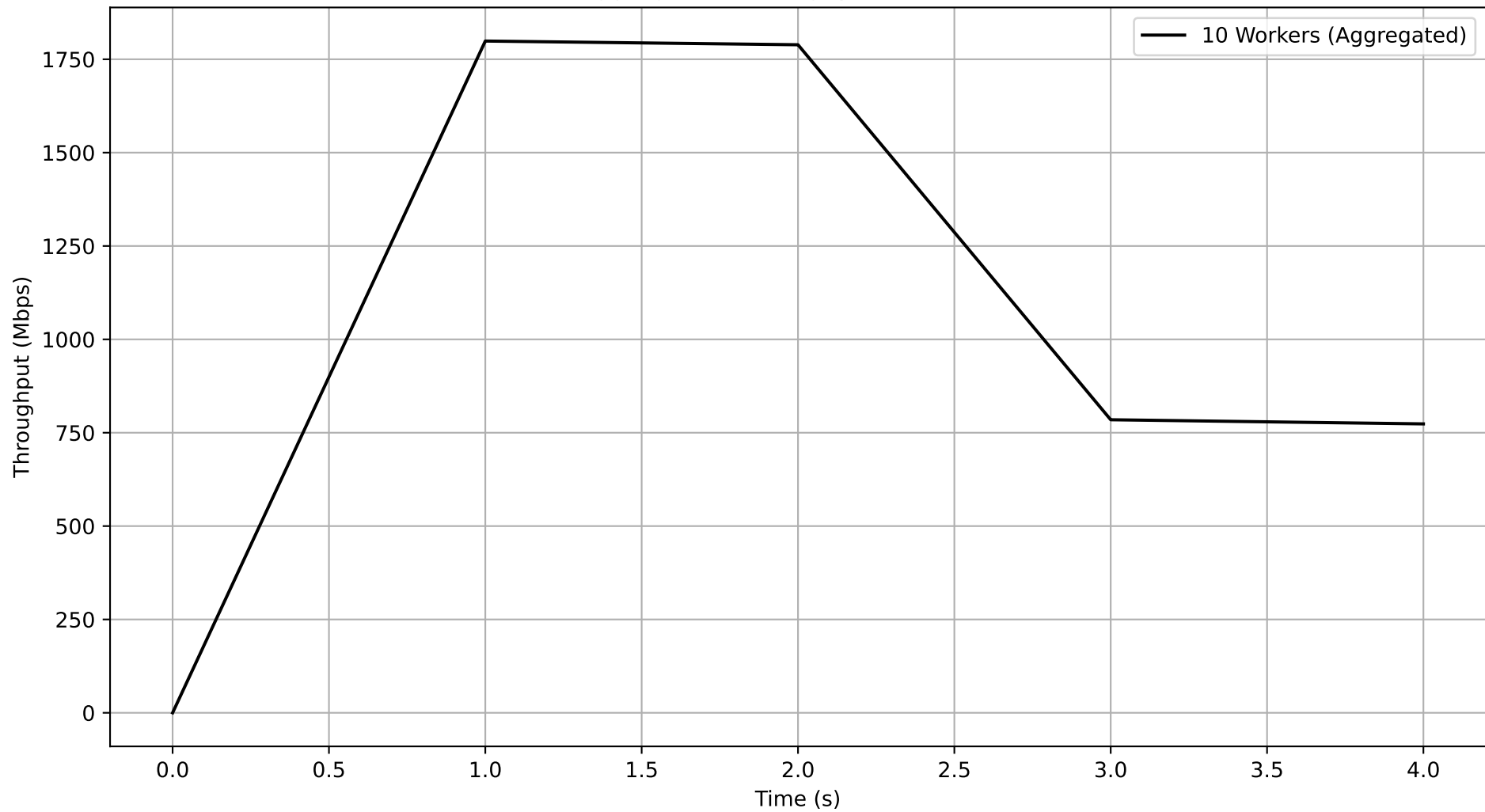
Job d9ec93b7-a37b-4a66-89e1-b9e215e7c25d - Subjob 60c2f62d-5c74-49bf-97cb-d19f1d318c0b Aggregated Throughput Over Time
