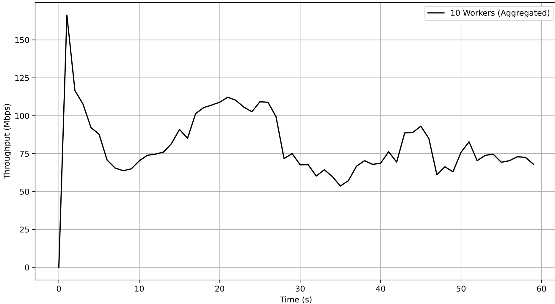
Job 96bcb907-fcaf-46fb-8fb8-2346a615bff4 - Subjob 7846e223-742c-4253-8cc5-f5898dfb850b Aggregated Throughput Over Time
