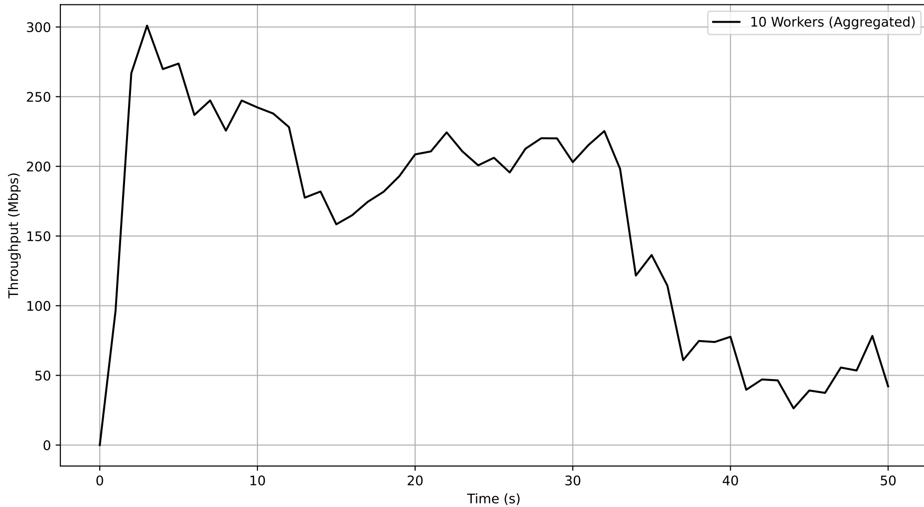
Job 86873df7-323e-40b9-a8b5-f13e825c4437 - Subjob 40ac1472-e8b4-4741-a40a-ad038c79b216 Aggregated Throughput Over Time
