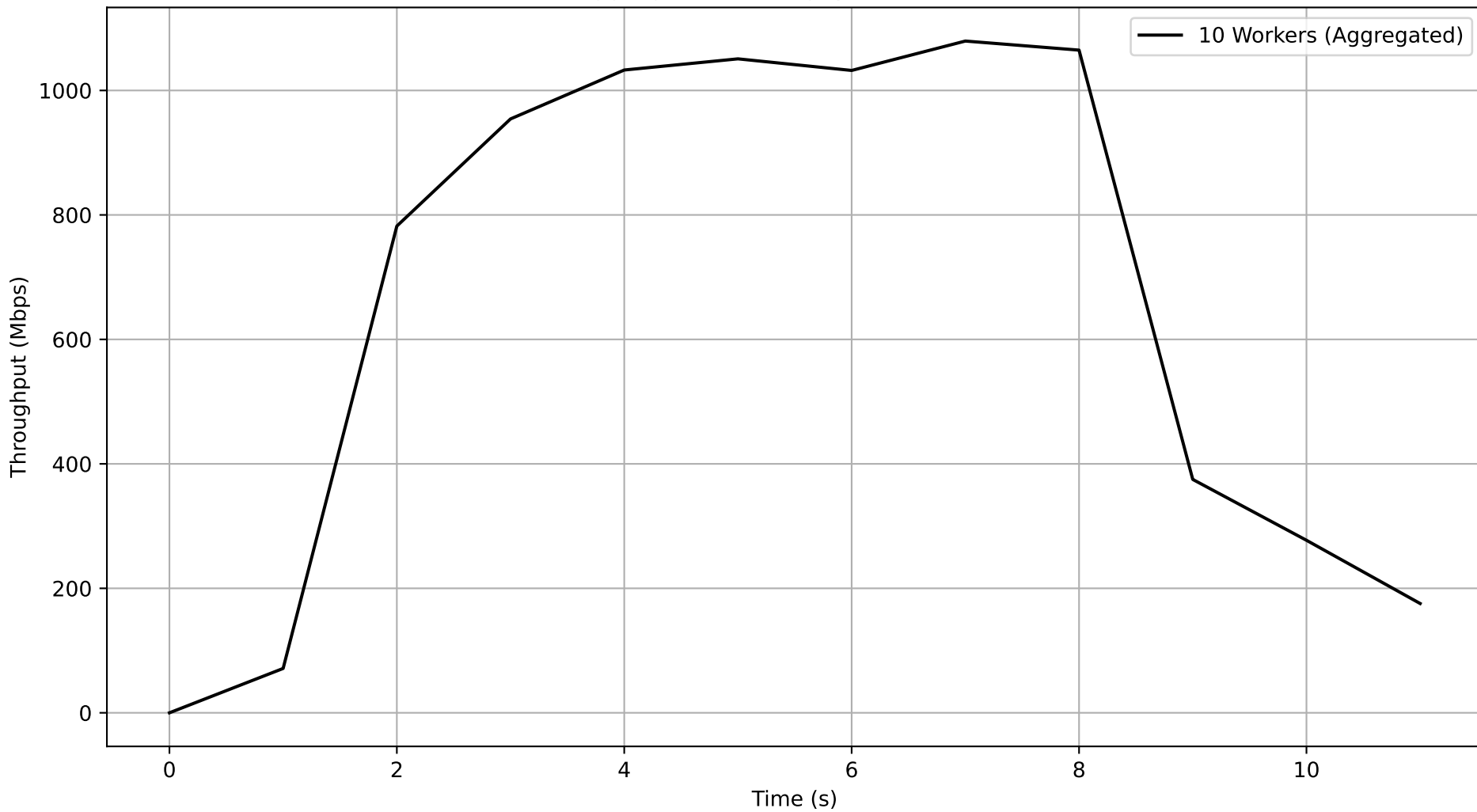
Job 4092d50b-9e15-484d-89f1-56a49edc2eeb - Subjob f856950a-93b7-443f-8e06-7e1088e04376 Aggregated Throughput Over Time
