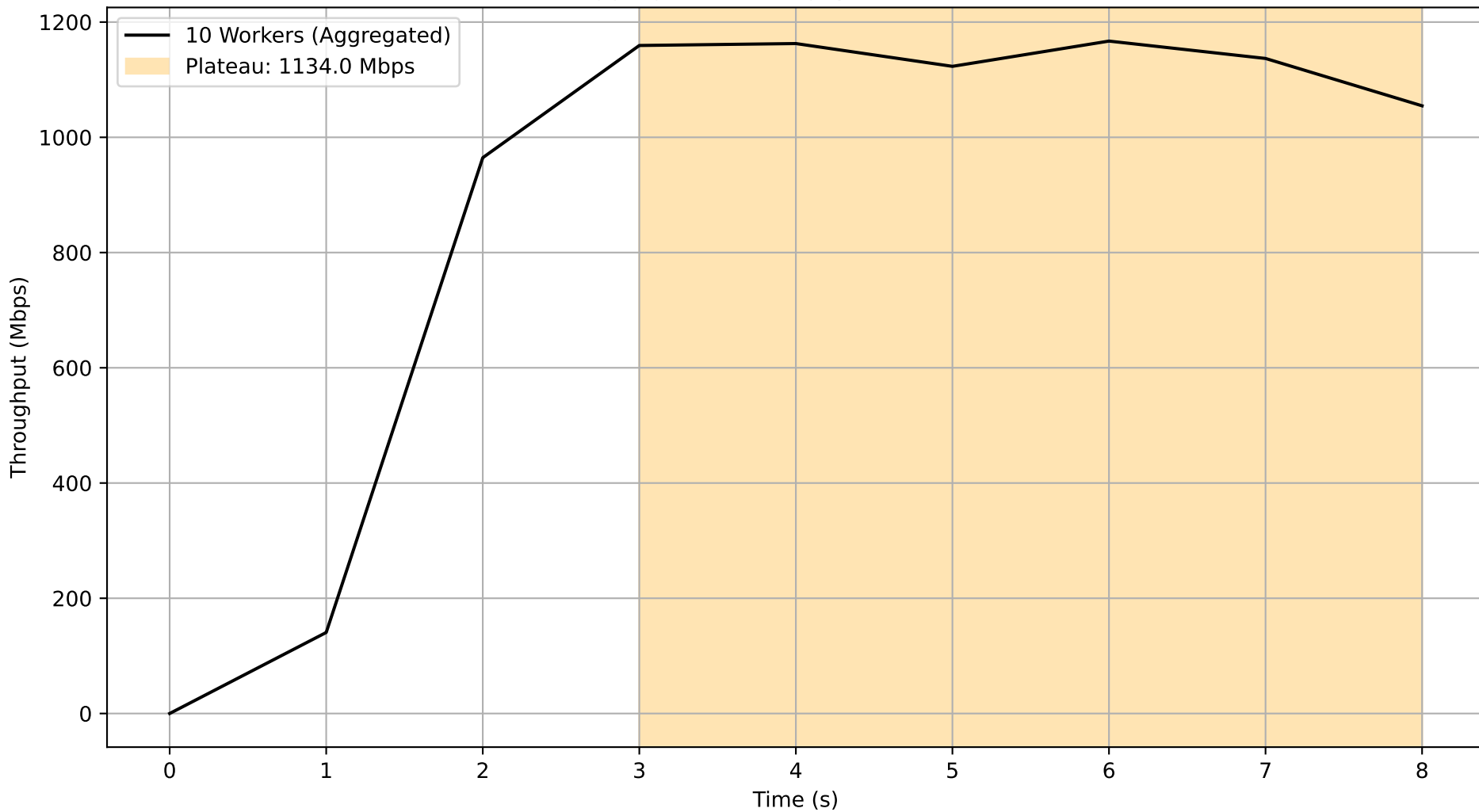
Job 1555dffd-62cd-4024-bed5-42a0b2a4e0f7 - Subjob dd144e66-a450-441f-88e6-2403277bccba Aggregated Throughput Over Time
