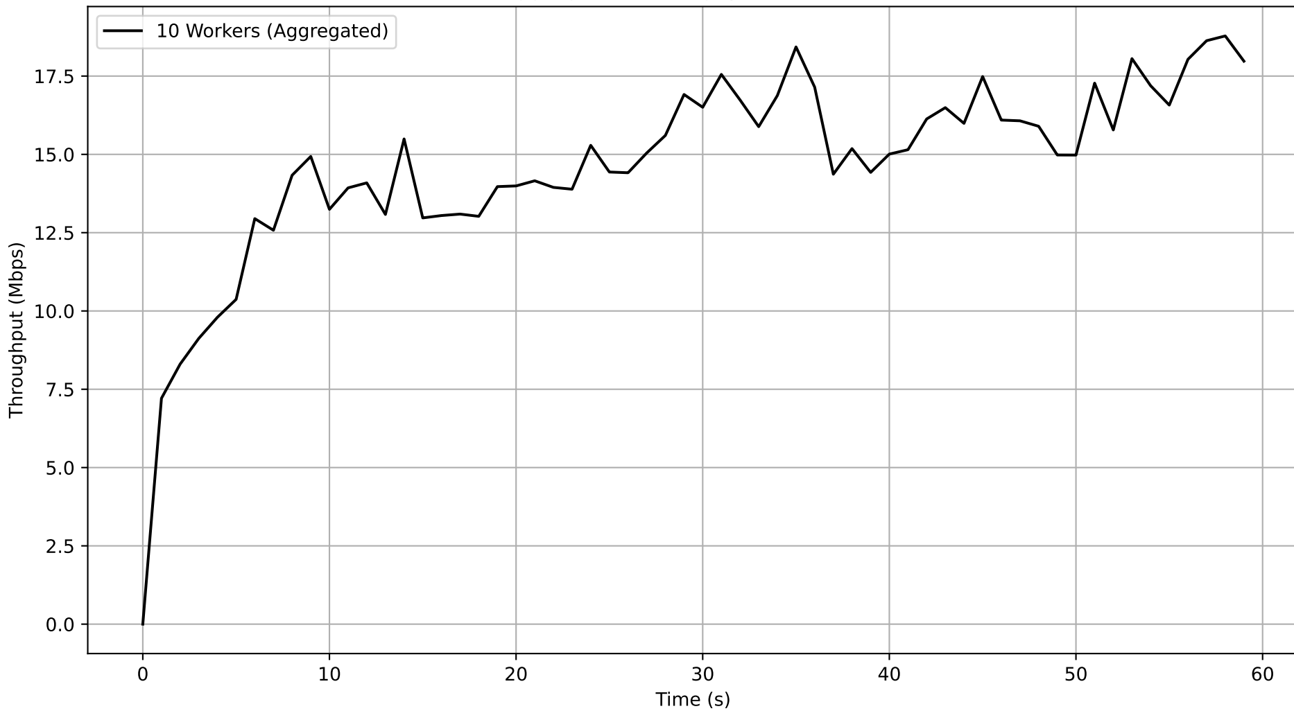
Job 3113c5d2-29b3-4968-8d59-79d7b4730cb3 - Subjob ab66b178-317a-43bd-b6da-70da8fe155b9 Aggregated Throughput Over Time
