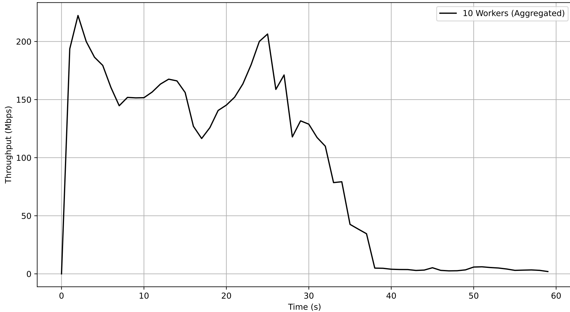
Job 4ebc1977-6ca6-4ca8-9f75-ed2c0c39c5e4 - Subjob 47e9c760-e666-4bc5-af42-1738748f8da5 Aggregated Throughput Over Time
