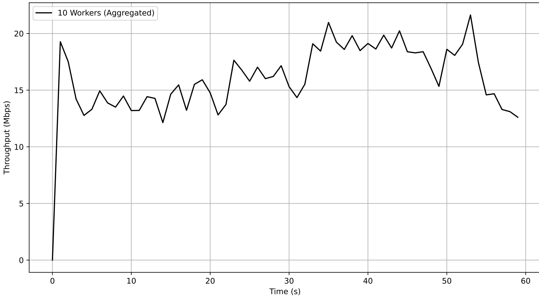
Job c2c2157c-a1fc-467a-a06a-d823ced51648 - Subjob 86f236b8-bf65-47be-aa7d-f5ba8c6f66b7 Aggregated Throughput Over Time
