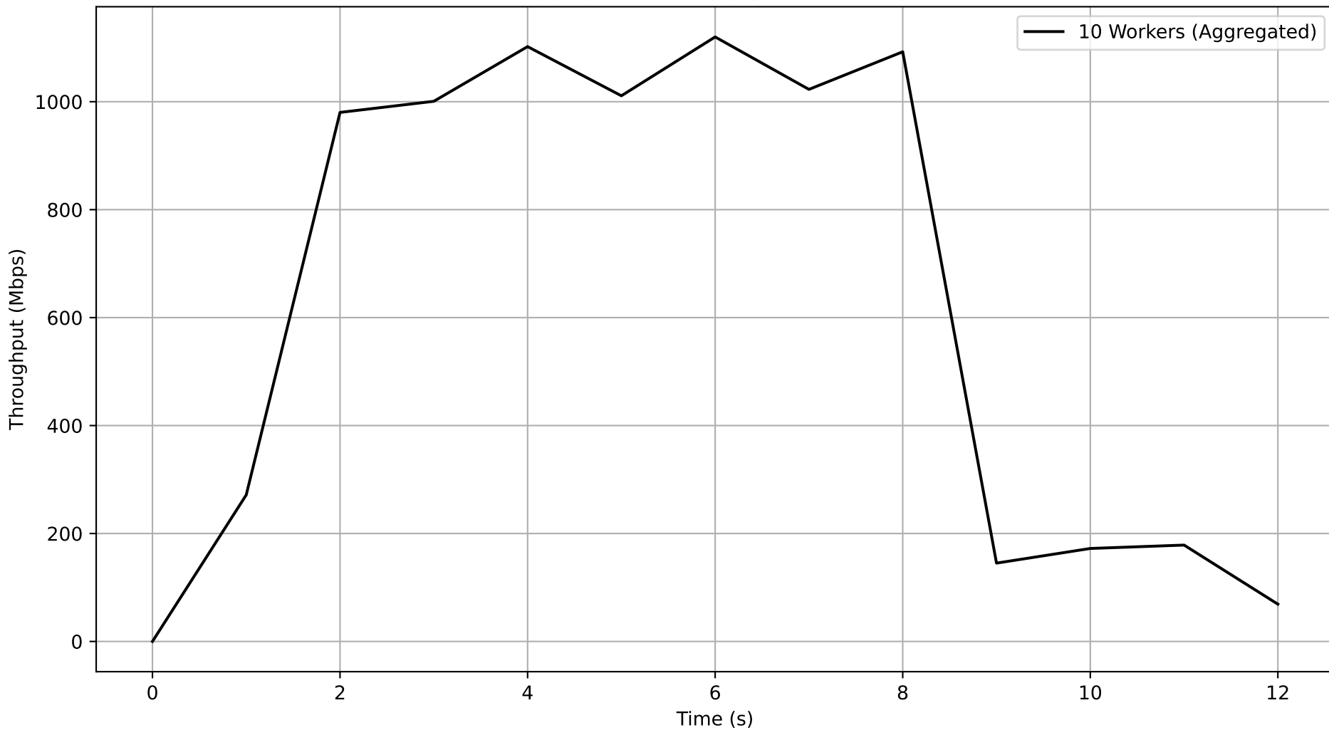
Job 27c30a3a-e893-4d49-a059-691a9c68d28a - Subjob c5b4f757-4e3d-4bf5-9392-ff798c5de974 Aggregated Throughput Over Time
