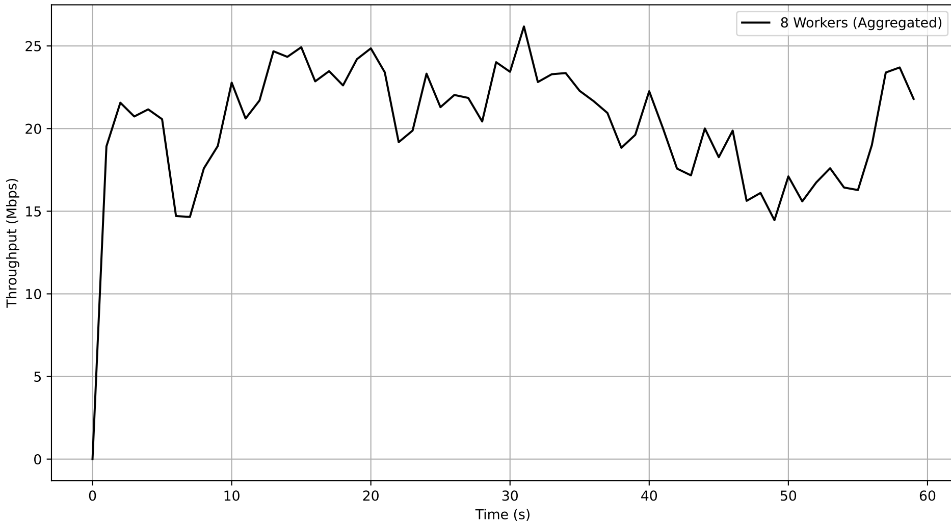
Job 61e021aa-be64-478c-b629-2b765c056351 - Subjob 9401c51e-bd64-45ce-88a0-f9a5ecc224fc Aggregated Throughput Over Time
