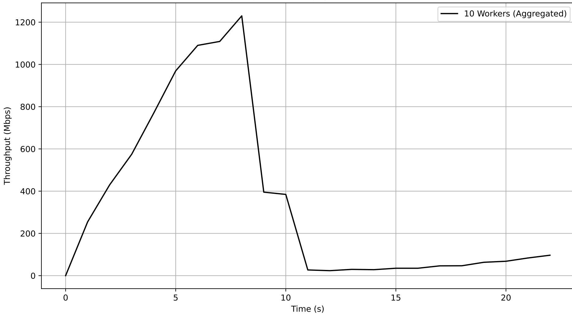
Job 0c66d895-471b-4059-a1ff-9a7926ed099e - Subjob a686db8a-50cc-4775-8295-e79df5e312e3 Aggregated Throughput Over Time
