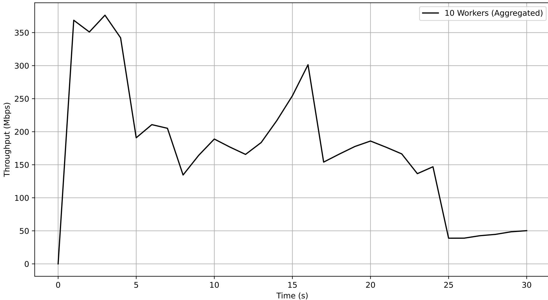
Job ae51b993-7de7-4333-8b0c-b304aa2e14eb - Subjob 17d14387-f757-4734-9211-5c9c08567a27 Aggregated Throughput Over Time
