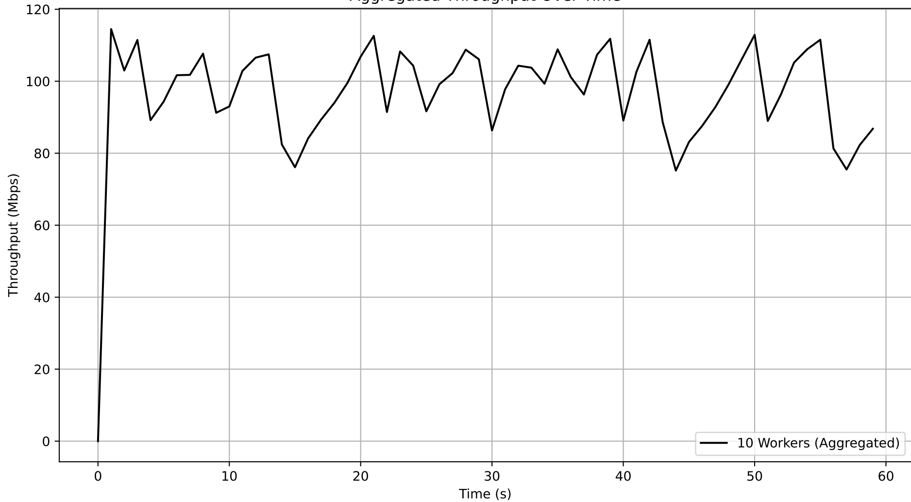
Job 7c626bba-3cbc-4664-a2e6-bfb7834978b5 - Subjob 02844f7a-7290-49ee-9809-c0b6af6c8ae5 Aggregated Throughput Over Time
