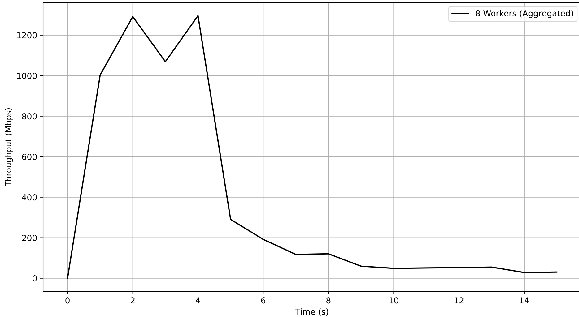
Job 0ed9699b-b898-458d-9e49-907e4c907d65 - Subjob a560ddef-9b91-40f8-99c9-00c44216b8b9 Aggregated Throughput Over Time
