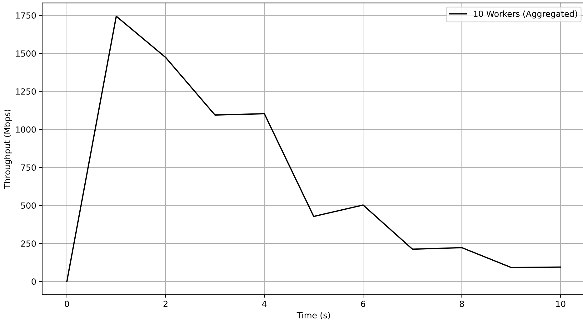
Job 50e3de30-efbe-4d79-8da6-13a09c1a83a7 - Subjob 544c0676-3d35-4521-9213-f200d01f6ab6 Aggregated Throughput Over Time
