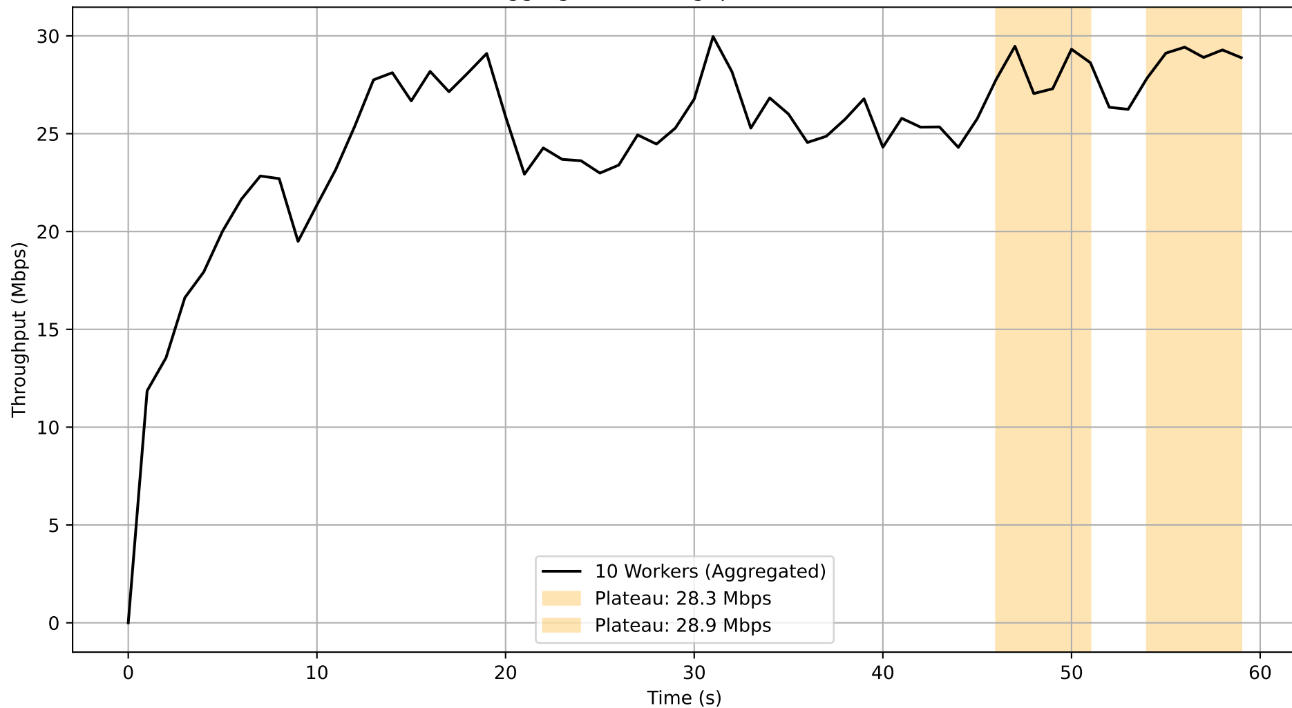
Job 69acafca-47c2-4e59-a191-d8528d4f1e2d - Subjob 10619138-f294-420b-b387-1f510da29e5a Aggregated Throughput Over Time
