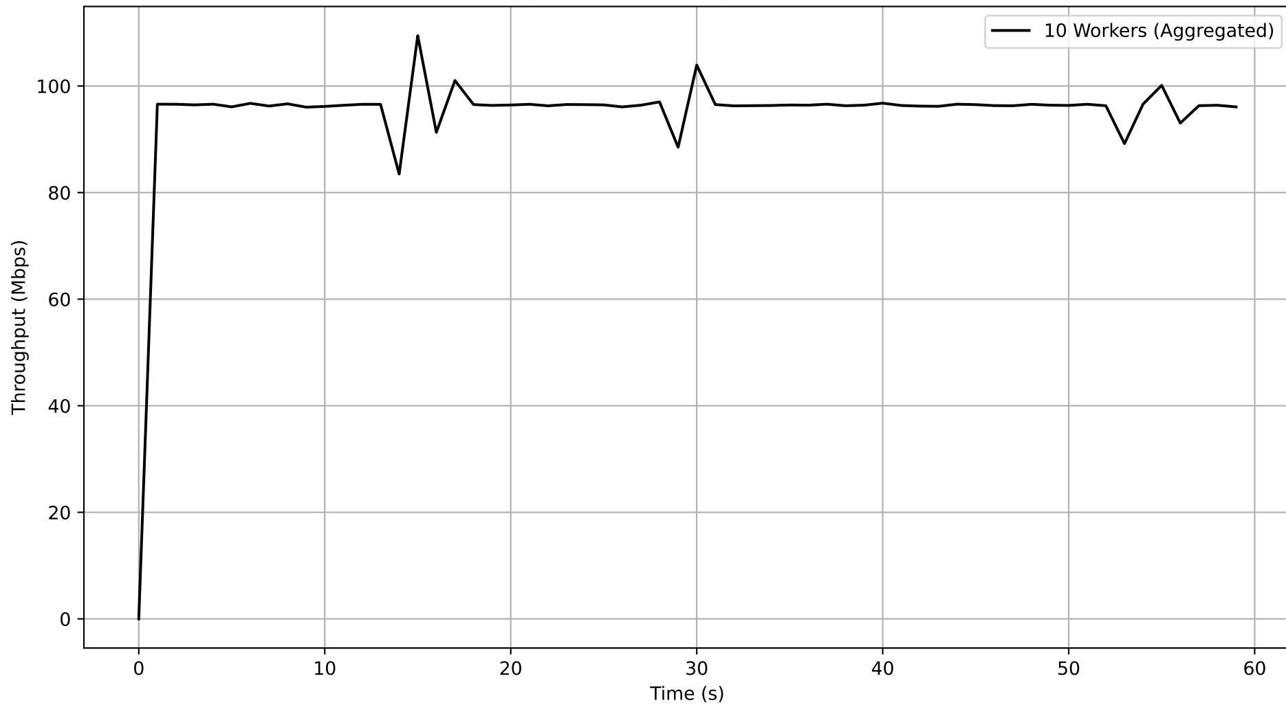
Job e1032366-5276-4375-9262-a854b777054e - Subjob 09f62e91-9705-464e-820b-827ac9983032 Aggregated Throughput Over Time
