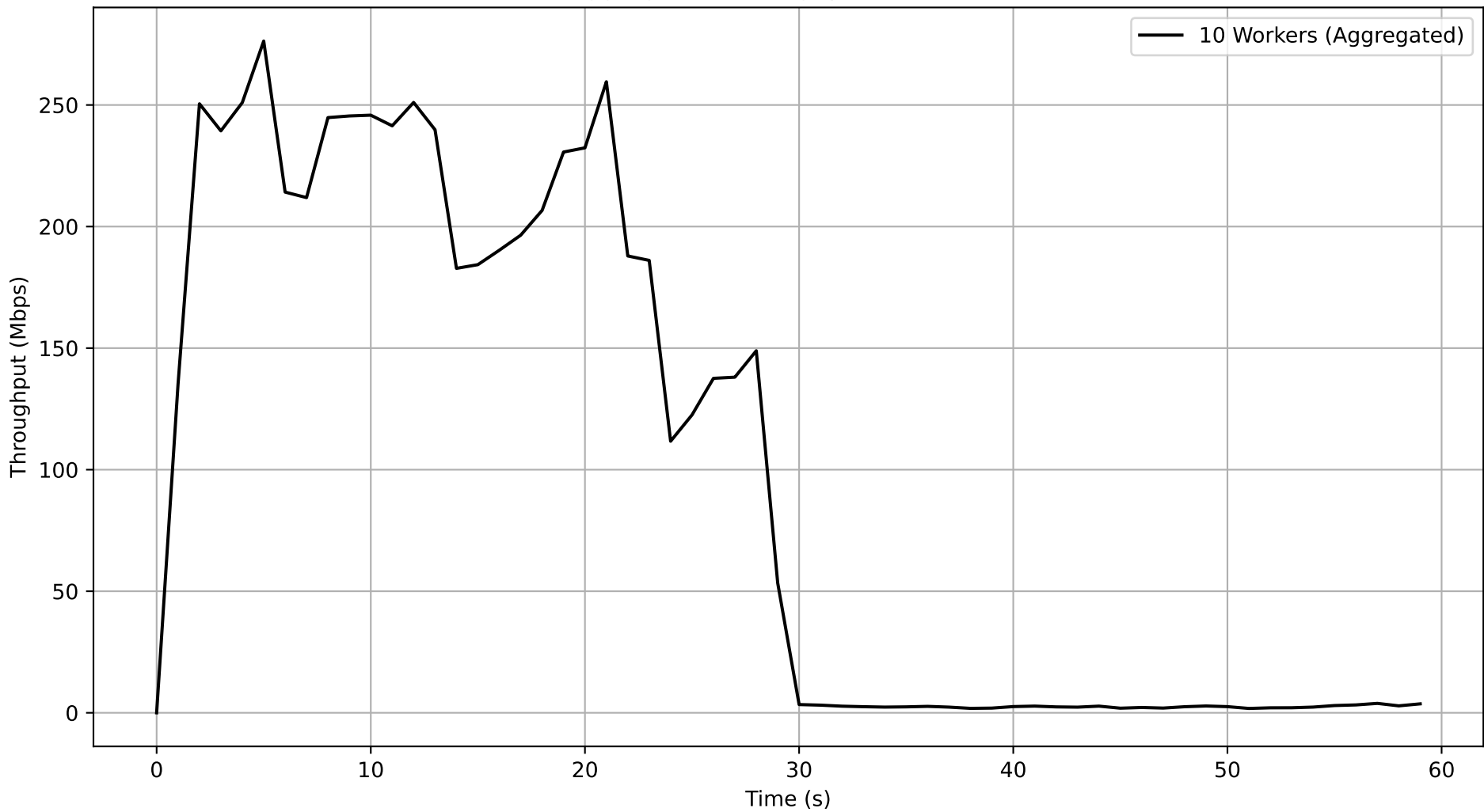
Job 40f92fe0-aa82-402f-8fce-9486841745aa - Subjob 43ee8332-acdb-465f-be2d-c2779979d1af Aggregated Throughput Over Time
