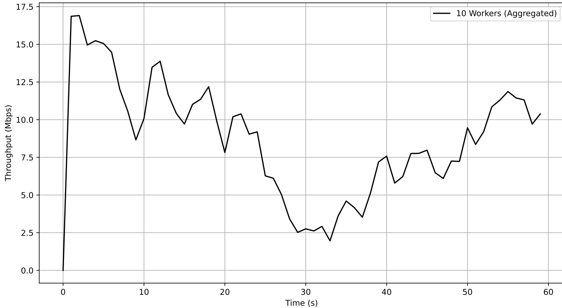
Job c2c2157c-a1fc-467a-a06a-d823ced51648 - Subjob a060f665-db3b-4796-91ba-de68a213e1f2 Aggregated Throughput Over Time
