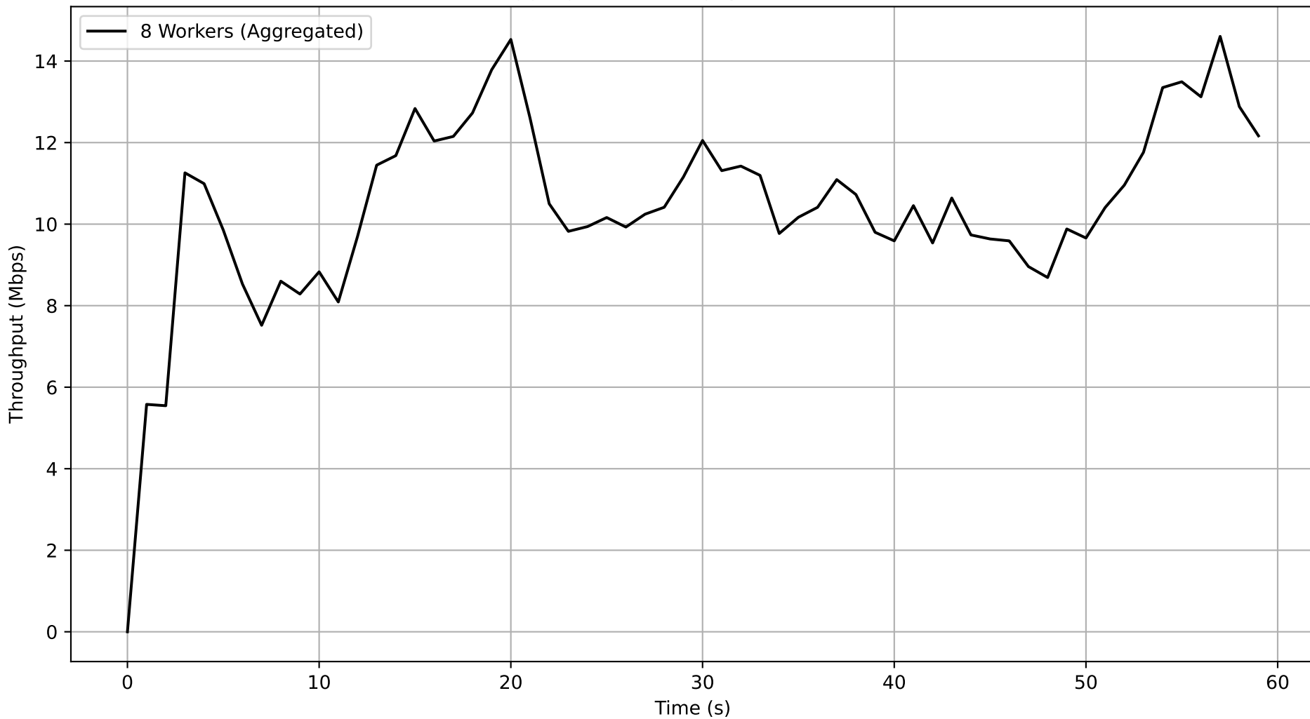
Job e7cfd0e0-cb64-4cb6-be33-e736988fd089 - Subjob d2e19aa5-8593-46b0-8733-e6cade2d302e Aggregated Throughput Over Time
