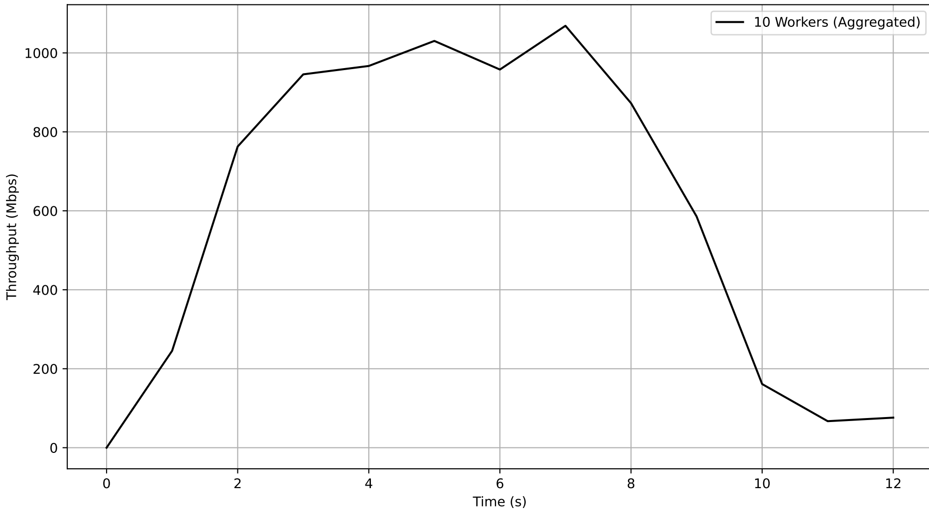
Job 7eb3d672-9c08-4a15-97ec-49b5dbfc2946 - Subjob e44cfb32-b886-48dd-b920-c989cb71fa91 Aggregated Throughput Over Time
