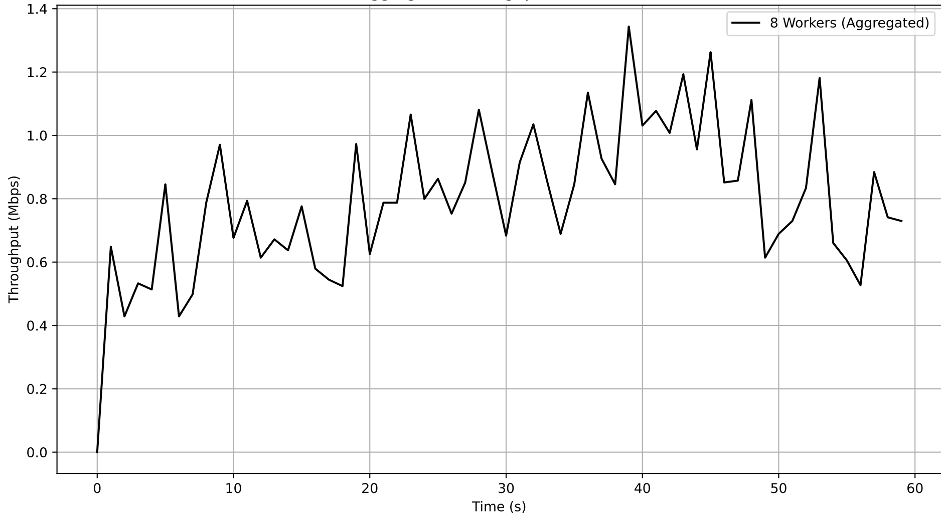
Job 29010eff-b6a0-4de7-953e-8953601cfda2 - Subjob 51e5ebcf-f008-4319-ad32-ef48797f015c Aggregated Throughput Over Time
