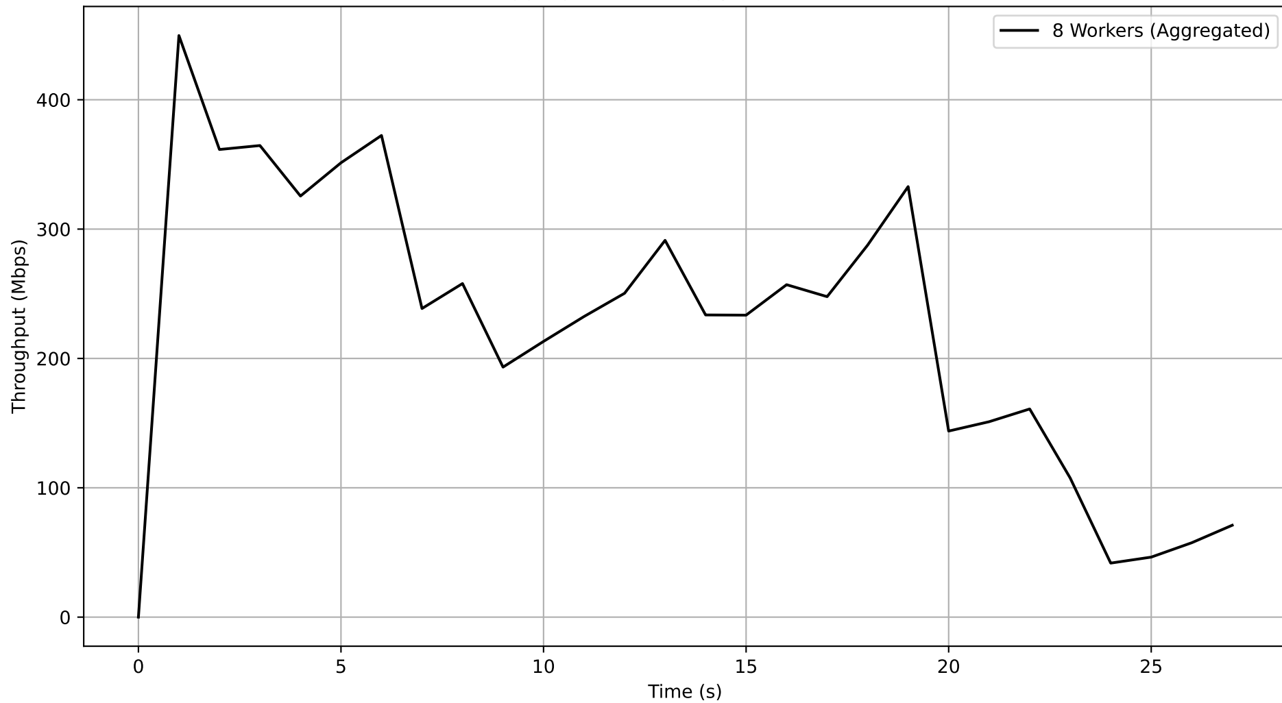
Job f6f76215-da14-4f20-872c-8a890bf9aaad - Subjob bafa95e1-0d90-4f71-aa04-0e1ea092462e Aggregated Throughput Over Time
