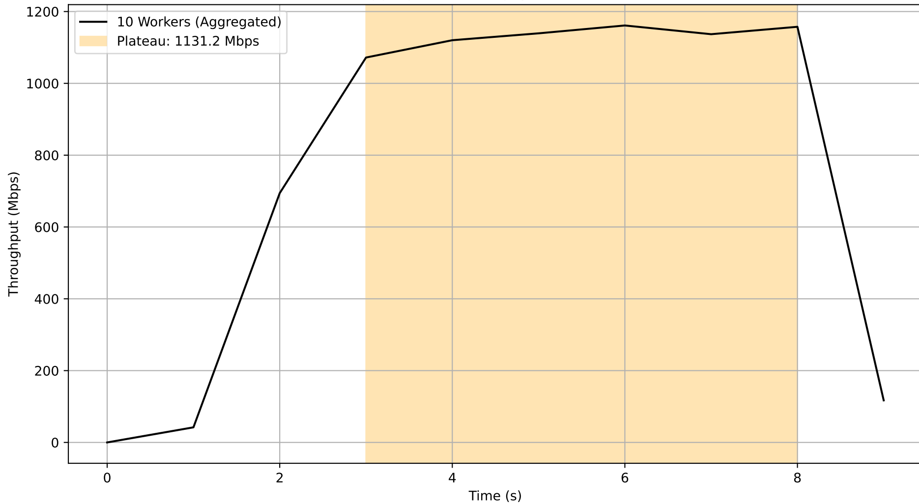
Job 4092d50b-9e15-484d-89f1-56a49edc2eeb - Subjob c46680d9-7db6-4cf7-9710-5fee077e33e0 Aggregated Throughput Over Time
