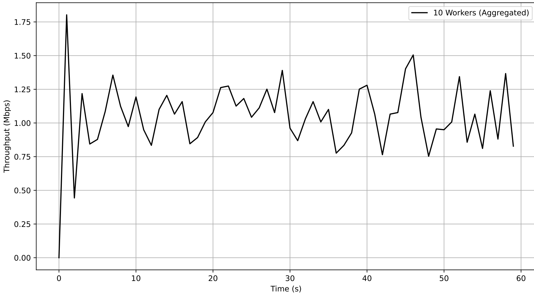
Job a3eea625-18fb-42ab-b89a-fa90eb7428b1 - Subjob 1a3761e3-991c-41ae-8d59-7e06104019b4 Aggregated Throughput Over Time
