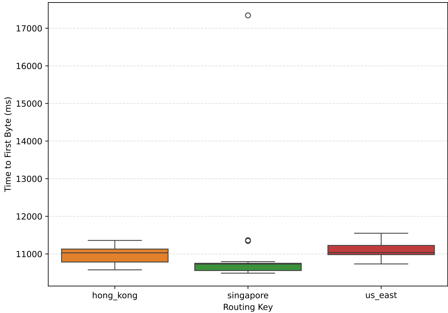
Time to First Byte Distribution by Routing Key
