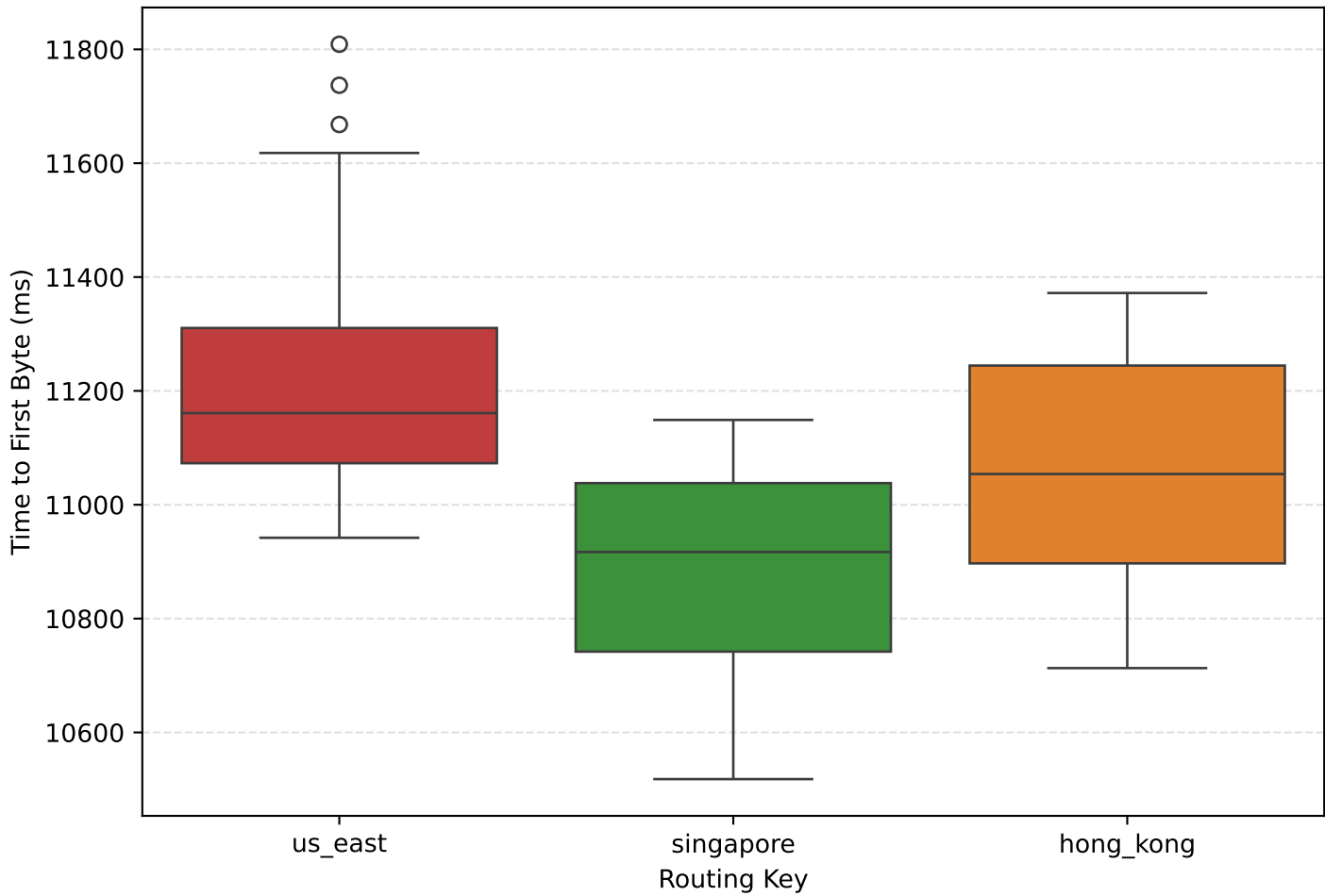
Time to First Byte Distribution by Routing Key
