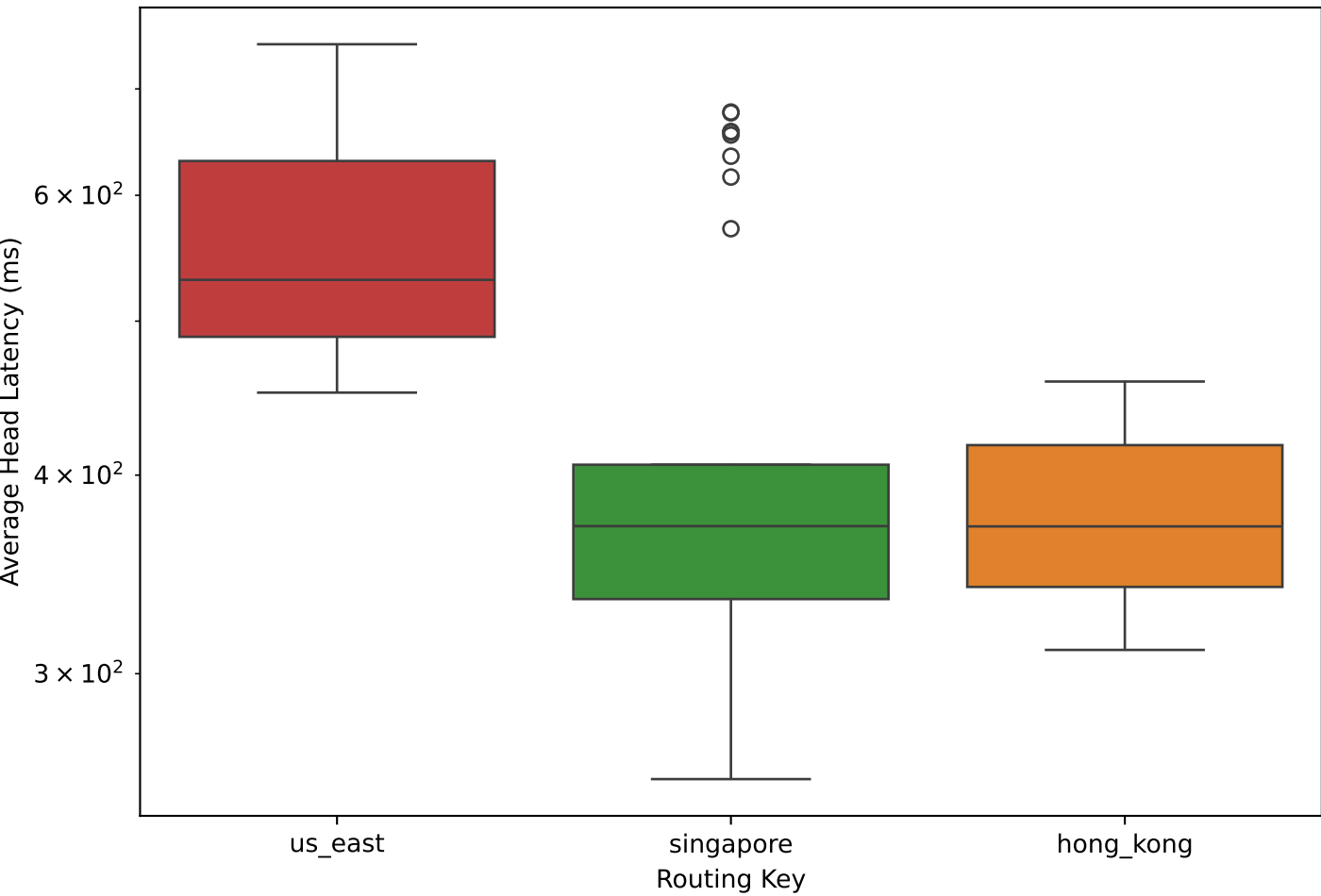
Head Latency Distribution by Routing Key
