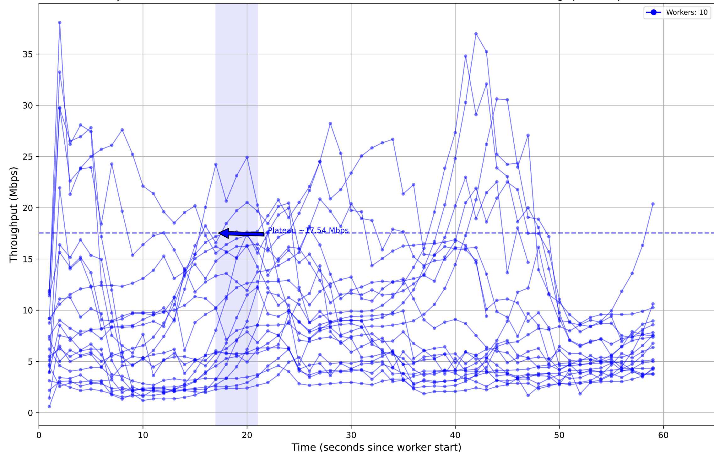
Job ID: c7057de1-b64e-48ac-aafe-cc17cdd37556 - Individual Worker Throughput (Mbps)
