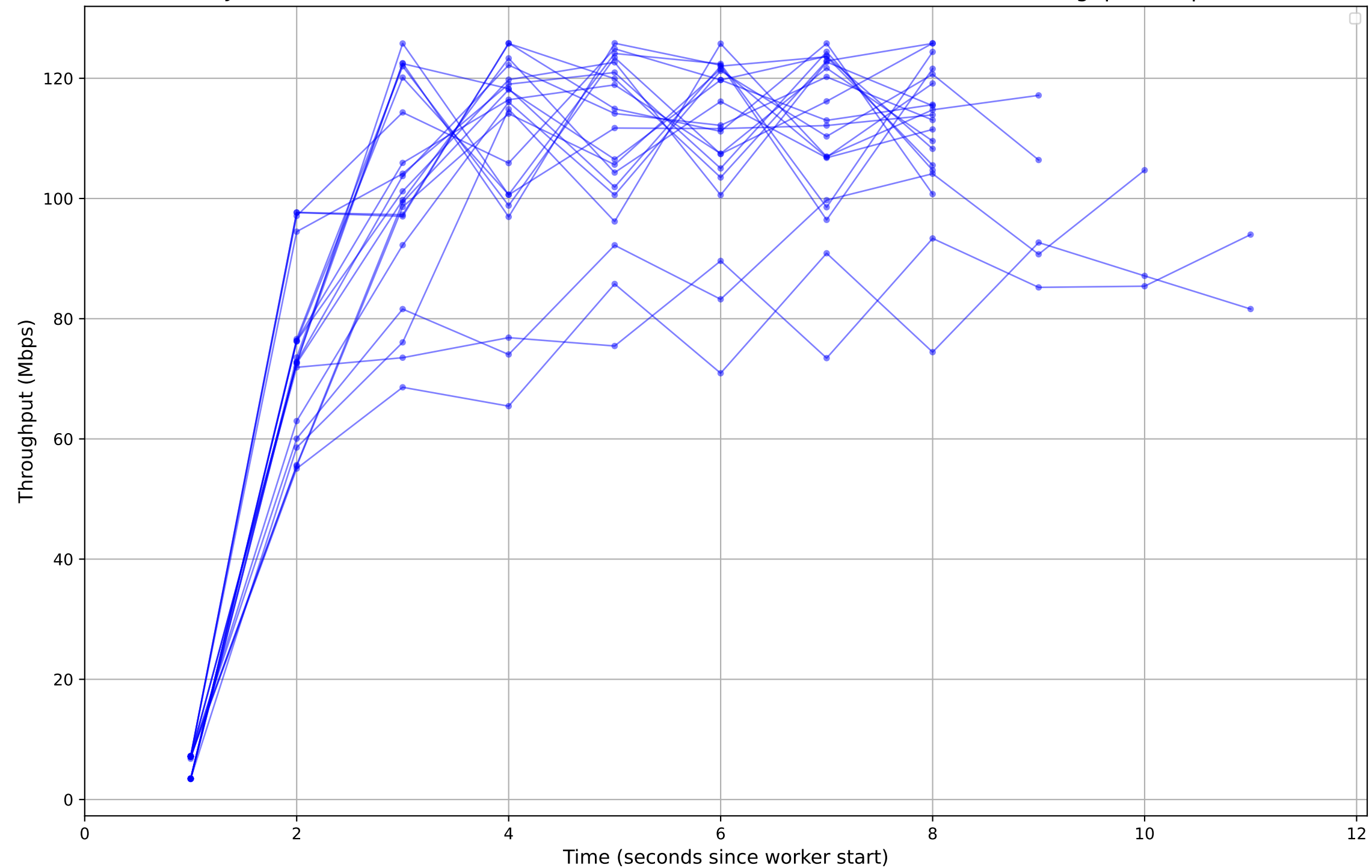
Job ID: 4092d50b-9e15-484d-89f1-56a49edc2eeb - Individual Worker Throughput (Mbps)
