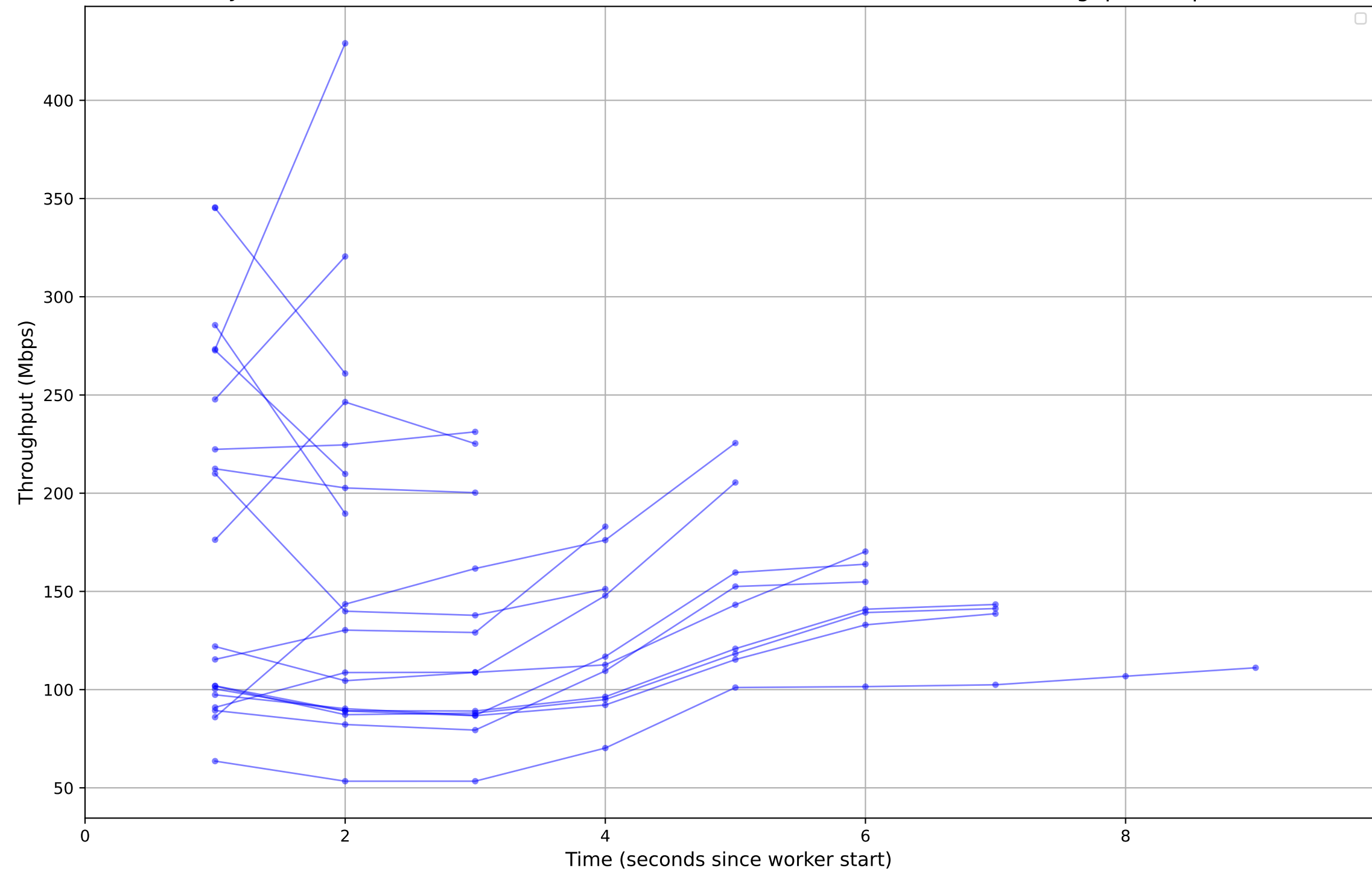
Job ID: 56bba3ef-1420-4874-9f21-c624d27a7066 - Individual Worker Throughput (Mbps)
