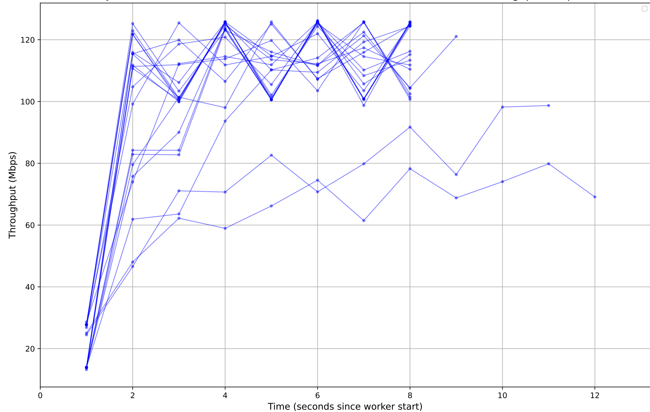
Job ID: 27c30a3a-e893-4d49-a059-691a9c68d28a - Individual Worker Throughput (Mbps)
