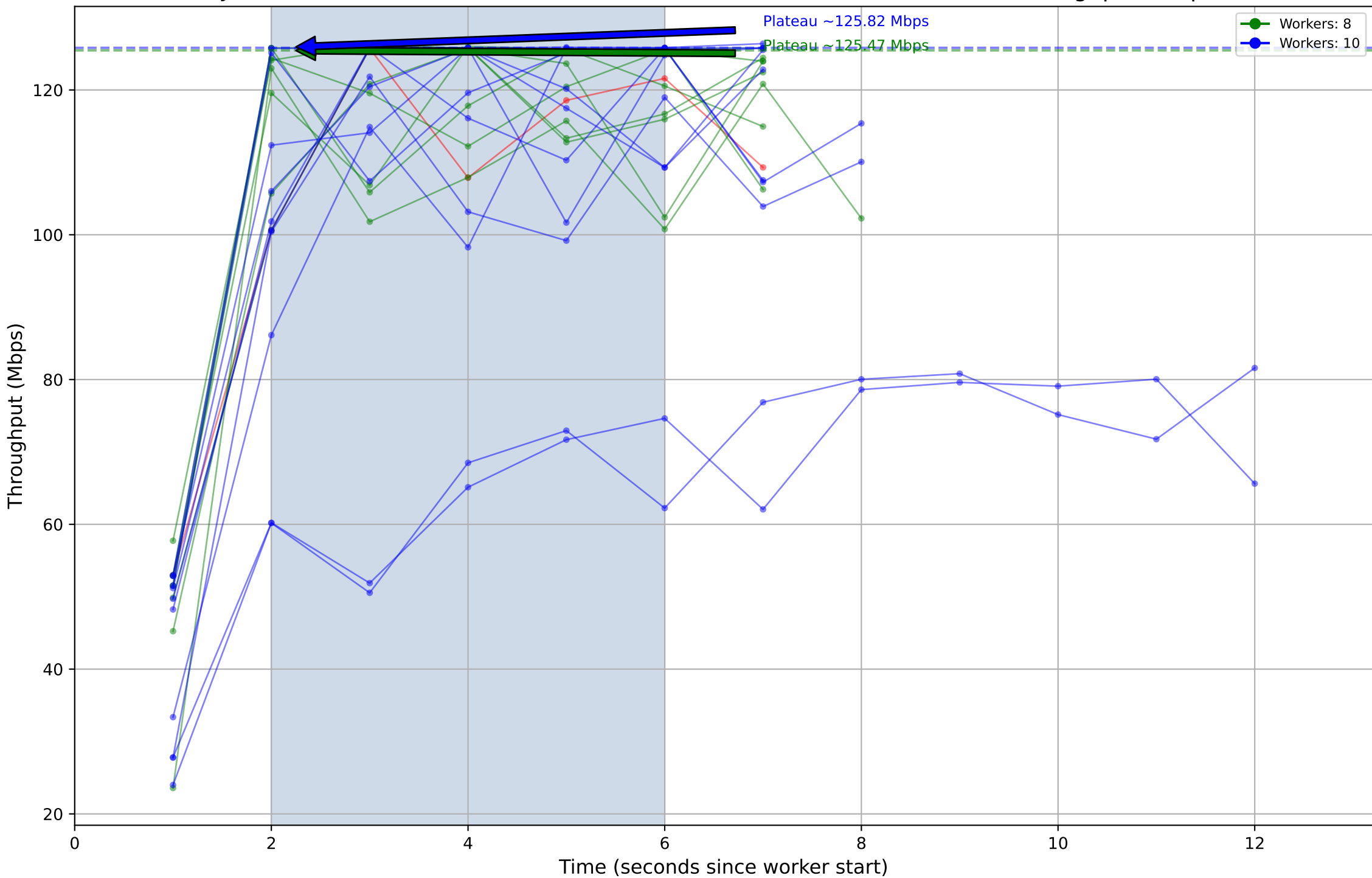
Job ID: 61828f8a-b2fc-4800-b817-544c6b0e8d55 - Individual Worker Throughput (Mbps)
