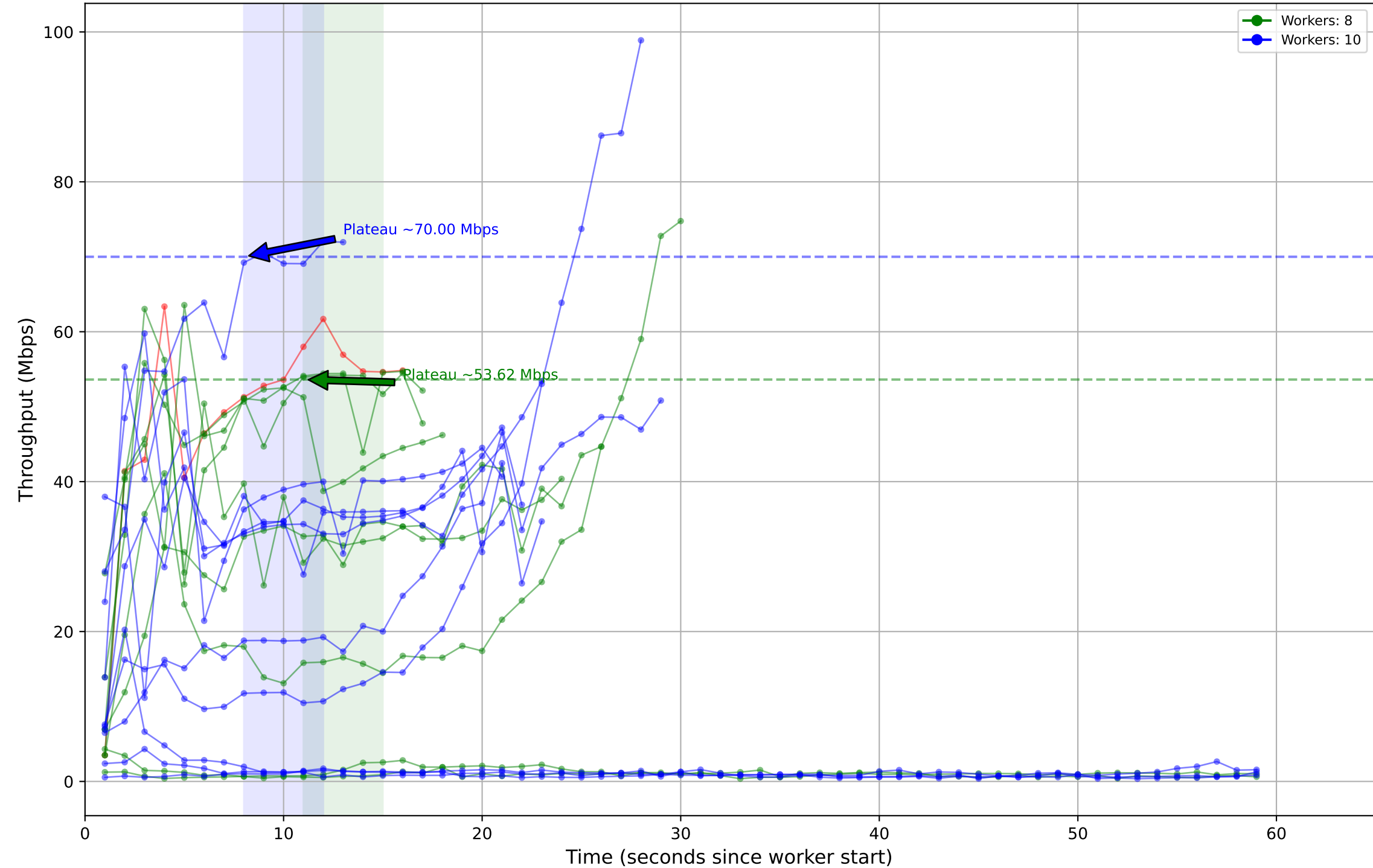
Job ID: 40f92fe0-aa82-402f-8fce-9486841745aa - Individual Worker Throughput (Mbps)
