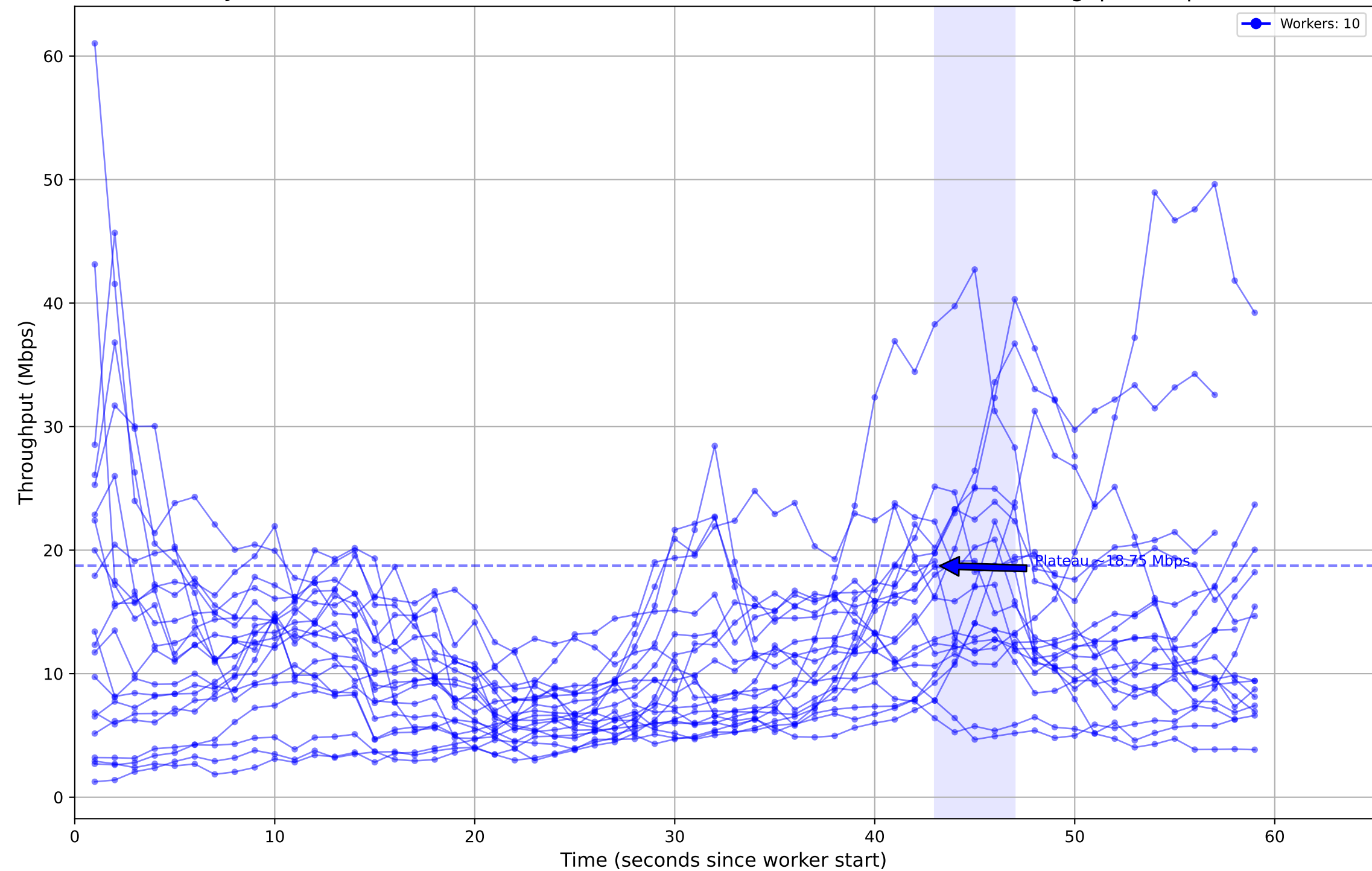
Job ID: 731ce9e9-cbd9-4ece-952c-de4b5897cb0f - Individual Worker Throughput (Mbps)
