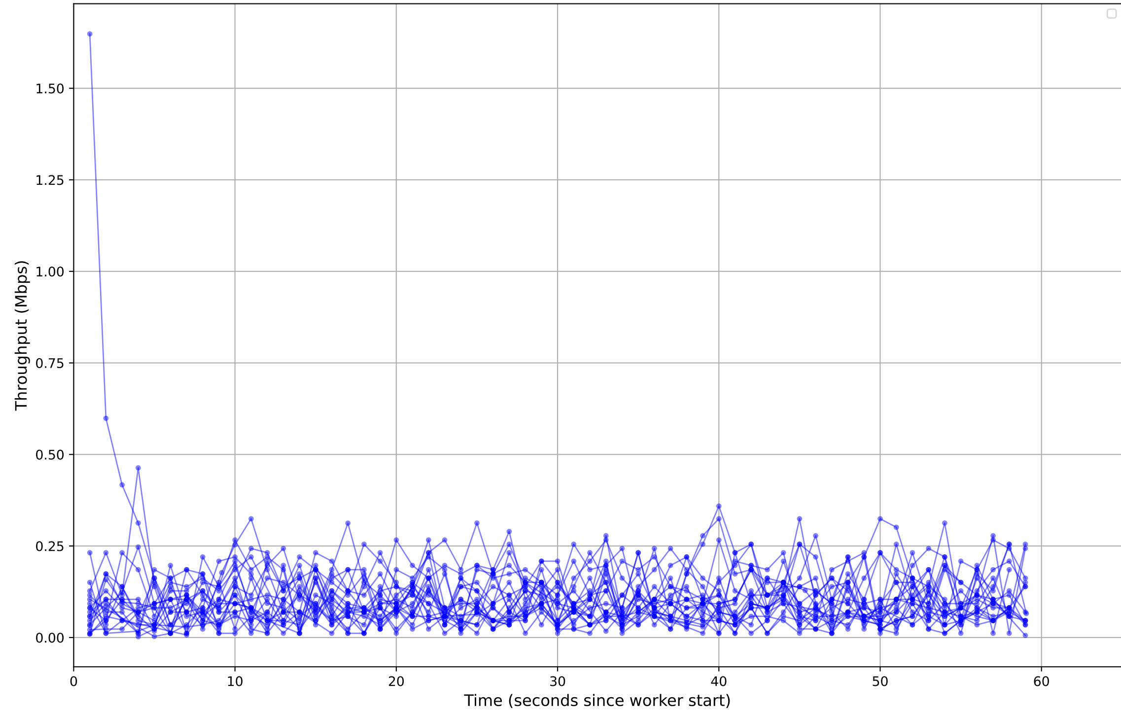
Job ID: 0b9b7cf0-c0ee-405a-8ed4-a11bba457525 - Individual Worker Throughput (Mbps)
