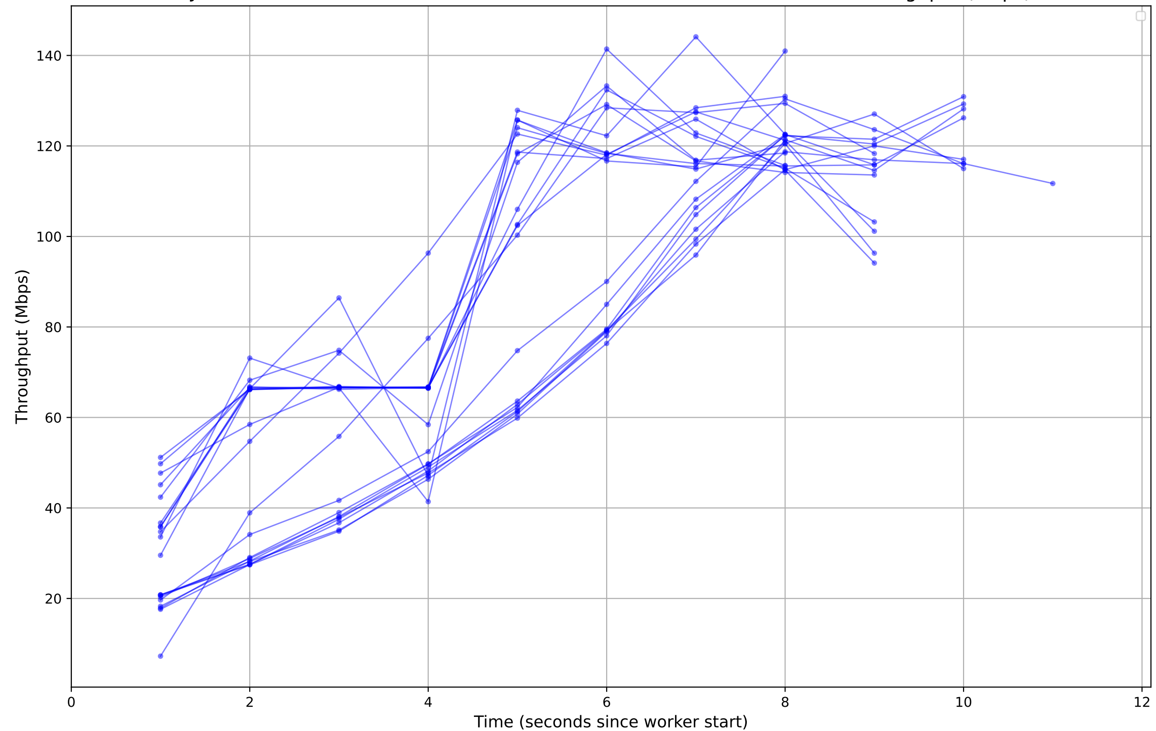
Job ID: 6cdcf5d0-a6db-4be1-b758-5789b32b4237 - Individual Worker Throughput (Mbps)
