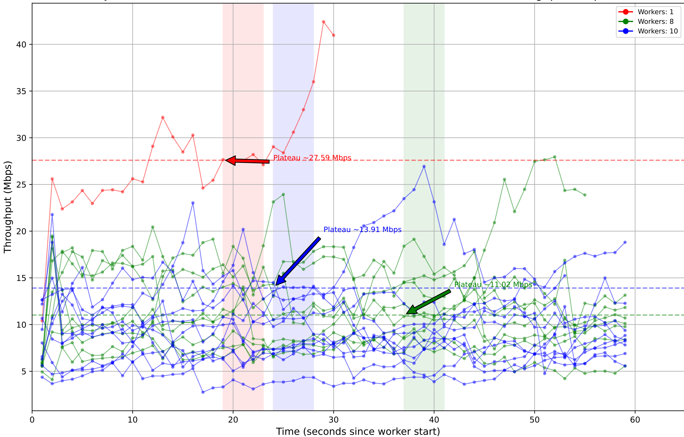
Job ID: 63ca3798-7166-4b9c-8859-ae752135a259 - Individual Worker Throughput (Mbps)
