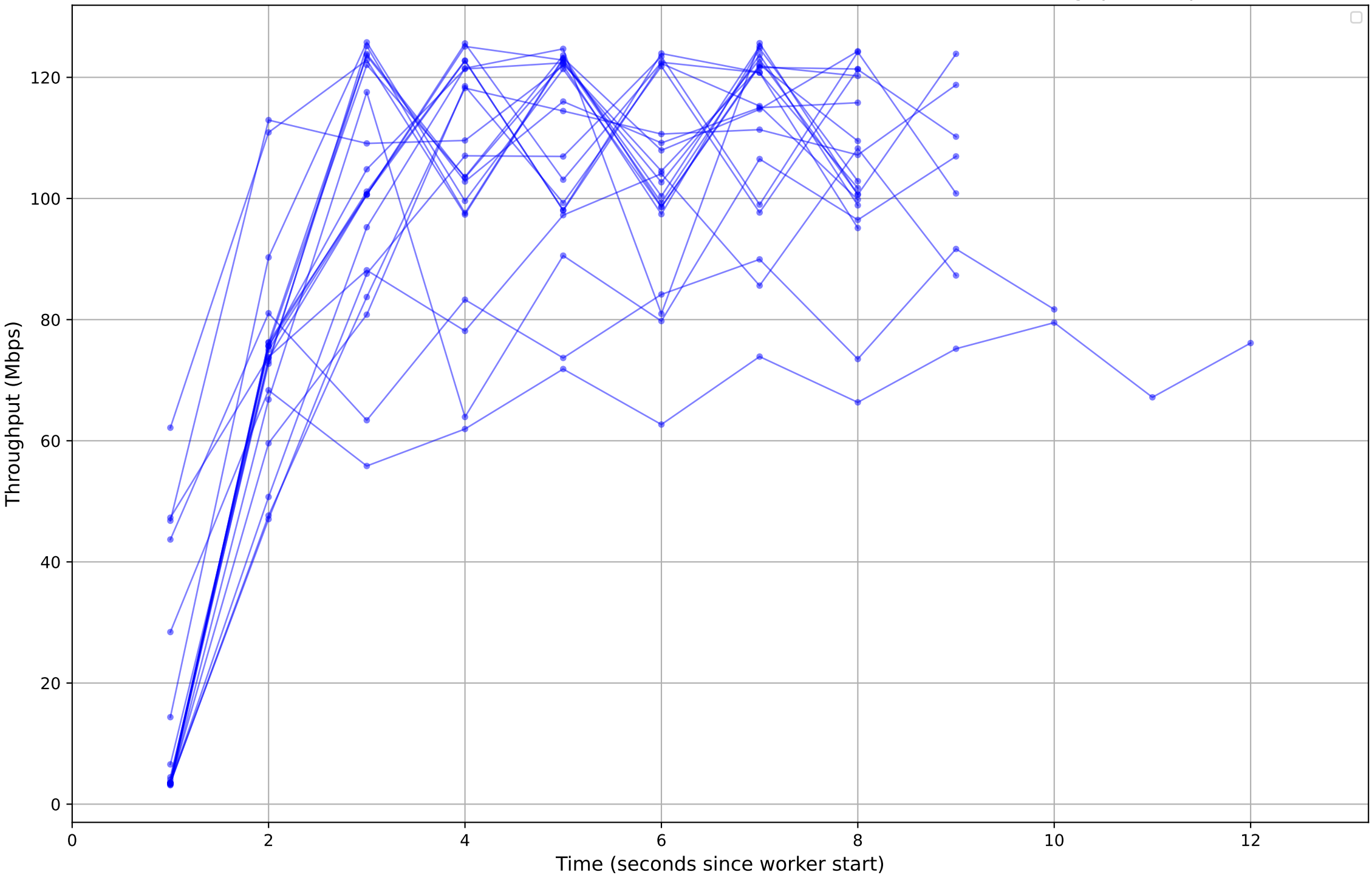
Job ID: 7eb3d672-9c08-4a15-97ec-49b5dbfc2946 - Individual Worker Throughput (Mbps)
