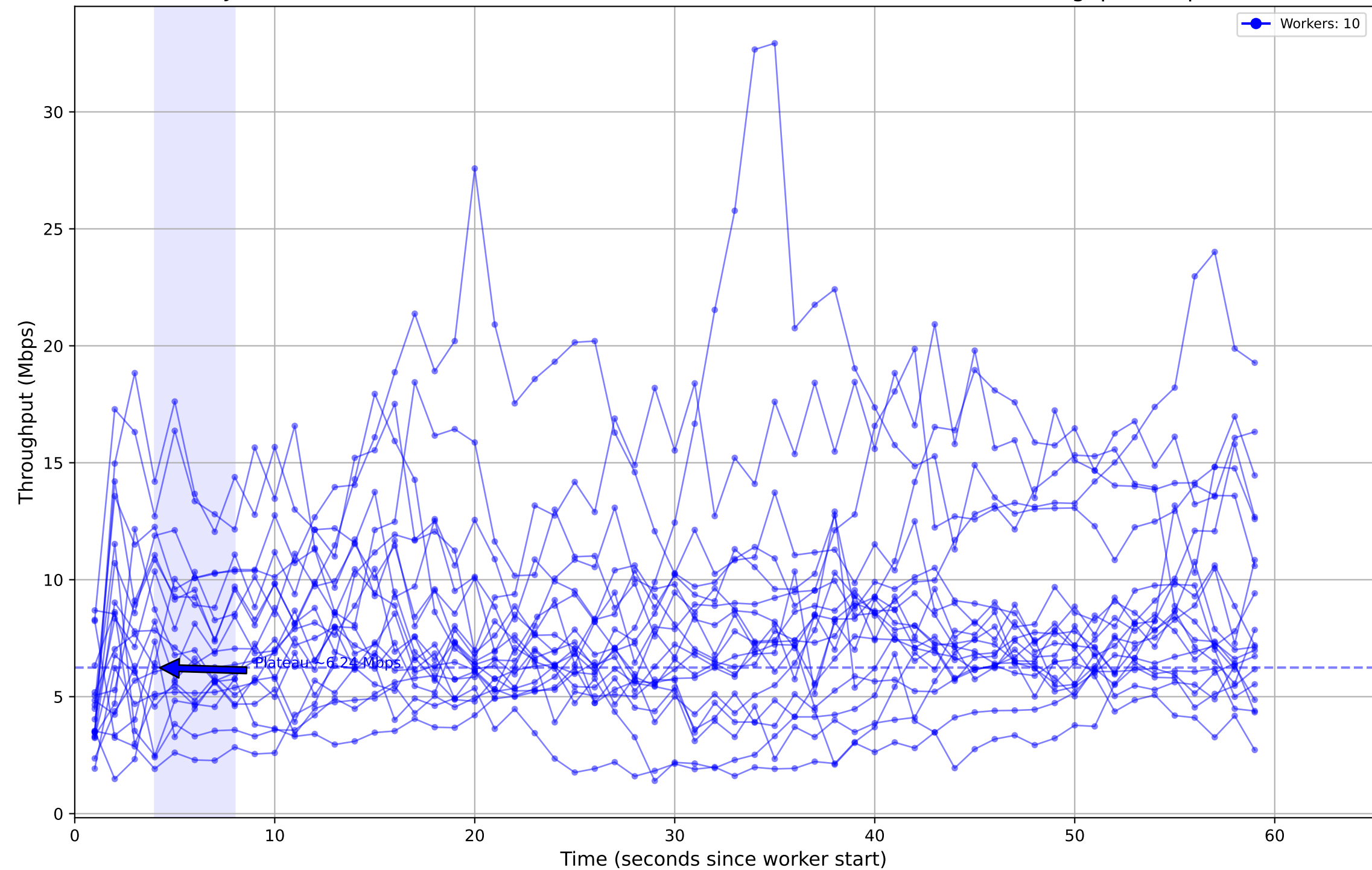
Job ID: bd910975-9ade-47d6-9e2f-edf9e2d49234 - Individual Worker Throughput (Mbps)
