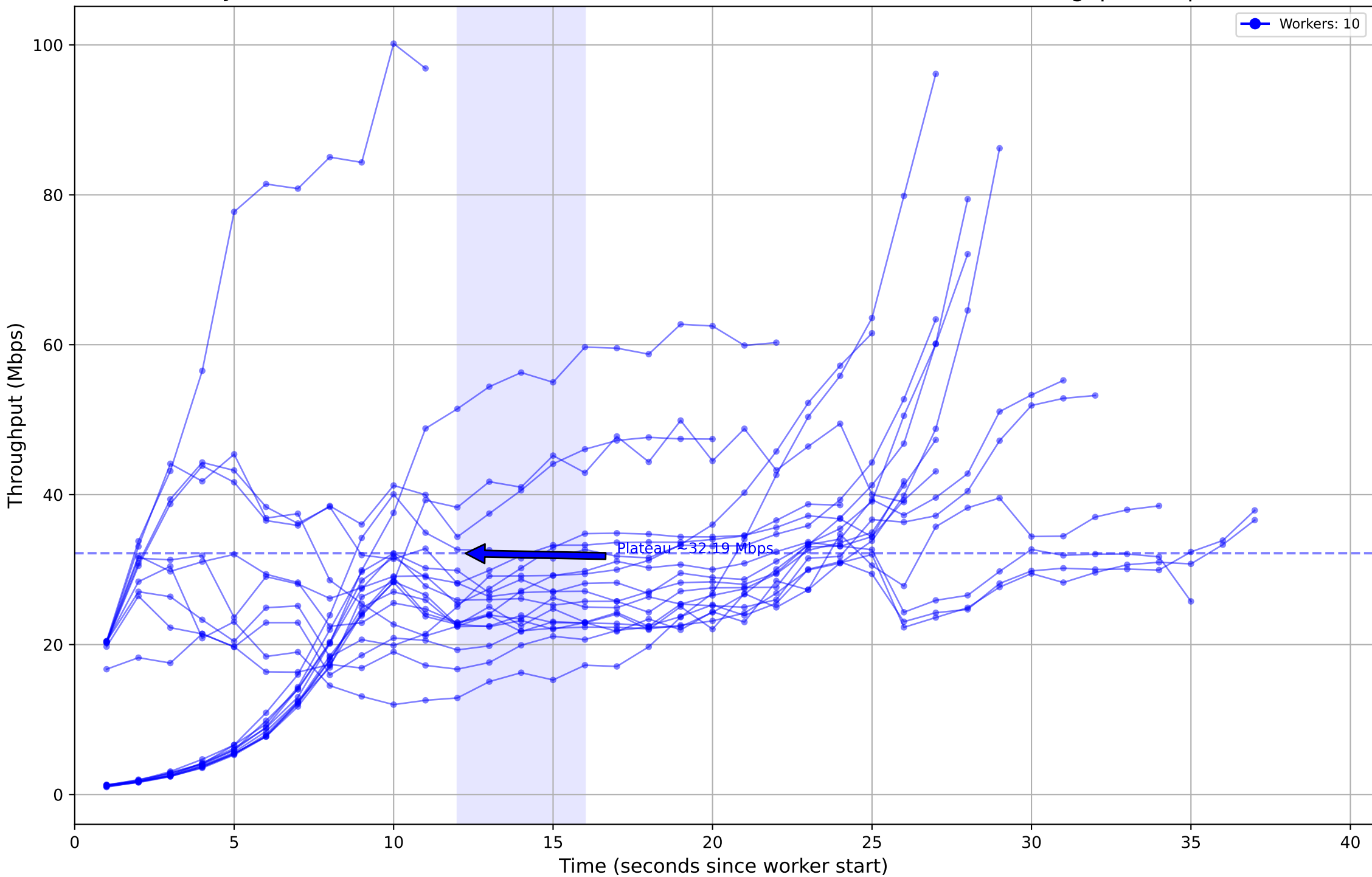
Job ID: ad3b74ec-c767-4b8c-94d6-f07cf3742c43 - Individual Worker Throughput (Mbps)
