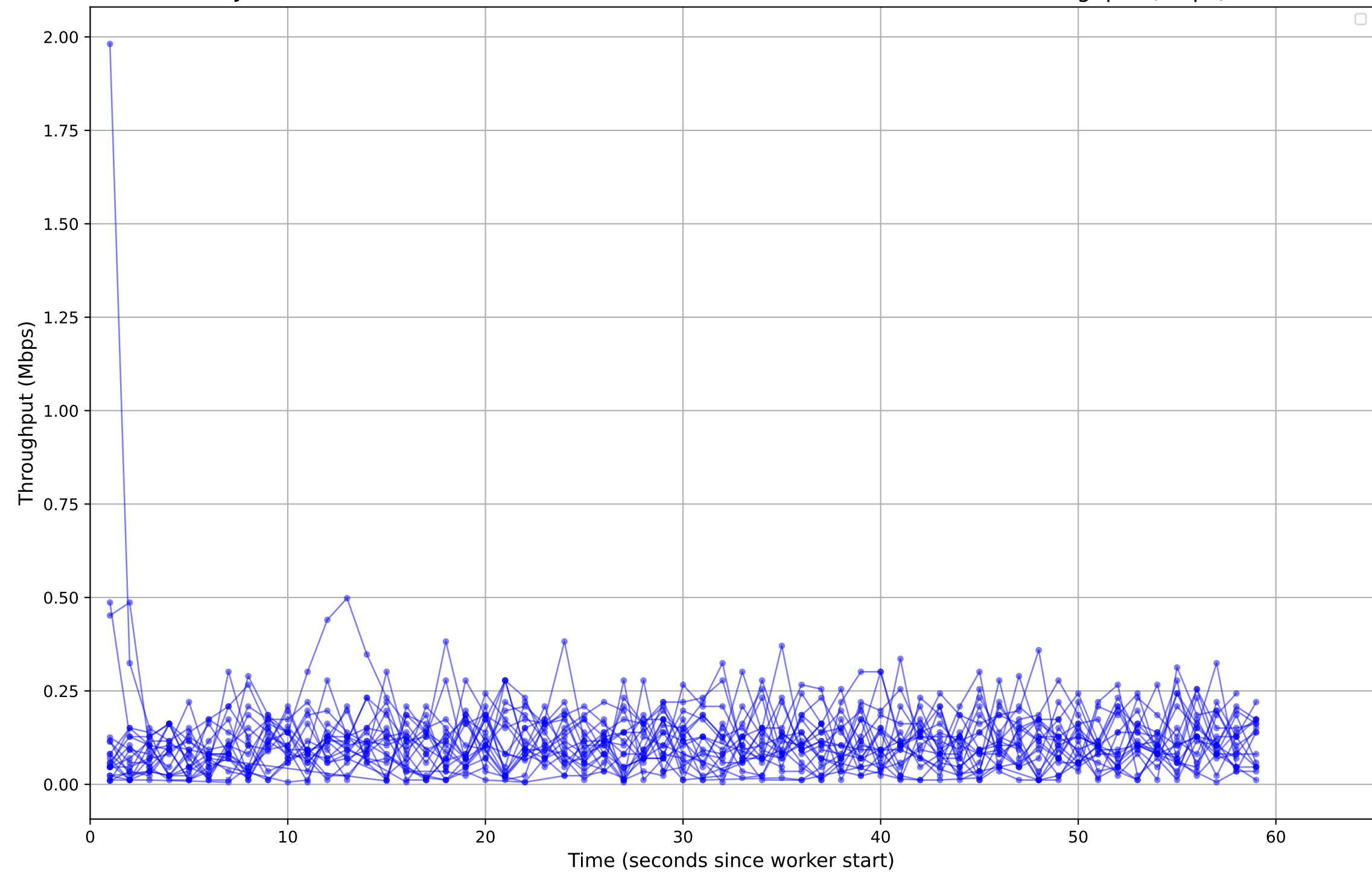
Job ID: c2c89732-9315-4011-83df-e7531f6a0c2e - Individual Worker Throughput (Mbps)
