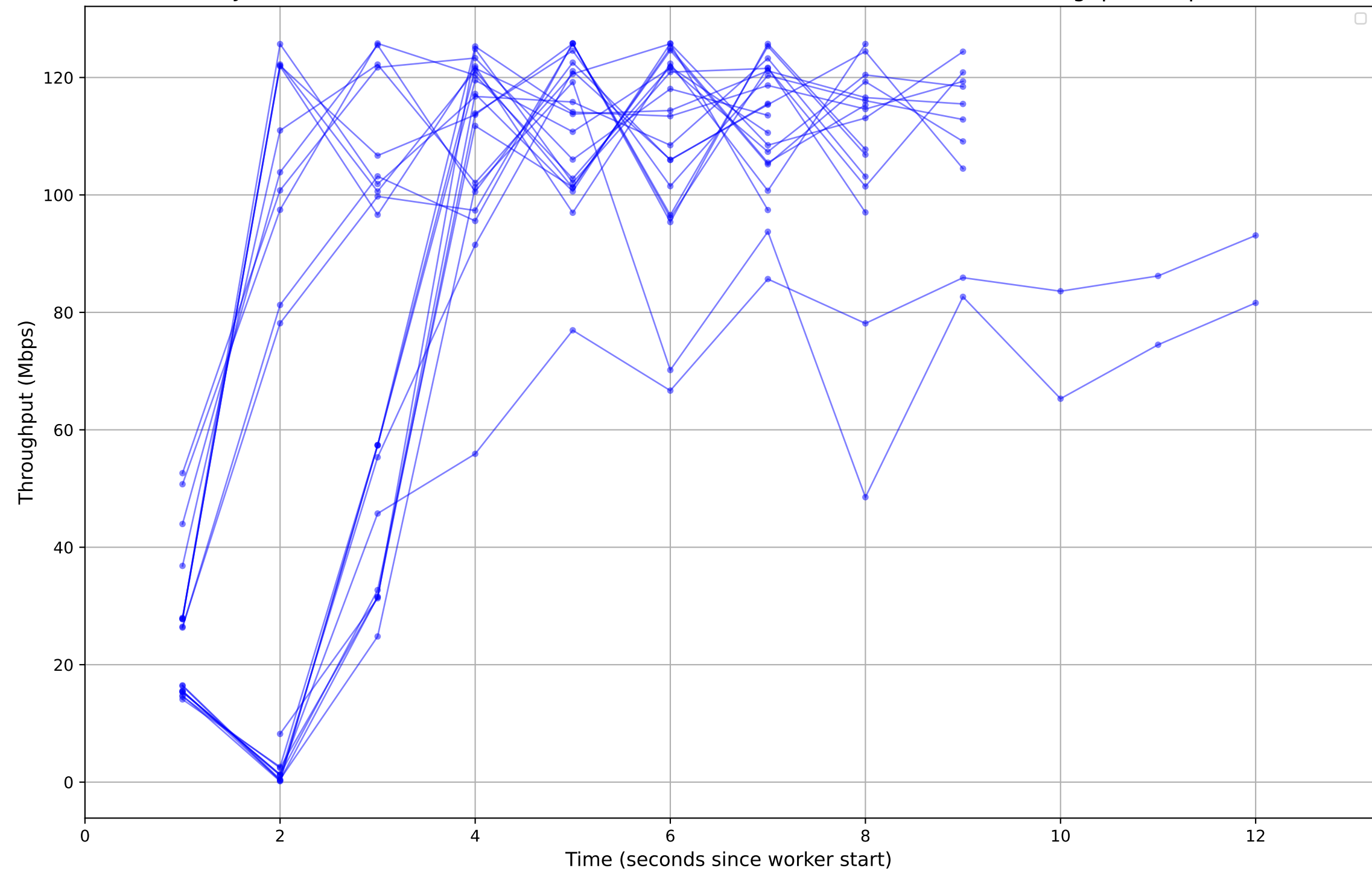
Job ID: 06fa6c3f-bd69-4e21-aea5-3b30c758cdac - Individual Worker Throughput (Mbps)
