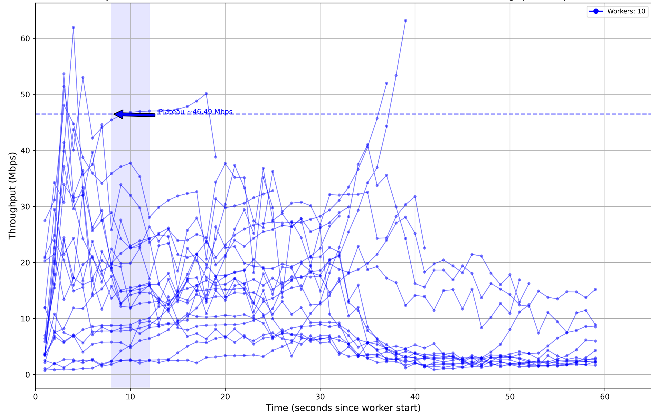
Job ID: aafdc19e-7c35-4413-8c84-5e70a28b0c97 - Individual Worker Throughput (Mbps)
