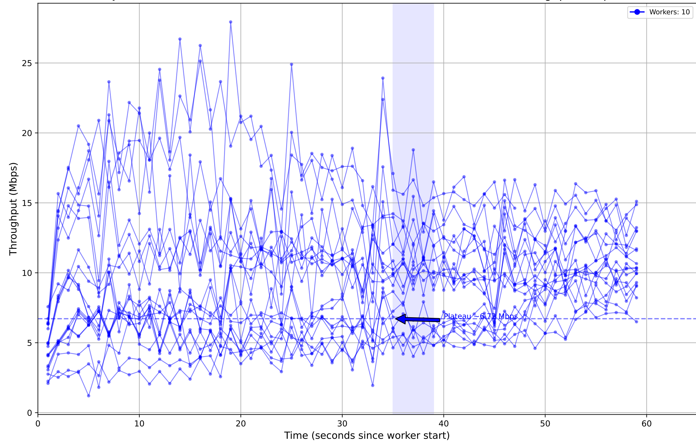
Job ID: 6fdc8043-0101-450a-9733-5a5c54de69e0 - Individual Worker Throughput (Mbps)
