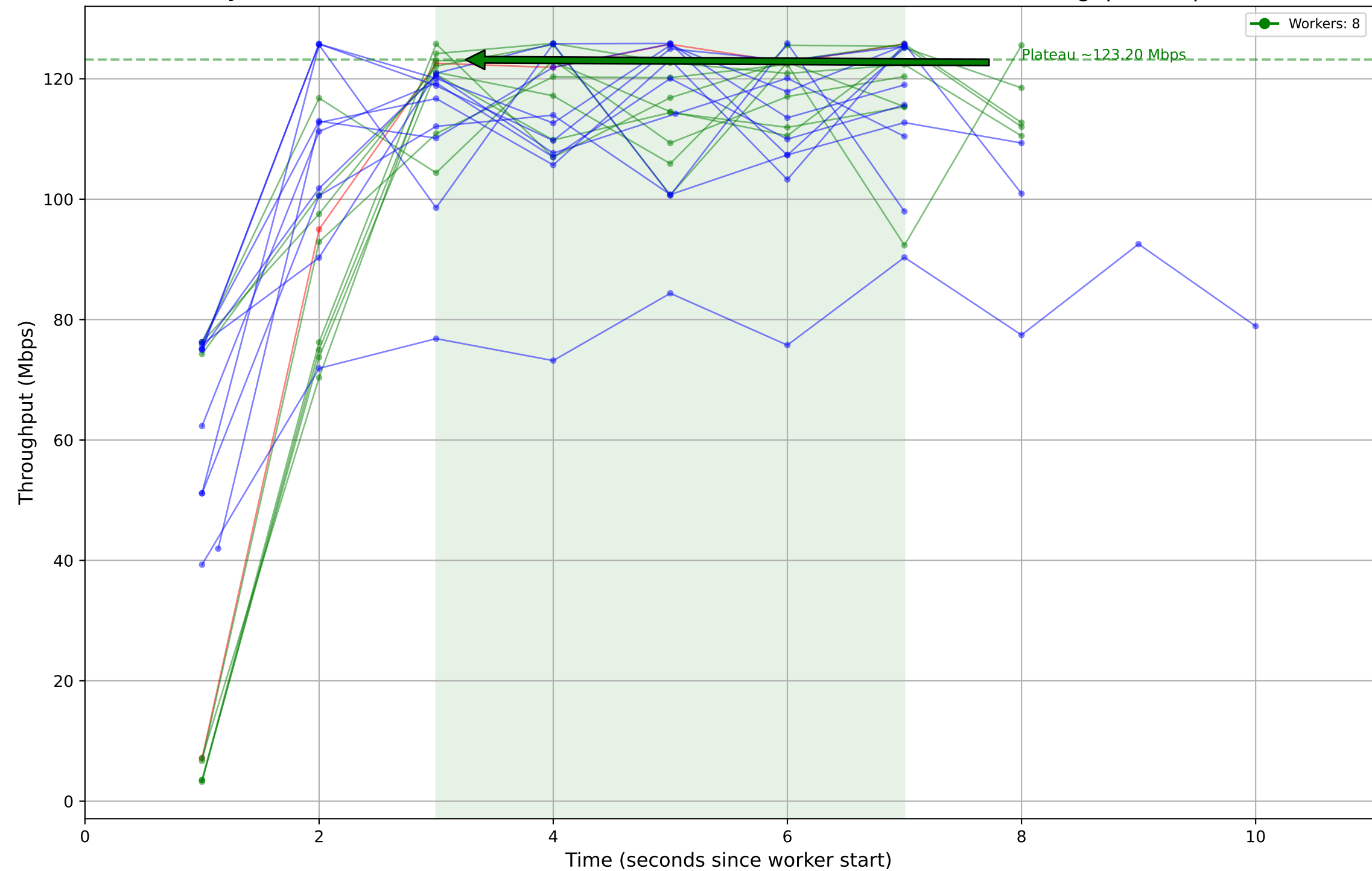
Job ID: 4e39288f-028a-4649-8ddc-2846acceb89e - Individual Worker Throughput (Mbps)
