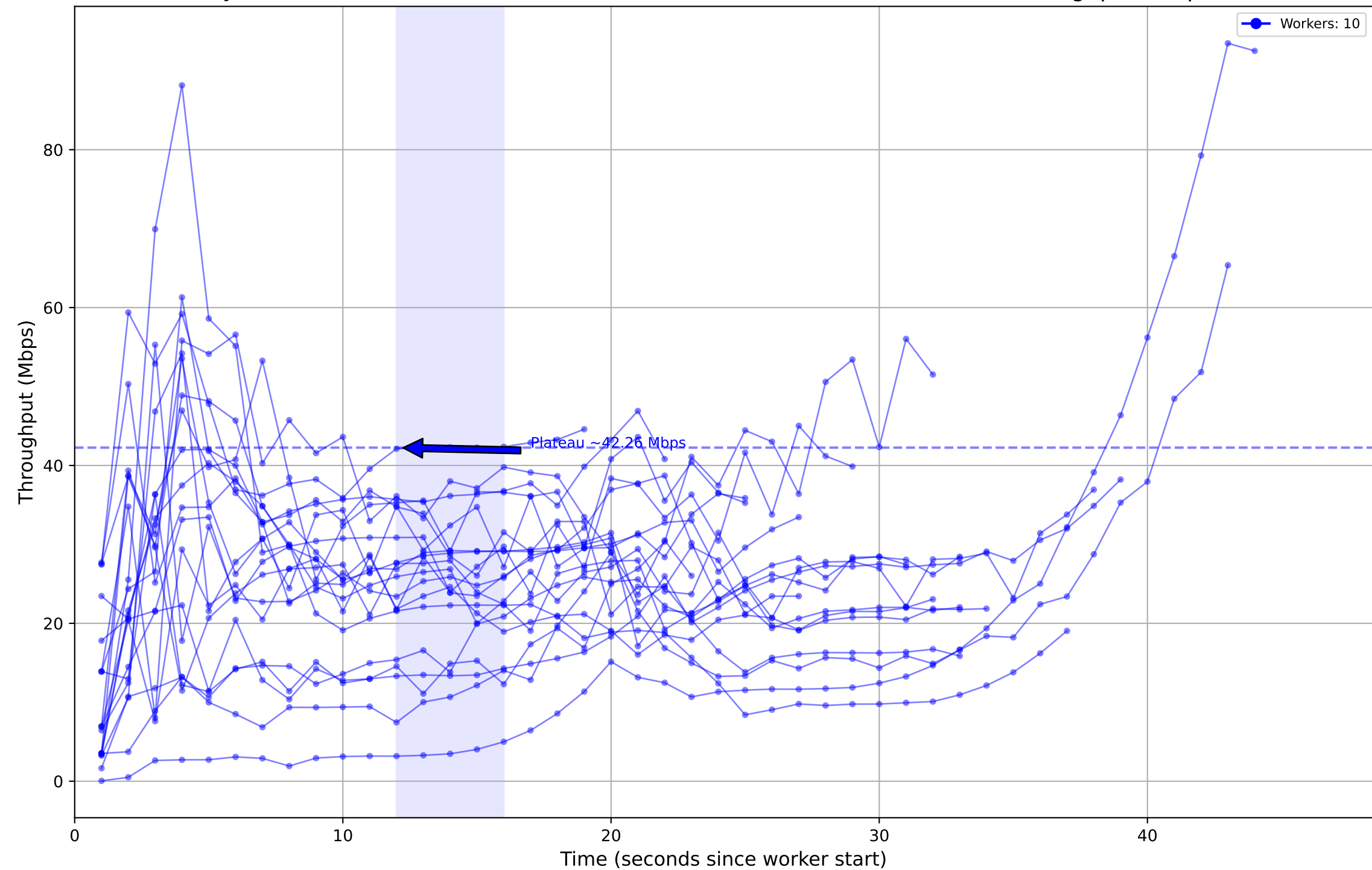
Job ID: 75ab2357-a408-40d4-b6ae-8b15df90c15f - Individual Worker Throughput (Mbps)
