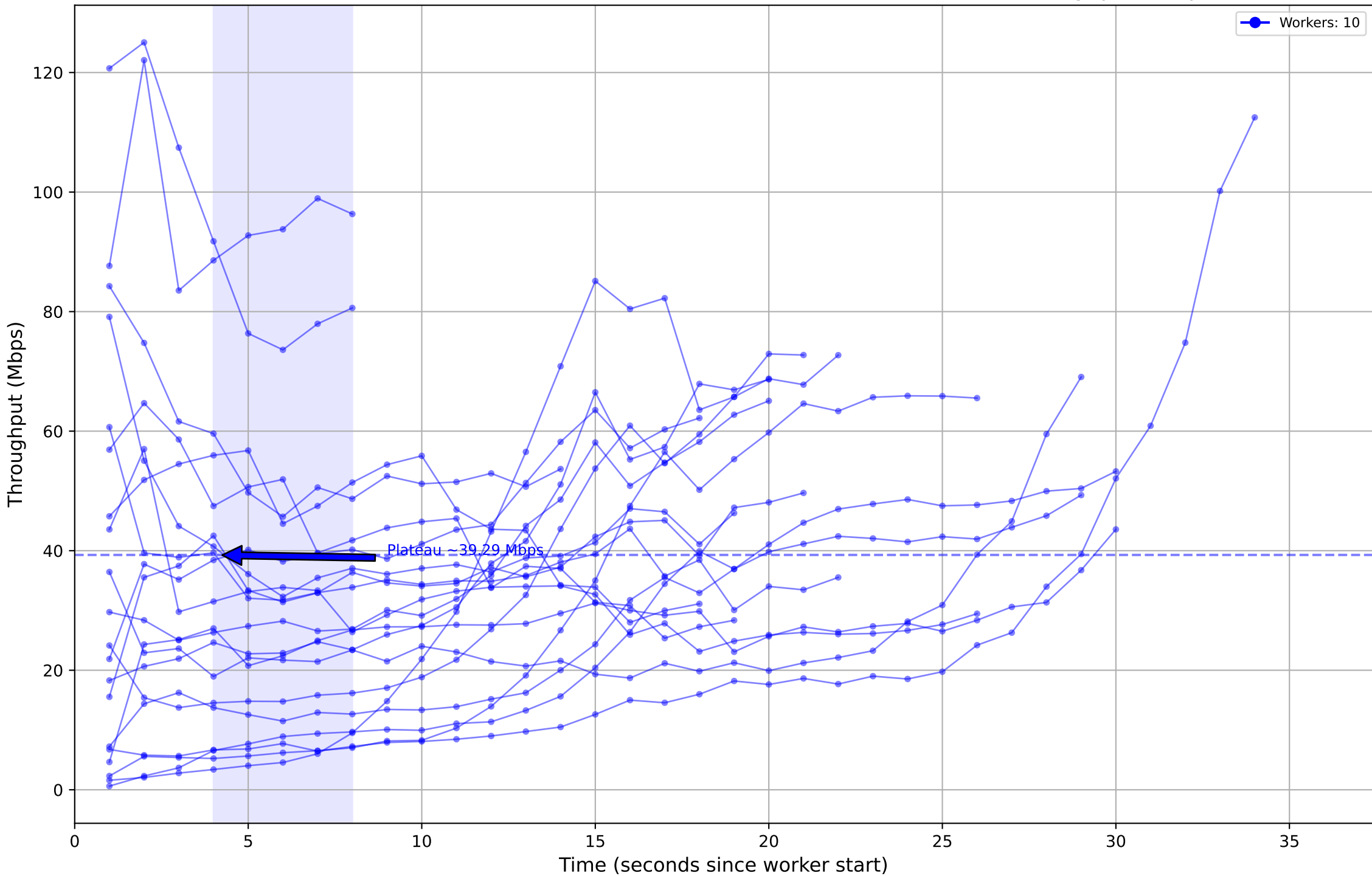
Job ID: 8dbdf583-3975-4f29-8294-c6068b3f6278 - Individual Worker Throughput (Mbps)
