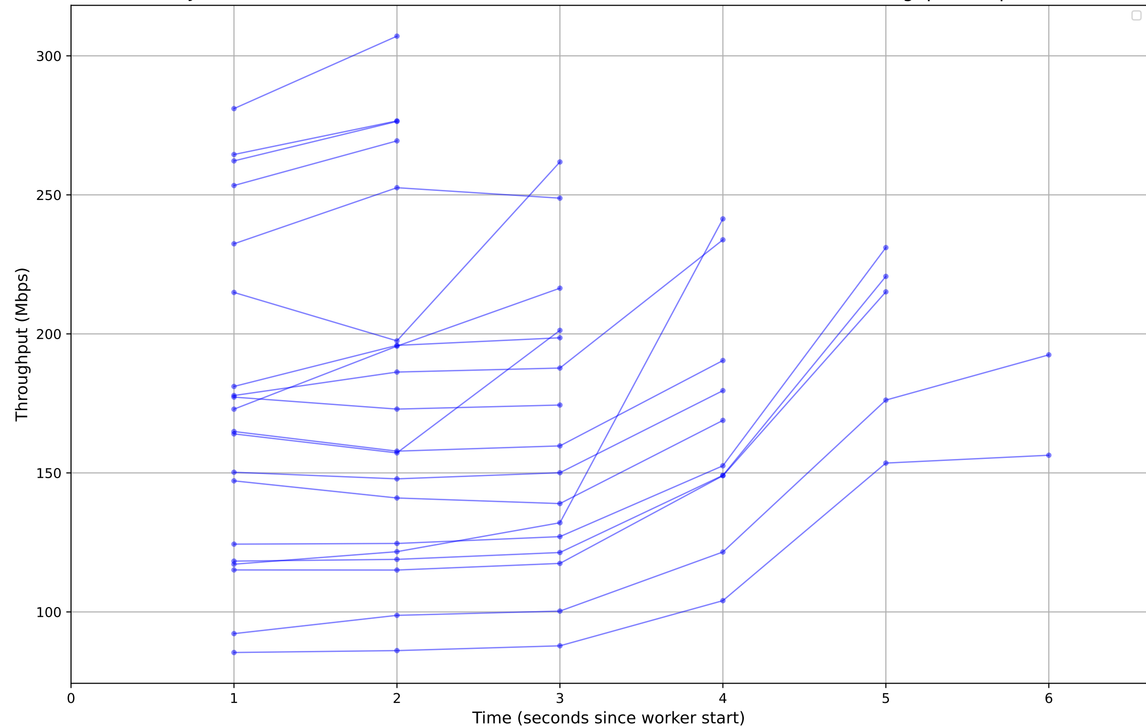
Job ID: 764df5aa-ae55-46db-b185-6d43be3bd179 - Individual Worker Throughput (Mbps)
