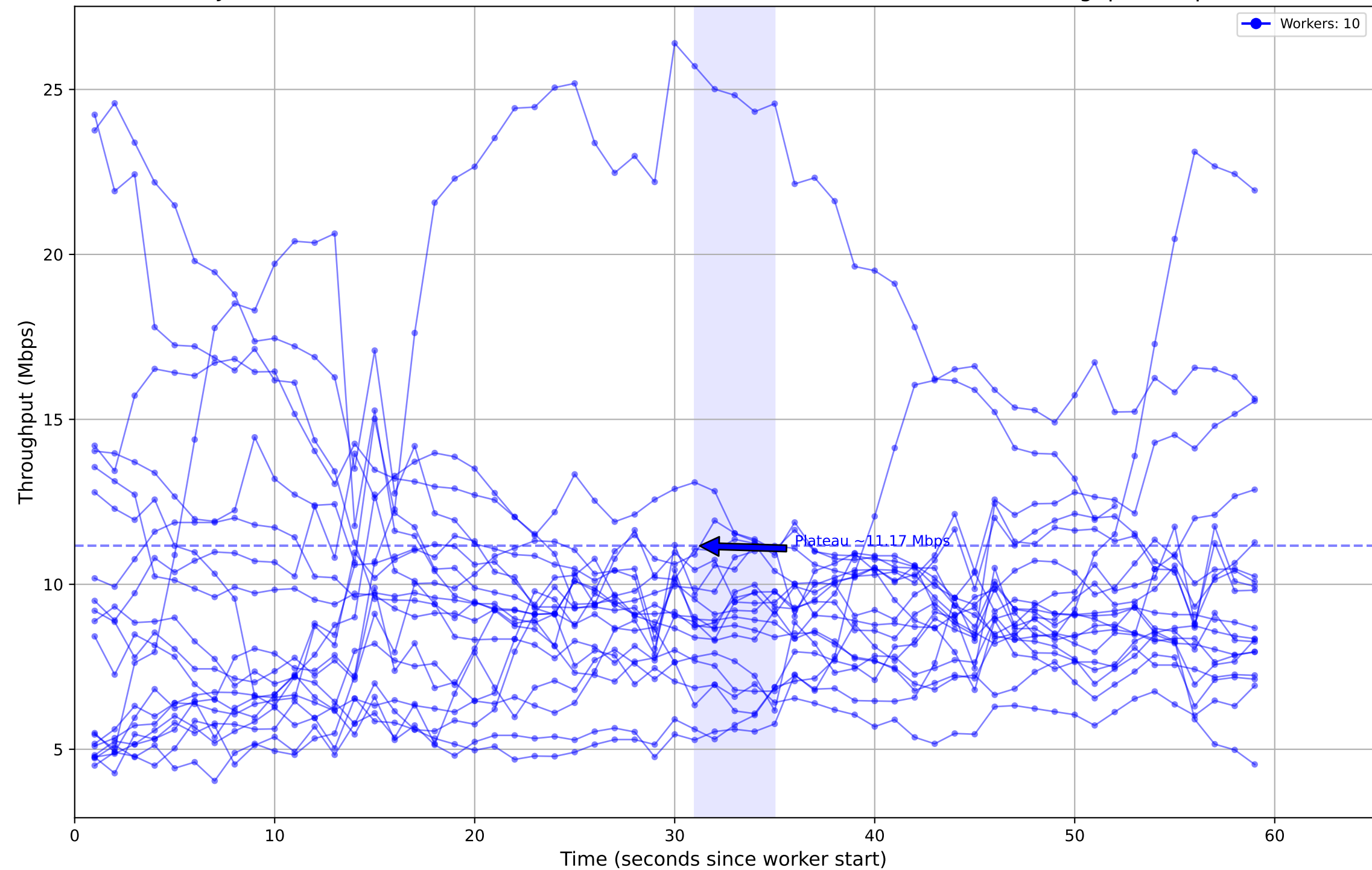
Job ID: e1032366-5276-4375-9262-a854b777054e - Individual Worker Throughput (Mbps)
