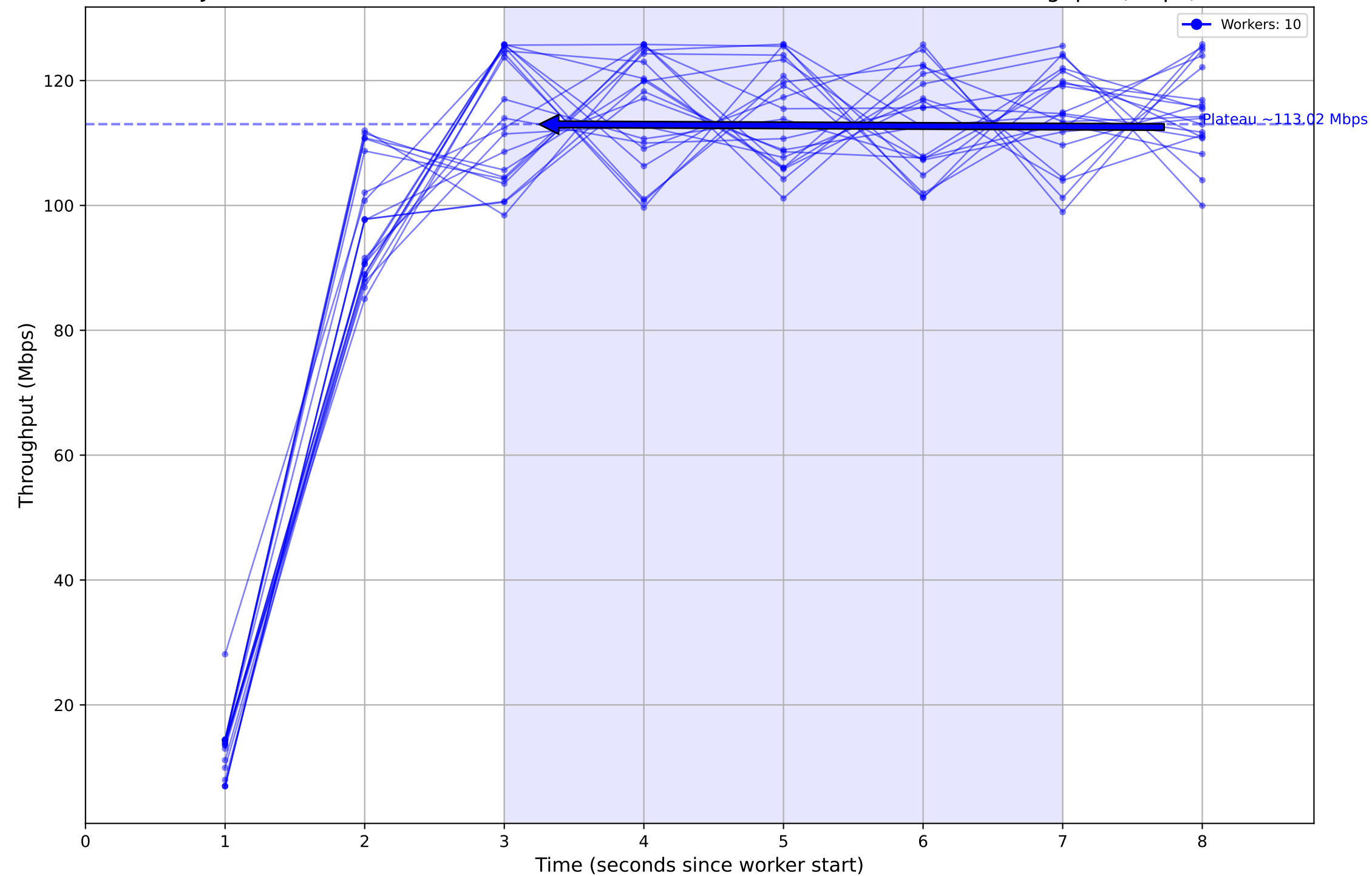
Job ID: 1555dffd-62cd-4024-bed5-42a0b2a4e0f7 - Individual Worker Throughput (Mbps)
