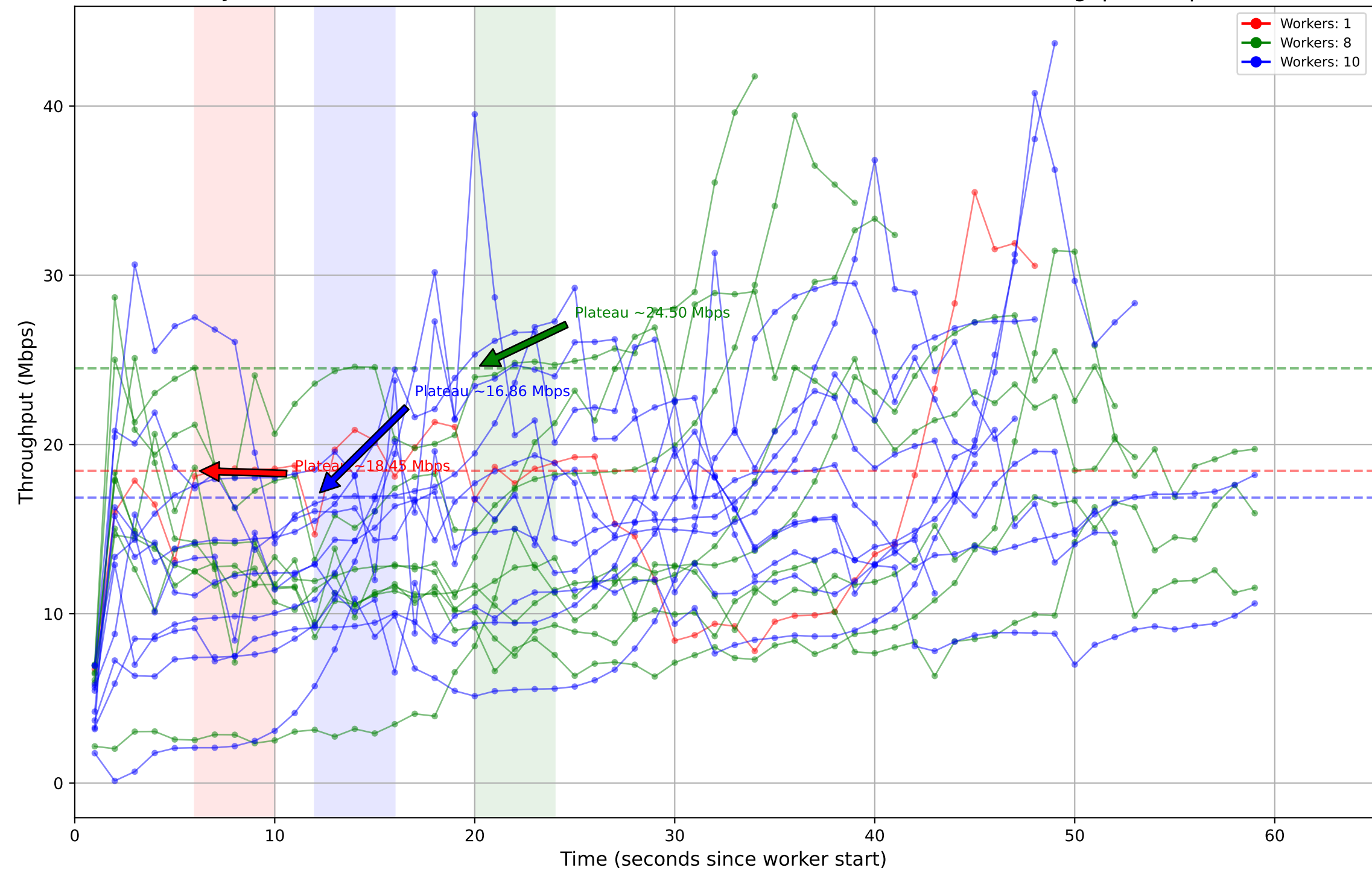
Job ID: ec0779ba-08d3-4e1d-91df-237d310273c6 - Individual Worker Throughput (Mbps)
