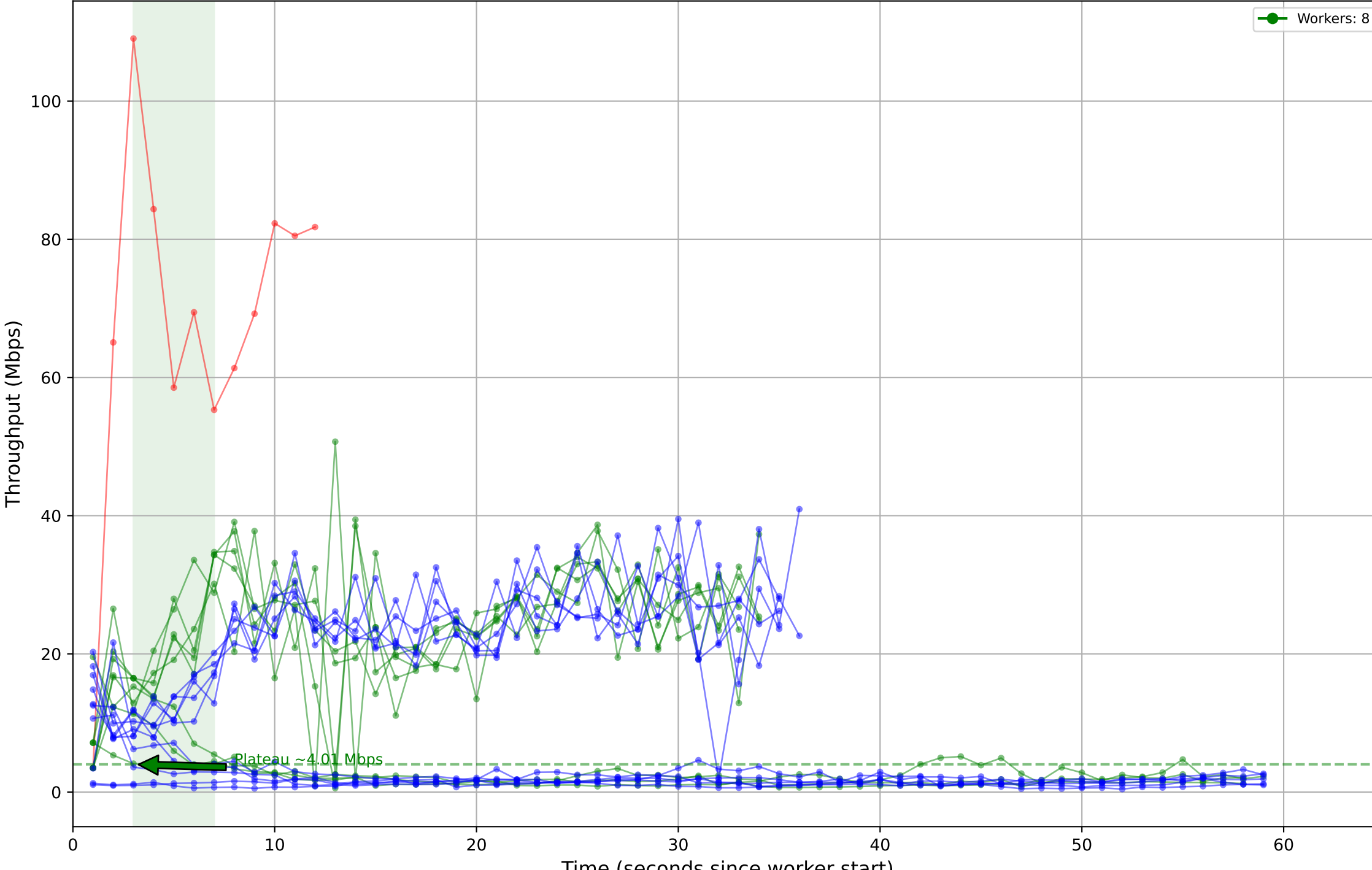
Job ID: 852e3844-8682-4864-8743-eb6cae0cbf31 - Individual Worker Throughput (Mbps)
