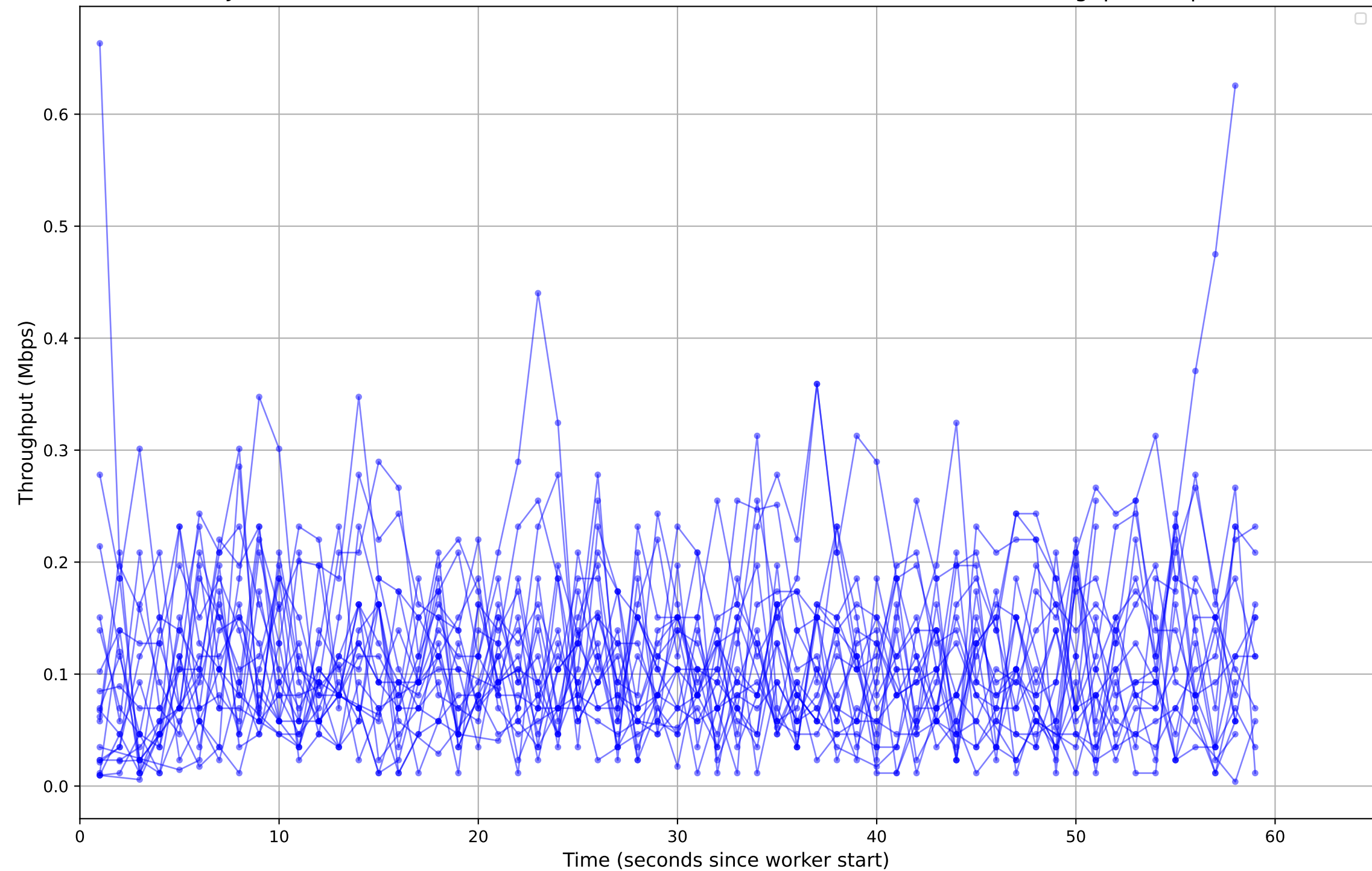
Job ID: 194b6fe7-6294-4564-91f8-63db94c08a87 - Individual Worker Throughput (Mbps)
