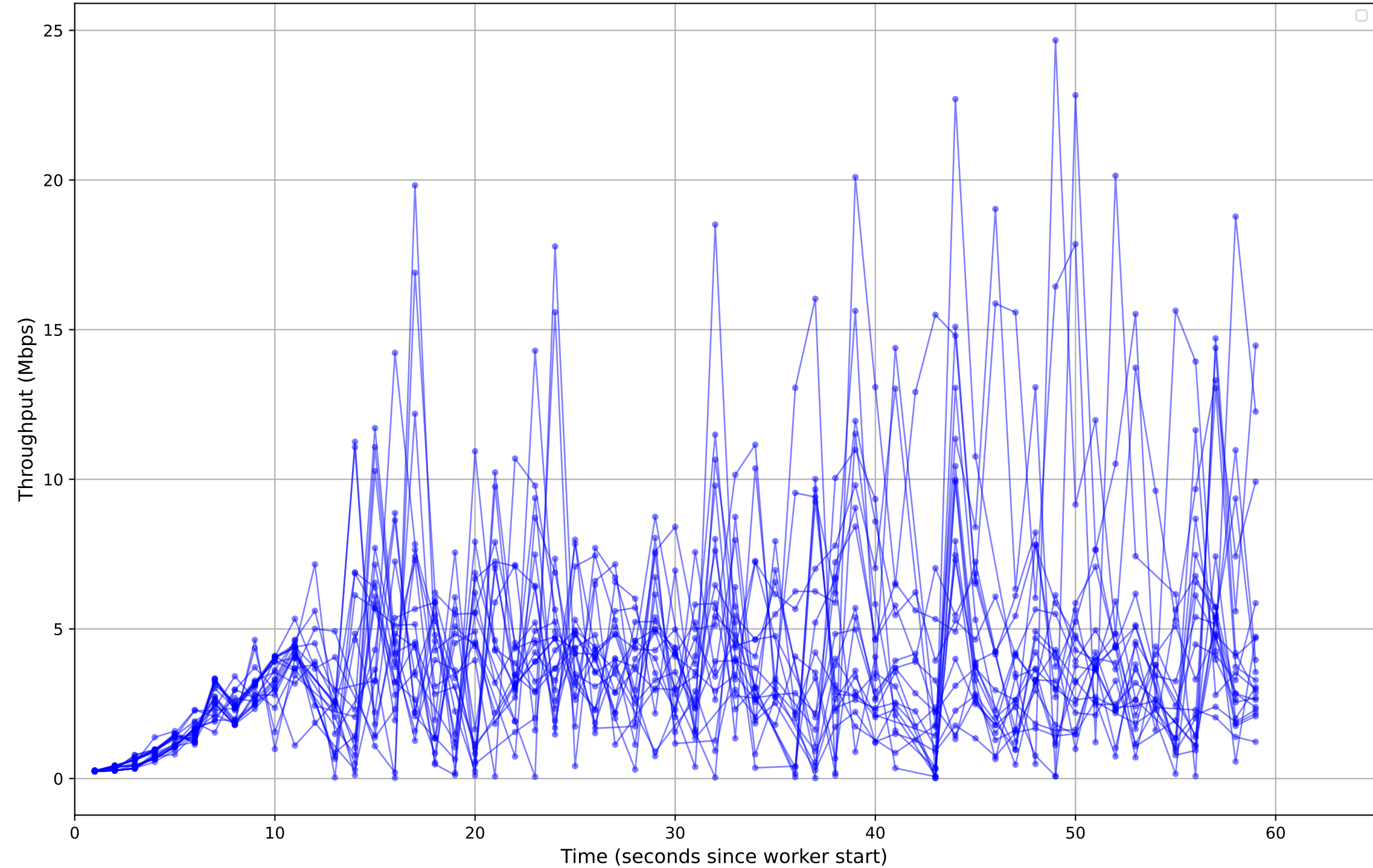
Job ID: db252037-a59c-43f1-adb5-538f5e24fbfd - Individual Worker Throughput (Mbps)
