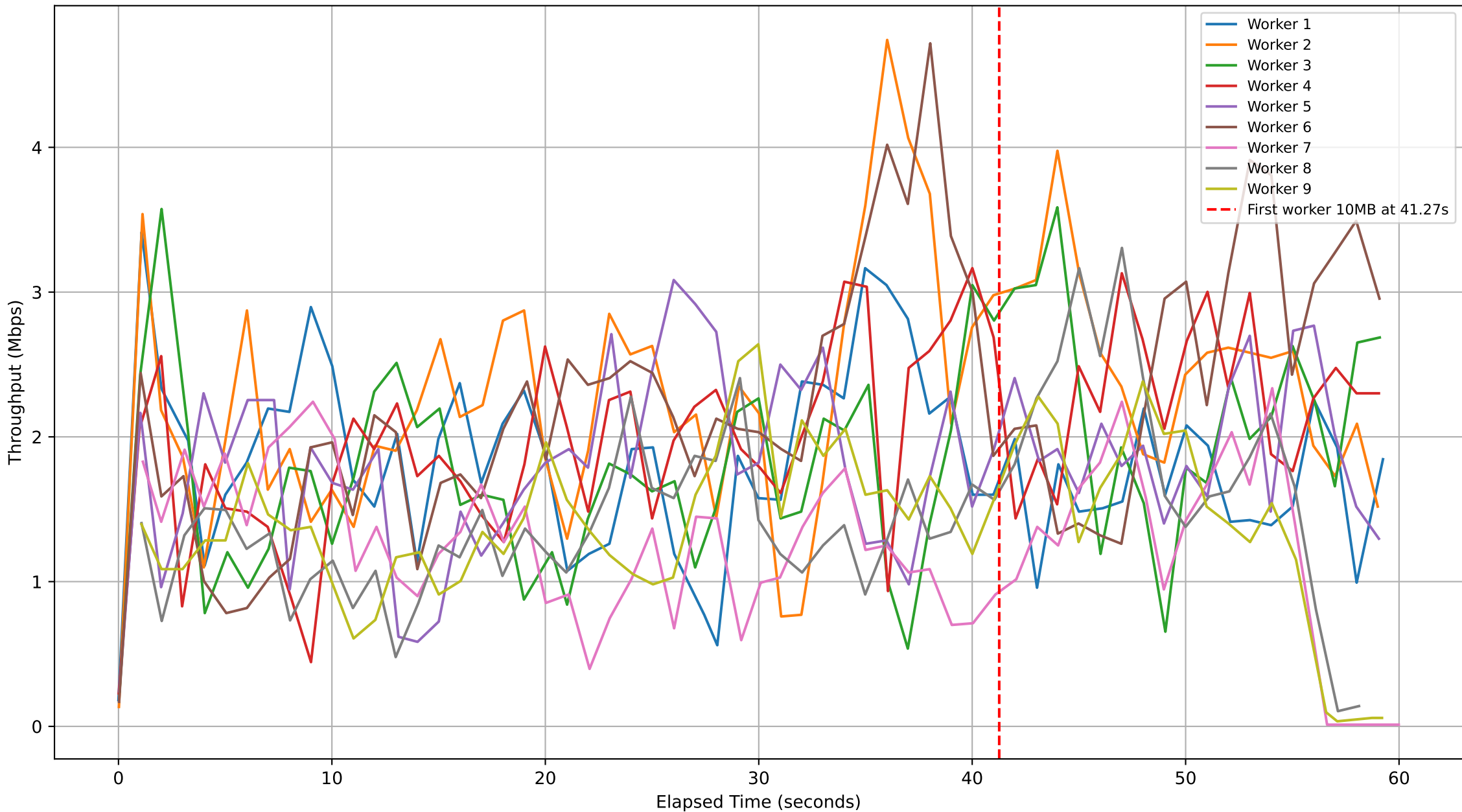
Subjob ID: 86f236b8-bf65-47be-aa7d-f5ba8c6f66b7 - Workers Throughput Over Time
