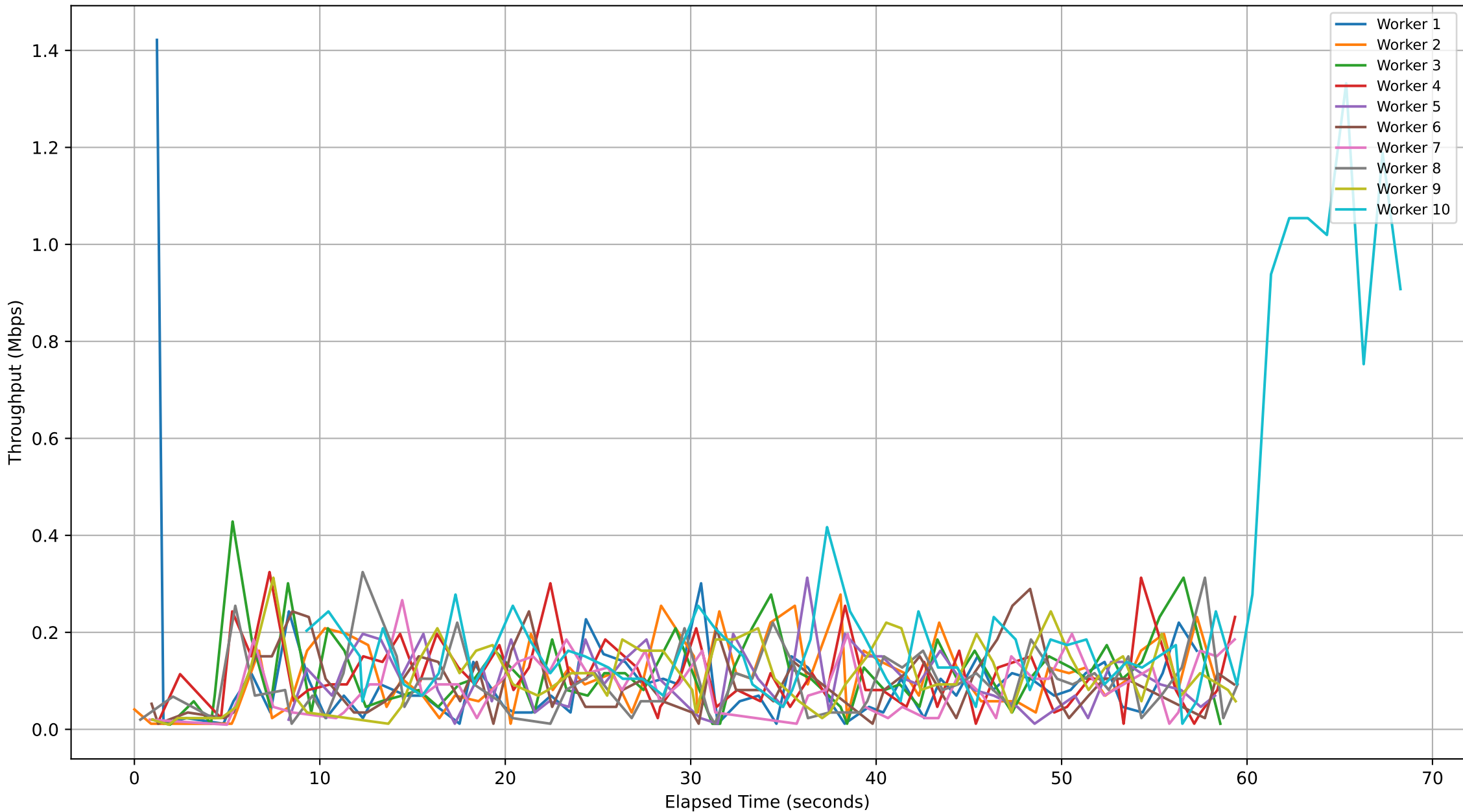
Subjob ID: 300af3e0-149b-4b05-804c-141a221e22ad - Workers Throughput Over Time
