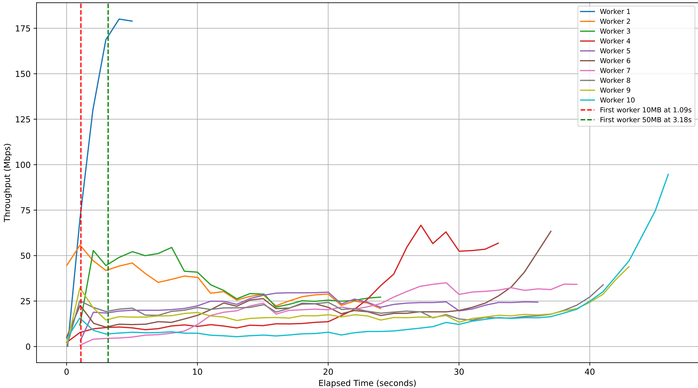
Subjob ID: 95649ddf-e6d1-433c-a1be-b5bfd0a5e0ad - Workers Throughput Over Time
