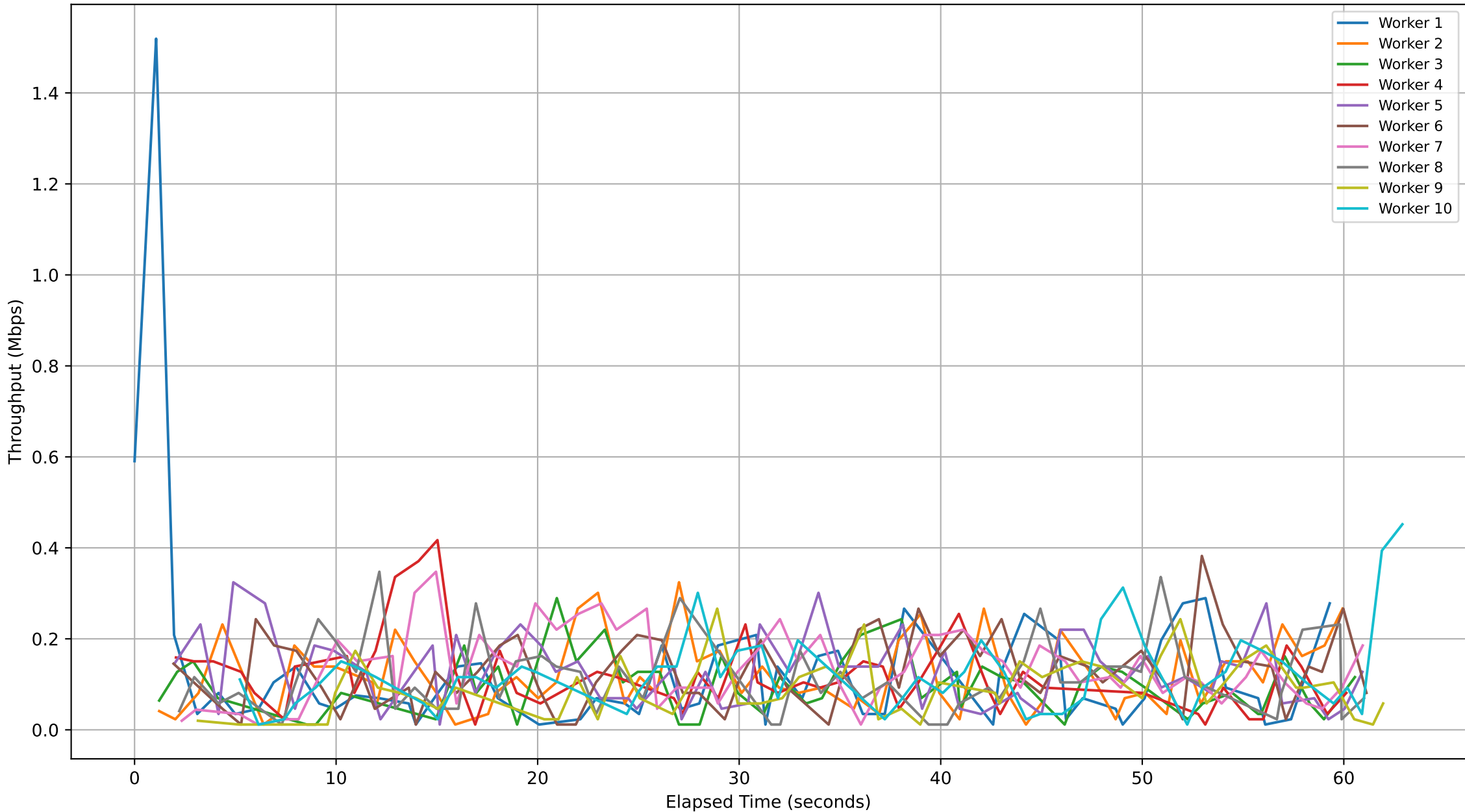
Subjob ID: 3a28f1cc-a632-4240-ac85-7f87e4f0a157 - Workers Throughput Over Time
