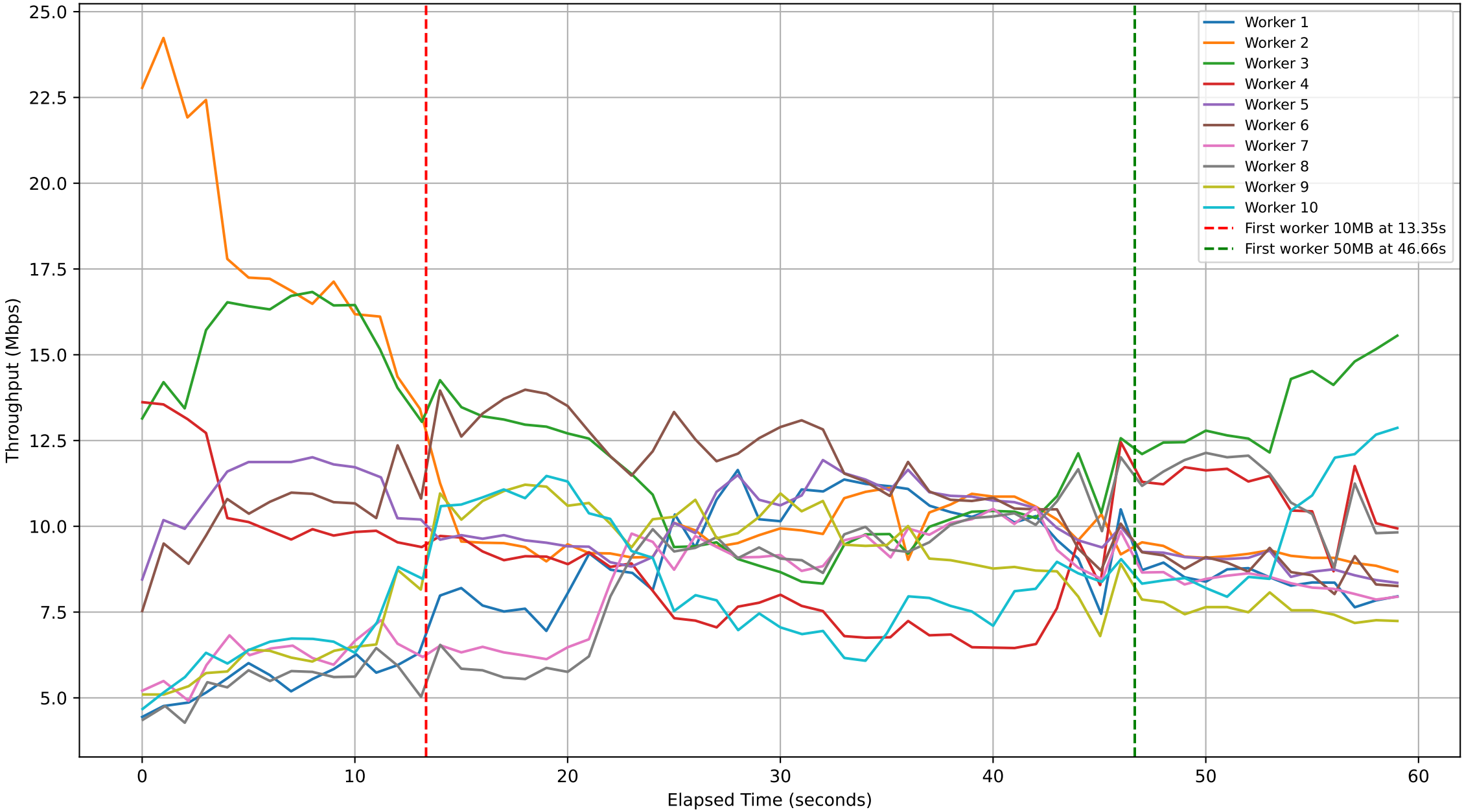
Subjob ID: 96cfedb9-626e-4c3e-bb32-75d5016a8769 - Workers Throughput Over Time
