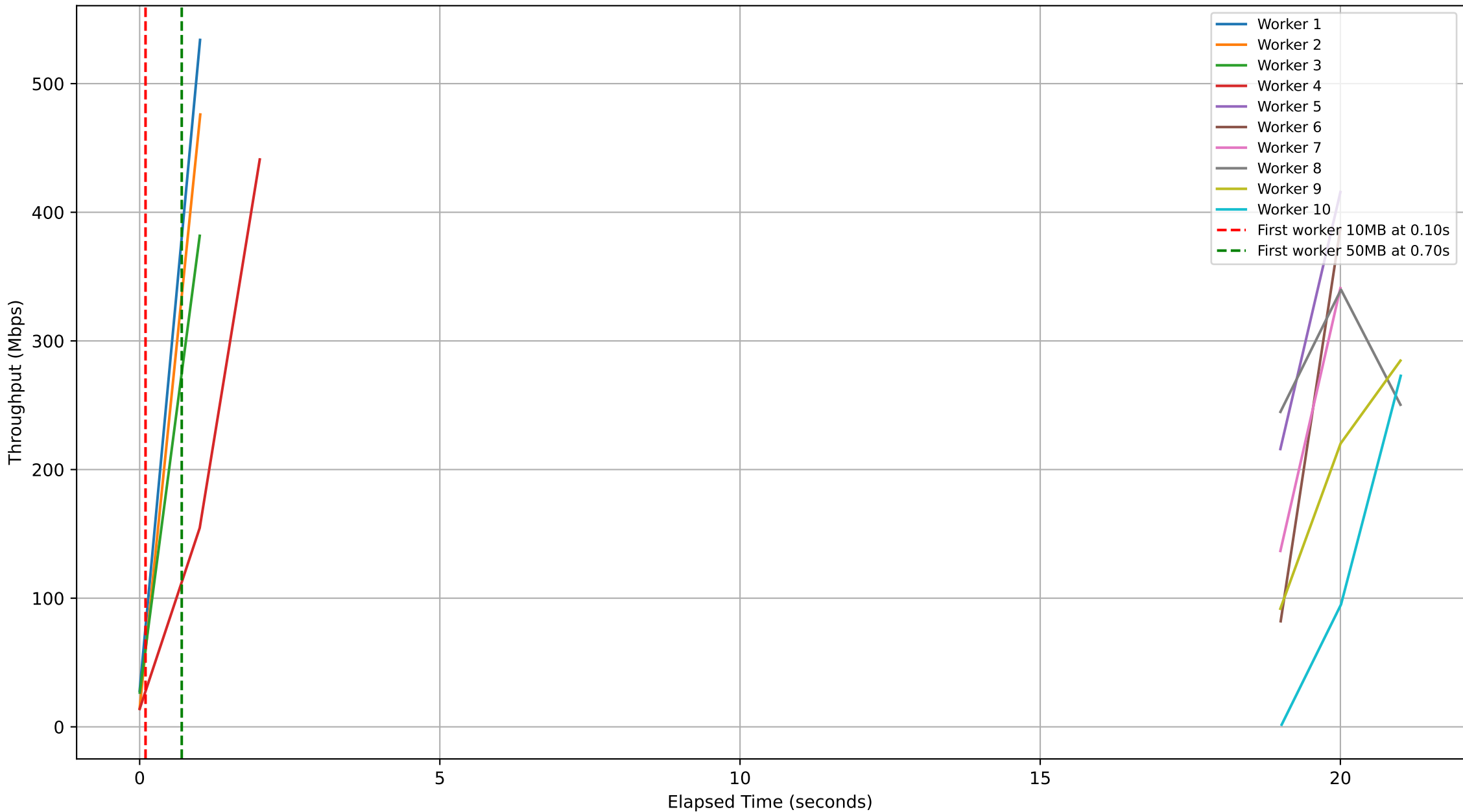
Subjob ID: 9f89a1dc-139f-4e79-aa1c-79a7cefd3c9a - Workers Throughput Over Time
