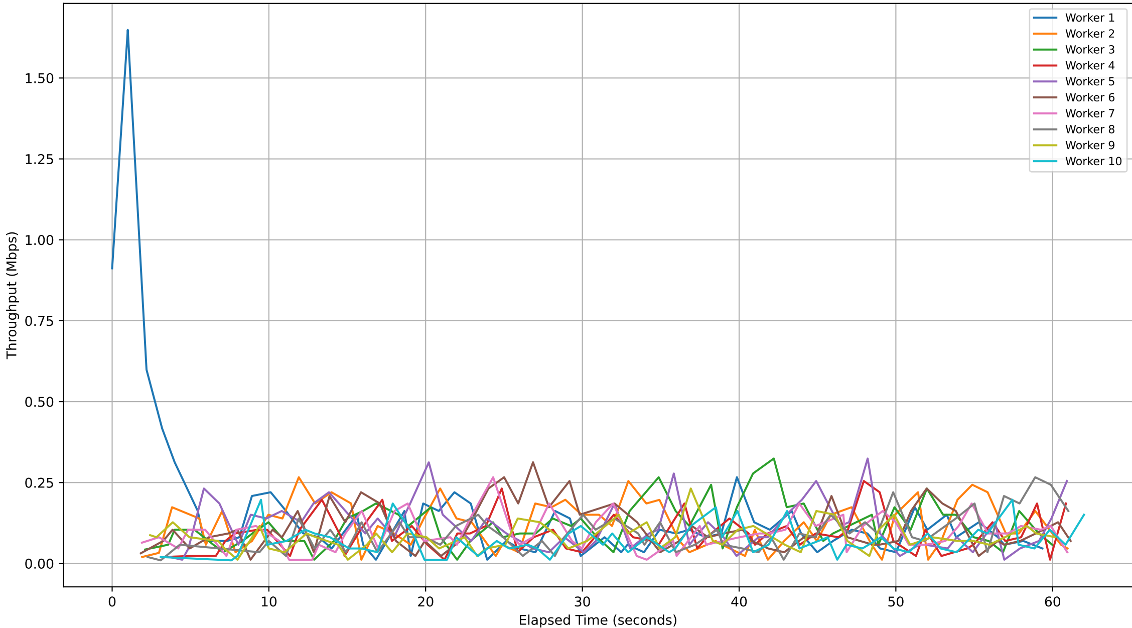
Subjob ID: ef30abd9-8e8d-421d-bdb7-6e62b2450206 - Workers Throughput Over Time
