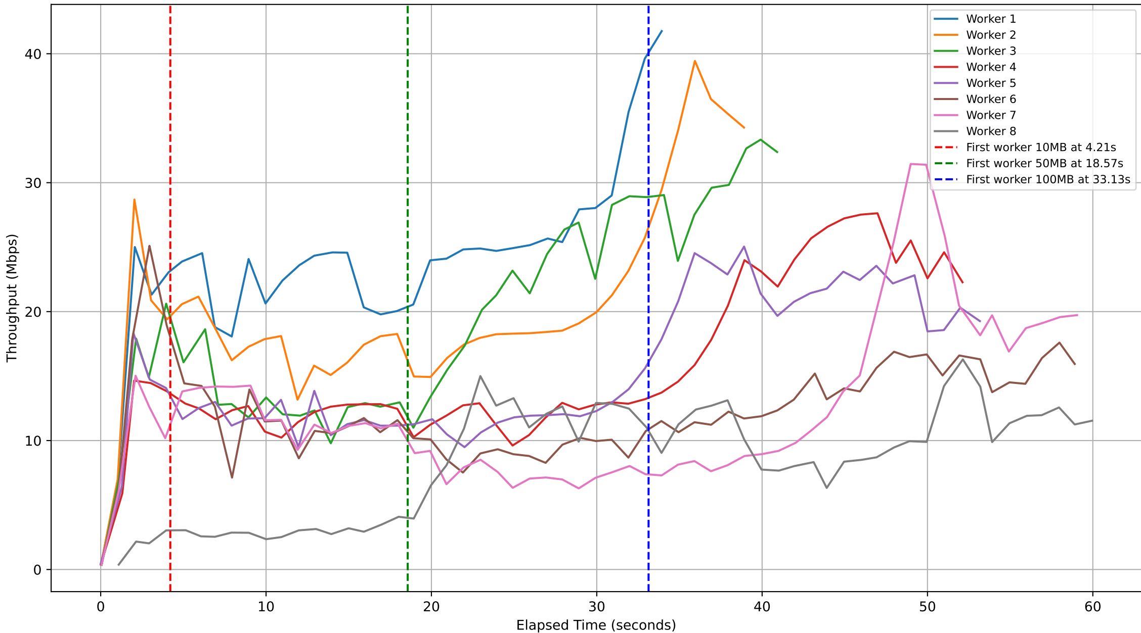
Subjob ID: 8cddc791-66ca-4ef9-83b2-a3893496efdd - Workers Throughput Over Time
