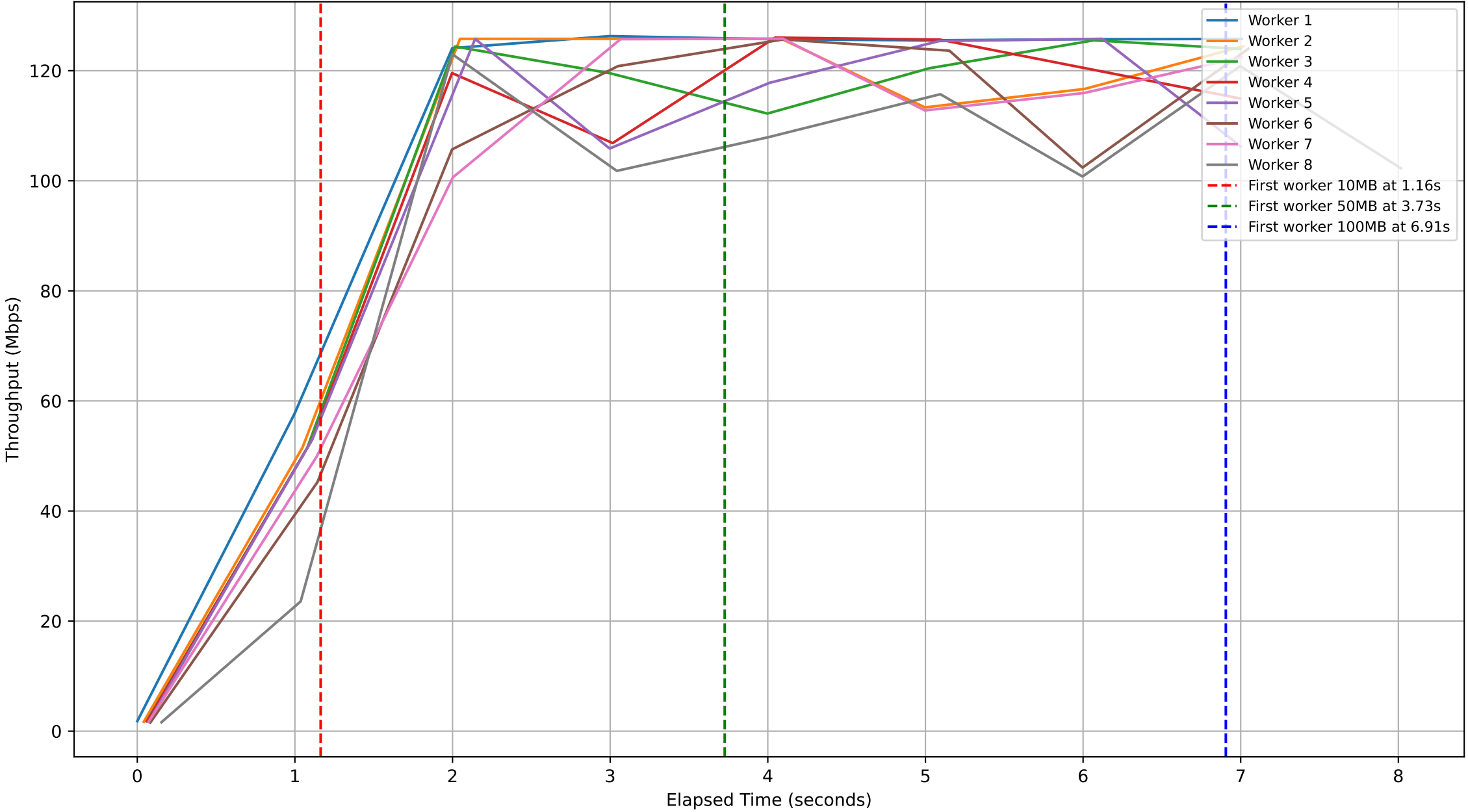
Subjob ID: b3df2c8e-7c7e-4920-ad02-fbc32d15a318 - Workers Throughput Over Time
