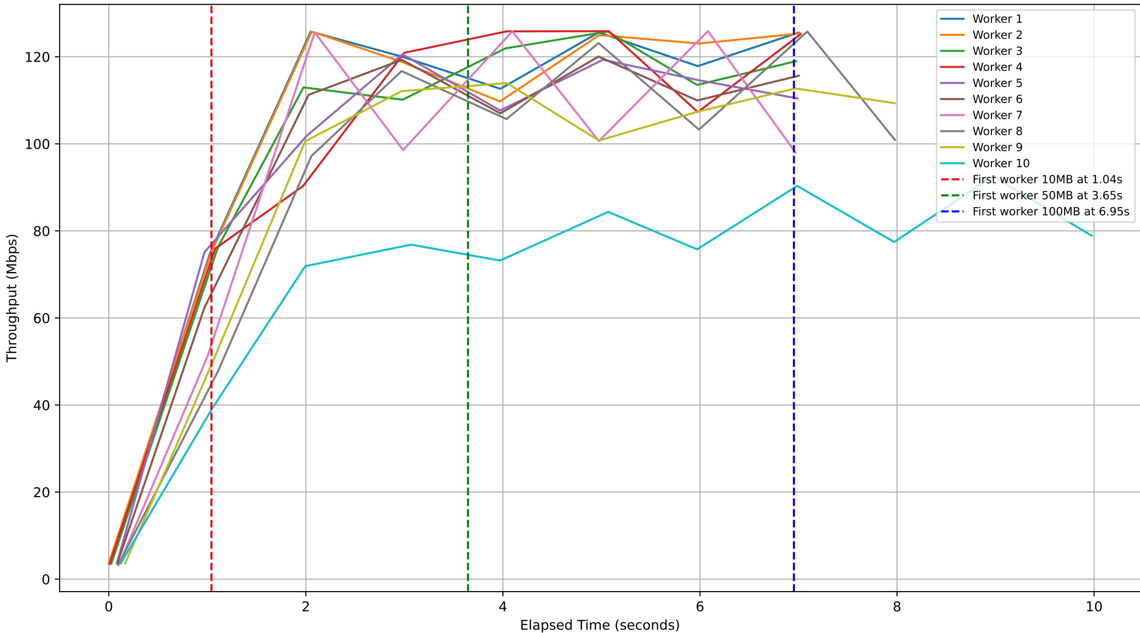
Subjob ID: 0d7afd25-323b-4832-8626-df72dc3f9b3f - Workers Throughput Over Time
