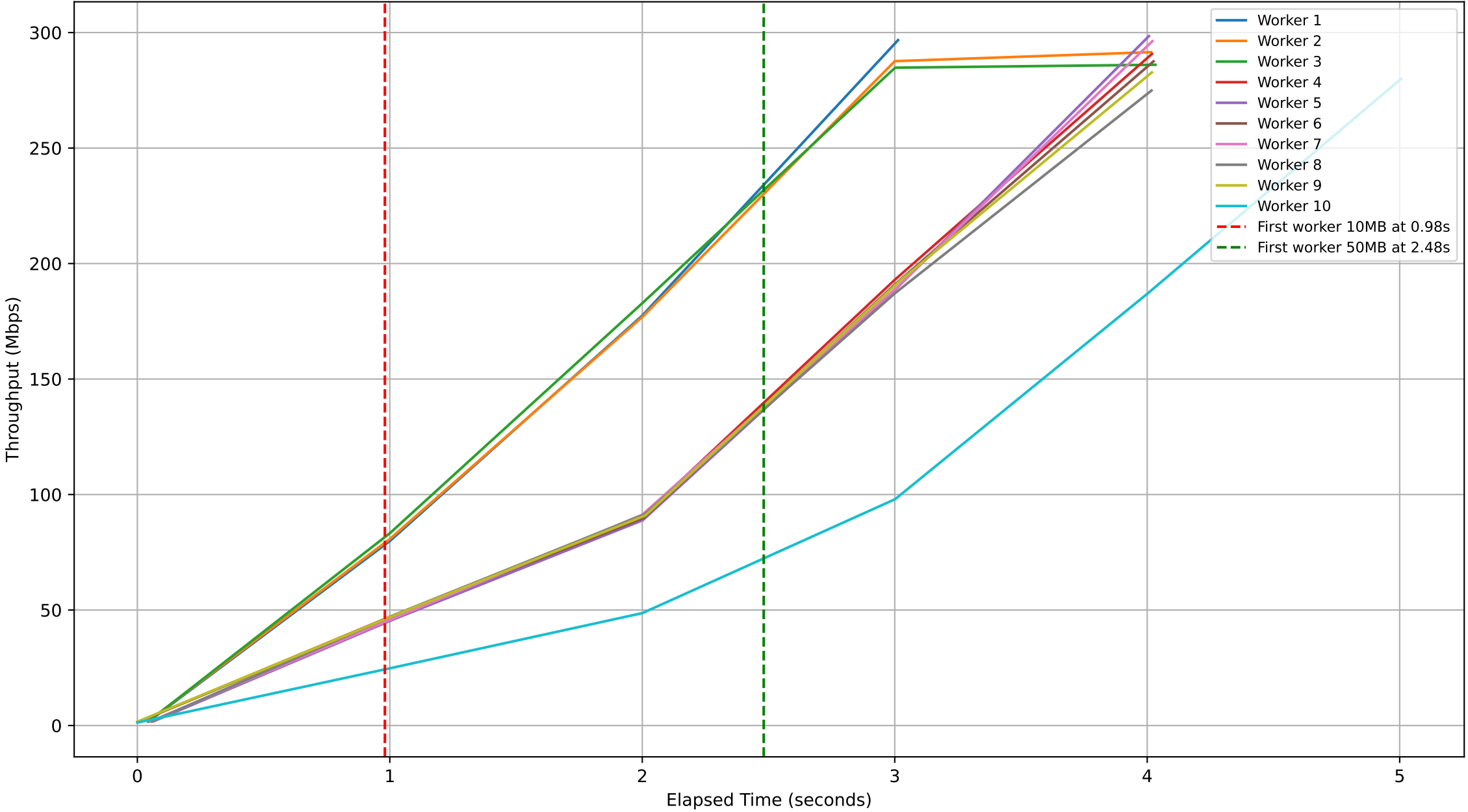
Subjob ID: 1bfbdcc8-25ec-4989-a764-172d5792eb49 - Workers Throughput Over Time
