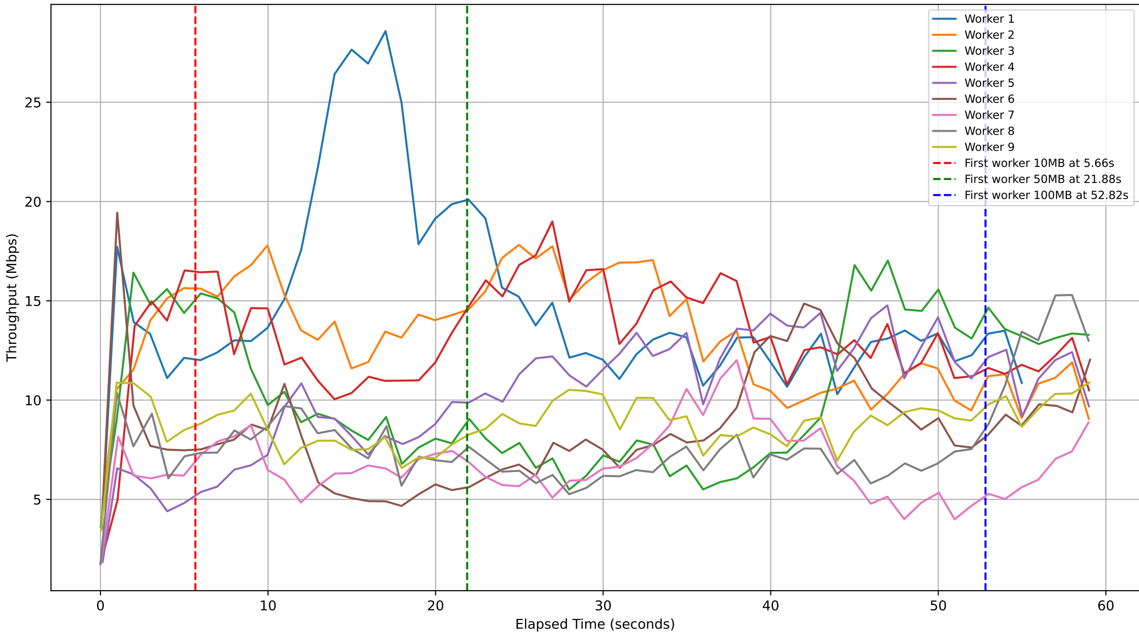
Subjob ID: a8e99a2b-f45a-475f-8226-c23139d72606 - Workers Throughput Over Time
