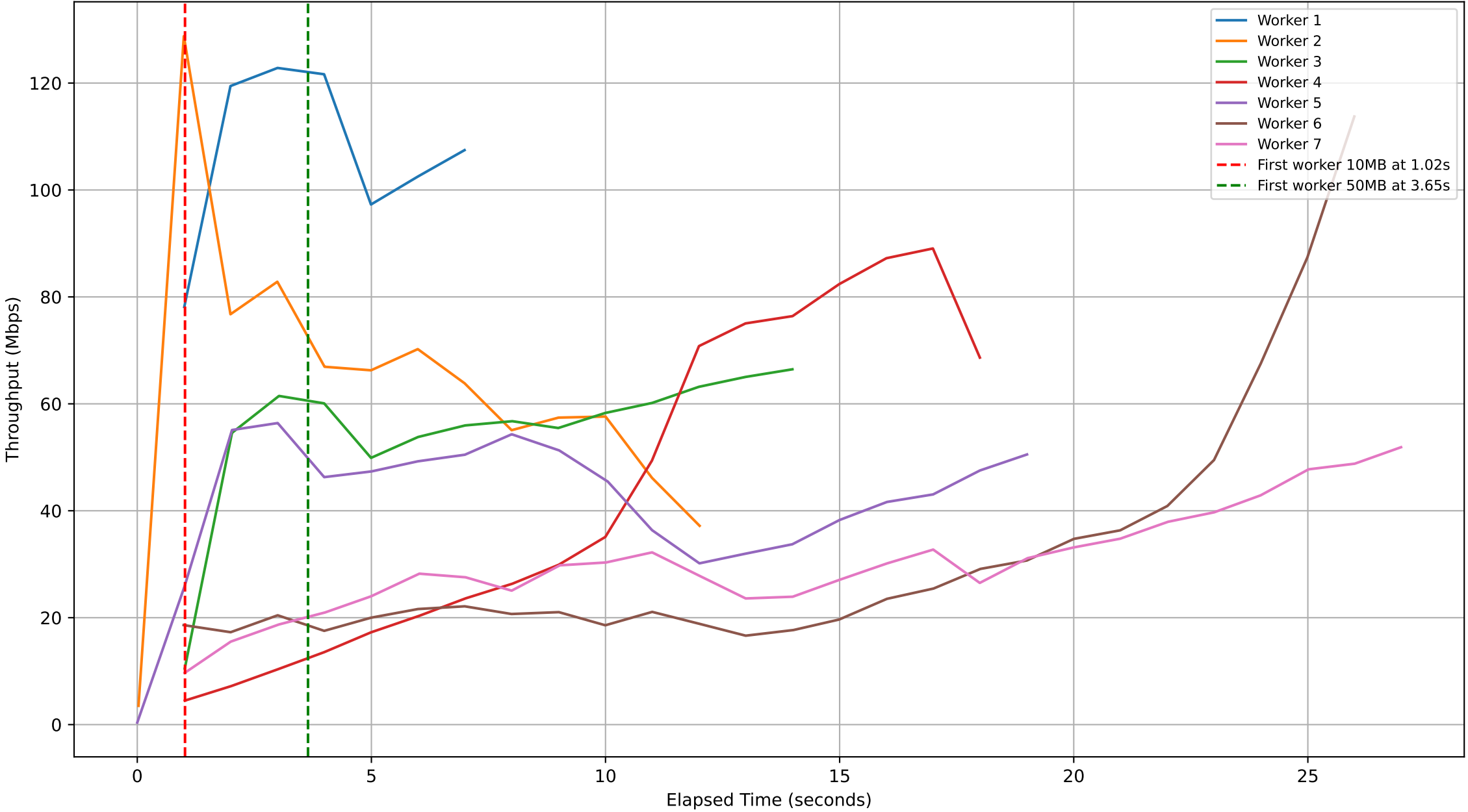
Subjob ID: 90b9640b-e12c-41a1-978e-d2f488bf82a3 - Workers Throughput Over Time
