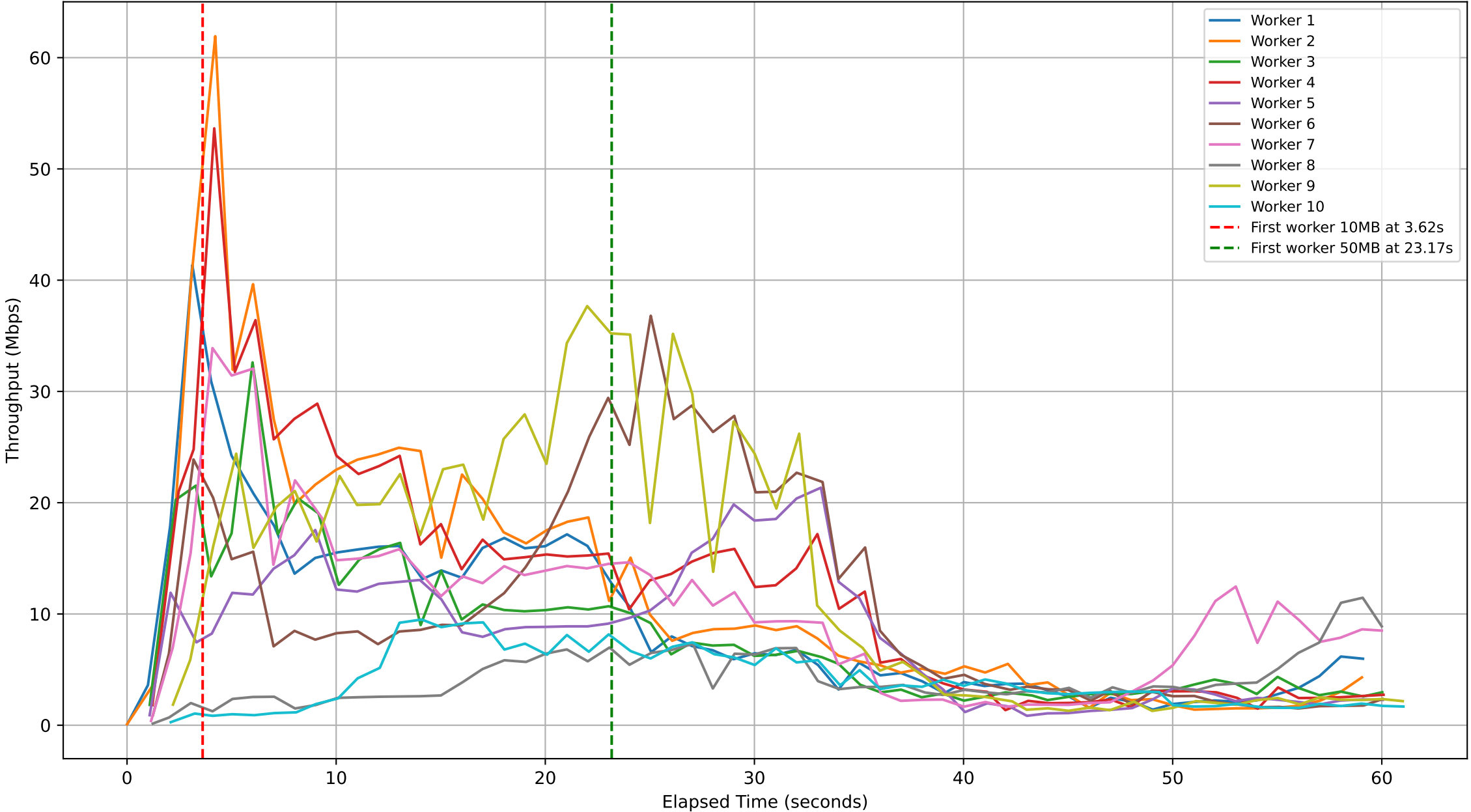
Subjob ID: fa867e00-8cfe-4e59-8b20-5657746c407f - Workers Throughput Over Time
