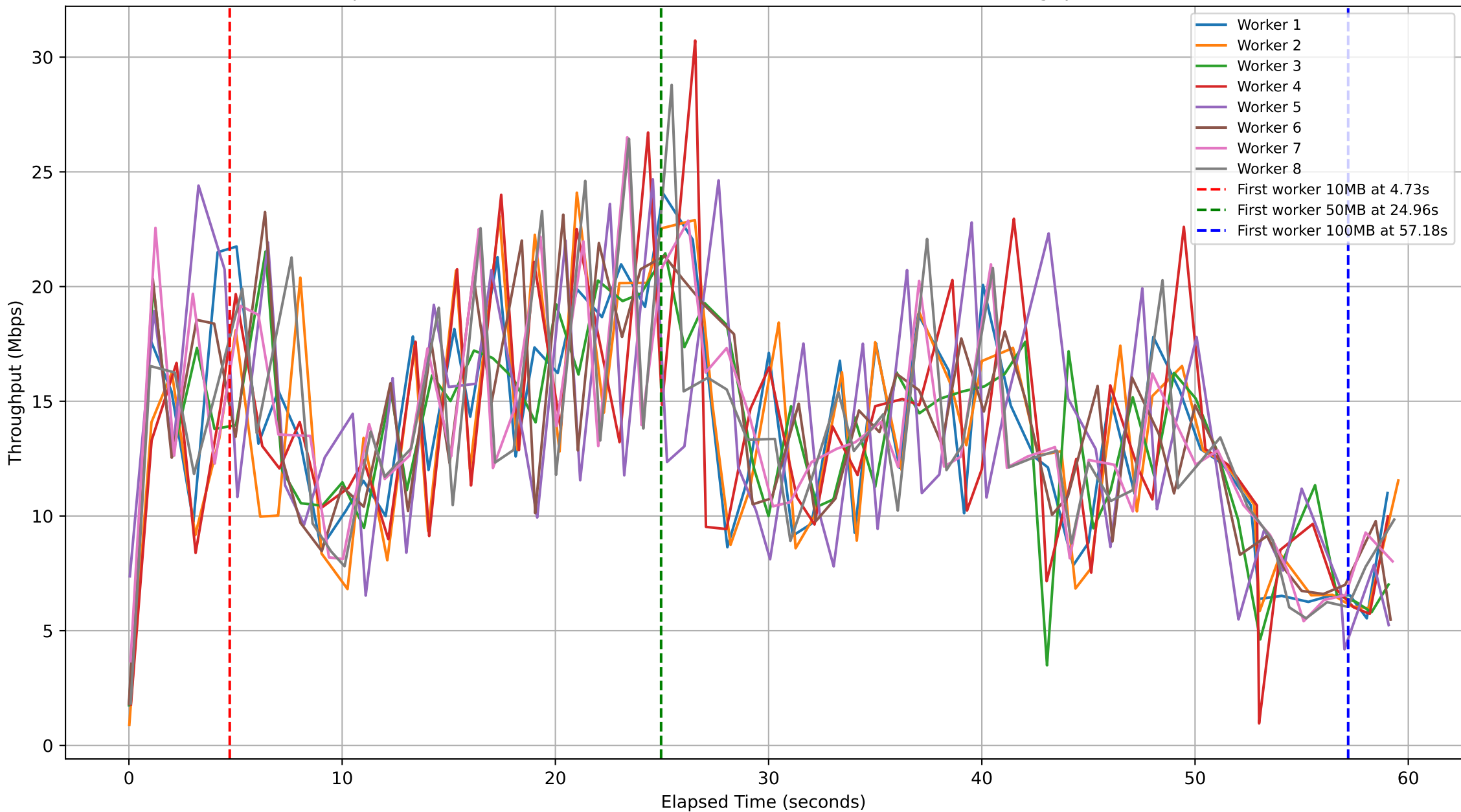
Subjob ID: 160543cb-51ef-4ac9-b61a-754451a72ad7 - Workers Throughput Over Time
