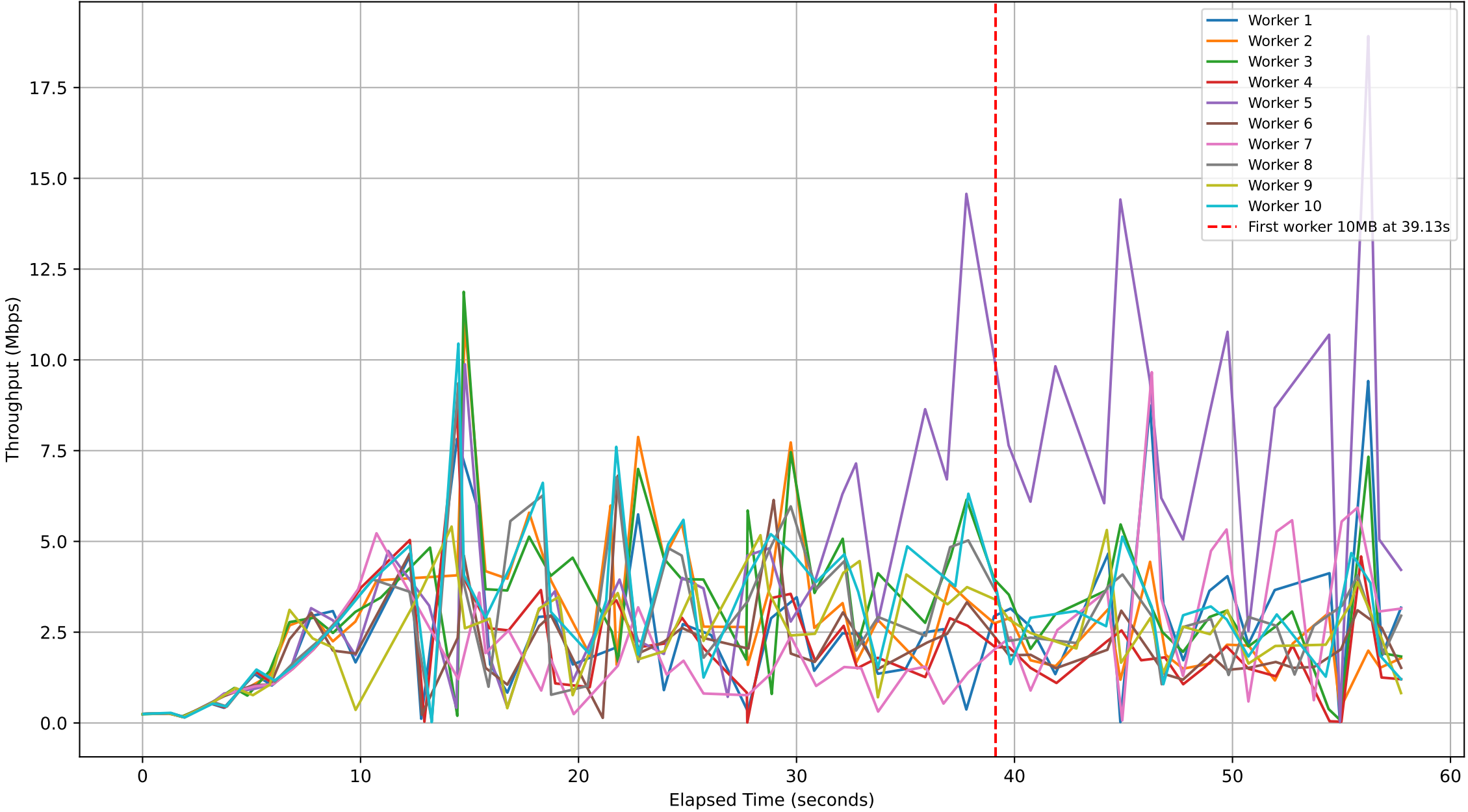
Subjob ID: eb7857d4-48b8-4f33-b44d-45b4814cfd34 - Workers Throughput Over Time
