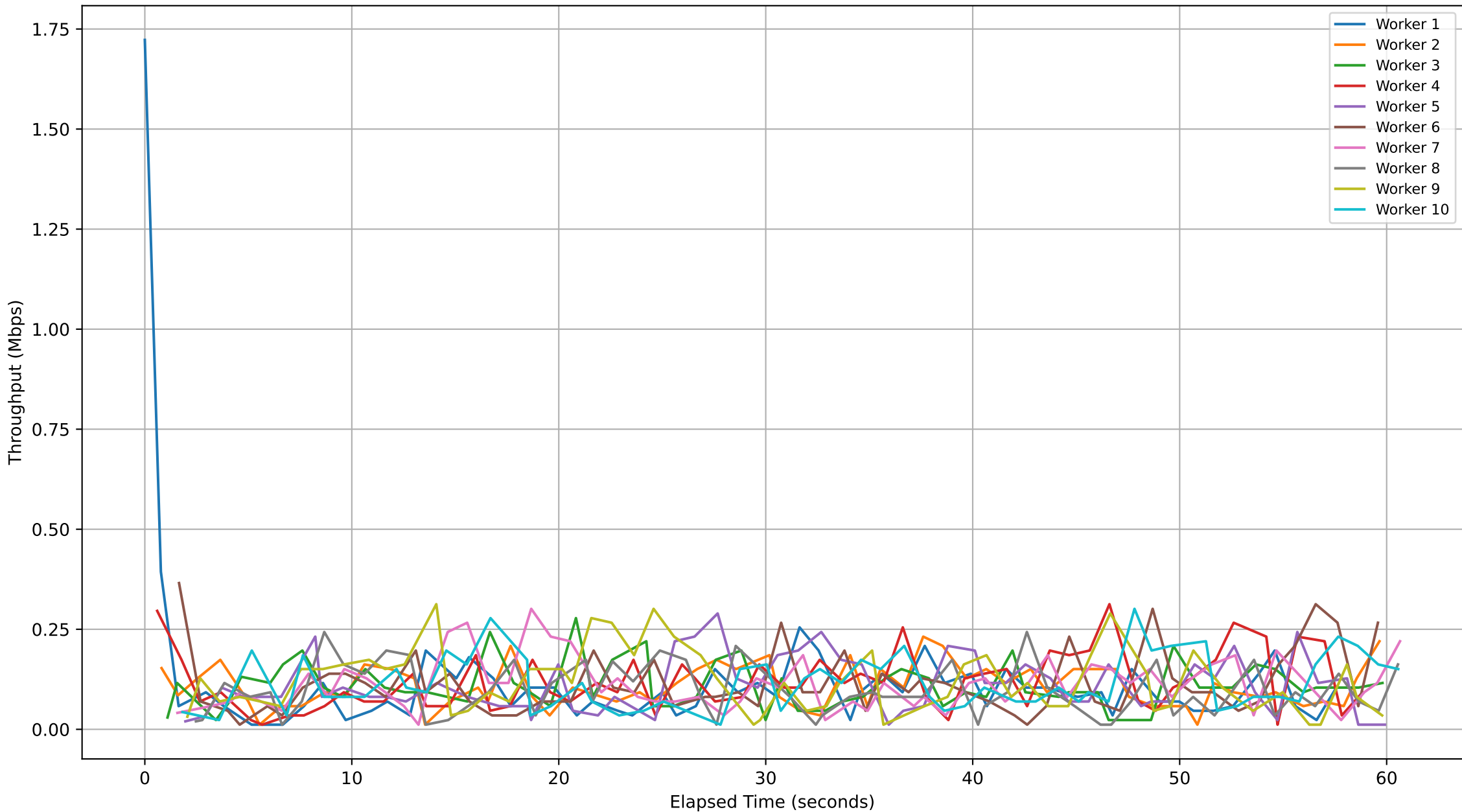
Subjob ID: 9e454ee0-3f51-40c9-b209-cb04a813b102 - Workers Throughput Over Time
