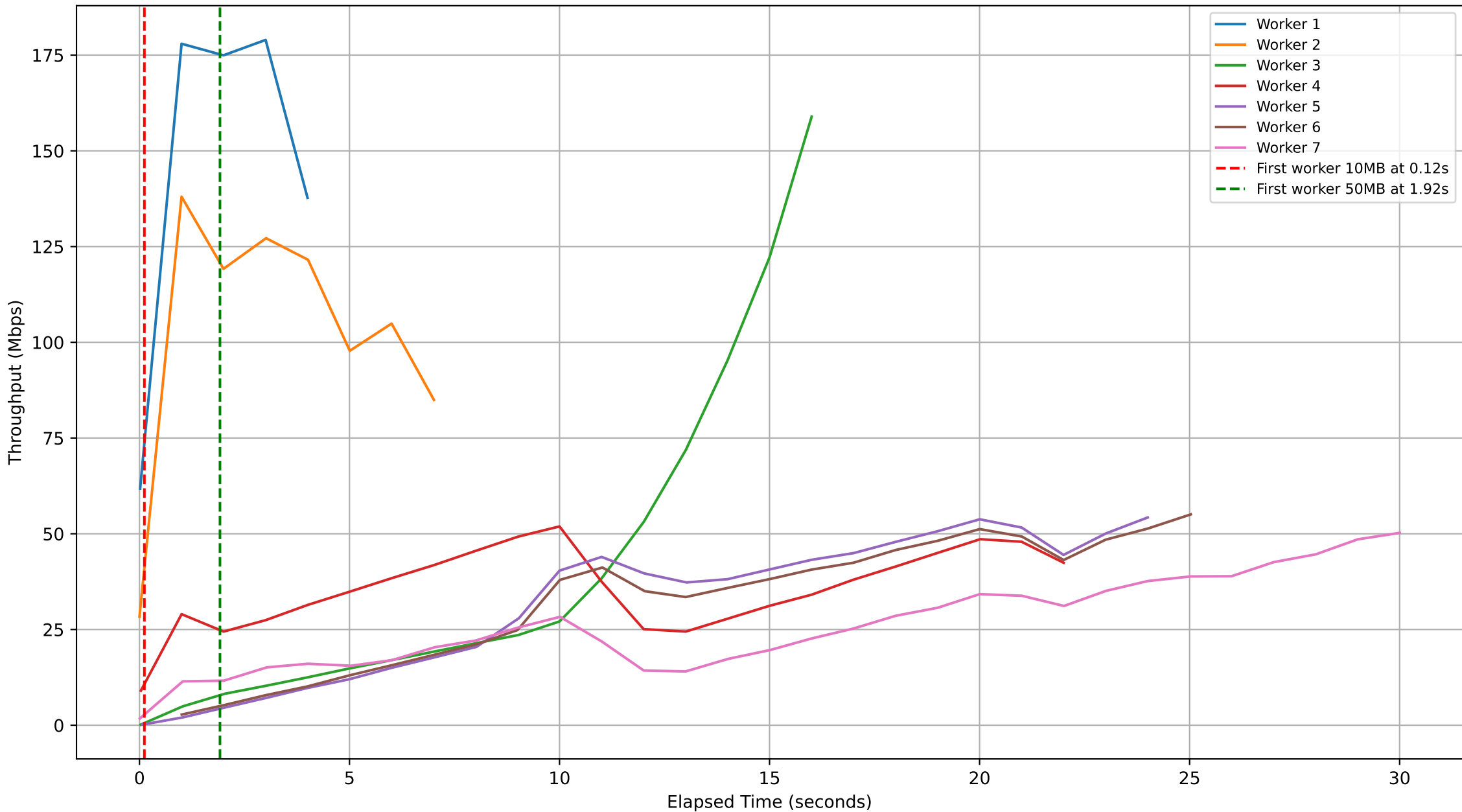
Subjob ID: 17d14387-f757-4734-9211-5c9c08567a27 - Workers Throughput Over Time
