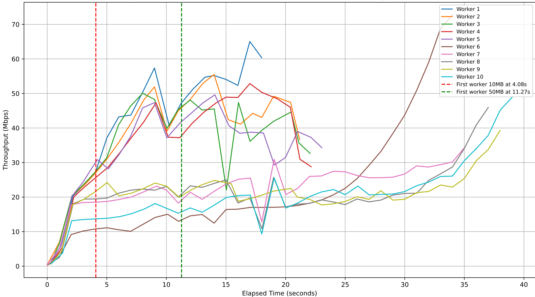
Subjob ID: 6737d374-5add-40d1-8d72-cf8c916e71c6 - Workers Throughput Over Time
