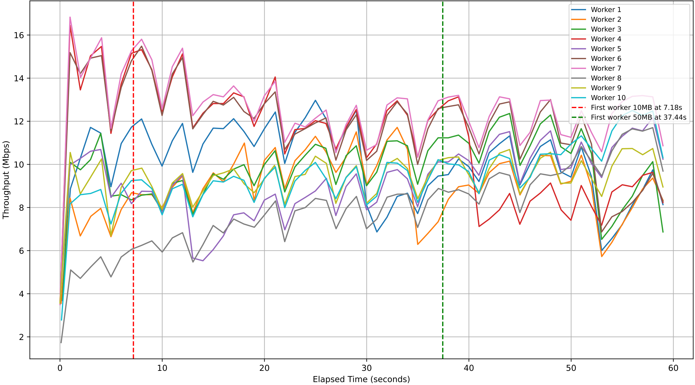
Subjob ID: 5cd6f07f-4f8f-4000-95e1-d118a119392b - Workers Throughput Over Time
