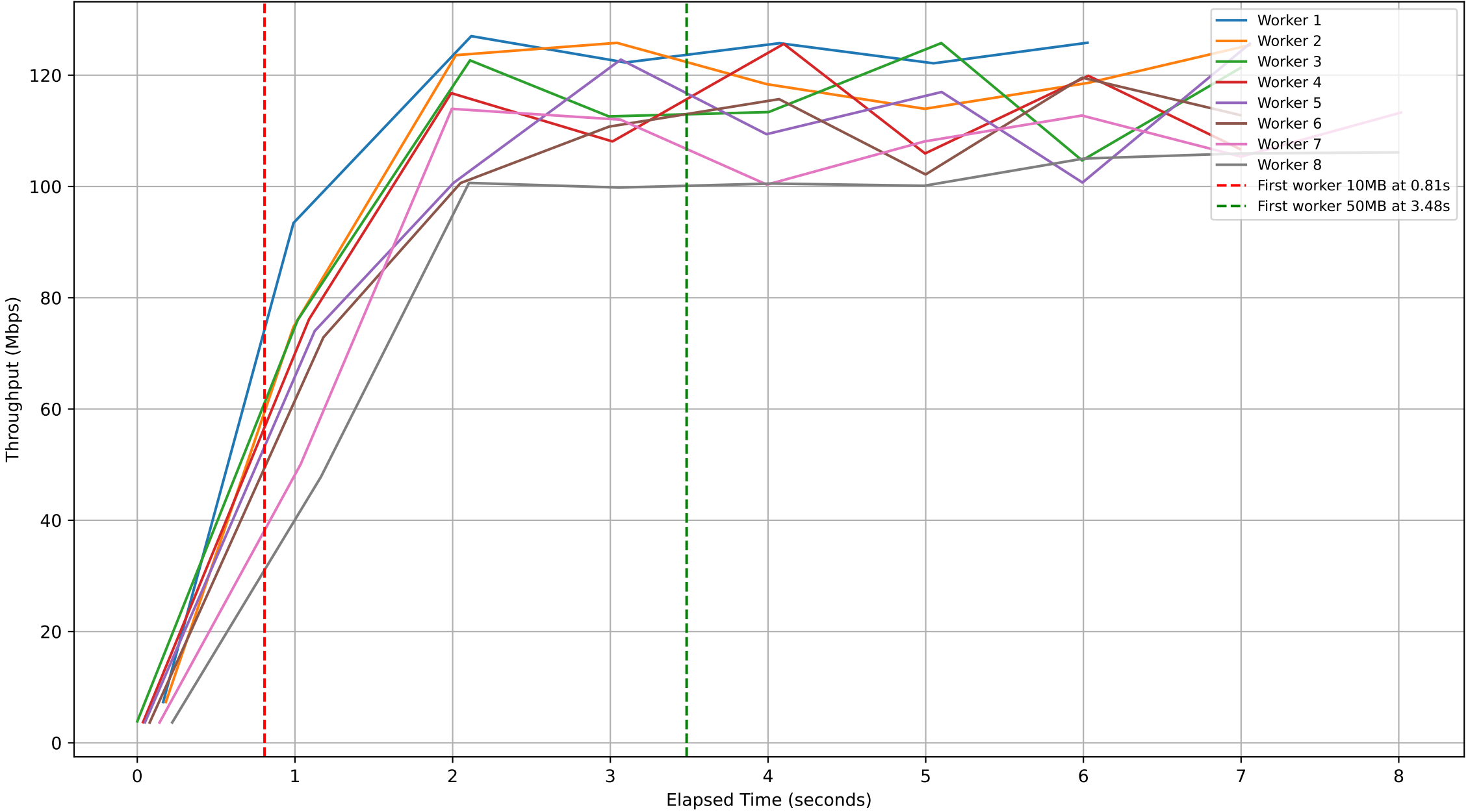
Subjob ID: 2f031337-e8ab-4676-96f1-bea5d72c80c1 - Workers Throughput Over Time
