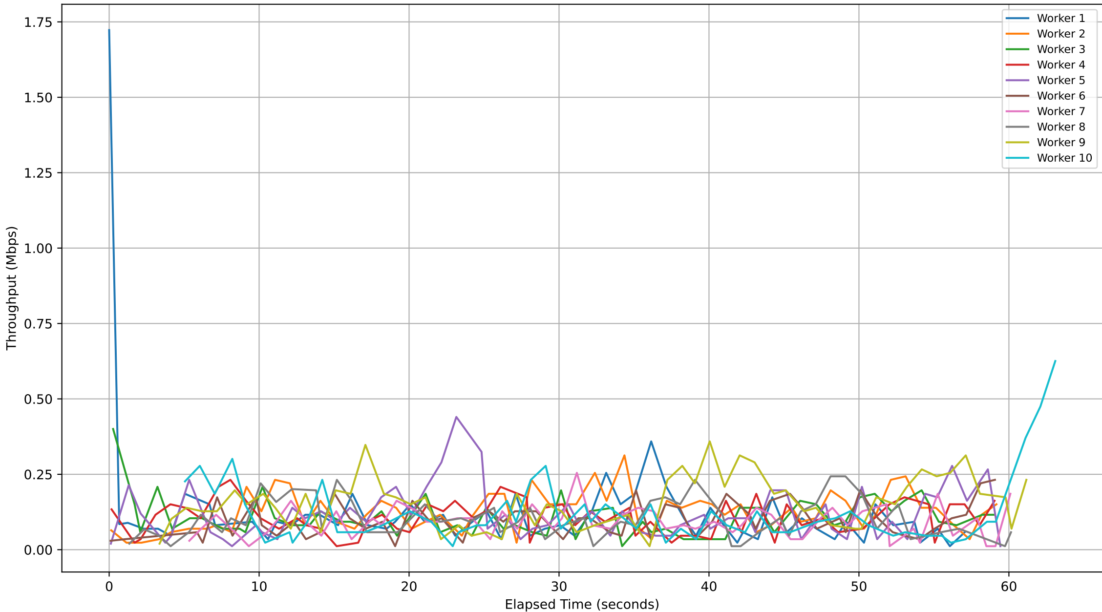
Subjob ID: 312a0365-7d2b-45f0-add0-11c4a0e7a22c - Workers Throughput Over Time
