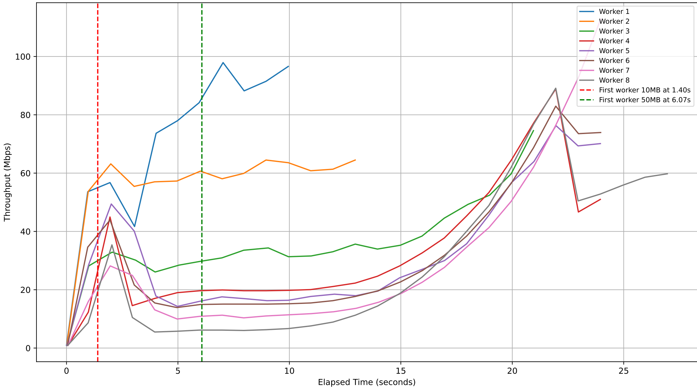
Subjob ID: 98f952e1-5d2b-493c-88e7-4b555578b430 - Workers Throughput Over Time
