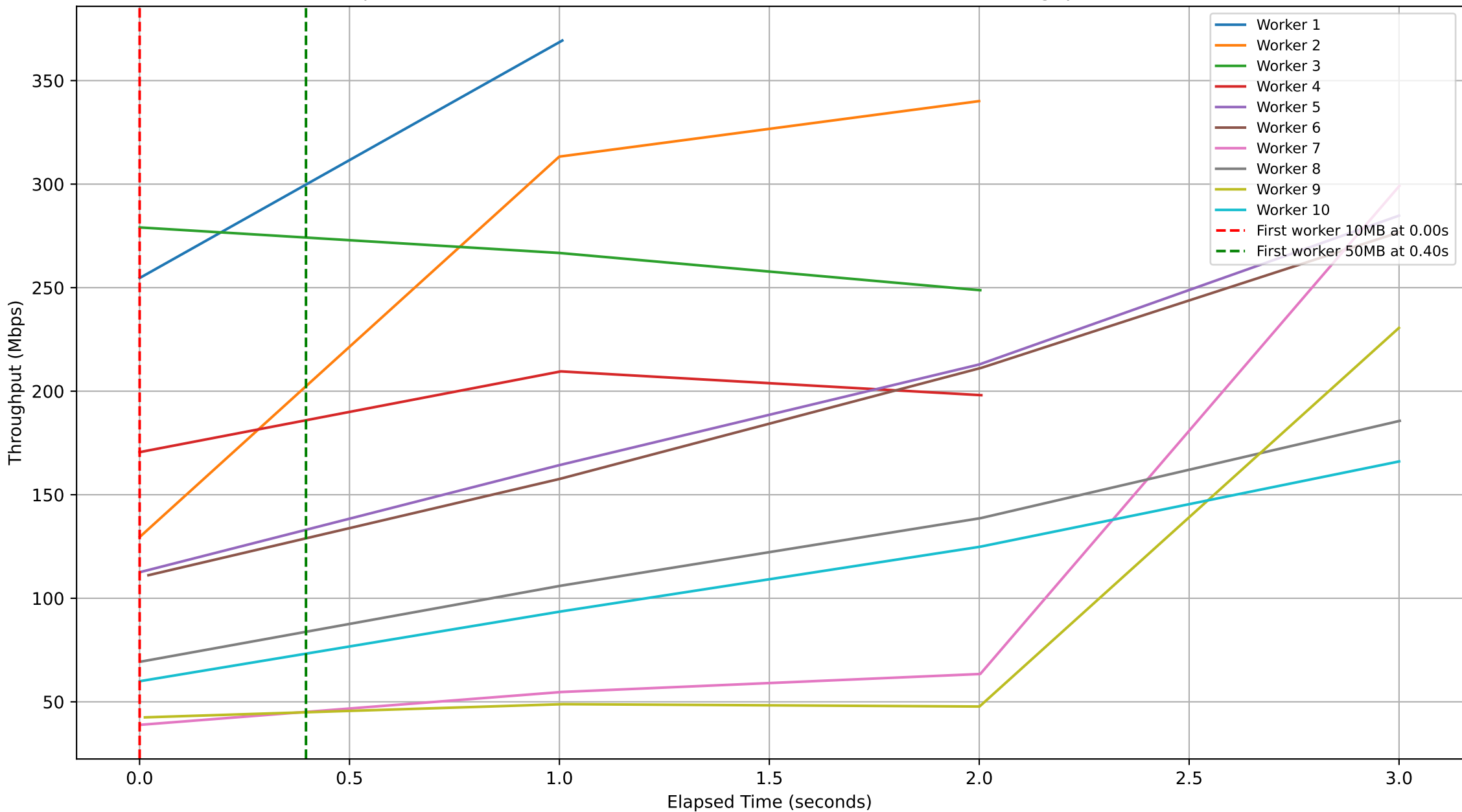
Subjob ID: 75c26e75-ee0d-448b-afa0-52a856f2ad5f - Workers Throughput Over Time
