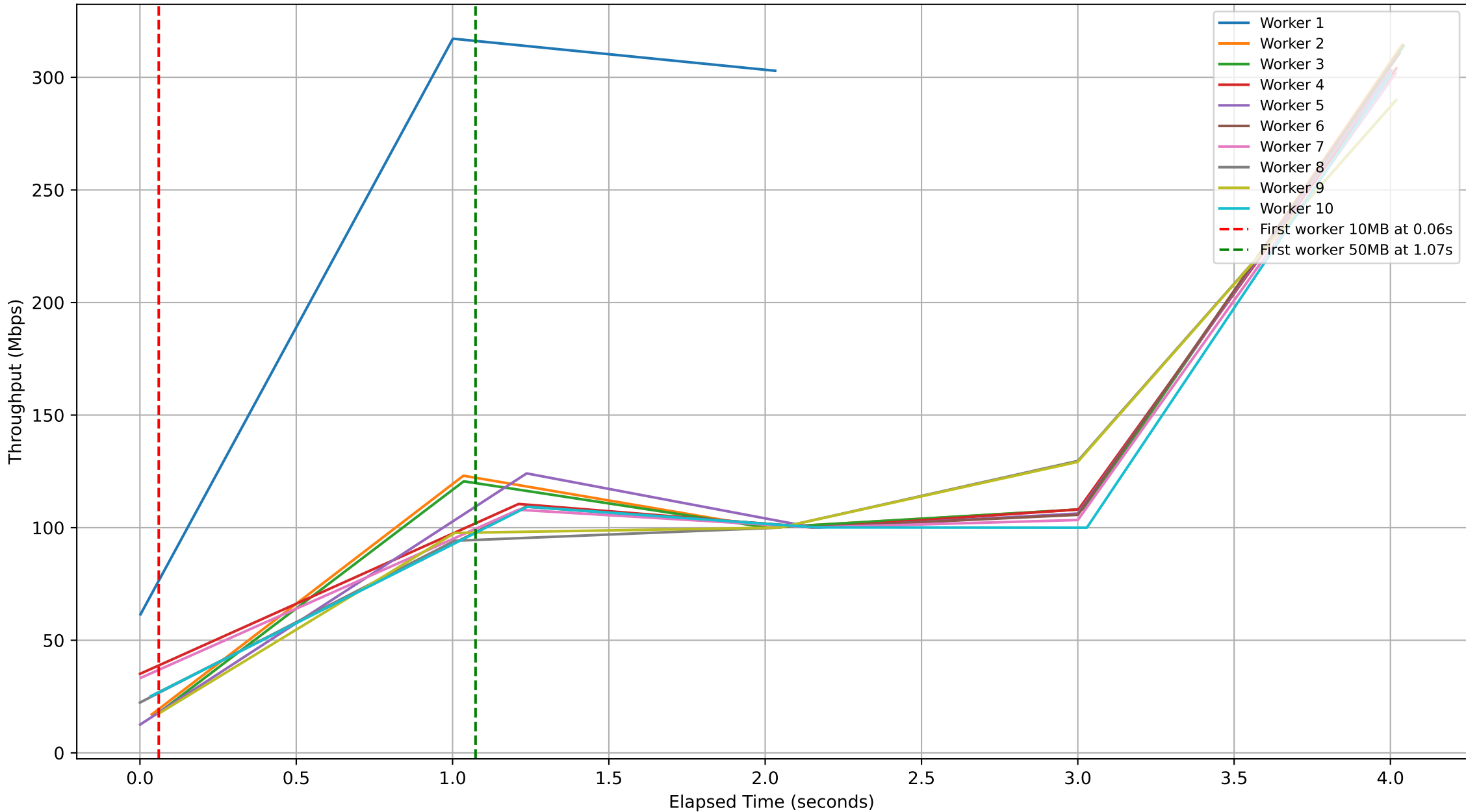
Subjob ID: b003ece1-ff38-48f8-84f6-0cac153b5bcd - Workers Throughput Over Time
