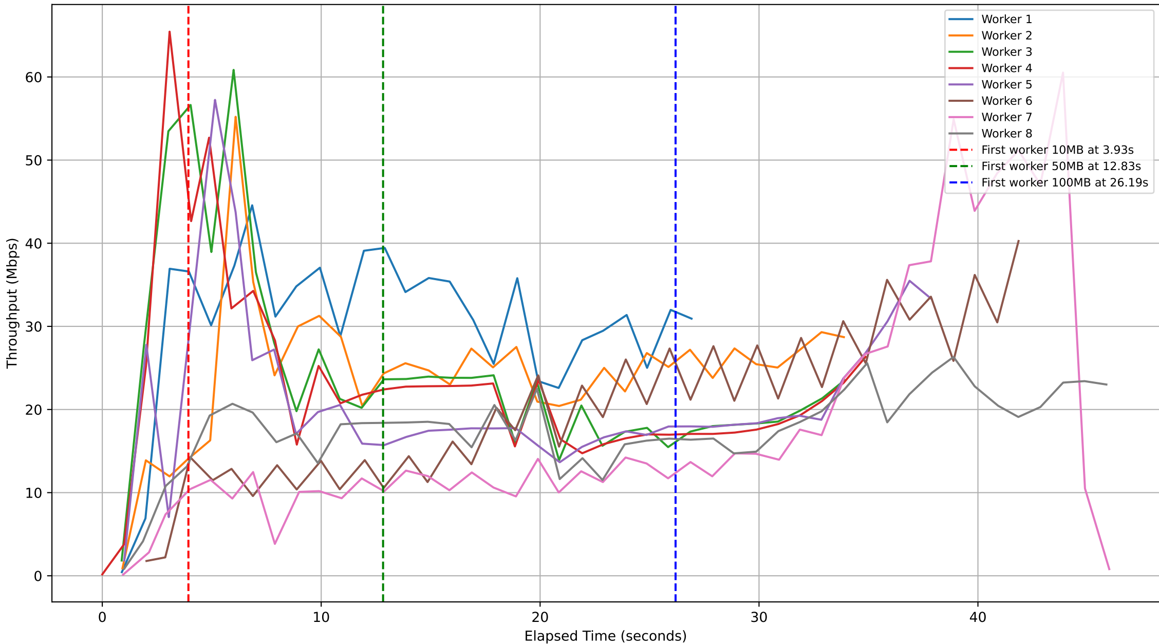
Subjob ID: 205c37a1-b5f3-4cce-8a0a-7f4d30dc7996 - Workers Throughput Over Time
