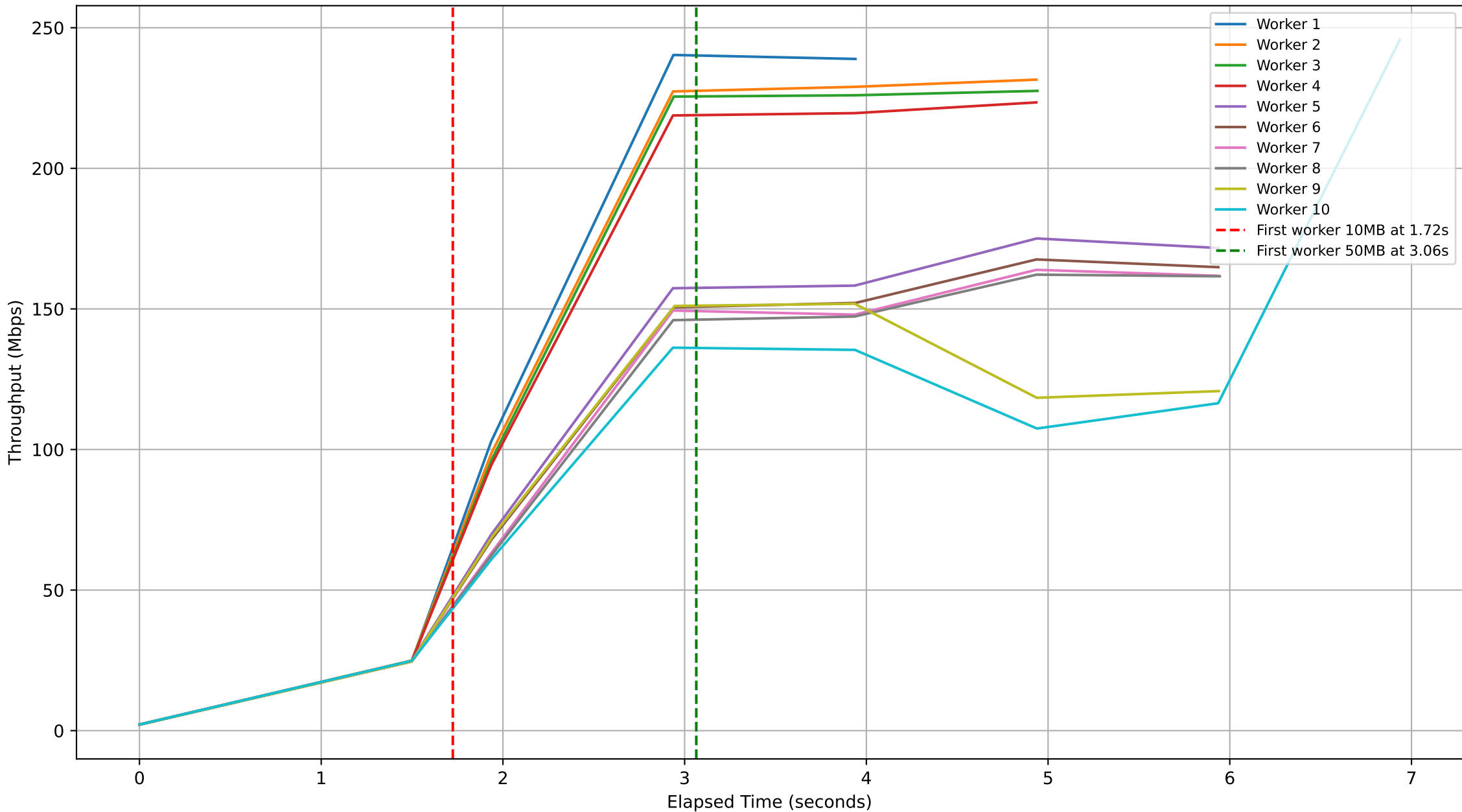
Subjob ID: f7186b93-98e9-4410-9266-3e83342eaeca - Workers Throughput Over Time
