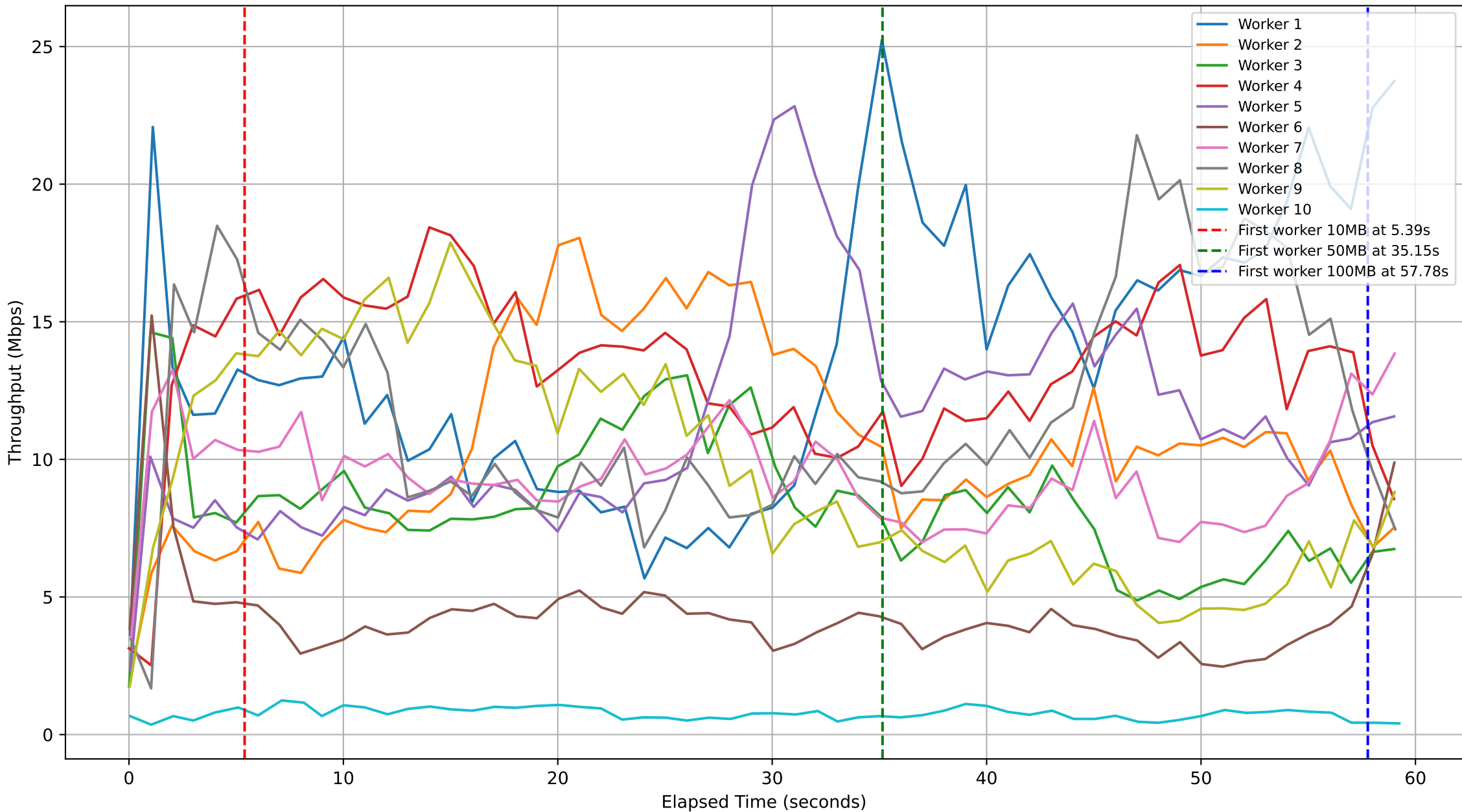
Subjob ID: b8d9a3d4-83b2-4297-a57b-ad2617f4ad54 - Workers Throughput Over Time
