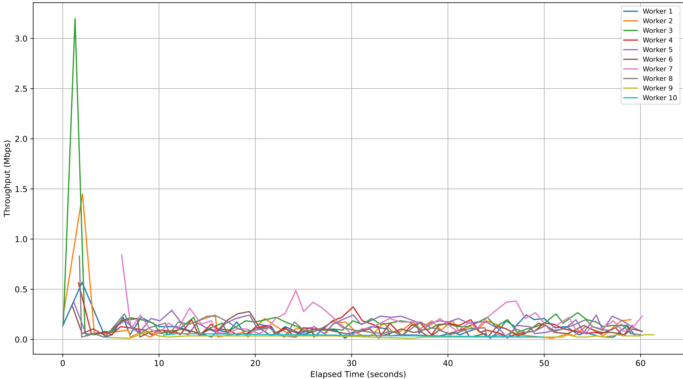
Subjob ID: fa8e7d91-f803-4f66-9844-492453bb183e - Workers Throughput Over Time
