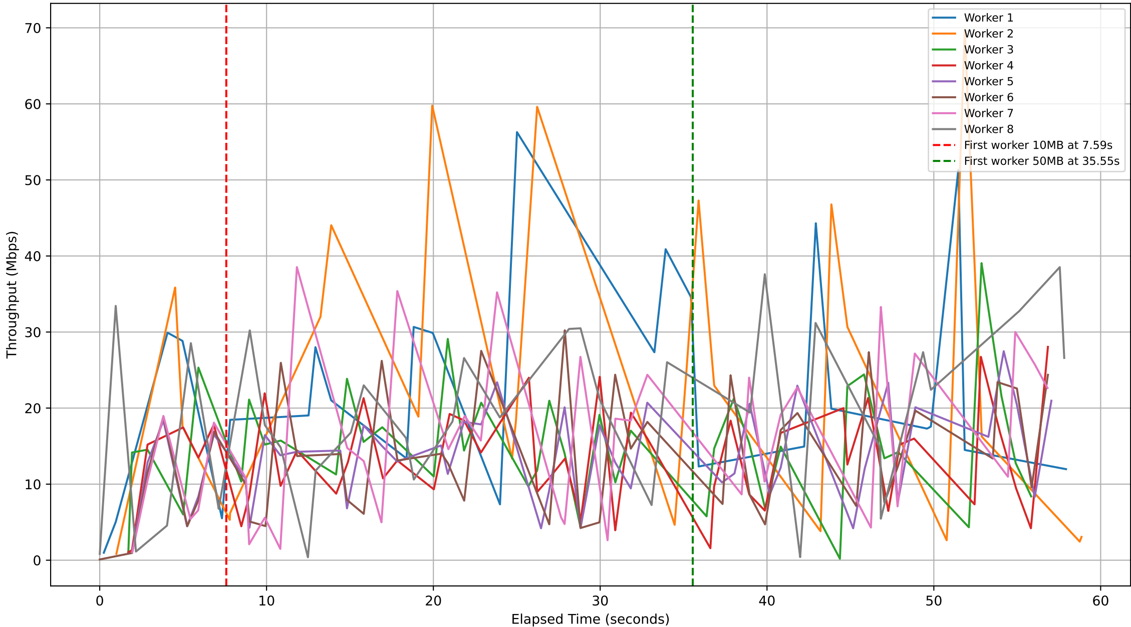
Subjob ID: 4e631cda-0ce6-41af-a997-a6a36f80b79a - Workers Throughput Over Time
