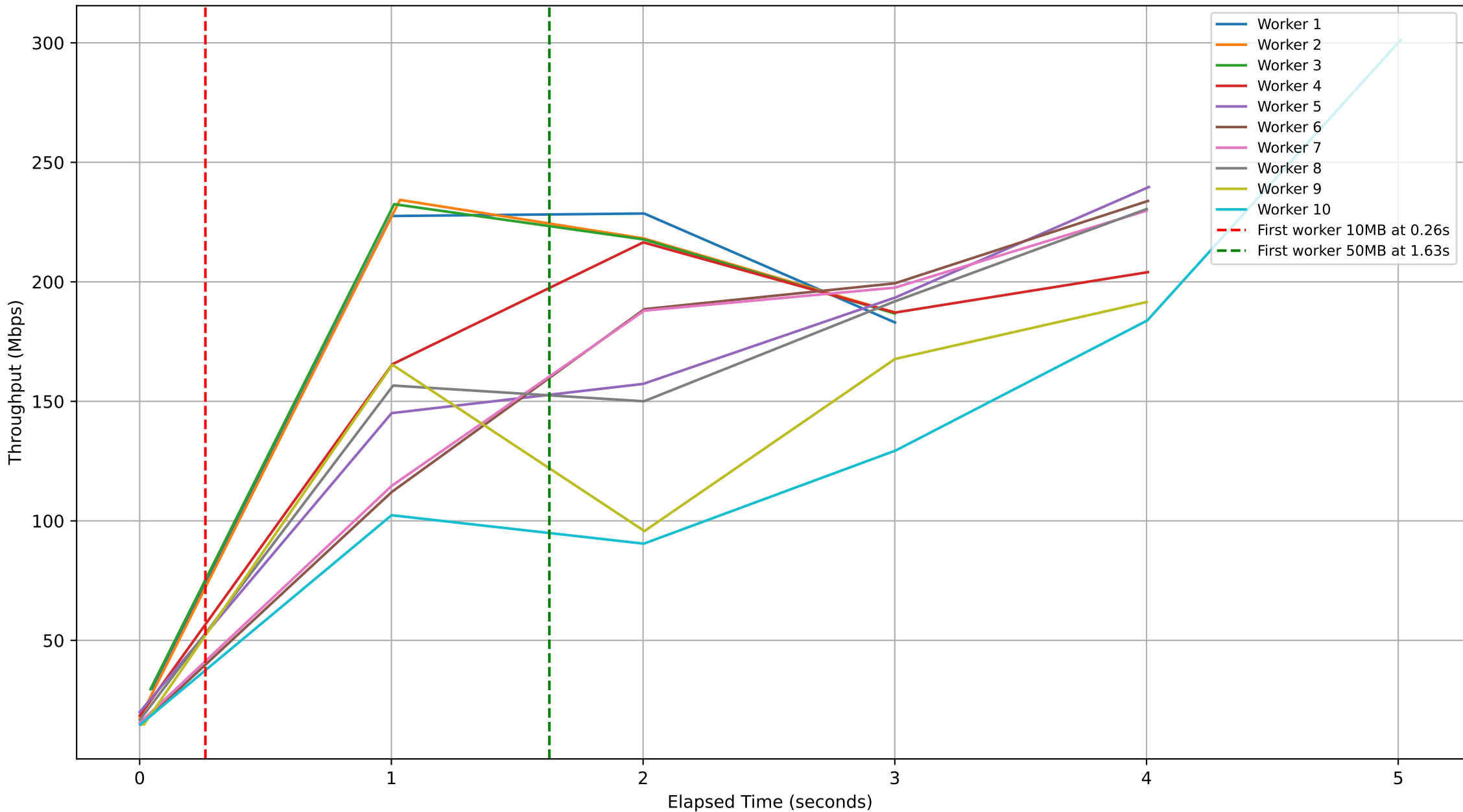
Subjob ID: 0d68e0f4-0fb0-47af-9444-240532ea6a05 - Workers Throughput Over Time
