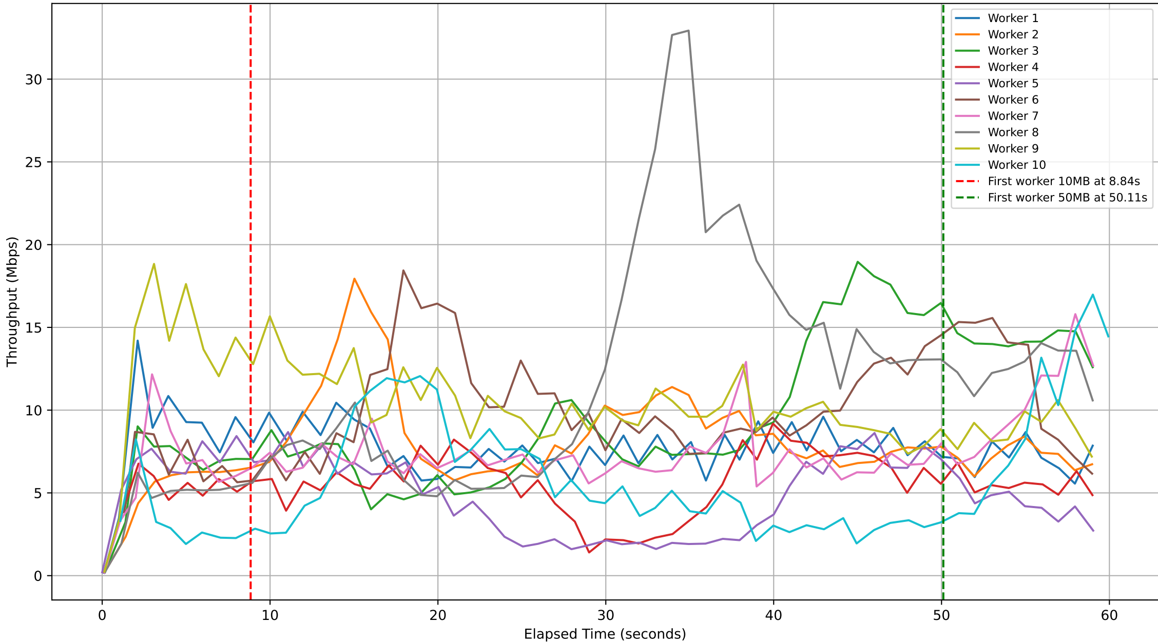
Subjob ID: 279096a6-8f5a-47ea-99ea-fd755443bb63 - Workers Throughput Over Time
