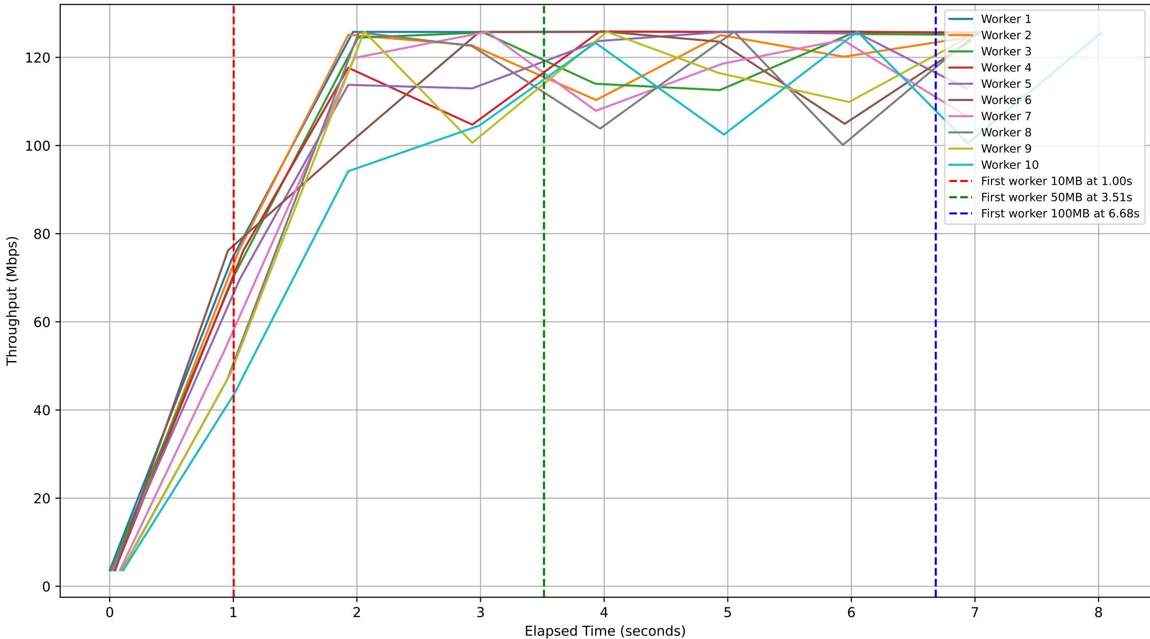
Subjob ID: 9cfebe39-6b65-4e82-b09a-b027a777f2fc - Workers Throughput Over Time
