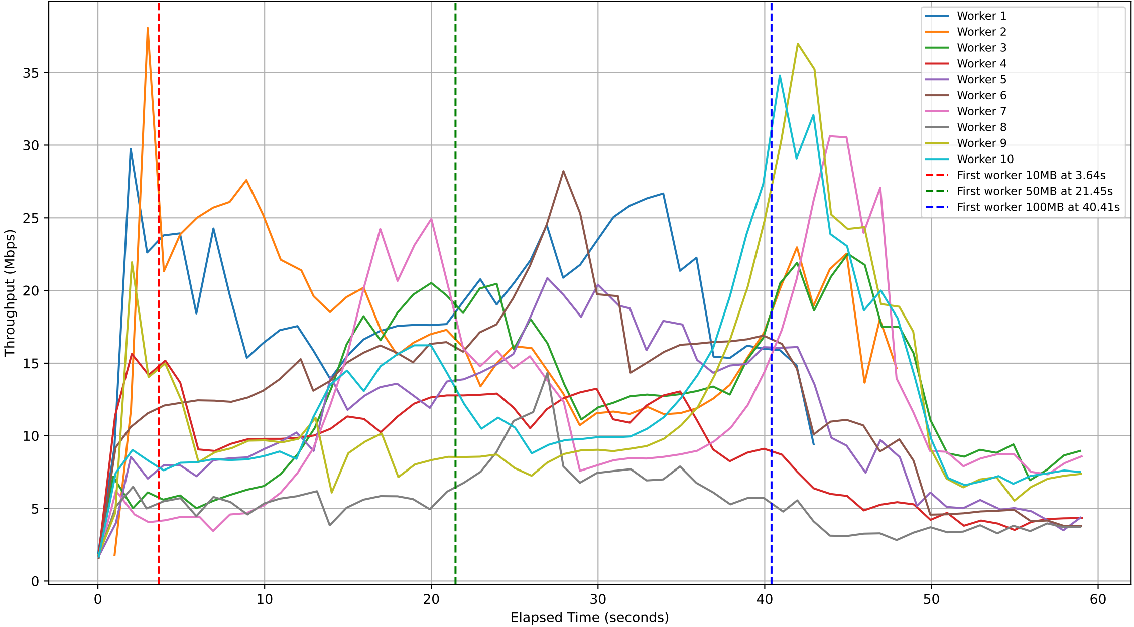
Subjob ID: 2985aa49-a121-4450-bb65-431df00dfffc - Workers Throughput Over Time
