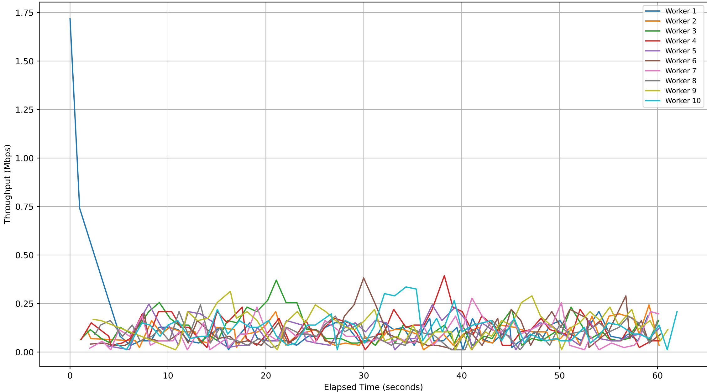
Subjob ID: a14f7205-7557-412a-bdee-93ddf94c114d - Workers Throughput Over Time
