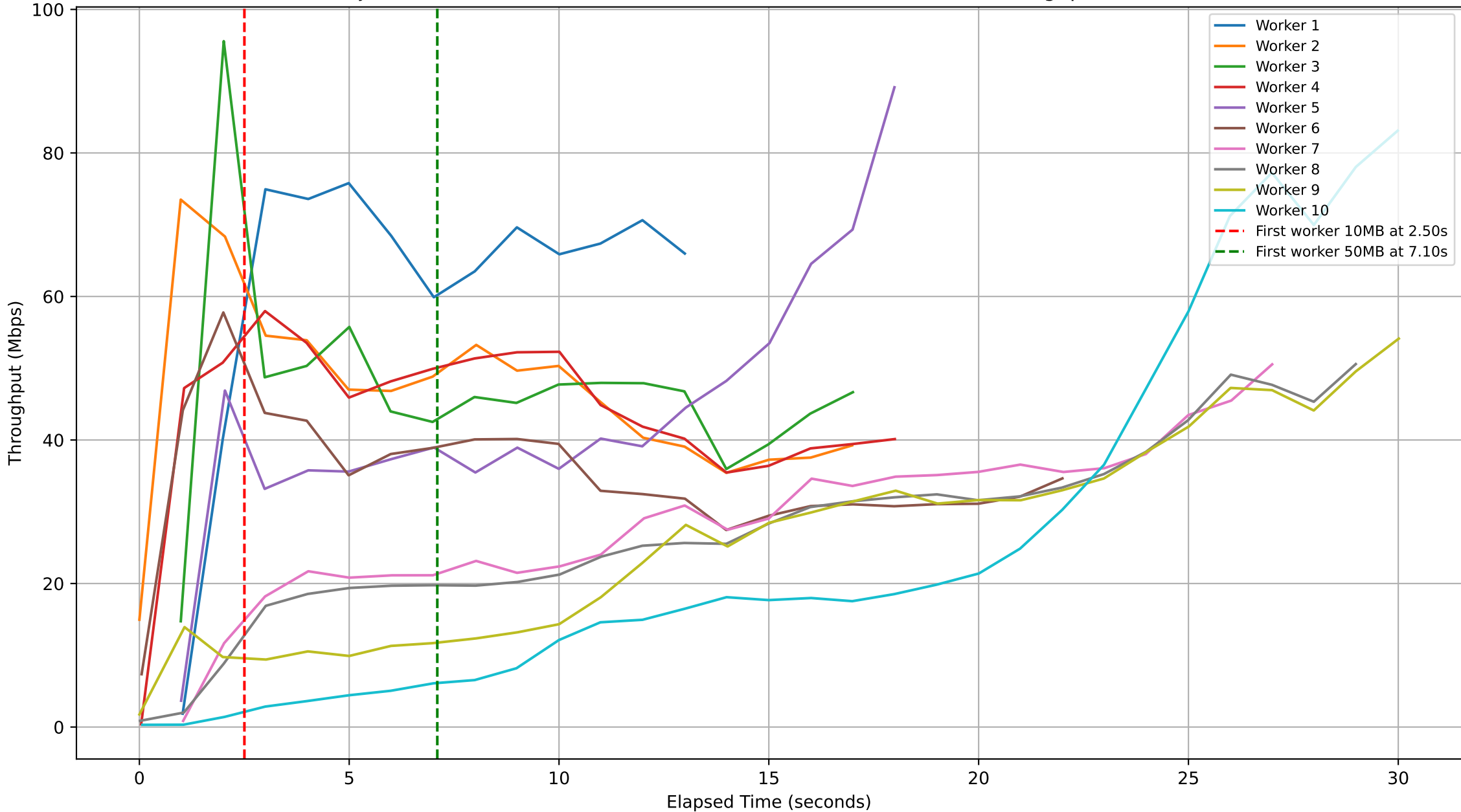
Subjob ID: 853a7f44-64ed-4e31-8a47-80cb2c366ede - Workers Throughput Over Time
