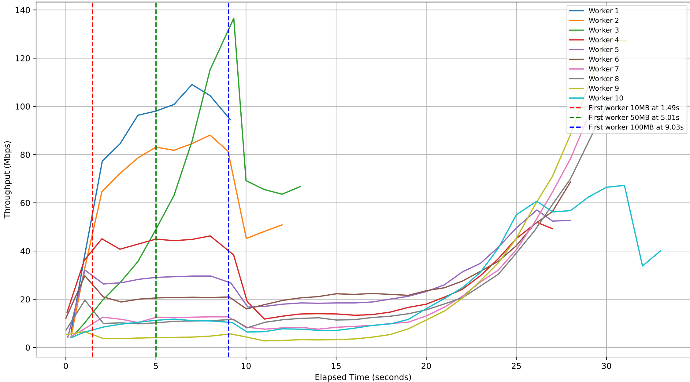
Subjob ID: 8ef4a069-c736-447d-bf20-d4f1dcb380fd - Workers Throughput Over Time
