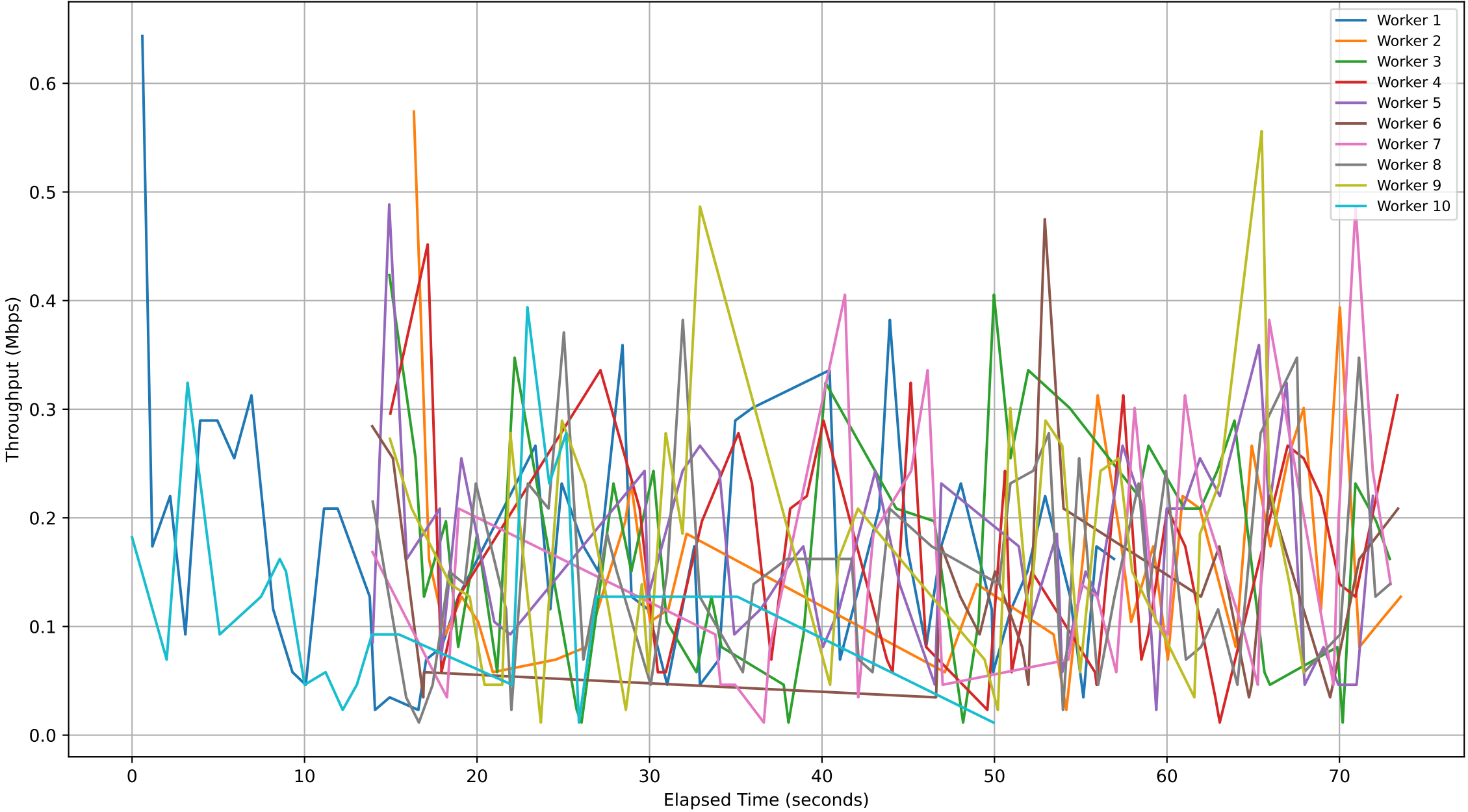
Subjob ID: 15fd166e-bf23-49c2-9d5c-fd07b55e3b43 - Workers Throughput Over Time
