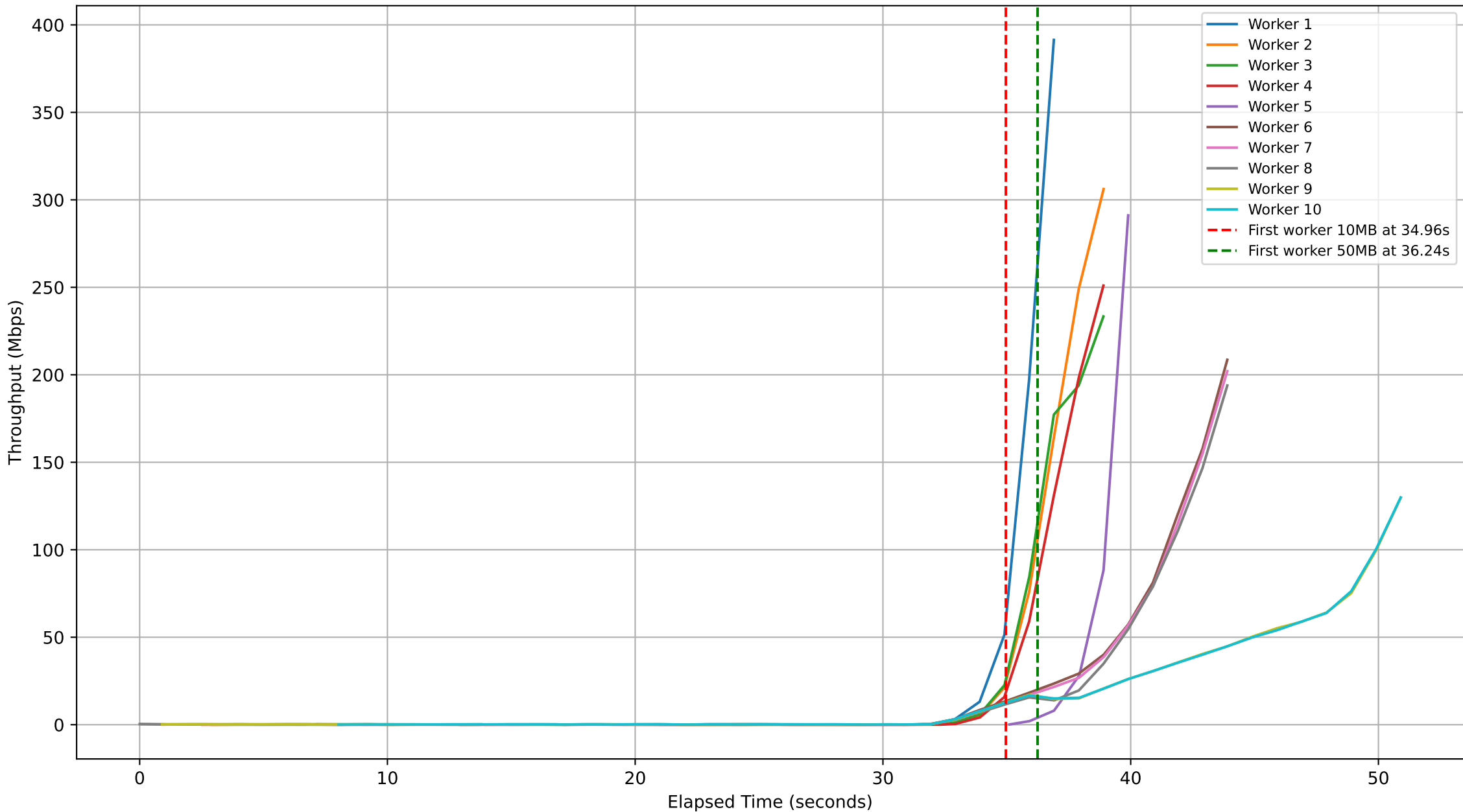
Subjob ID: e22d95c0-6b7e-42ae-8302-cd1e121fffb4 - Workers Throughput Over Time
