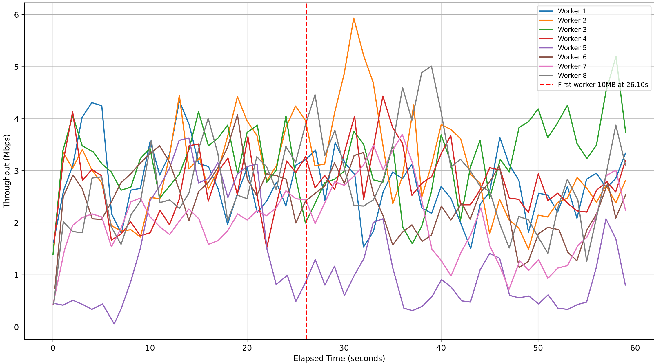
Subjob ID: 9401c51e-bd64-45ce-88a0-f9a5ecc224fc - Workers Throughput Over Time
