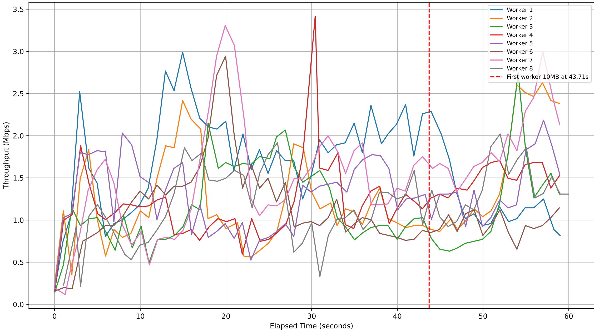
Subjob ID: d2e19aa5-8593-46b0-8733-e6cade2d302e - Workers Throughput Over Time
