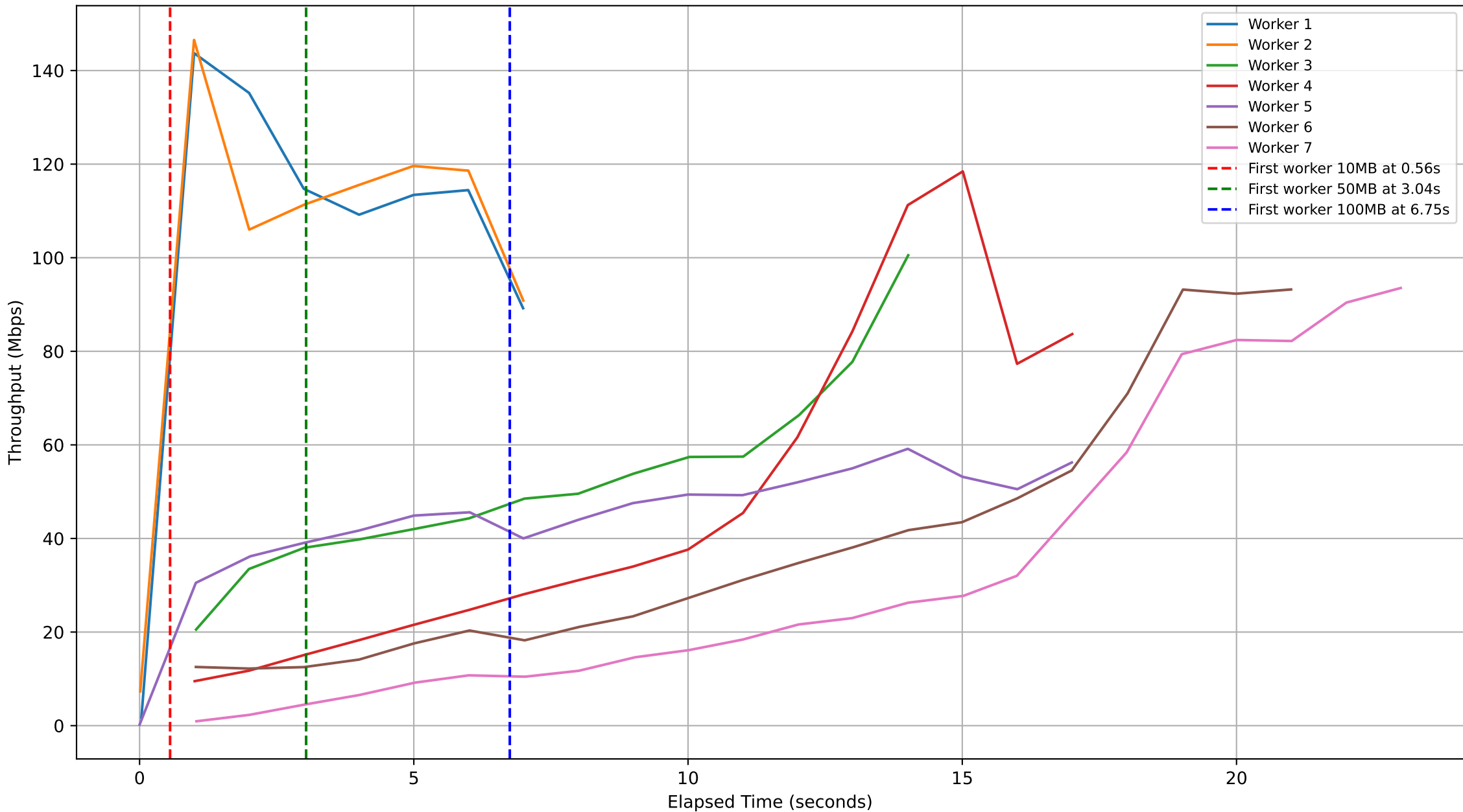
Subjob ID: c1cf686f-a822-4676-8227-2e8f33d70c33 - Workers Throughput Over Time
