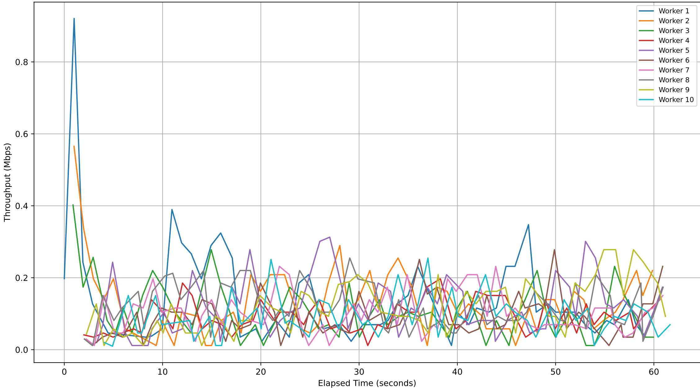
Subjob ID: 5d8af224-0d10-405b-a134-8635bd3e5d4d - Workers Throughput Over Time
