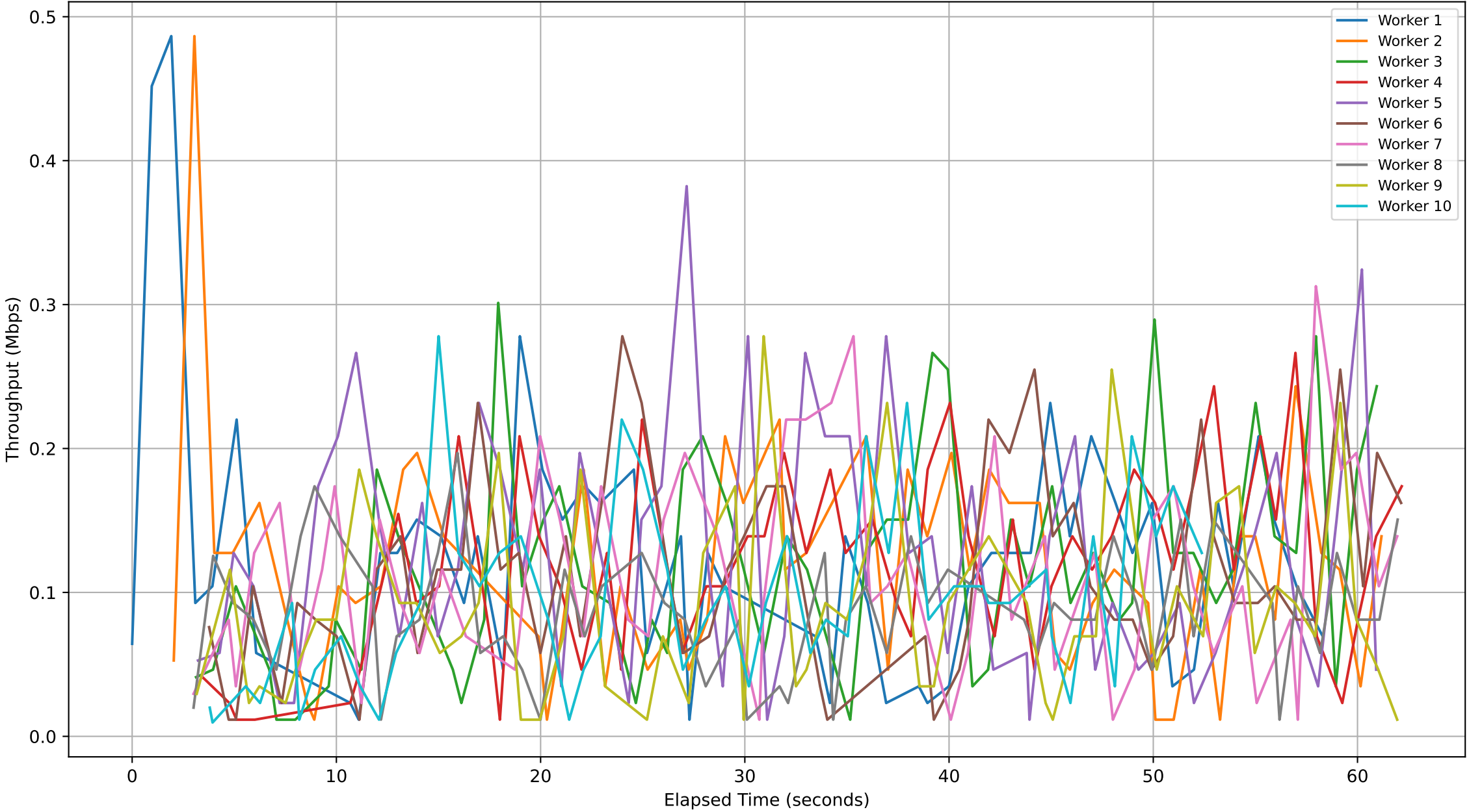
Subjob ID: 0890c051-ba3b-4b3a-9bdf-41fcc88c743c - Workers Throughput Over Time
