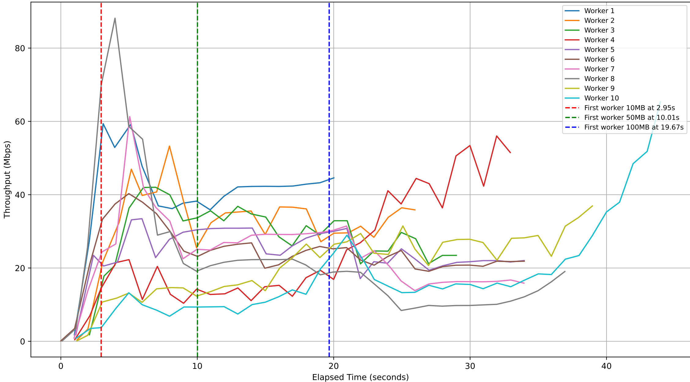
Subjob ID: b64e9450-e294-4bd6-a13c-17545105f102 - Workers Throughput Over Time
