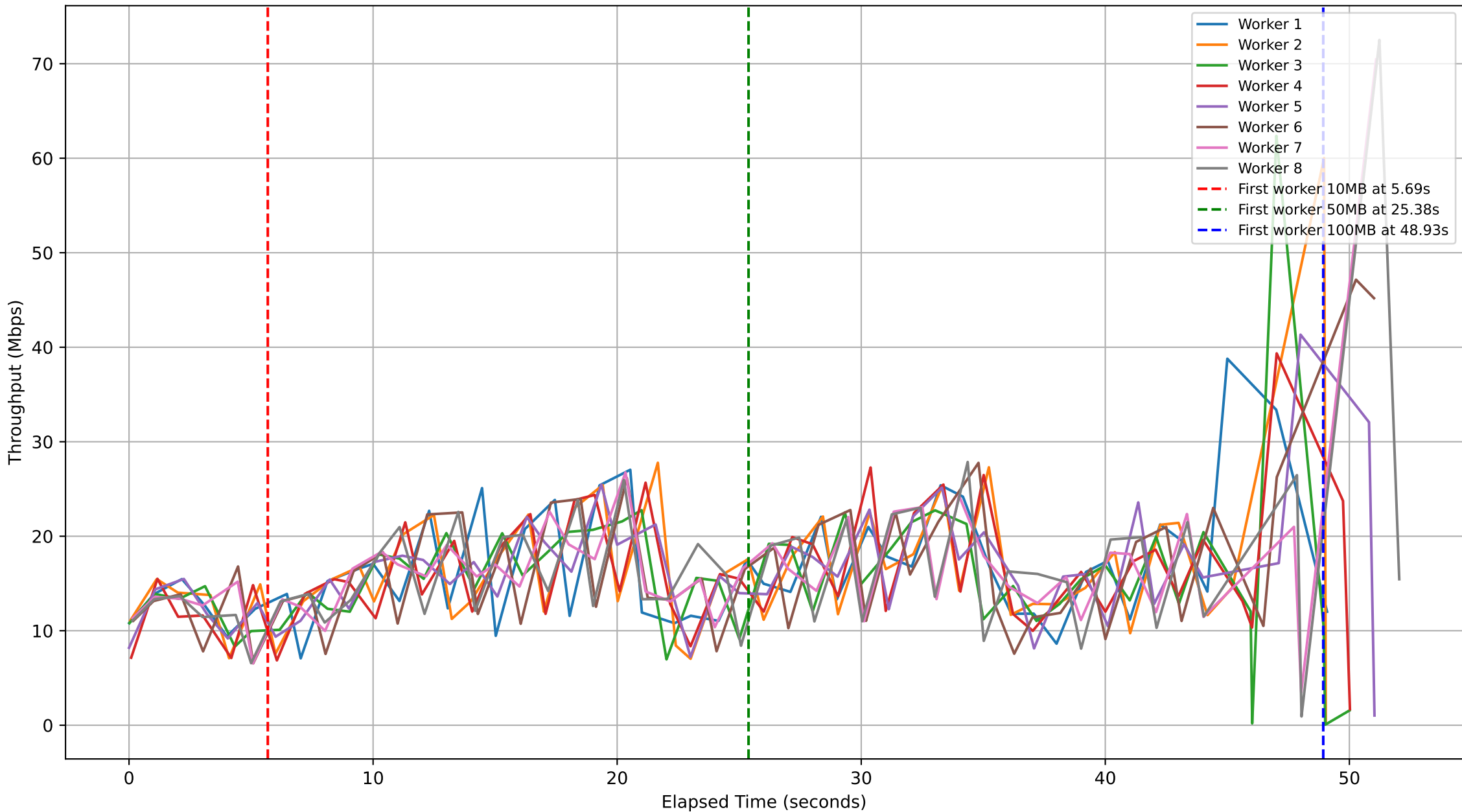
Subjob ID: 517f317f-7108-48be-99a6-78118eb16adb - Workers Throughput Over Time
