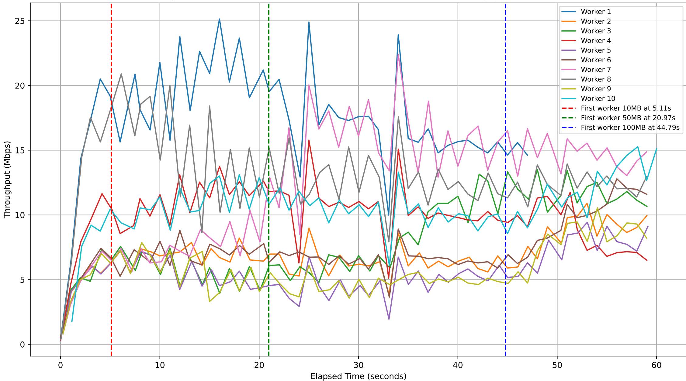
Subjob ID: 3f294494-3fe7-47fd-8f2a-f15a536fc8da - Workers Throughput Over Time
