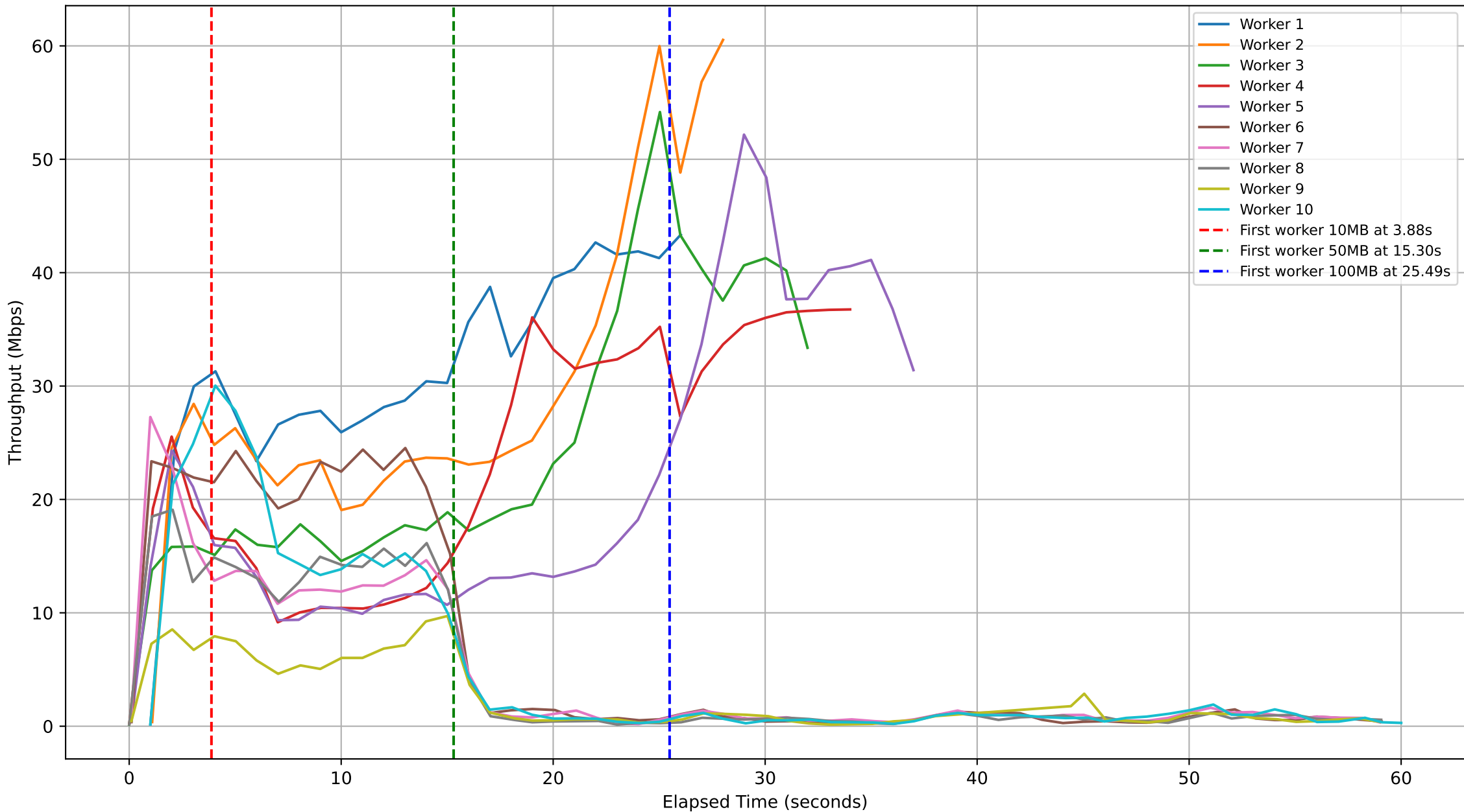
Subjob ID: 47e9c760-e666-4bc5-af42-1738748f8da5 - Workers Throughput Over Time
