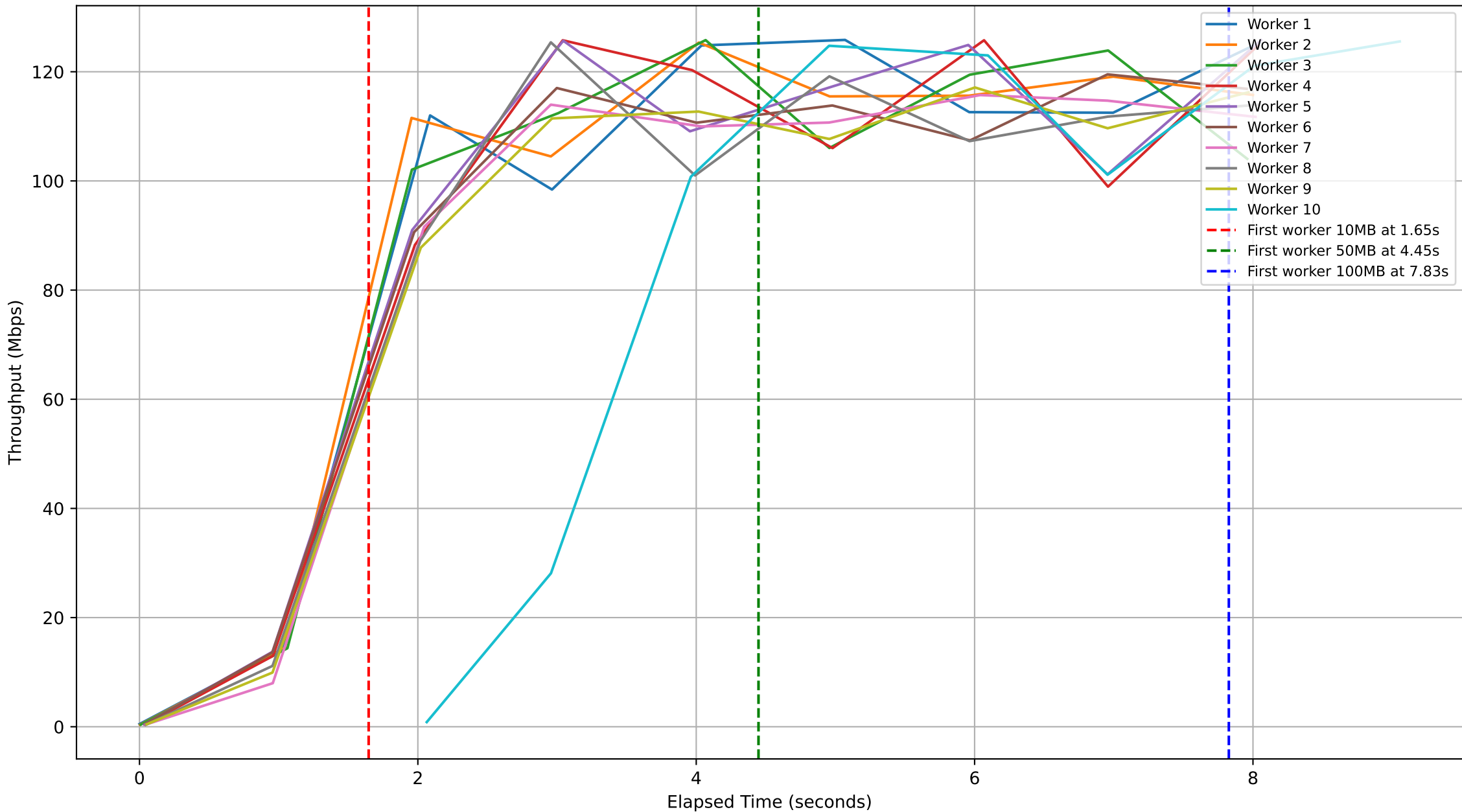
Subjob ID: dd144e66-a450-441f-88e6-2403277bccba - Workers Throughput Over Time
