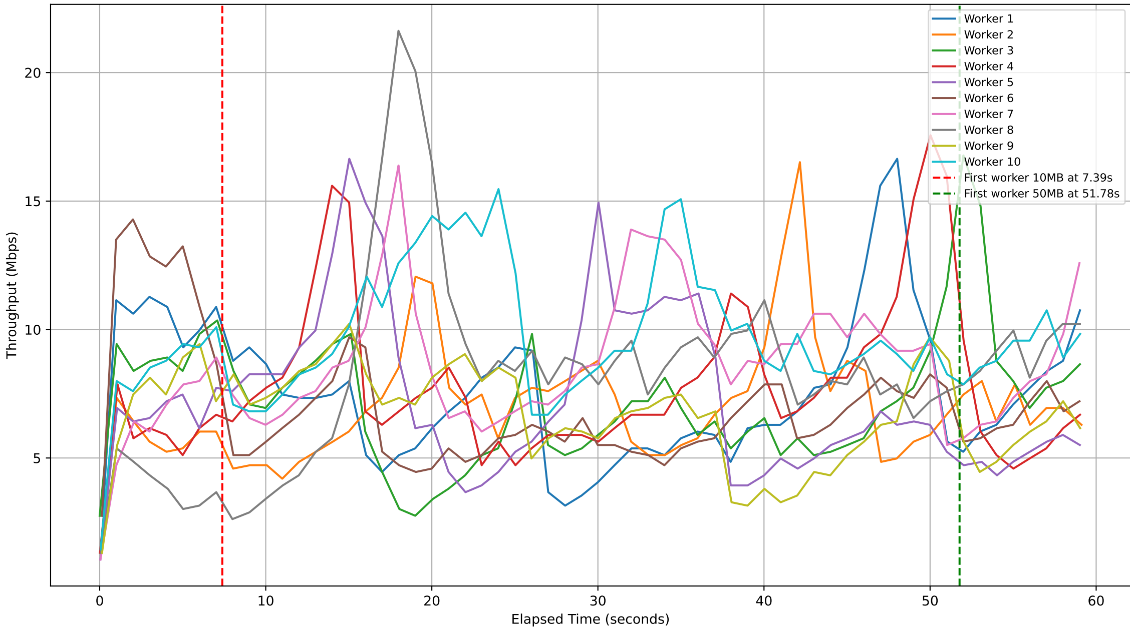
Subjob ID: b235412f-ba0b-4874-a638-e30c1c1abc3a - Workers Throughput Over Time
