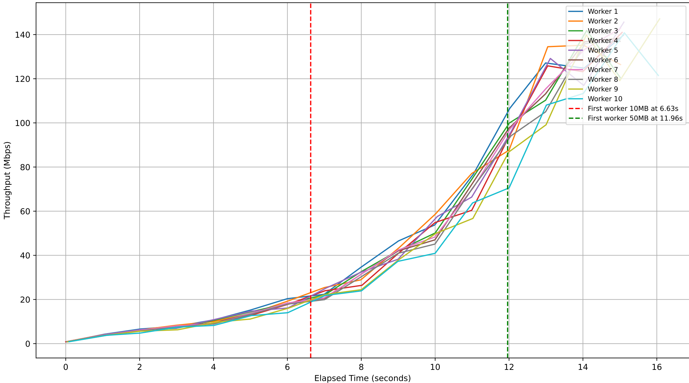
Subjob ID: 6436bbc6-8cb3-455b-9fc5-b0e7a932c08f - Workers Throughput Over Time
