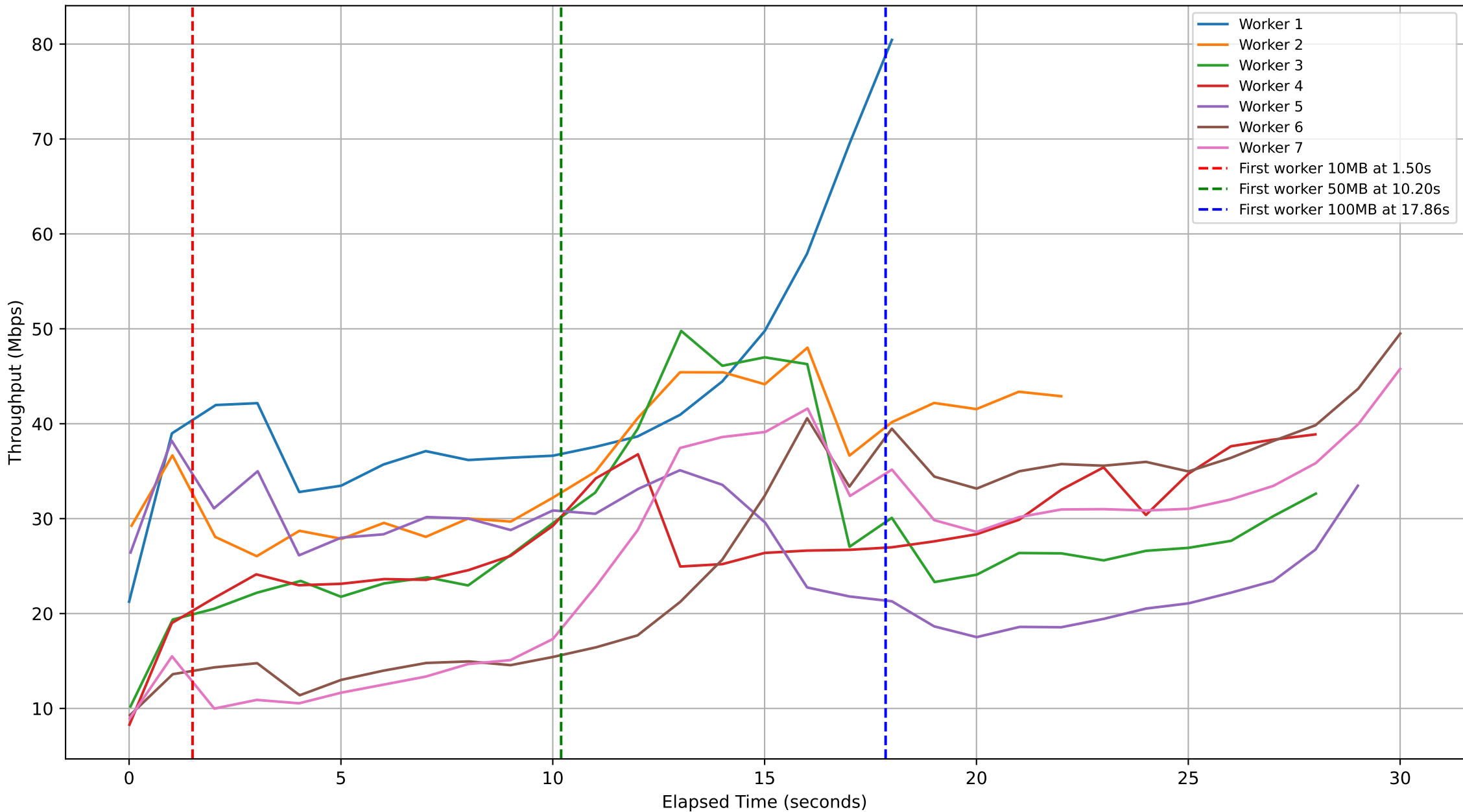
Subjob ID: 9f342142-275c-498d-9b47-8f953ec3b8bf - Workers Throughput Over Time
