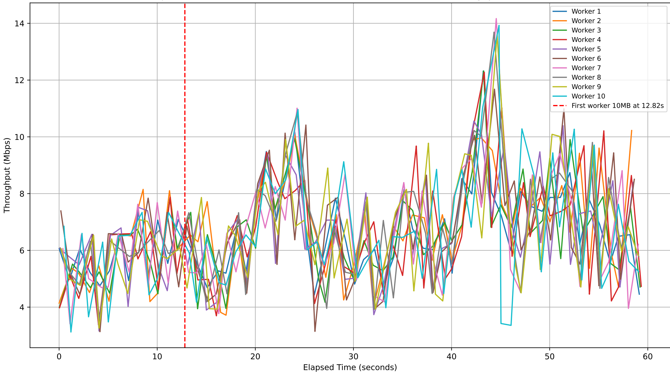
Subjob ID: 498d2432-ba1a-411c-be6b-530cd9af24e2 - Workers Throughput Over Time
