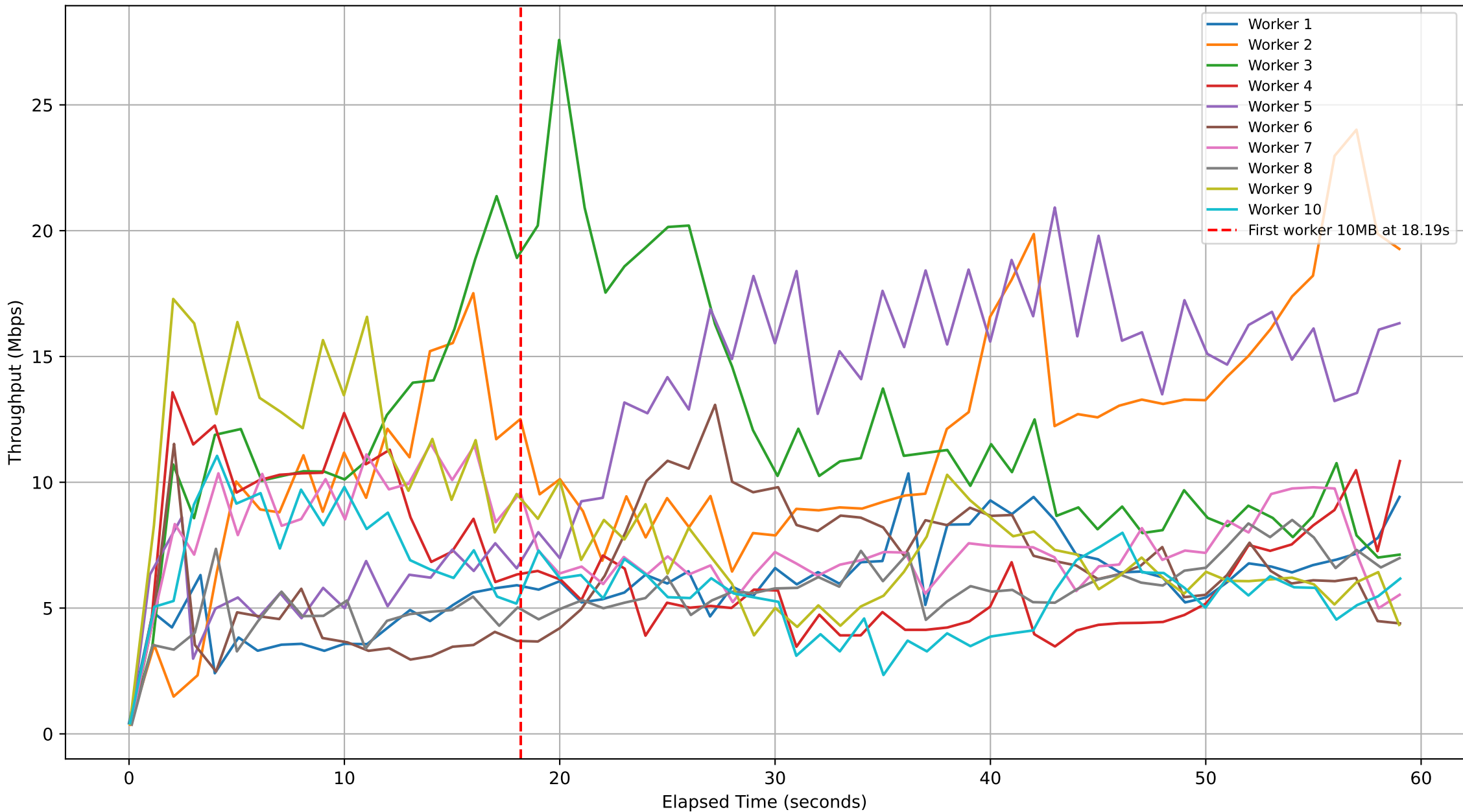
Subjob ID: 114e3e17-1cc1-4189-9350-8d8b23a568d0 - Workers Throughput Over Time
