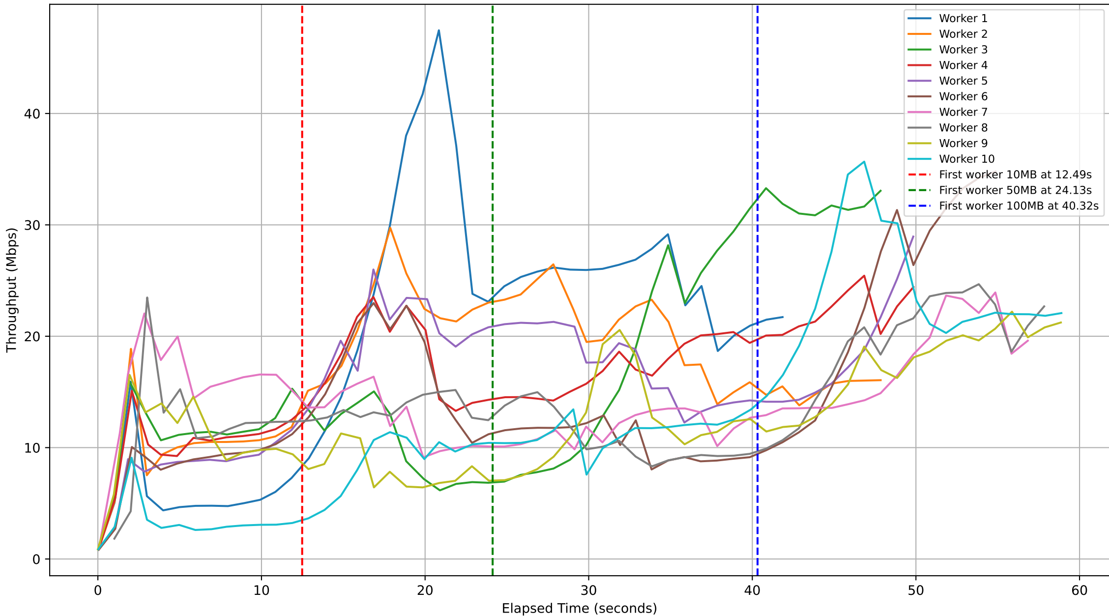
Subjob ID: 0a24427b-64cc-43b0-b525-529cce258e6c - Workers Throughput Over Time
