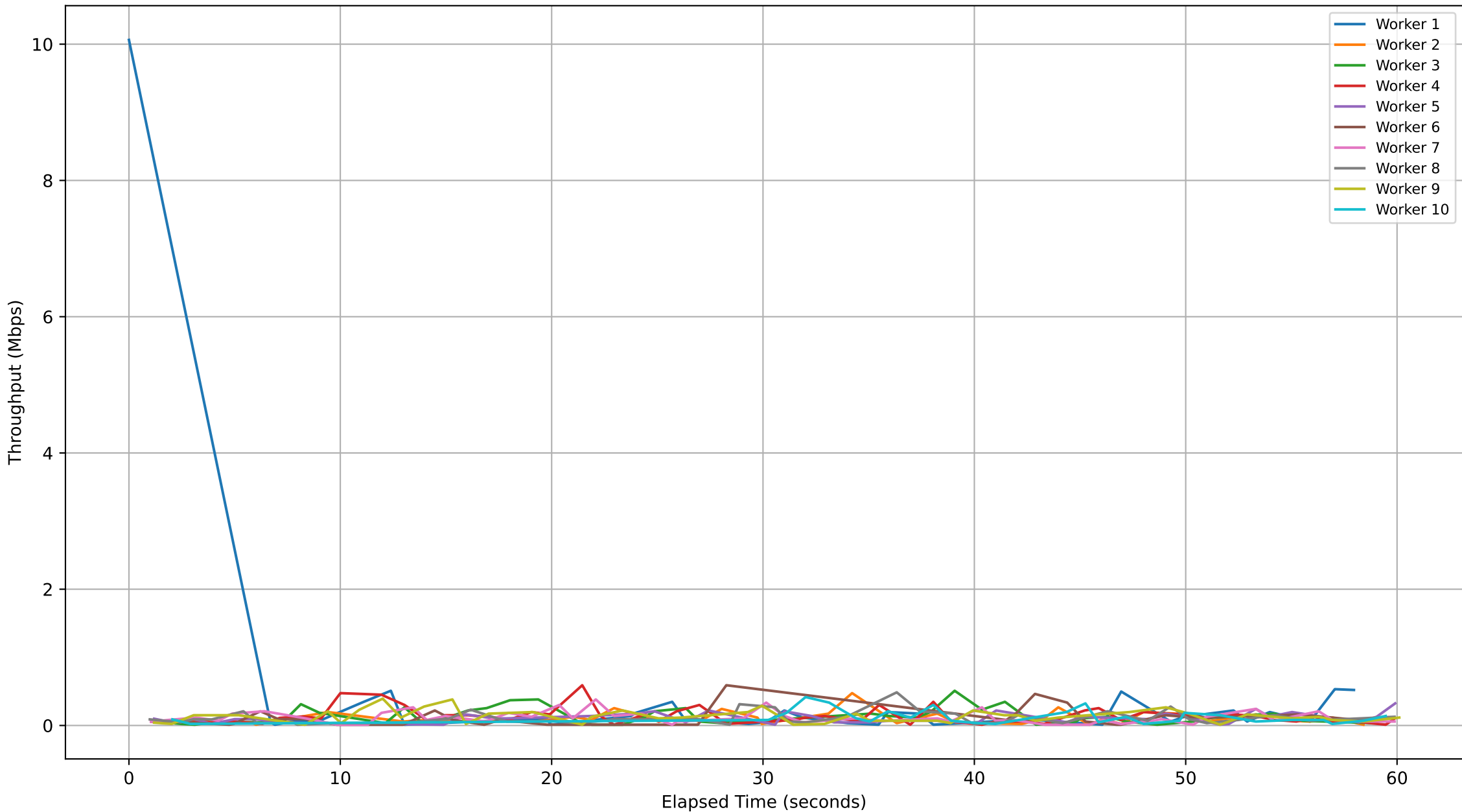
Subjob ID: 83590a9f-1097-4efd-be32-8e97ea6197ca - Workers Throughput Over Time
