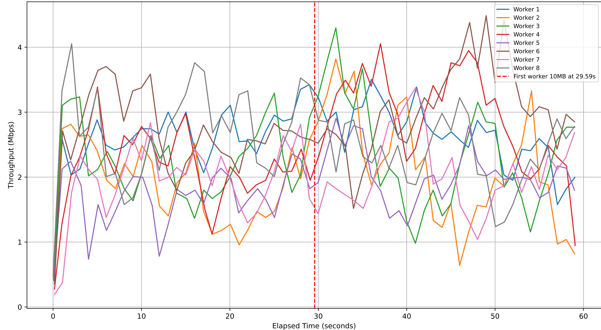
Subjob ID: a057e966-83a9-47e6-bf0f-b84c65994c34 - Workers Throughput Over Time
