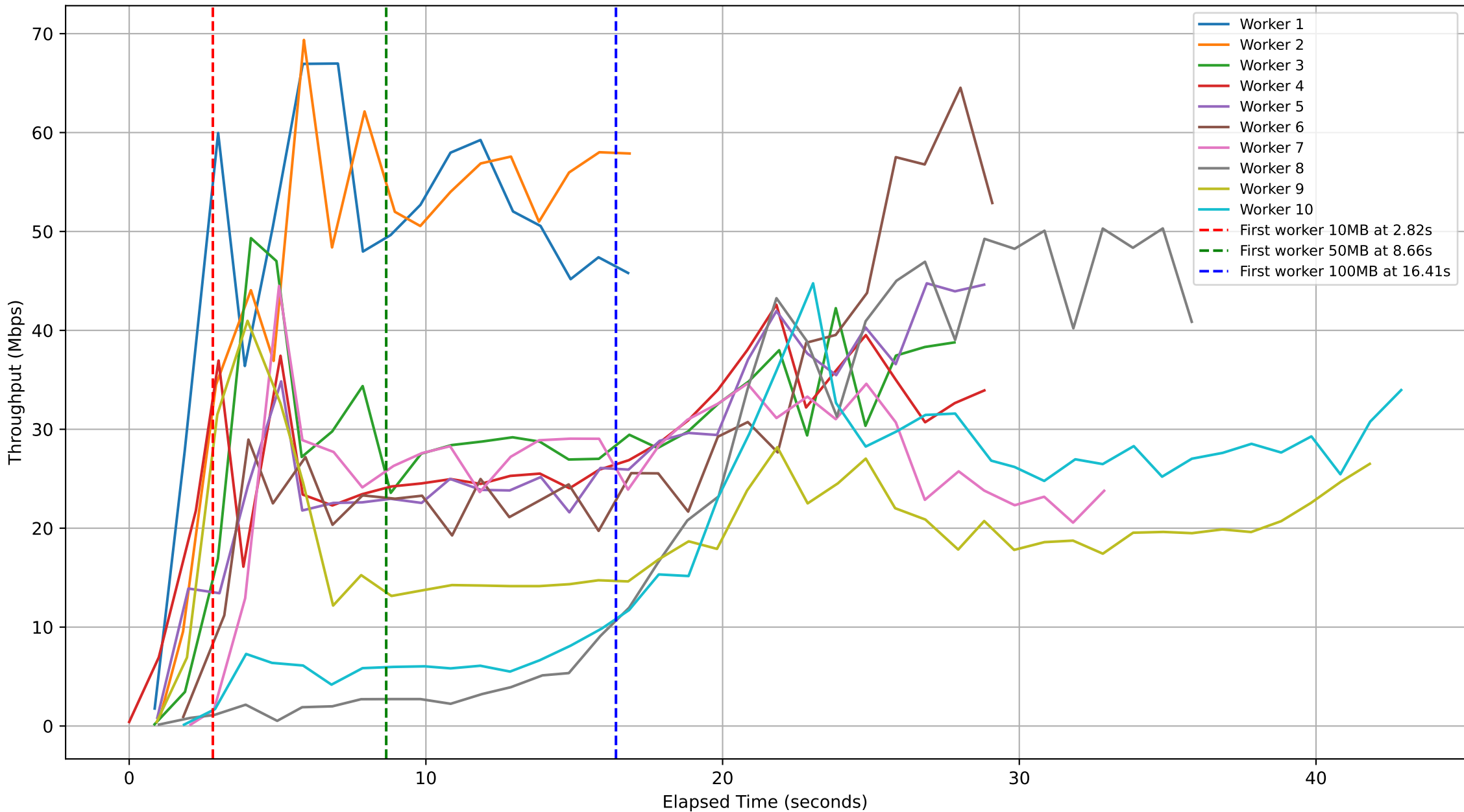
Subjob ID: ba69ad08-aa04-4401-9b76-53768b15554a - Workers Throughput Over Time
