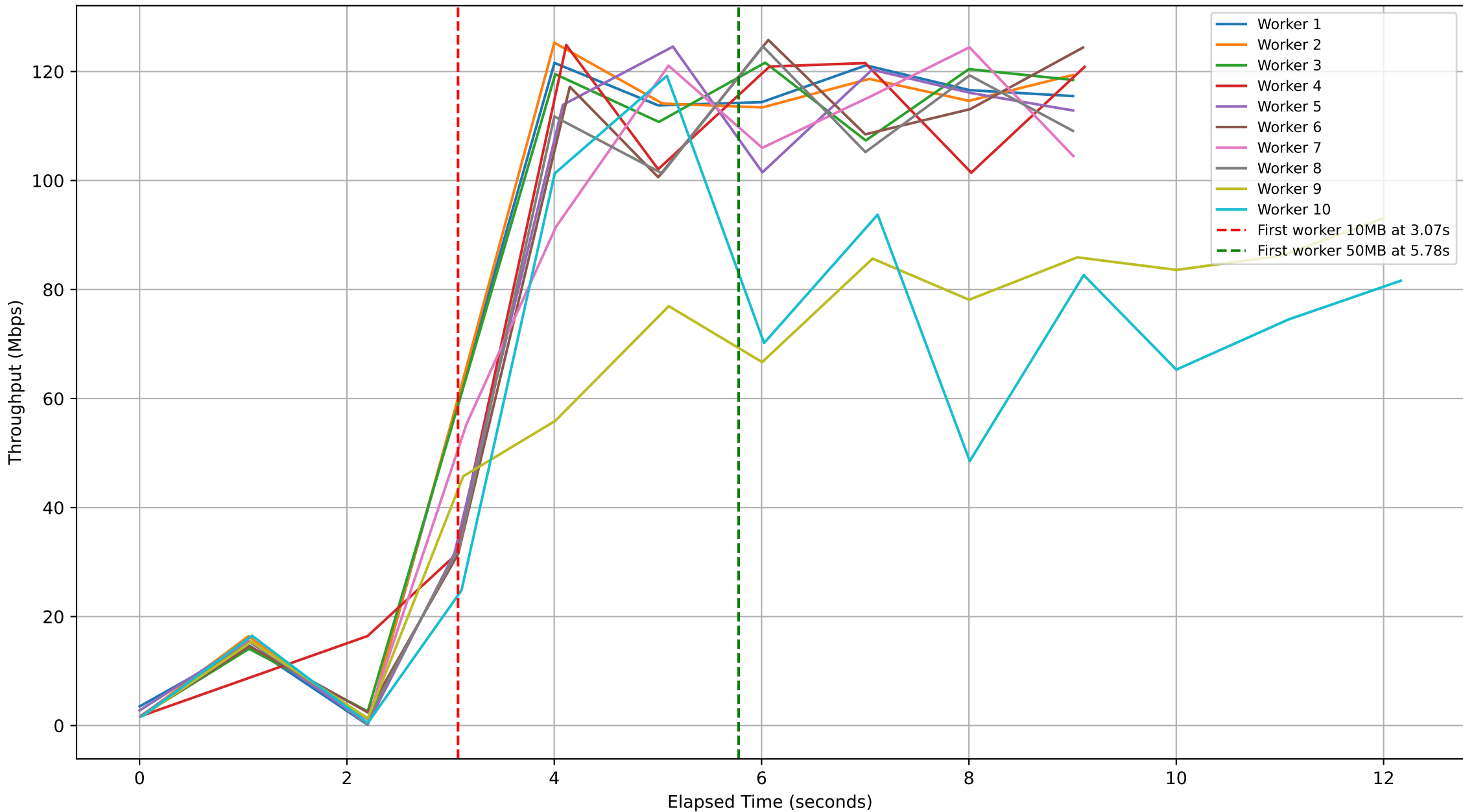
Subjob ID: 22b23c8d-cf13-44c6-99c0-f6da535d7c30 - Workers Throughput Over Time
