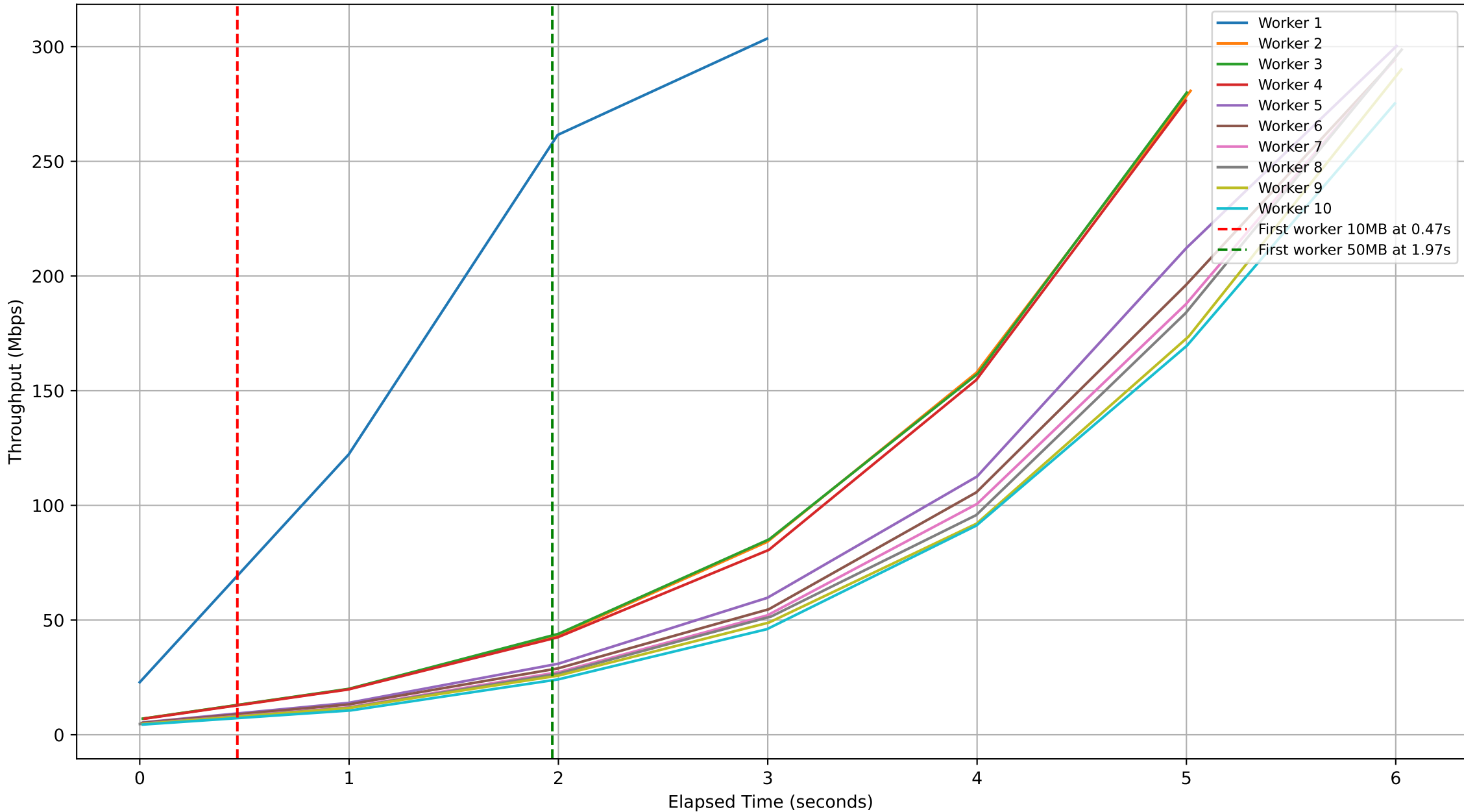
Subjob ID: 91054405-330d-4f3d-b648-b8ee64527891 - Workers Throughput Over Time
