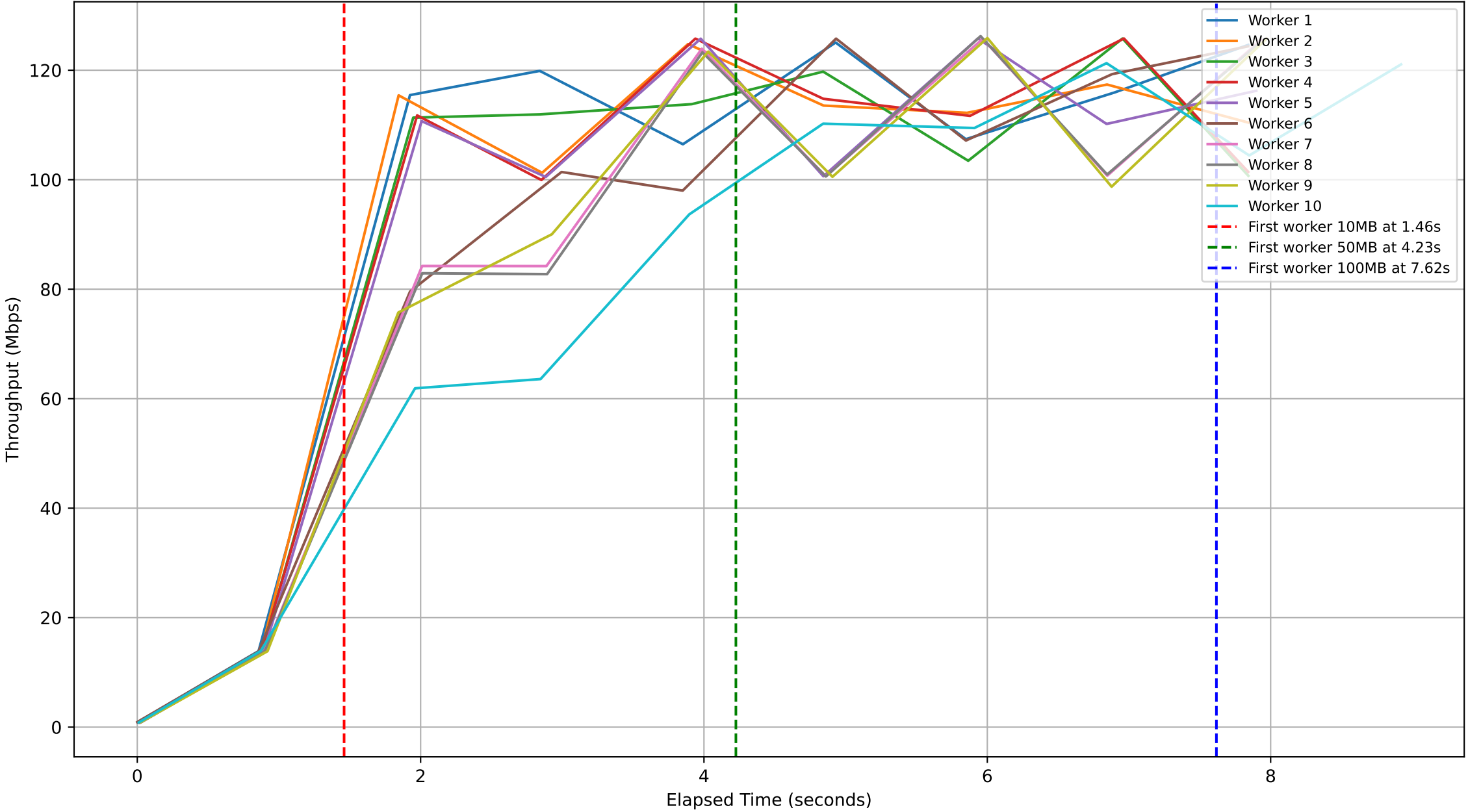
Subjob ID: bb3e9226-f97d-4df5-8ed5-6e6b85816b91 - Workers Throughput Over Time
