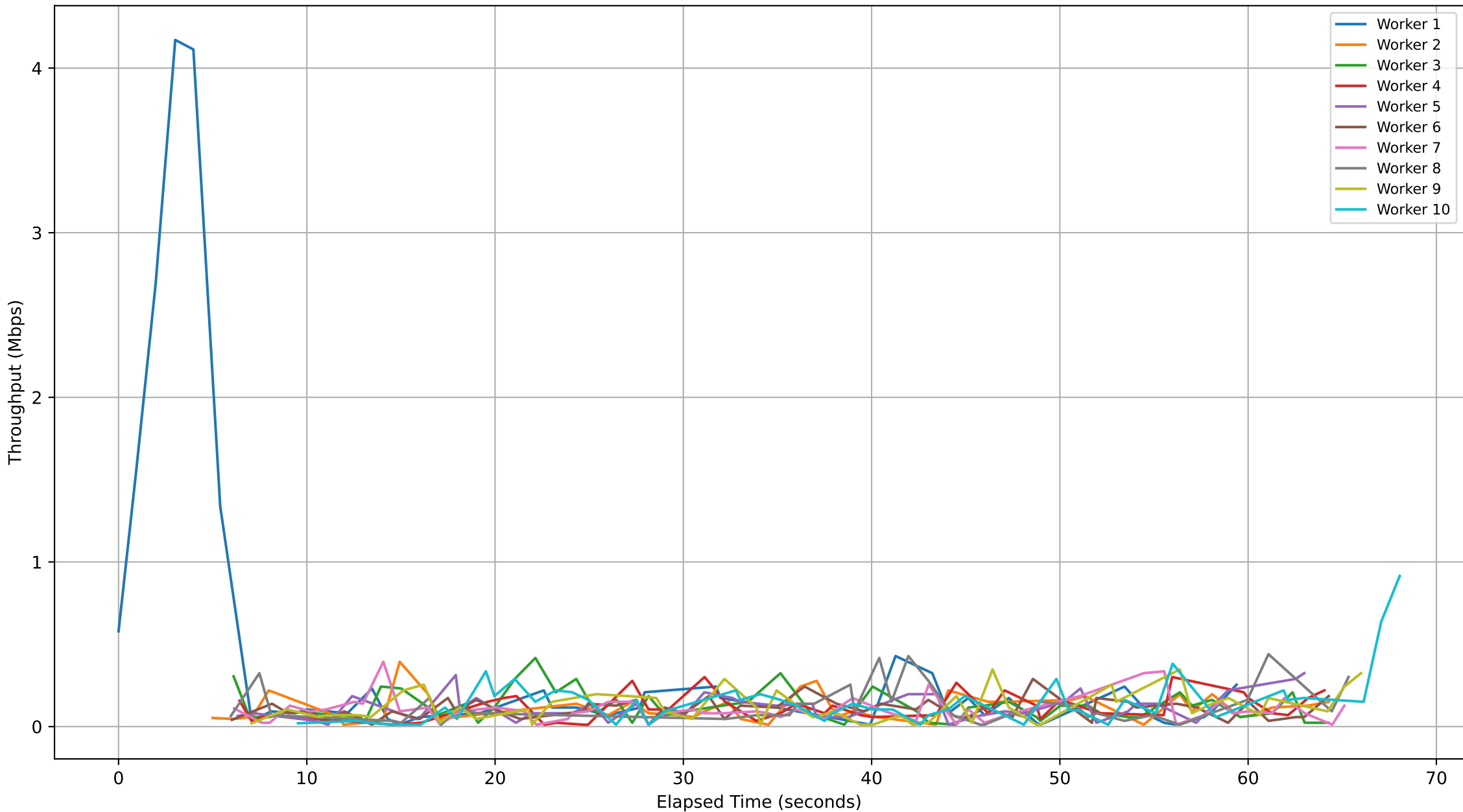
Subjob ID: 4dc5f42f-8962-4831-a828-b021123d7b02 - Workers Throughput Over Time
