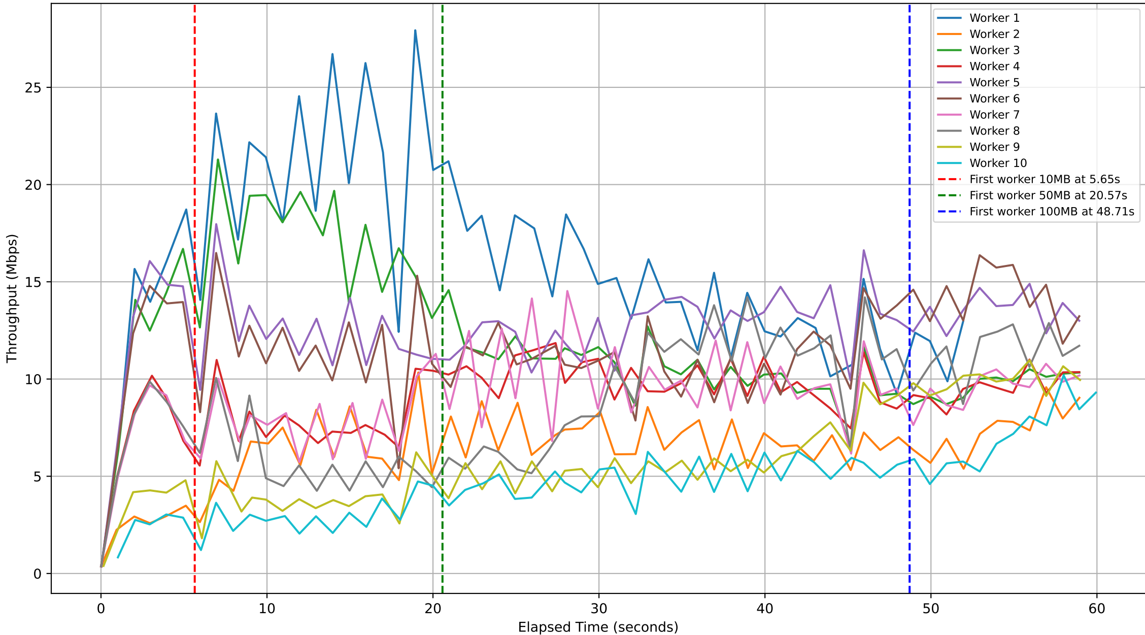
Subjob ID: cab055bc-39d4-40a0-a59f-d34e3a3f2359 - Workers Throughput Over Time
