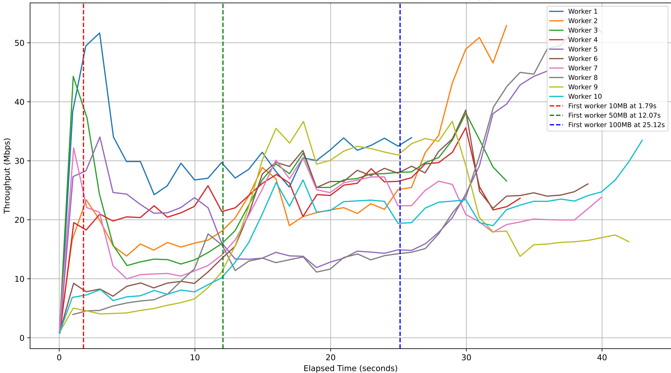
Subjob ID: 530ab850-70c0-4a33-819c-c638477bb3f3 - Workers Throughput Over Time
