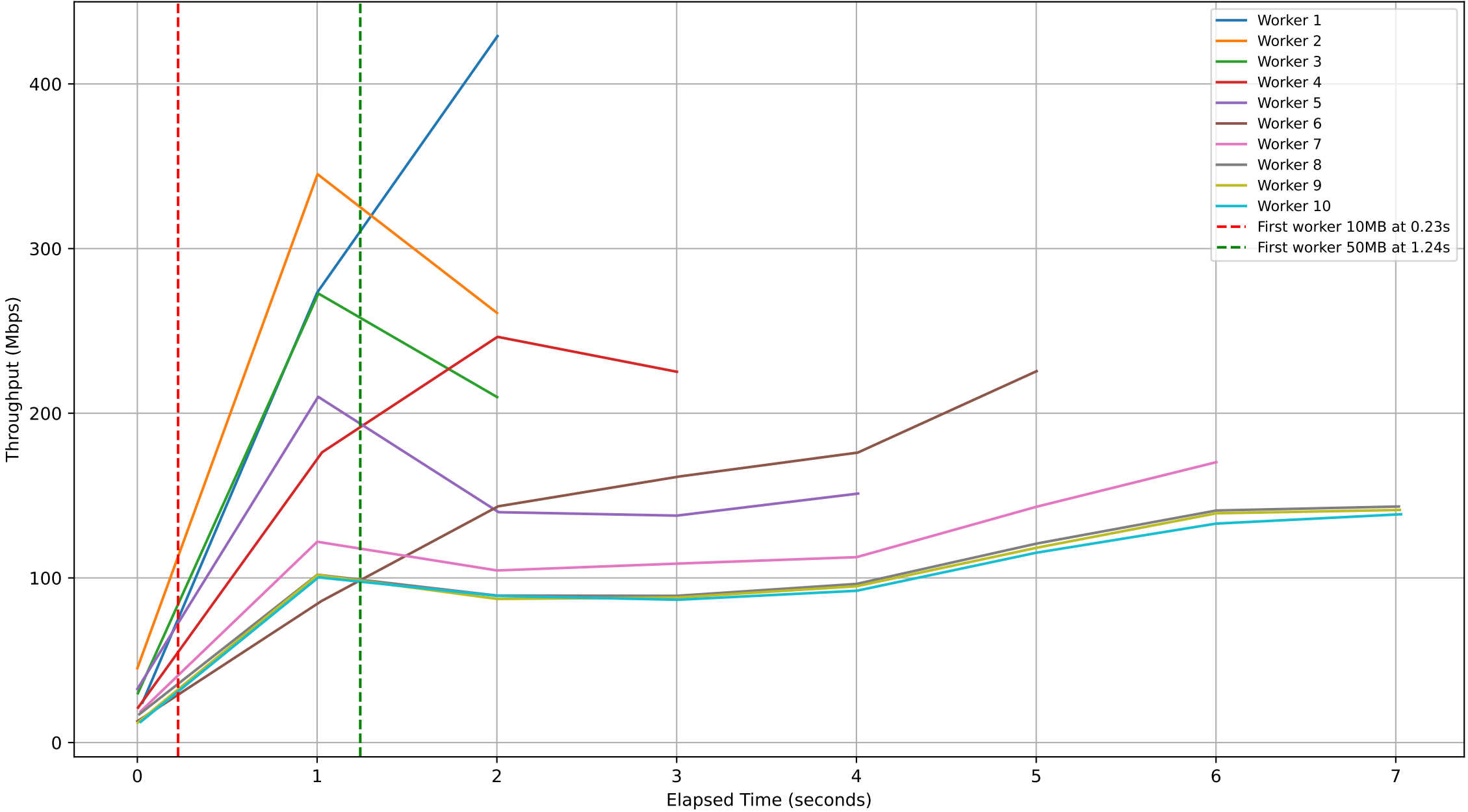
Subjob ID: db0ccf59-602c-45bc-8a49-4a334853400c - Workers Throughput Over Time
