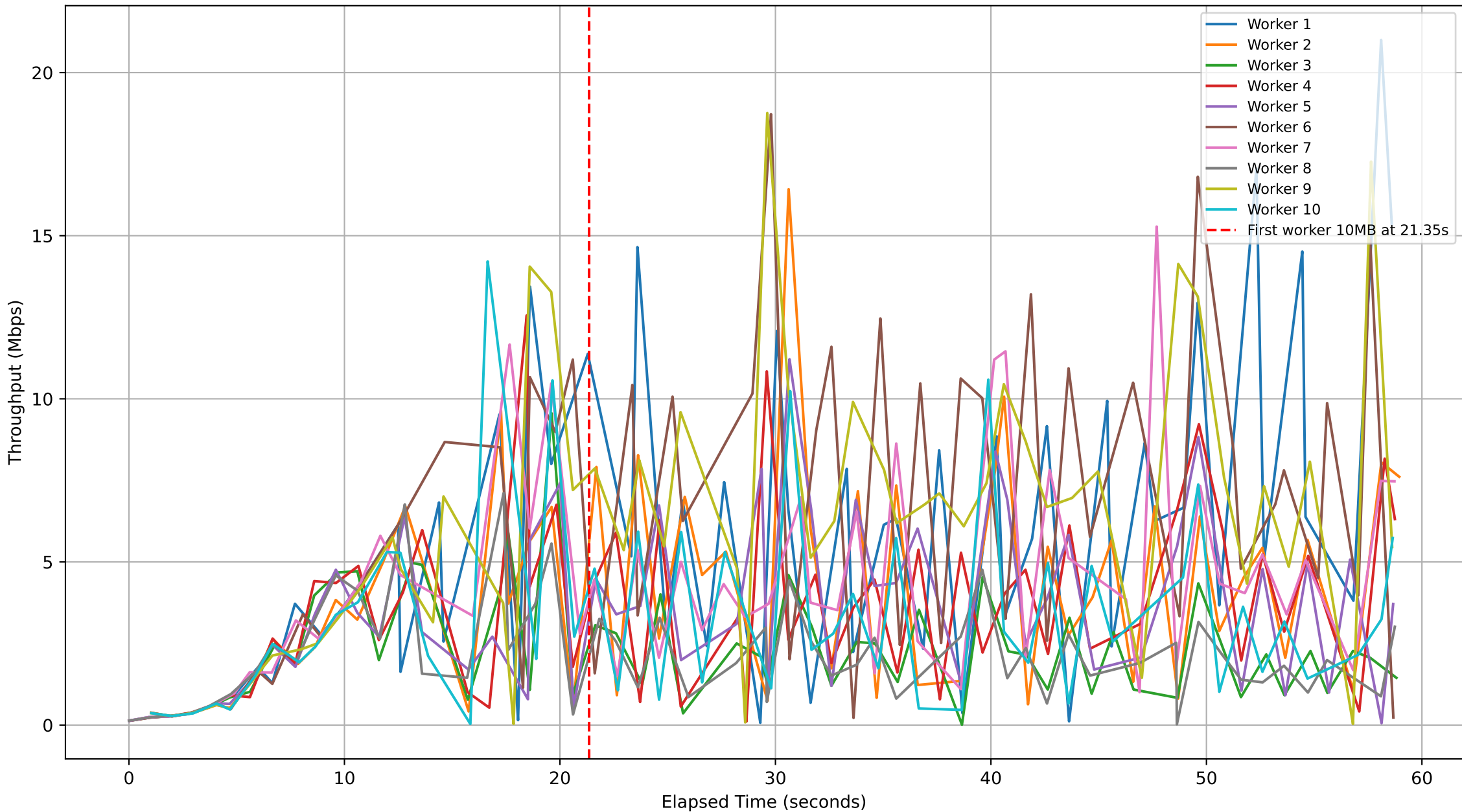
Subjob ID: 1d4904ce-c854-45bc-a9cb-a4111fd954d3 - Workers Throughput Over Time
