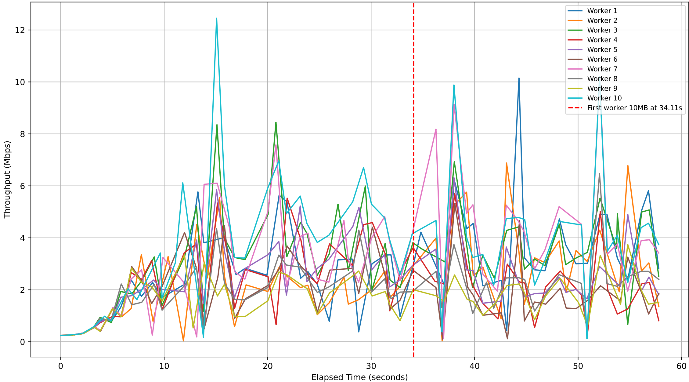
Subjob ID: 210c79e9-f8db-48a7-ad72-414605ca7f90 - Workers Throughput Over Time
