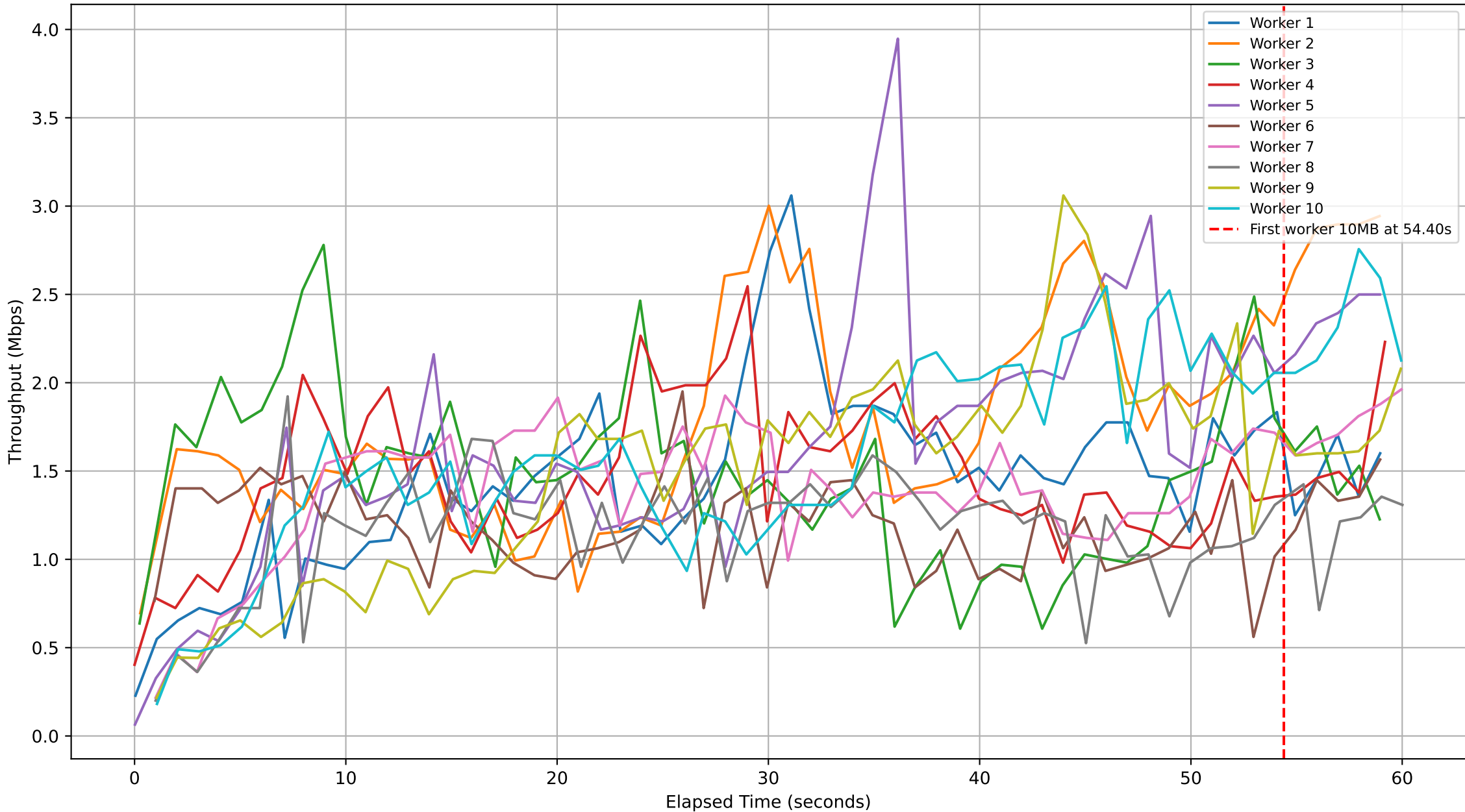
Subjob ID: ab66b178-317a-43bd-b6da-70da8fe155b9 - Workers Throughput Over Time
