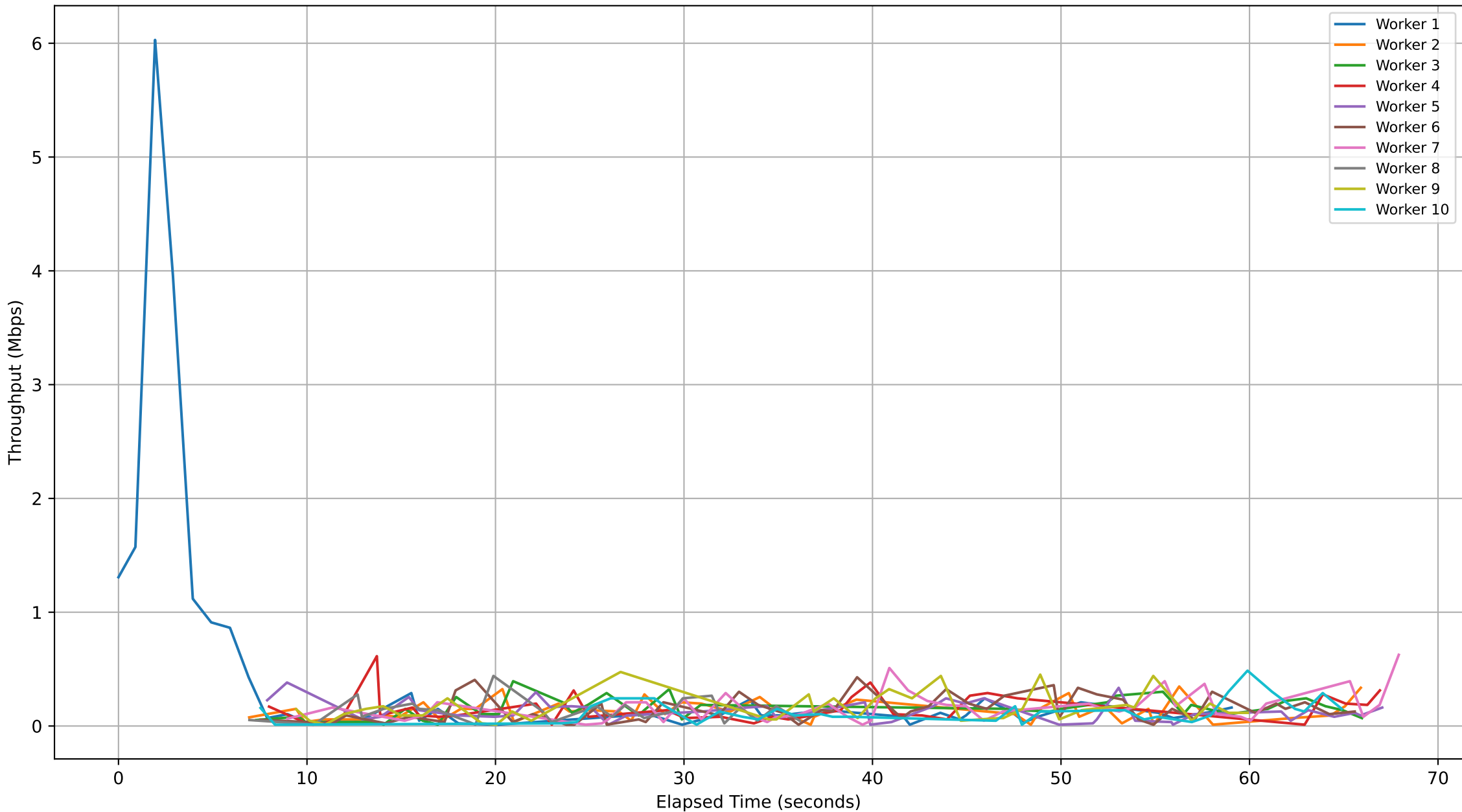
Subjob ID: 19765f0e-cb5e-4c73-8dde-e1c419eb8d84 - Workers Throughput Over Time
