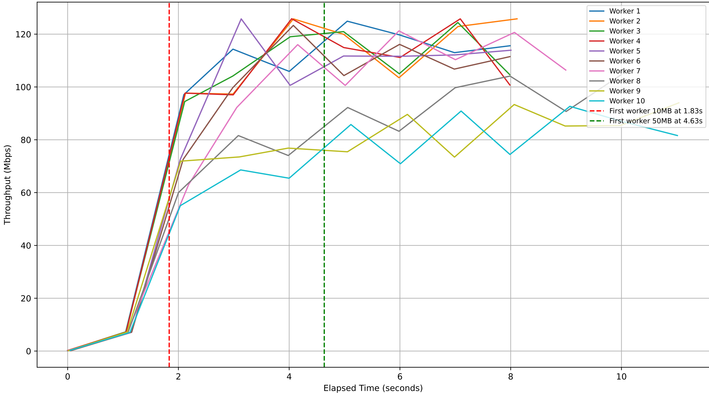
Subjob ID: f856950a-93b7-443f-8e06-7e1088e04376 - Workers Throughput Over Time
