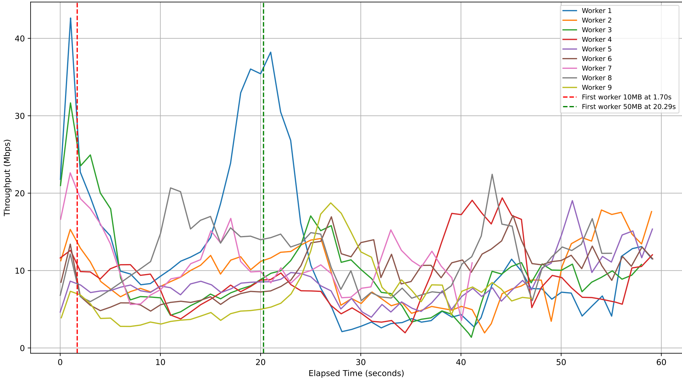
Subjob ID: 7846e223-742c-4253-8cc5-f5898dfb850b - Workers Throughput Over Time
