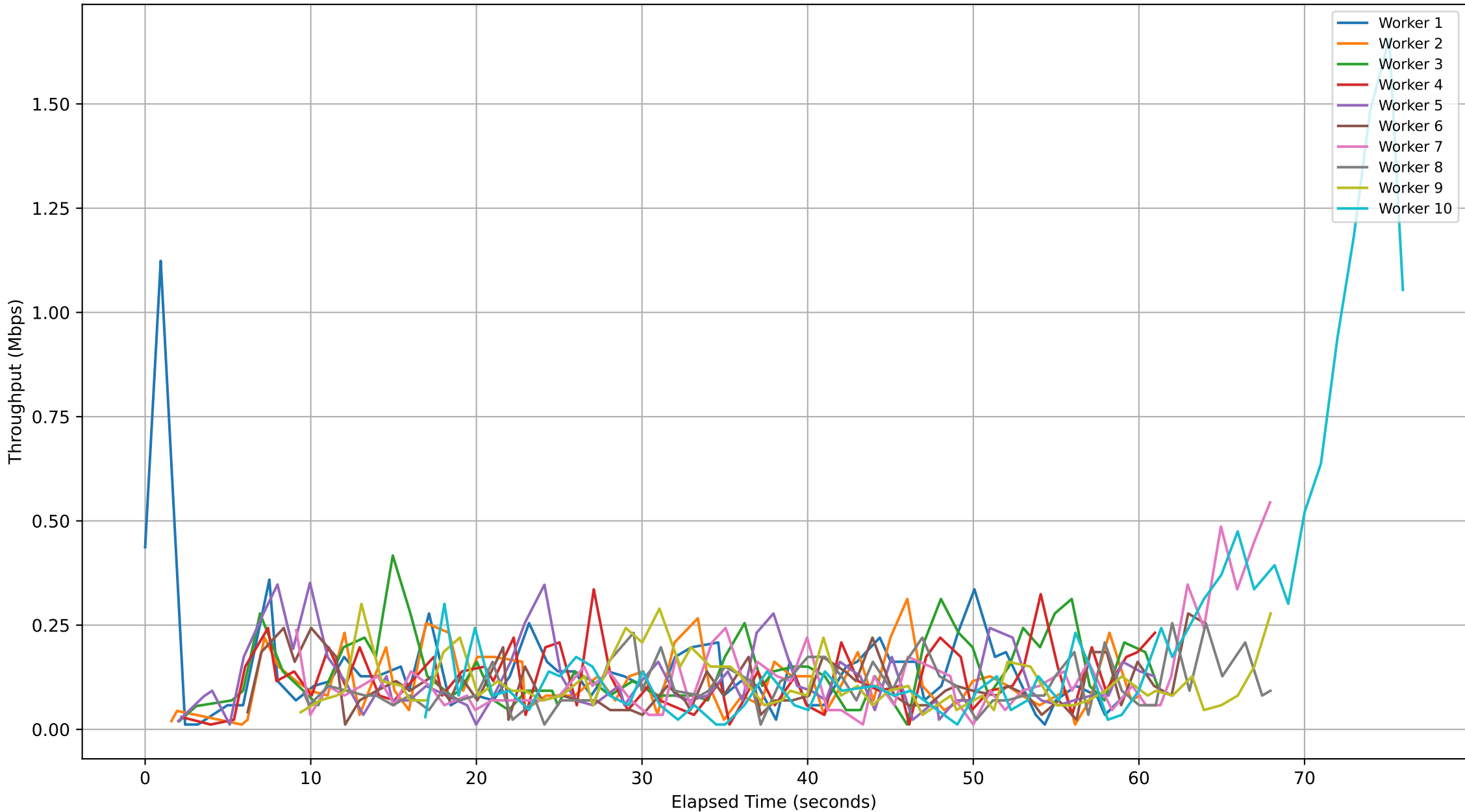
Subjob ID: 6790e508-ecdb-4e1d-b59c-01abd3086403 - Workers Throughput Over Time
