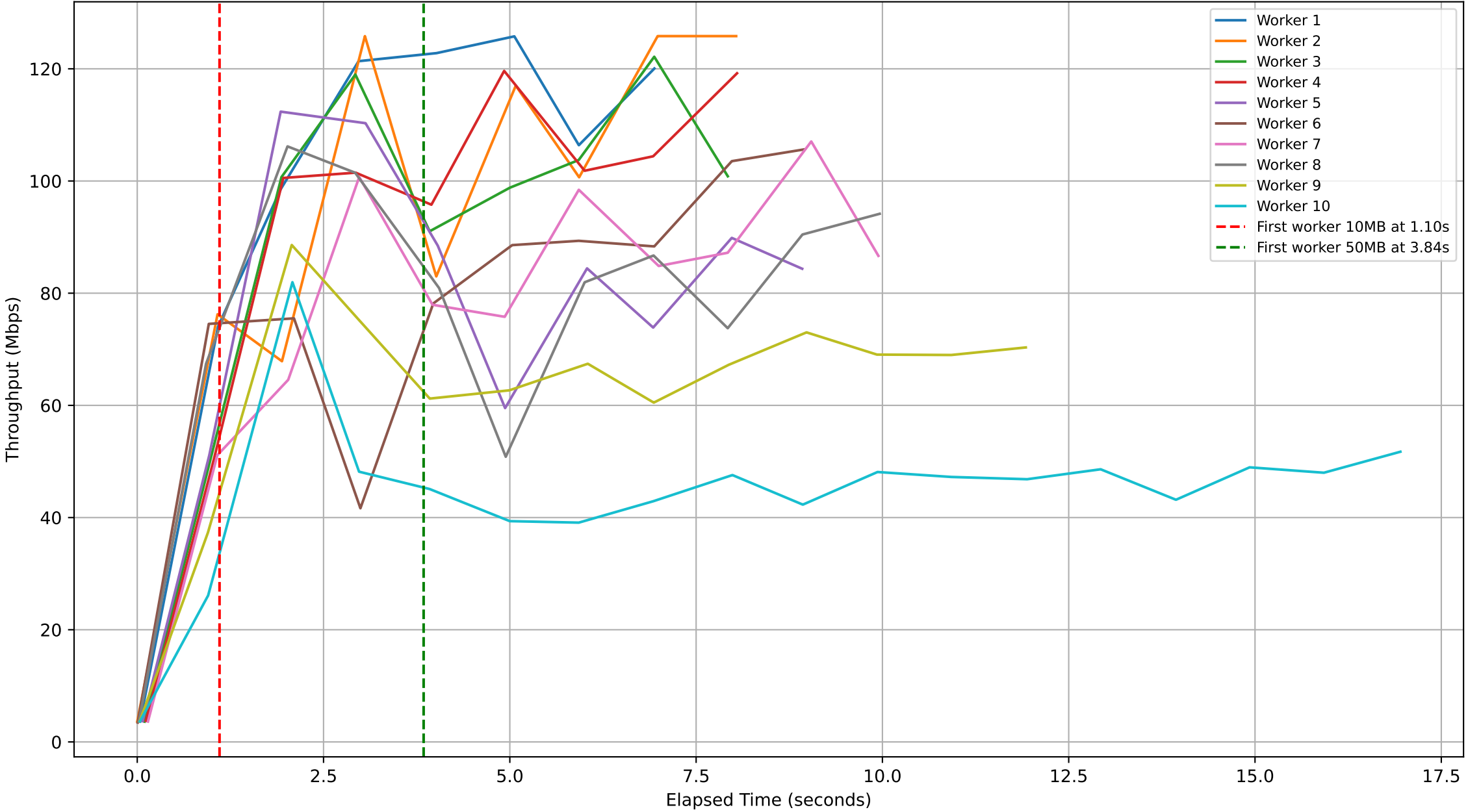
Subjob ID: 5ac2a361-c4f0-4522-9892-76e64fa473cd - Workers Throughput Over Time
