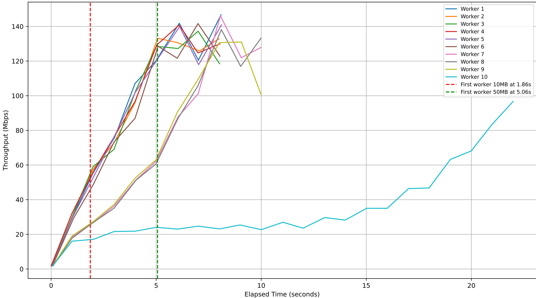
Subjob ID: a686db8a-50cc-4775-8295-e79df5e312e3 - Workers Throughput Over Time
