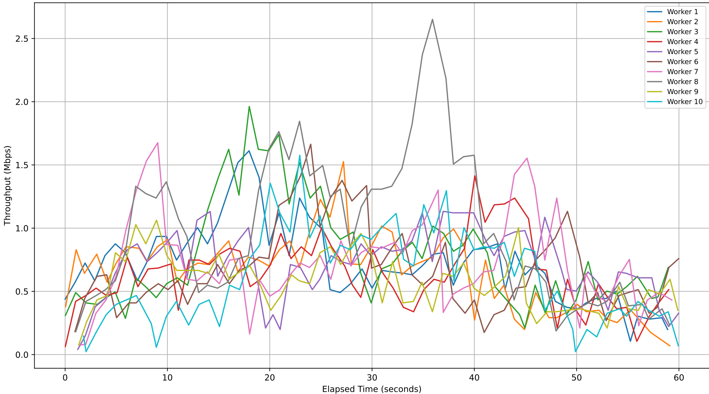
Subjob ID: 2c1b76dd-520f-47b1-bced-b4930b66f6b3 - Workers Throughput Over Time
