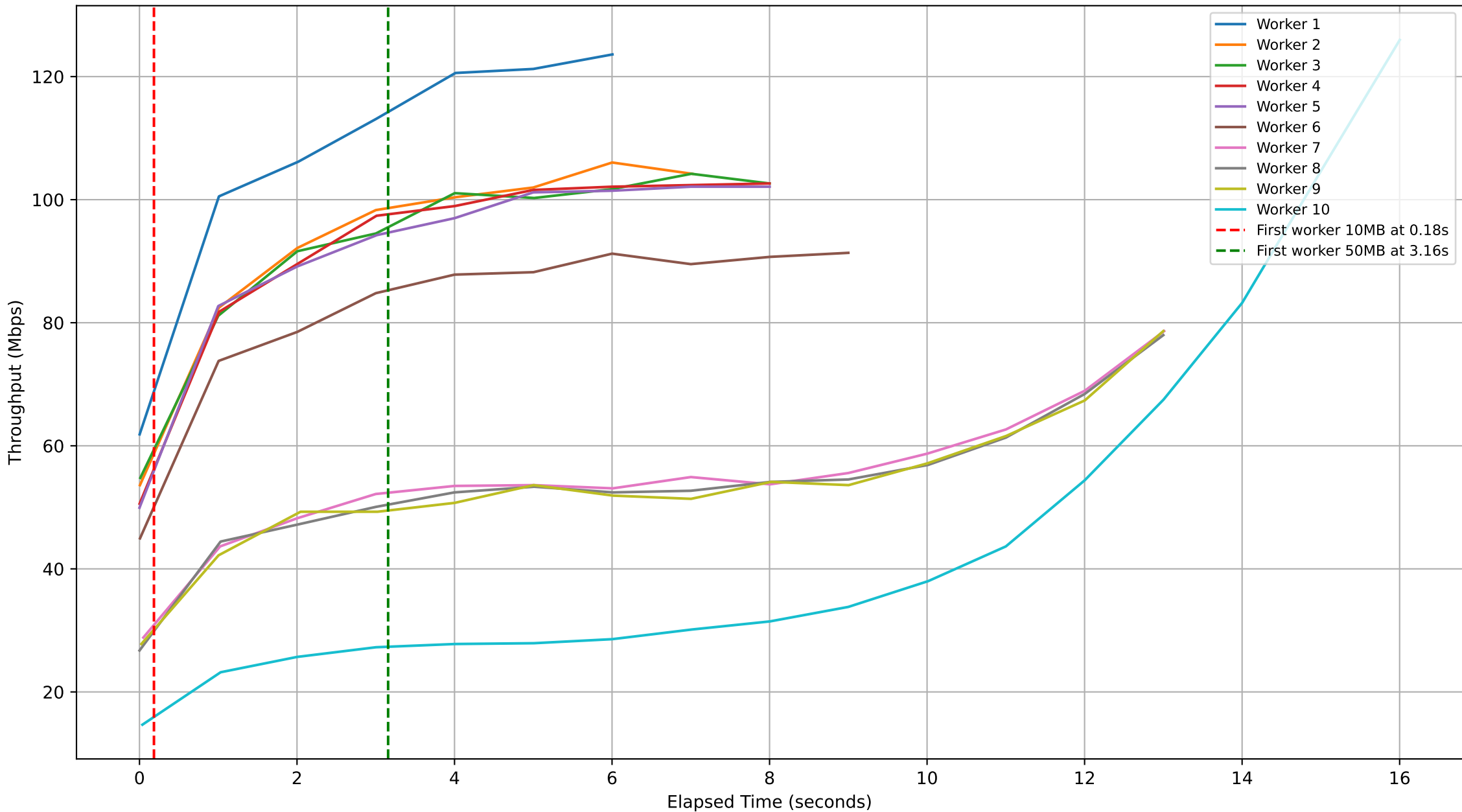
Subjob ID: a31d9578-11bc-40bb-a86d-aafcb8087458 - Workers Throughput Over Time
