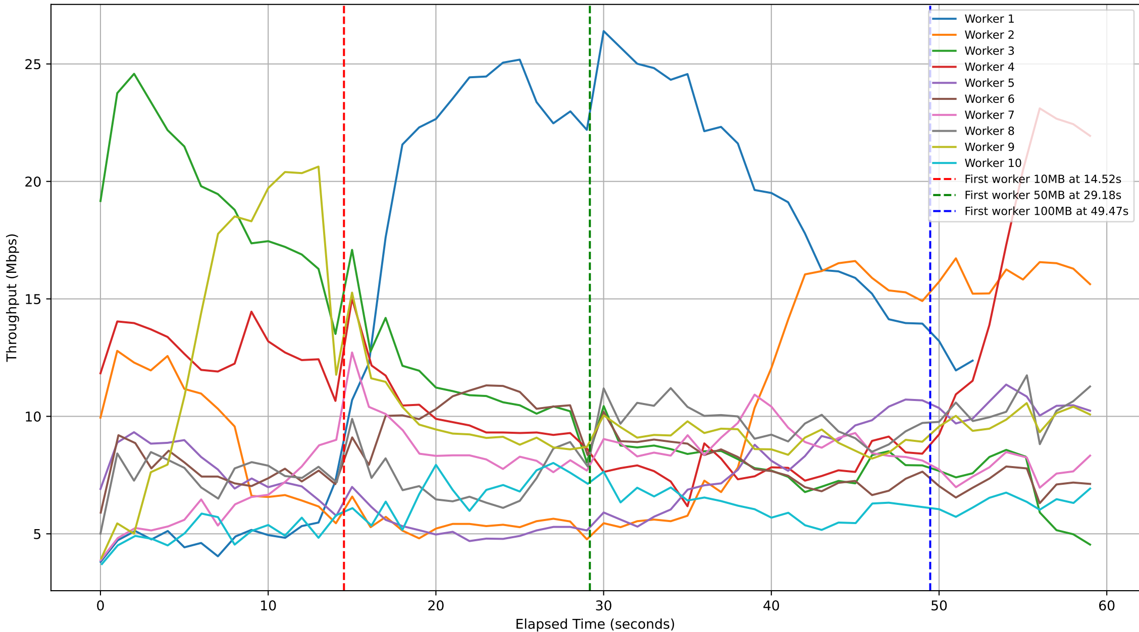
Subjob ID: 09f62e91-9705-464e-820b-827ac9983032 - Workers Throughput Over Time
