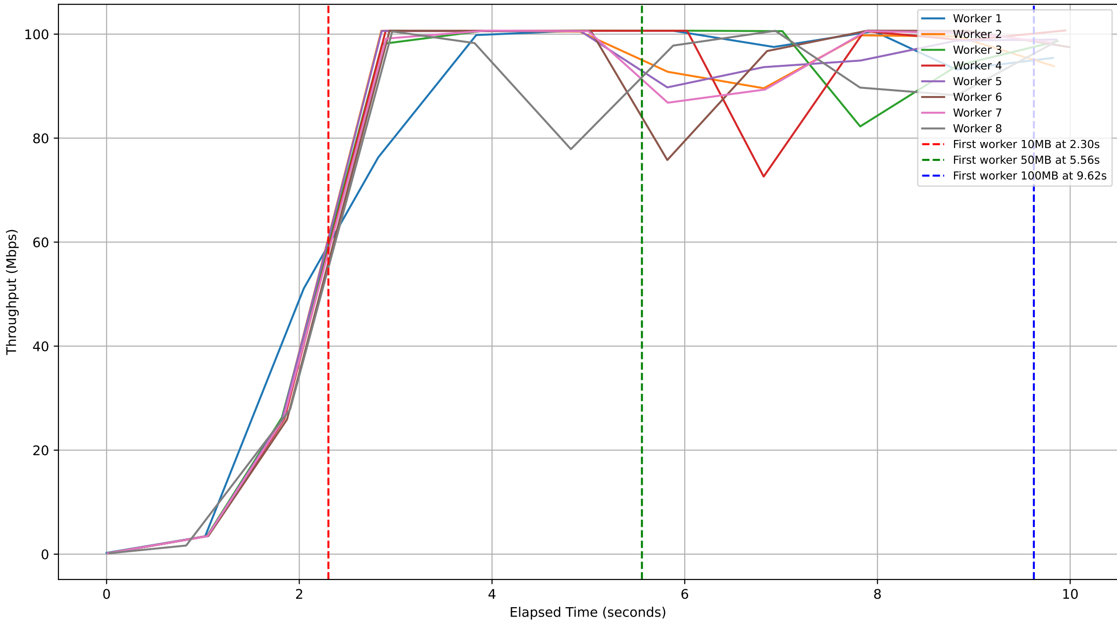
Subjob ID: ad55438a-6f3e-44c8-b9fe-64cb5d8a7338 - Workers Throughput Over Time
