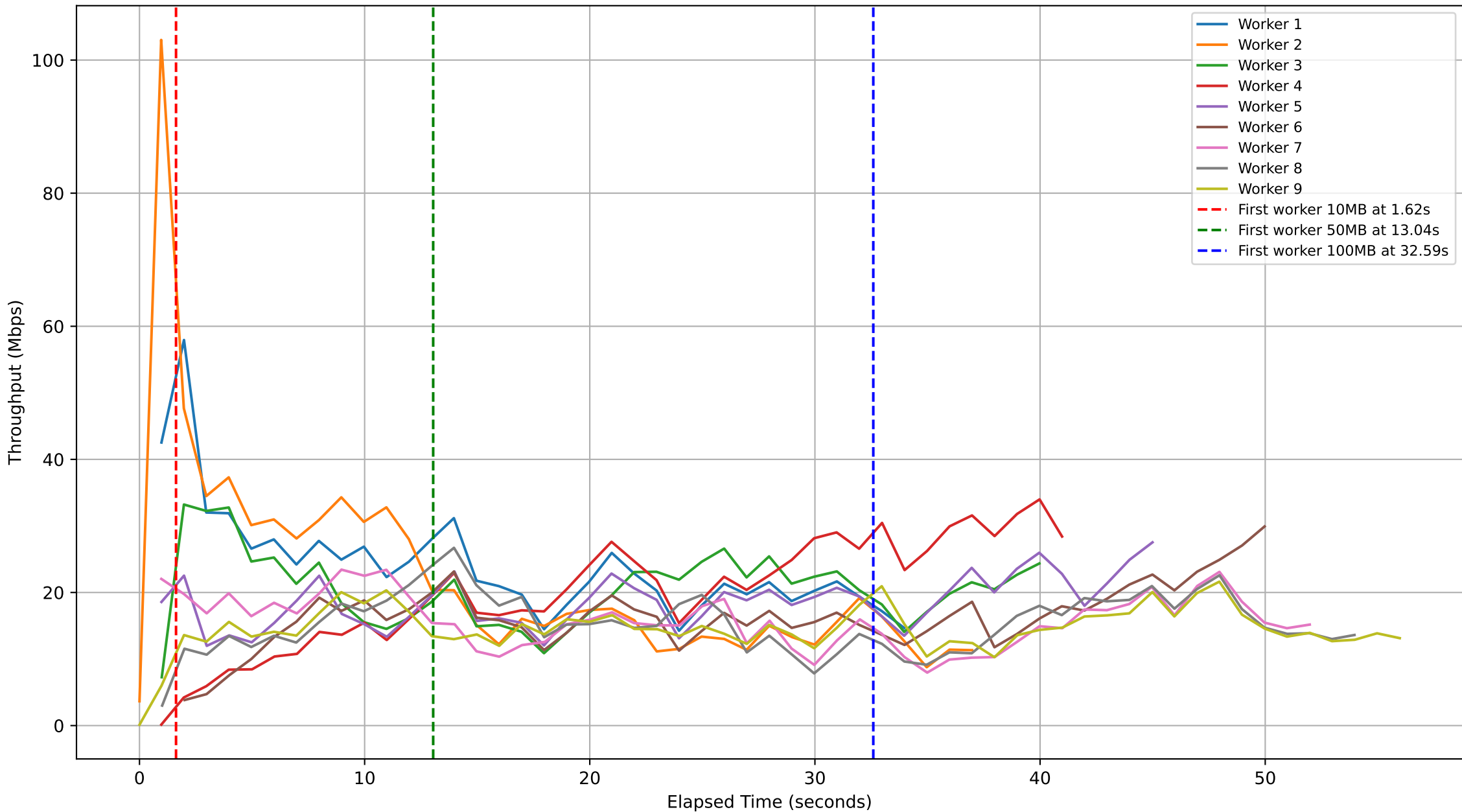
Subjob ID: 21b95281-18e7-45df-814b-70635dc55764 - Workers Throughput Over Time
