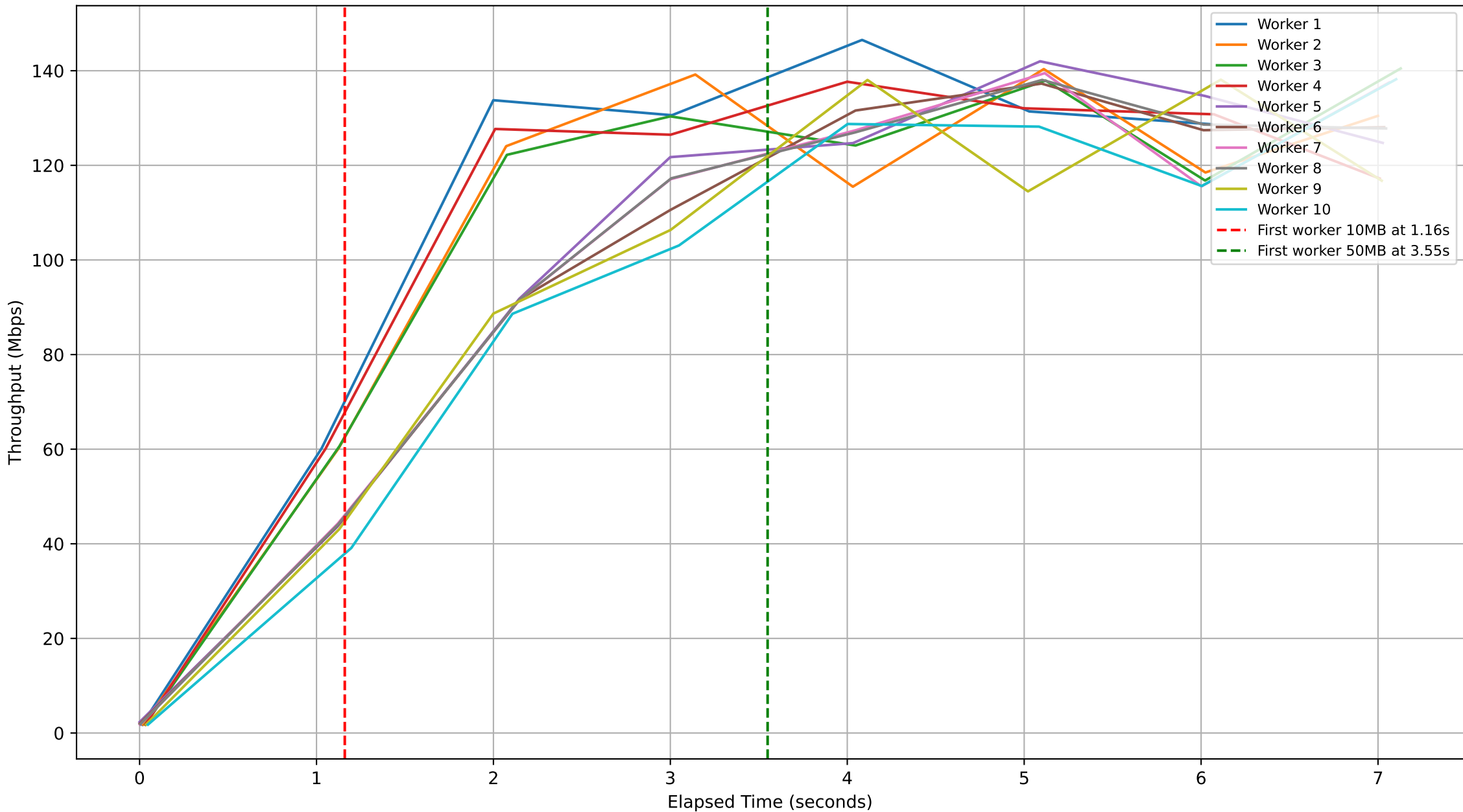
Subjob ID: c40afbb4-0293-491b-b2b4-6cc57abba68b - Workers Throughput Over Time
