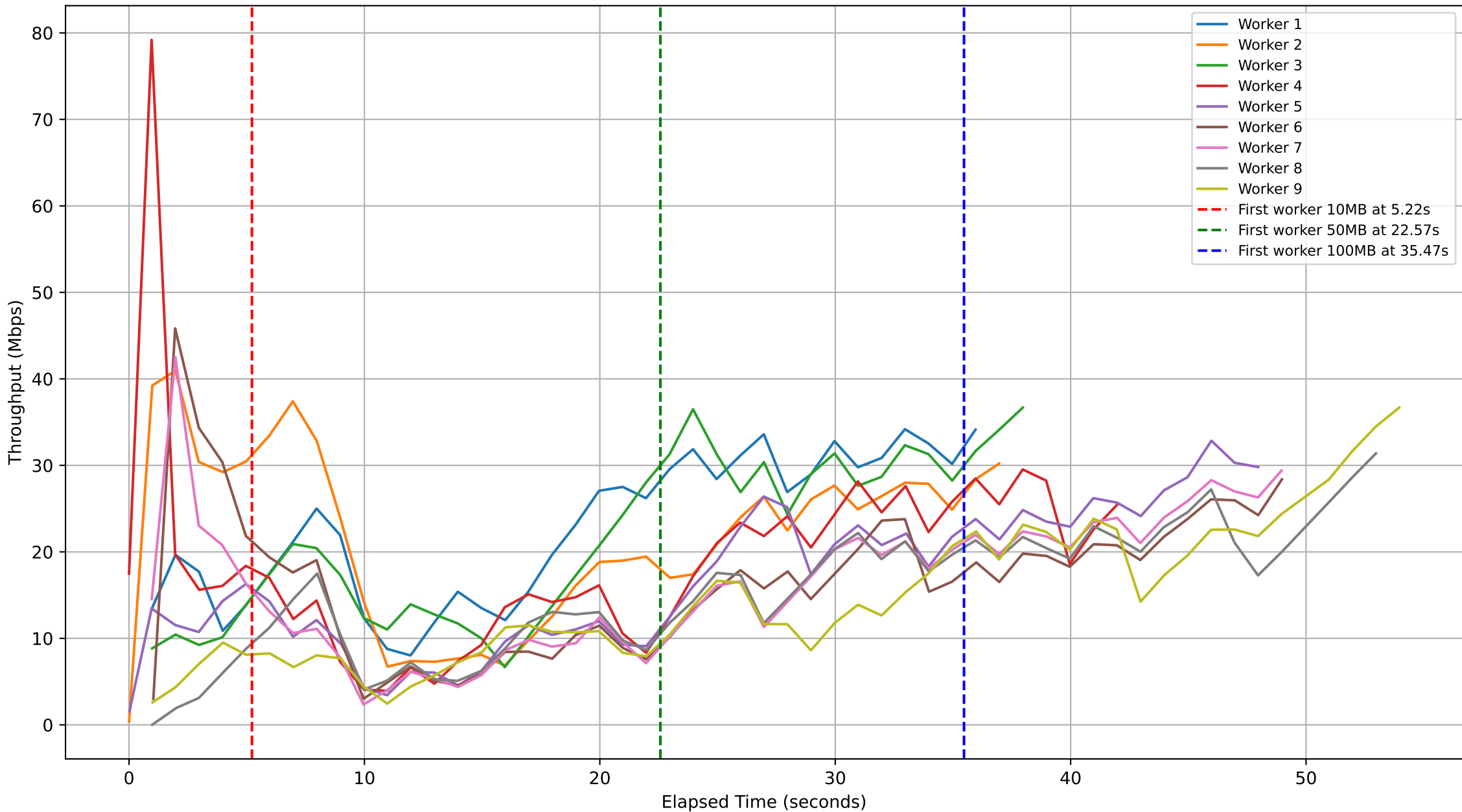
Subjob ID: 9b6b74aa-de3c-46ea-a42c-df737ab824ae - Workers Throughput Over Time
