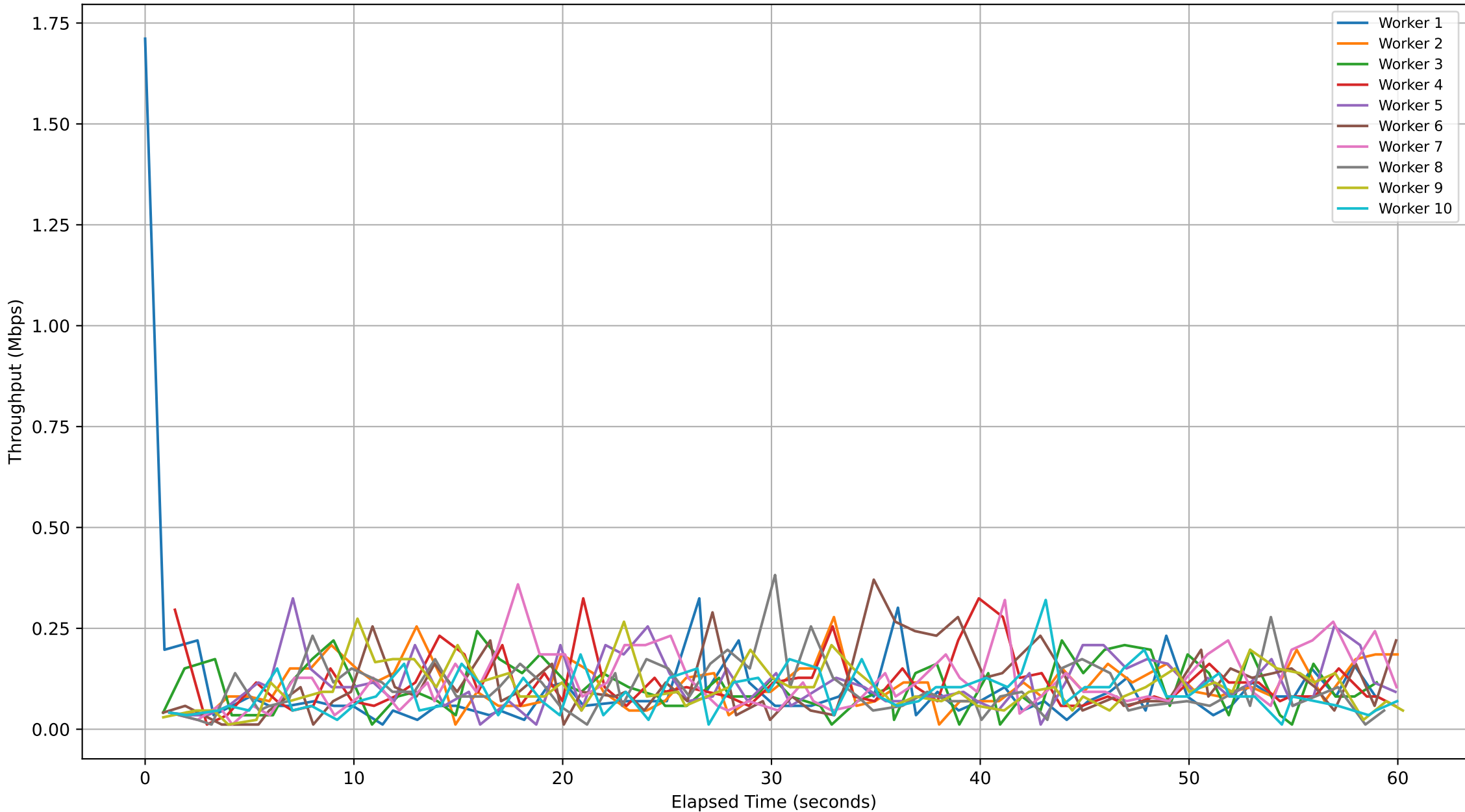
Subjob ID: 5dd2076f-224e-429a-bacc-38dcf541701e - Workers Throughput Over Time
