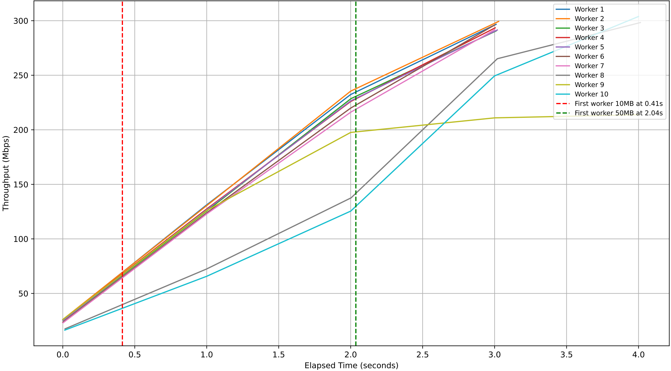
Subjob ID: eca3a3be-aa12-4de0-96dc-8036c011cf50 - Workers Throughput Over Time
