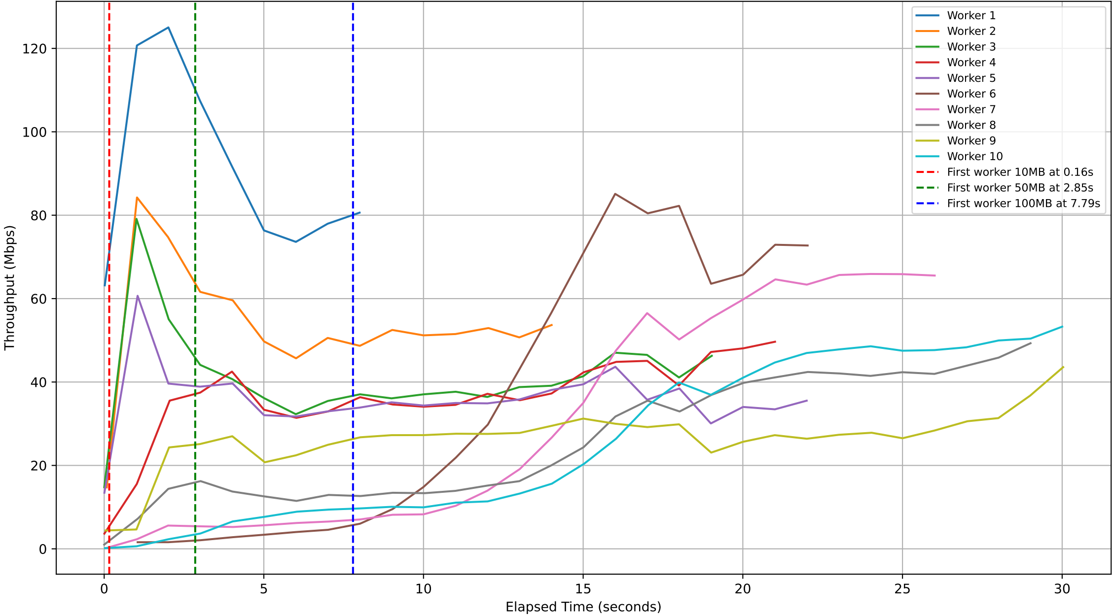
Subjob ID: 880f65ae-7f5a-4741-8ad5-e254c23c987b - Workers Throughput Over Time
