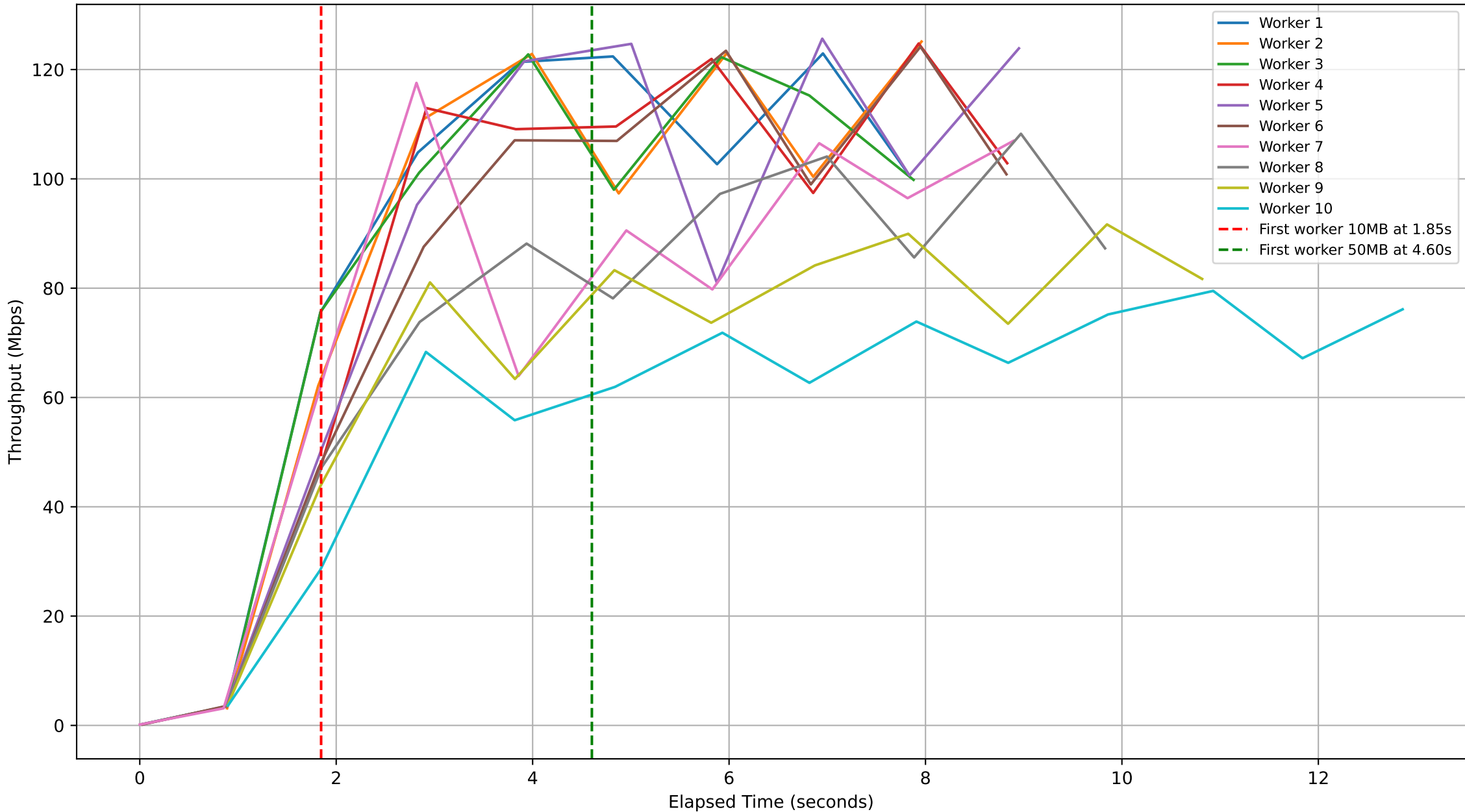
Subjob ID: e44cfb32-b886-48dd-b920-c989cb71fa91 - Workers Throughput Over Time
