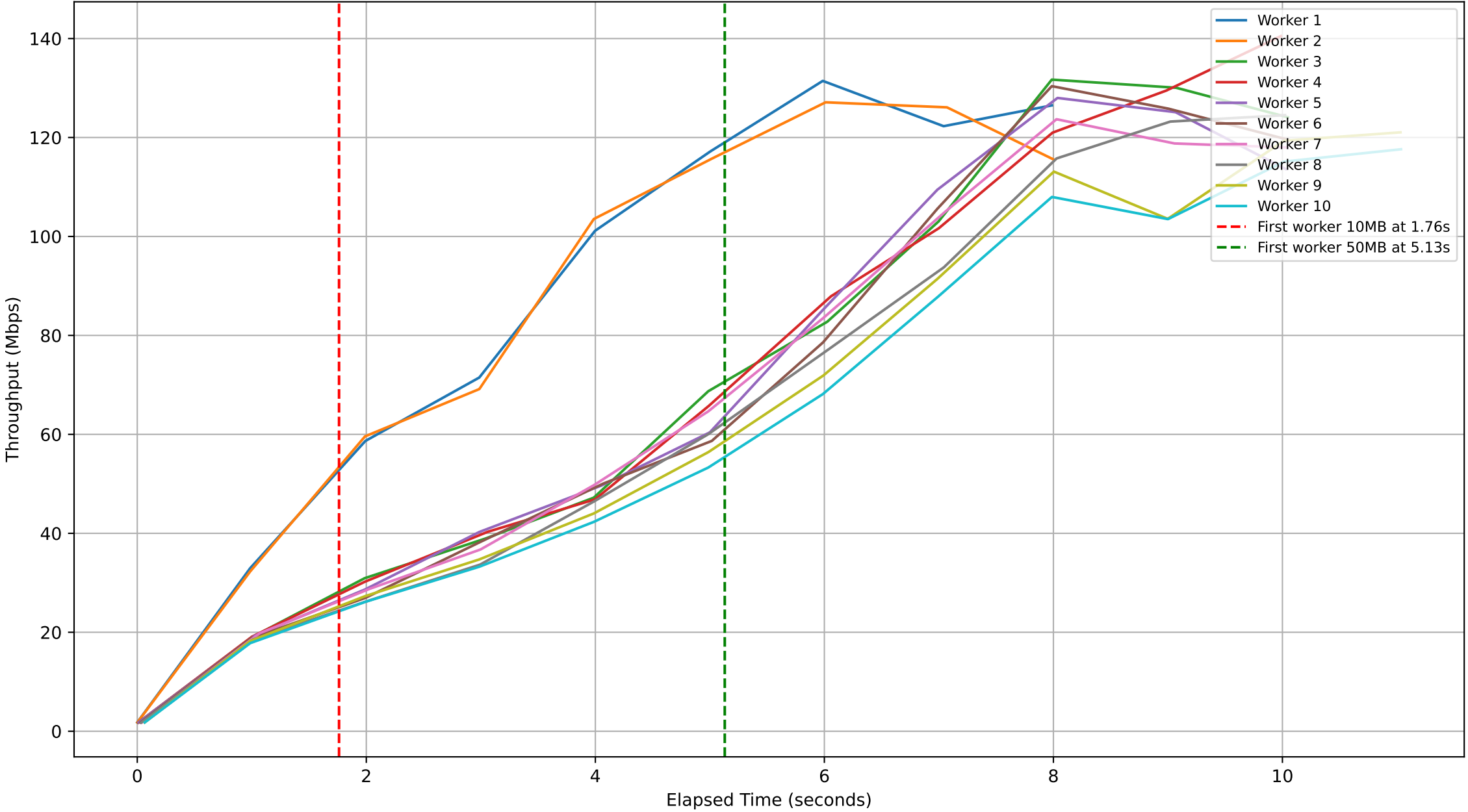
Subjob ID: 4083e653-1fcc-40c4-8a71-9f9a12d0287c - Workers Throughput Over Time
