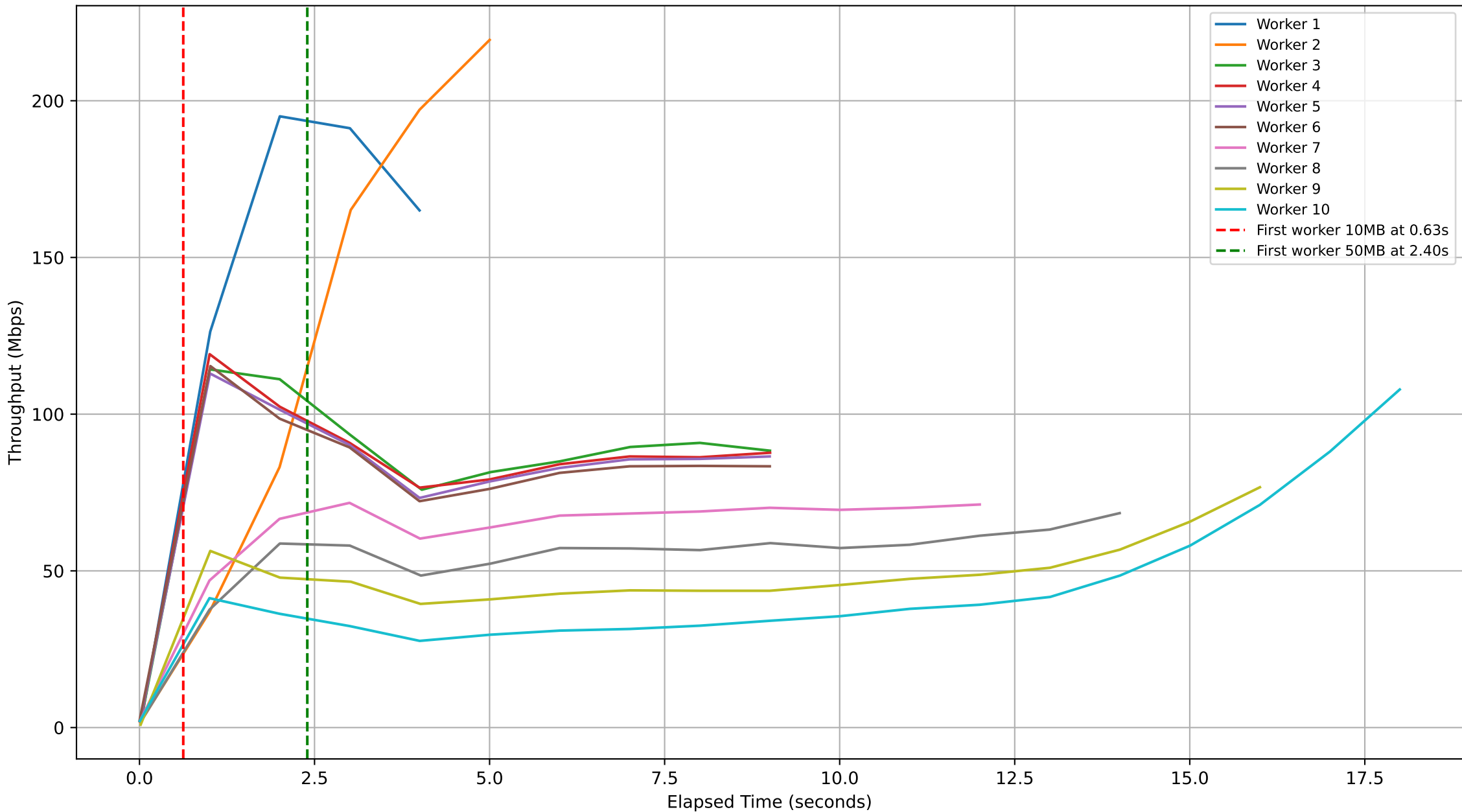
Subjob ID: b12d73b0-20be-4c8b-9f2e-bee48f0f36a4 - Workers Throughput Over Time
