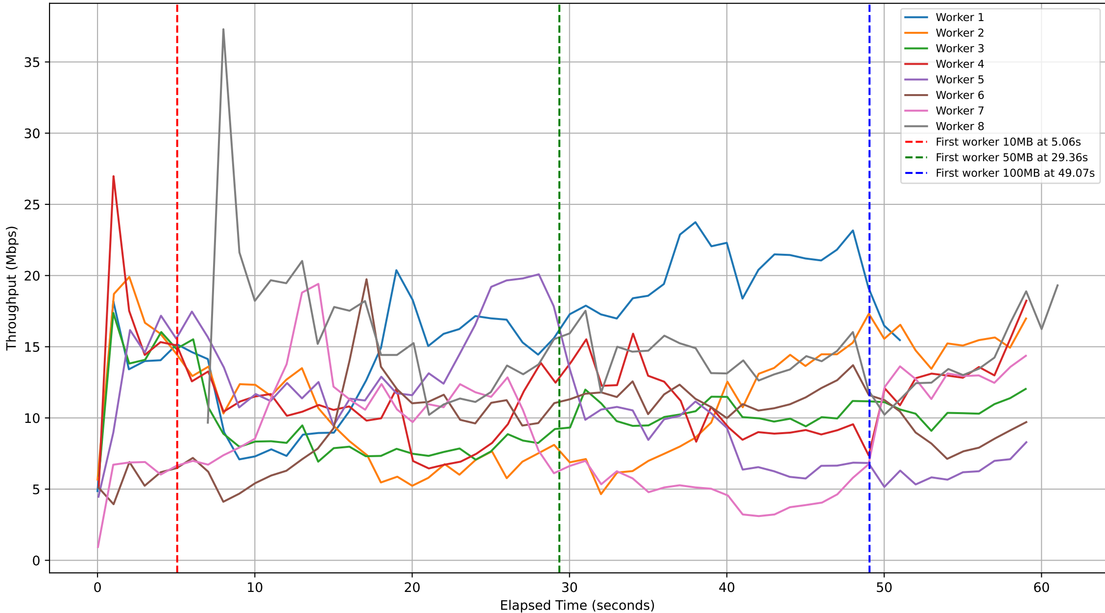
Subjob ID: ba90e1fc-bade-4c4f-bdf9-1980da6ab1ec - Workers Throughput Over Time
