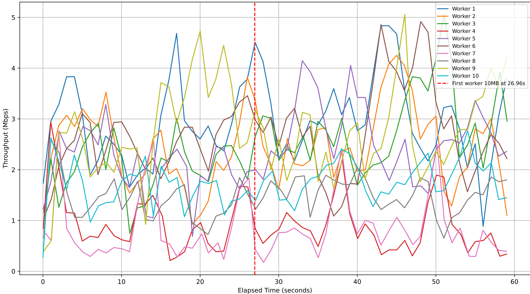
Subjob ID: af07d920-533f-4b8f-bc72-bde5e1d6c61b - Workers Throughput Over Time
