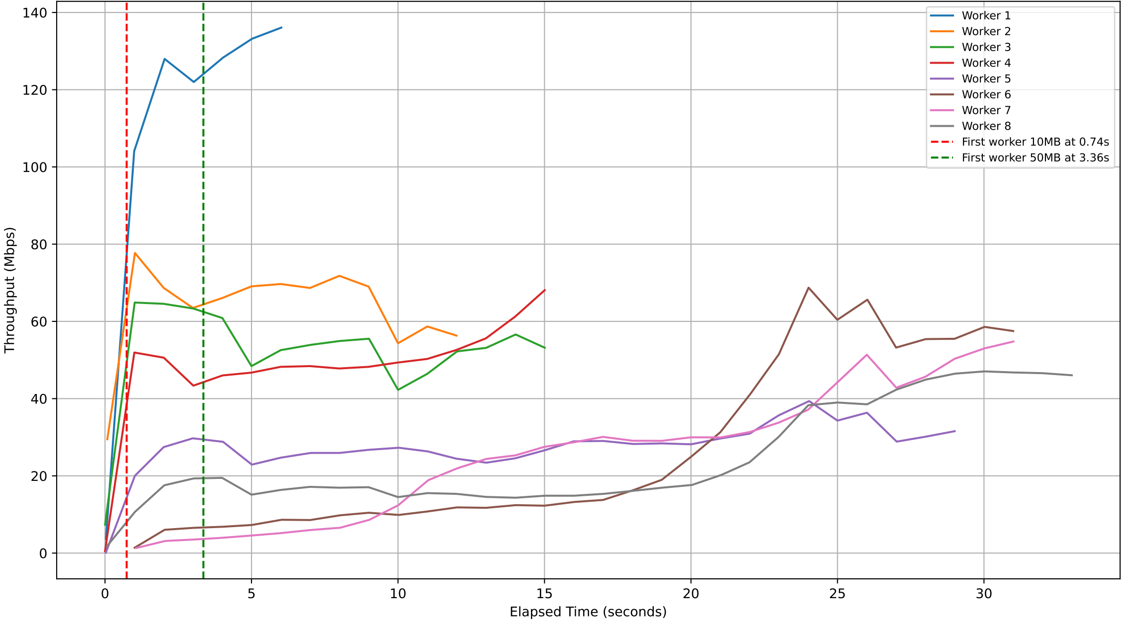
Subjob ID: bdf27886-2456-4282-9e3d-f02f911d58d8 - Workers Throughput Over Time
