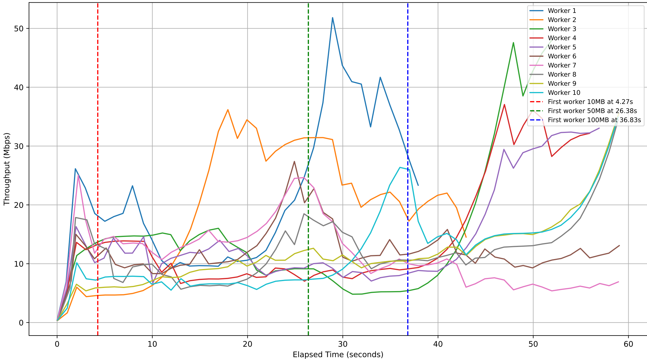
Subjob ID: c40033dd-289e-4e79-b0a4-e4fd62a8da97 - Workers Throughput Over Time
