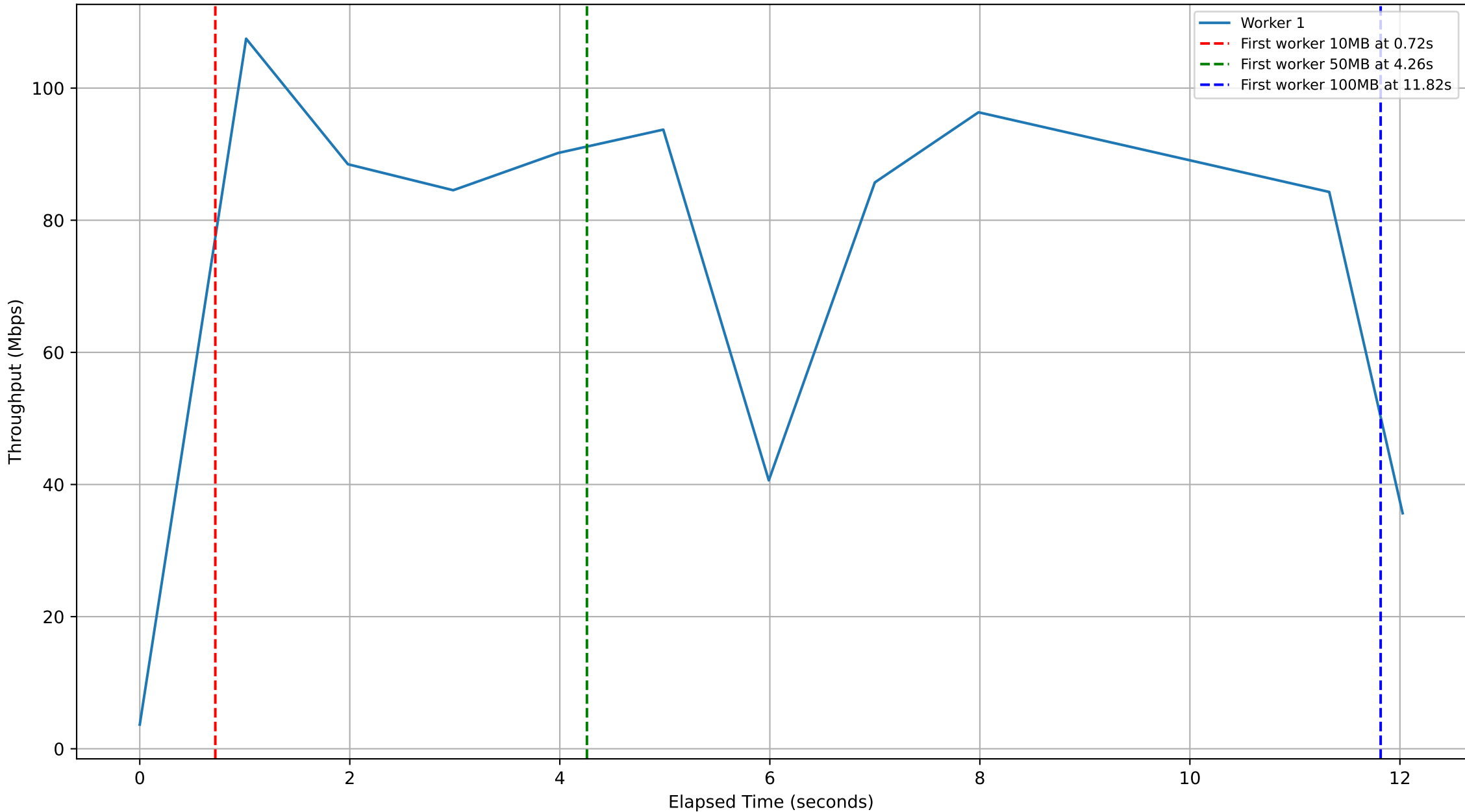
Subjob ID: 05e81d10-ea99-46c5-9856-54482b14ddcf - Workers Throughput Over Time
