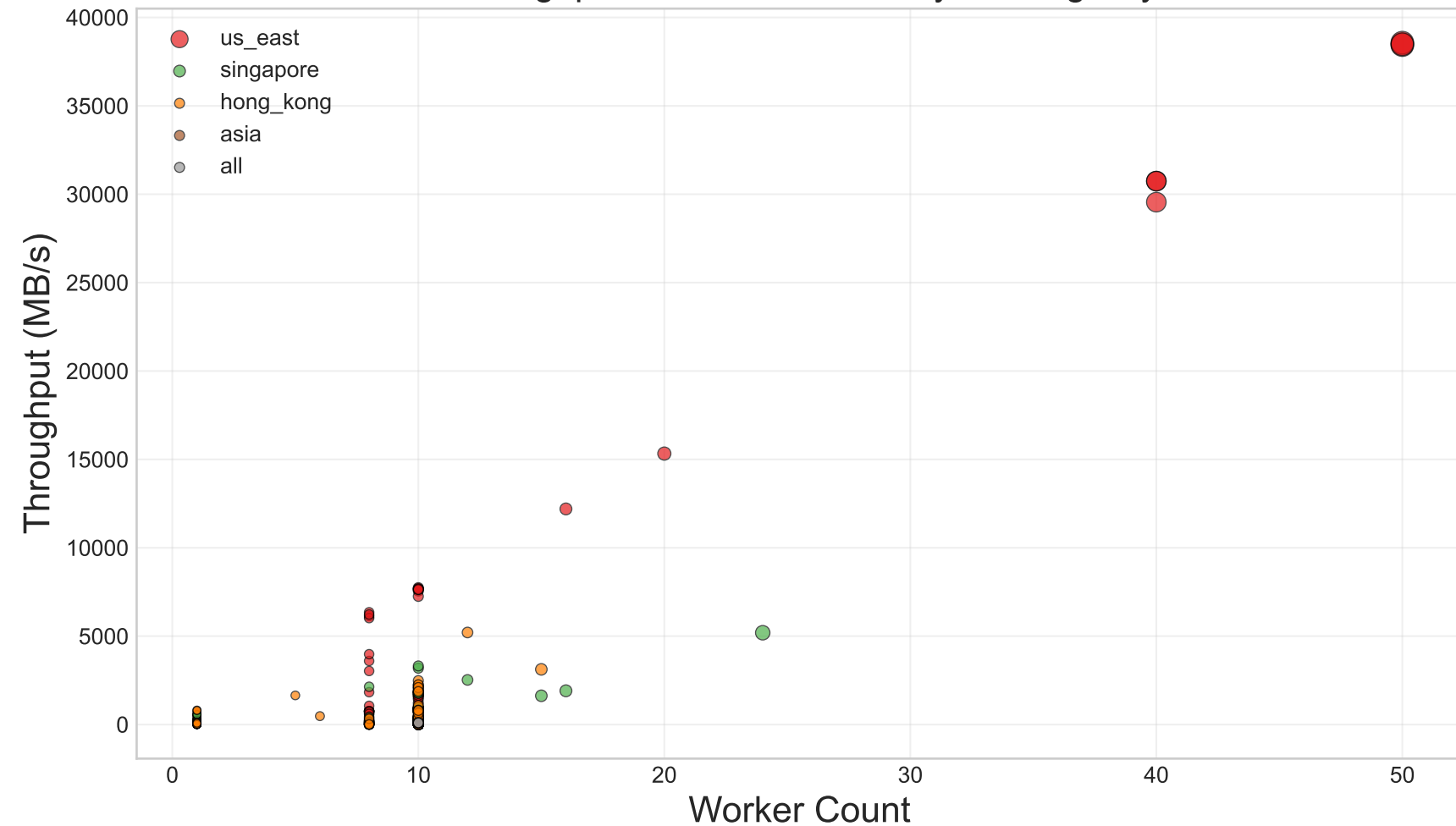
Throughput vs Worker Count by Routing Key
