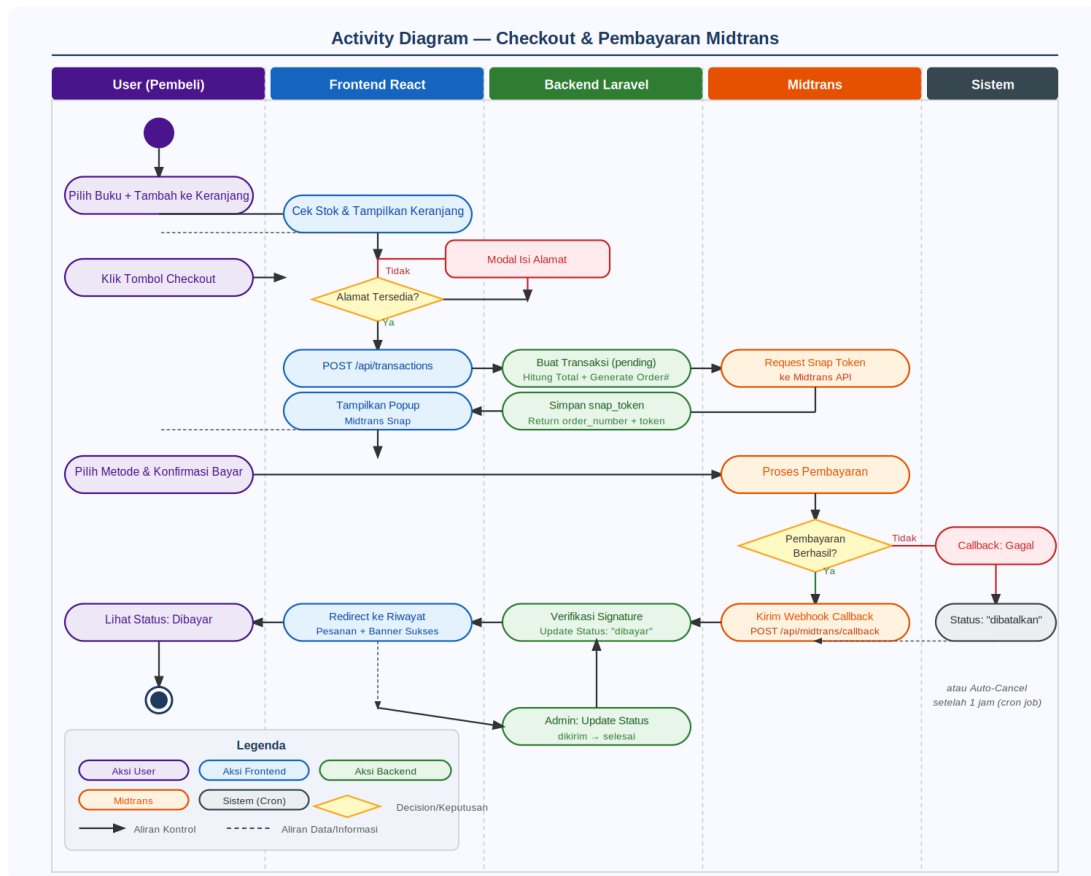
Gambar 7.2 — Activity Diagram: Checkout &amp; Pembayaran Midtrans
