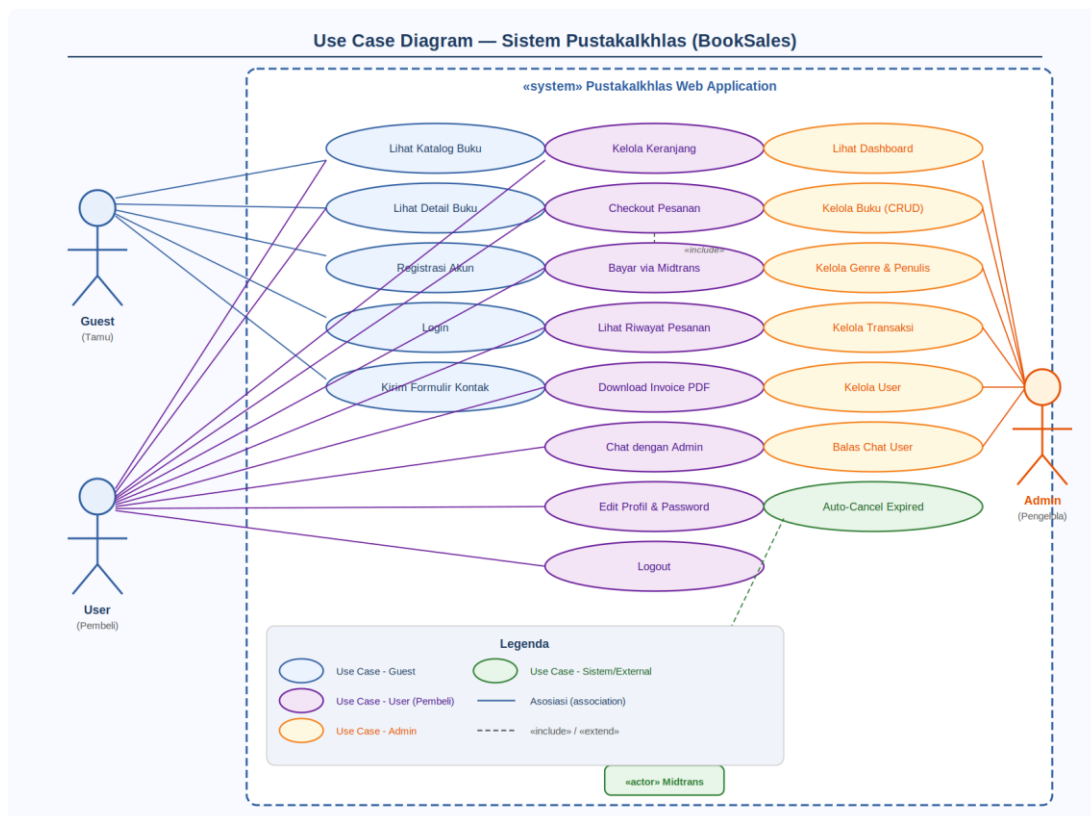
Gambar 6.1 — Use Case Diagram Sistem Pustakalkhlas (BookSales)
