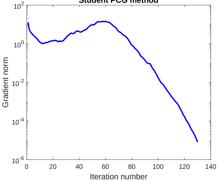
Student PCG method
