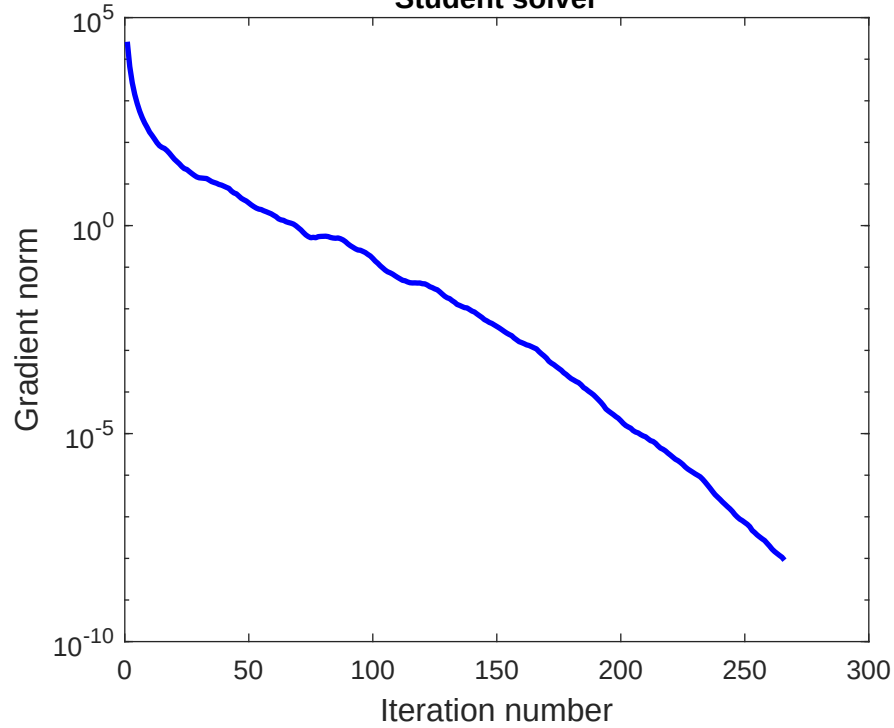
Student solver
