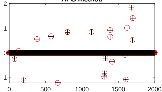
APG method
