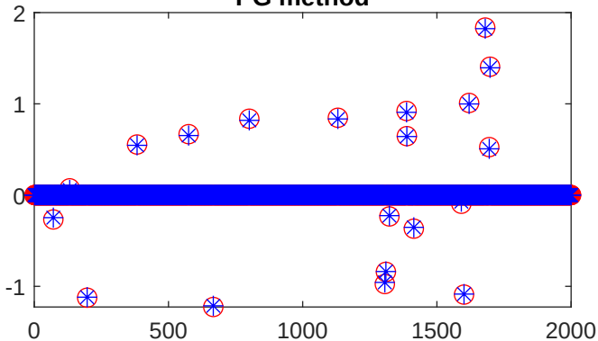
PG method
