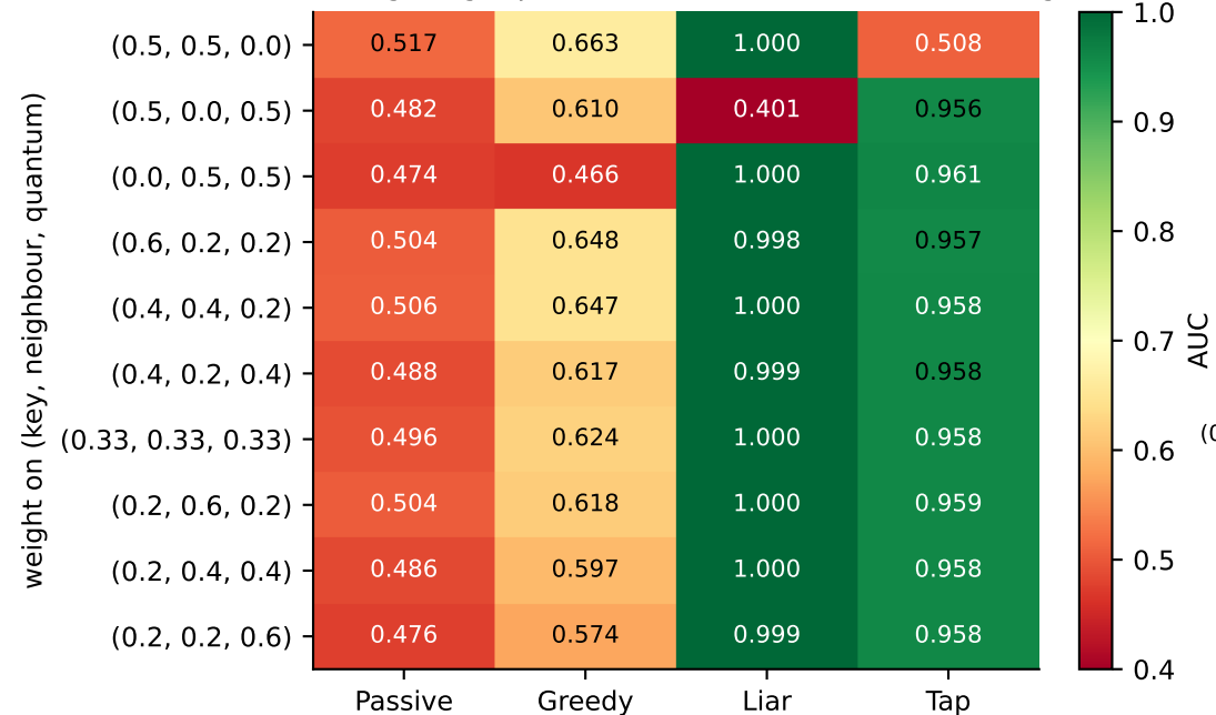
dropping w_k kills exactly profile k ; re-weighting a present feature does almost nothing
