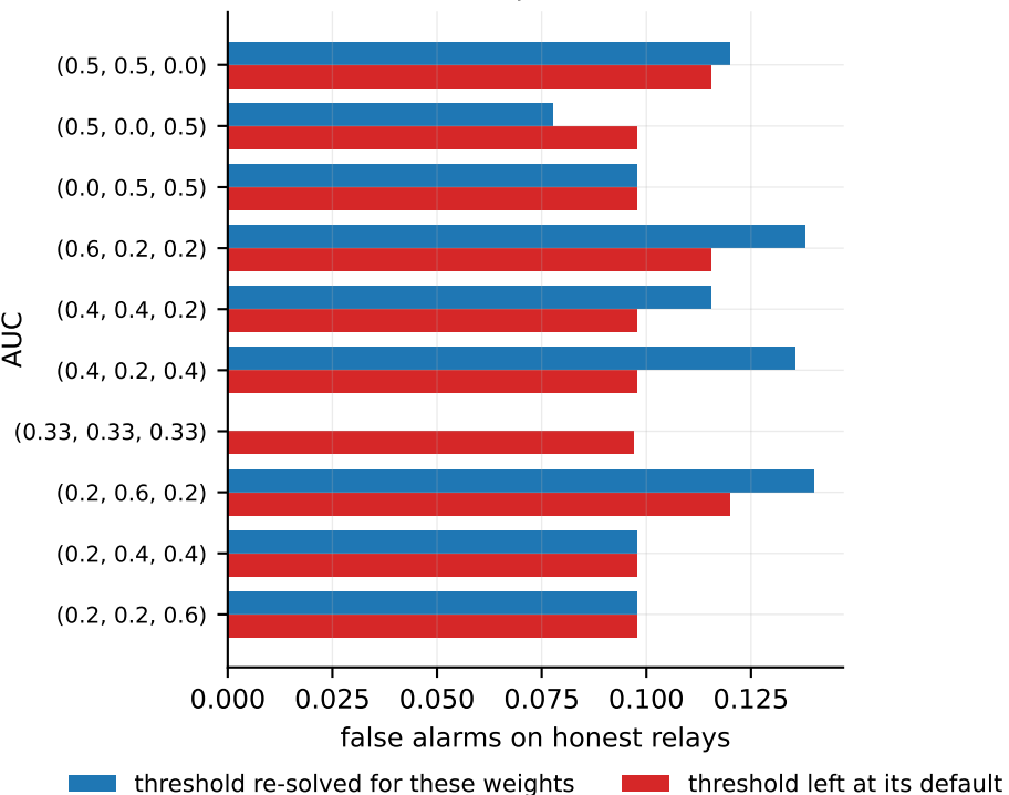
the same weights, judged on a threshold-dependent metric
