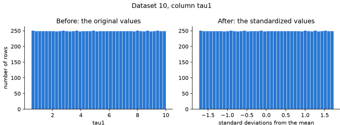
Column 0 of dataset 10, before and after standardization.
