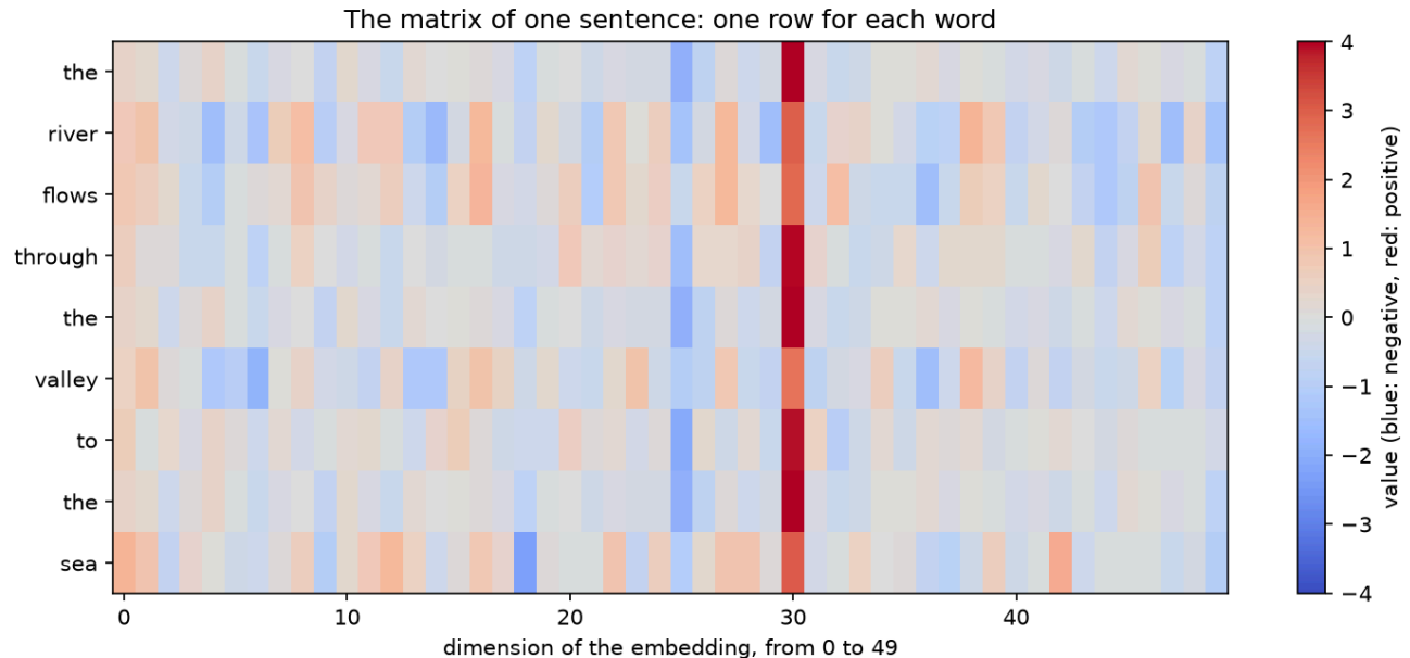
The matrix of one sentence: one row for each word, fifty columns.
