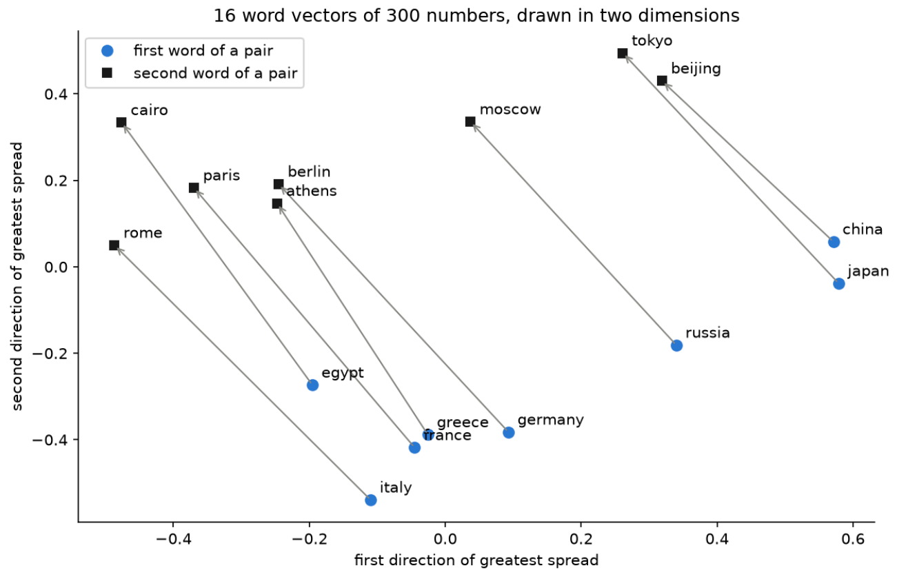
Eight countries and their capitals, drawn in the two directions of greatest spread.
