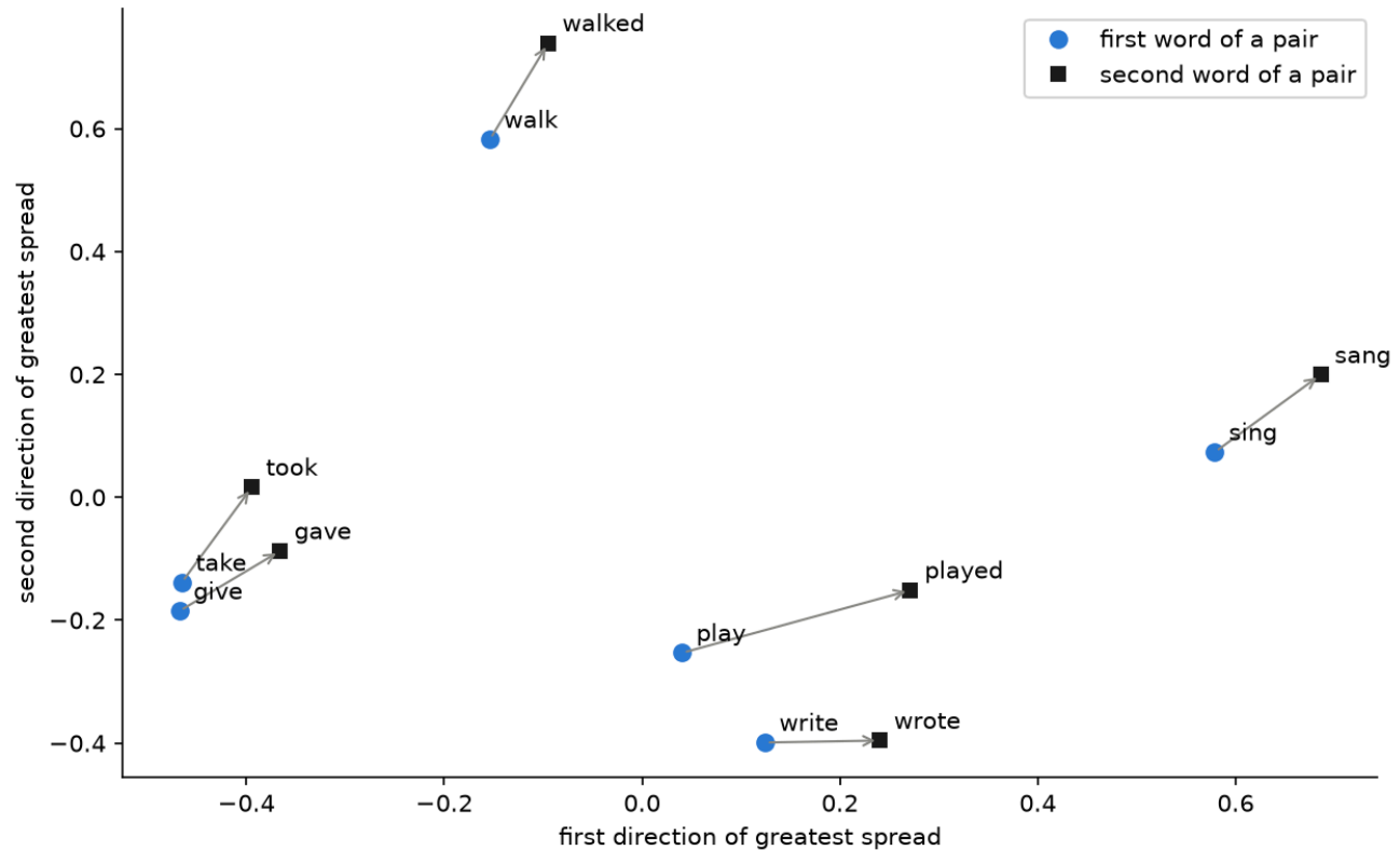
12 word vectors of 300 numbers, drawn in two dimensions
