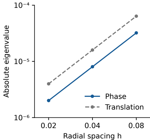
b Expected symmetry zero modes
