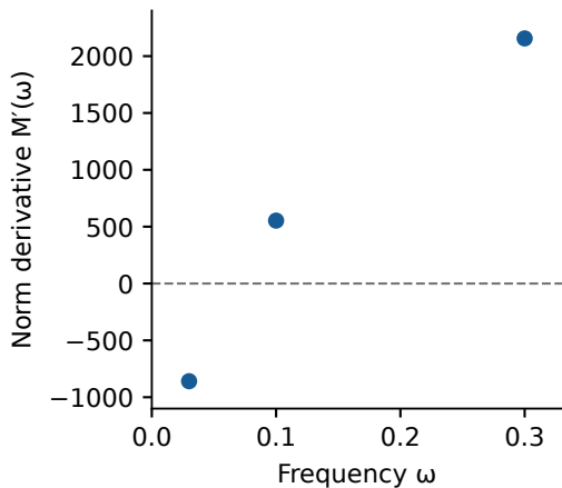
a Branch-specific slope evidence
