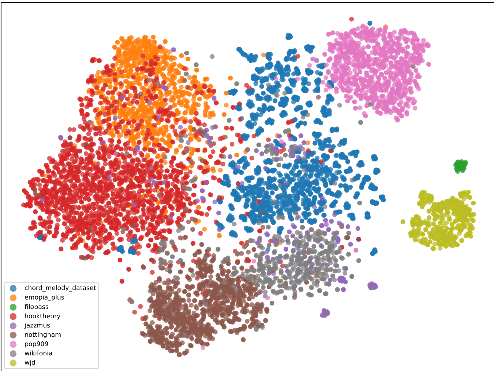
t-SNE of CLaMP2 music embeddings, colored by dataset
