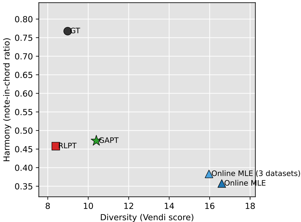
Melody condition from nottingham test set
